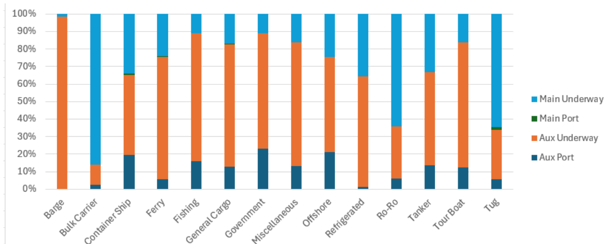
Figure 6 Ship Type Energy Distribution by Ship Type, Engine Type, and Port/Underway
