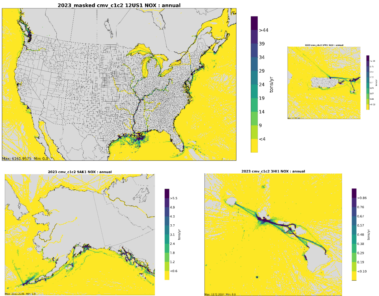
Figure 5 2023 Annual C1C2 NO x Emissions
