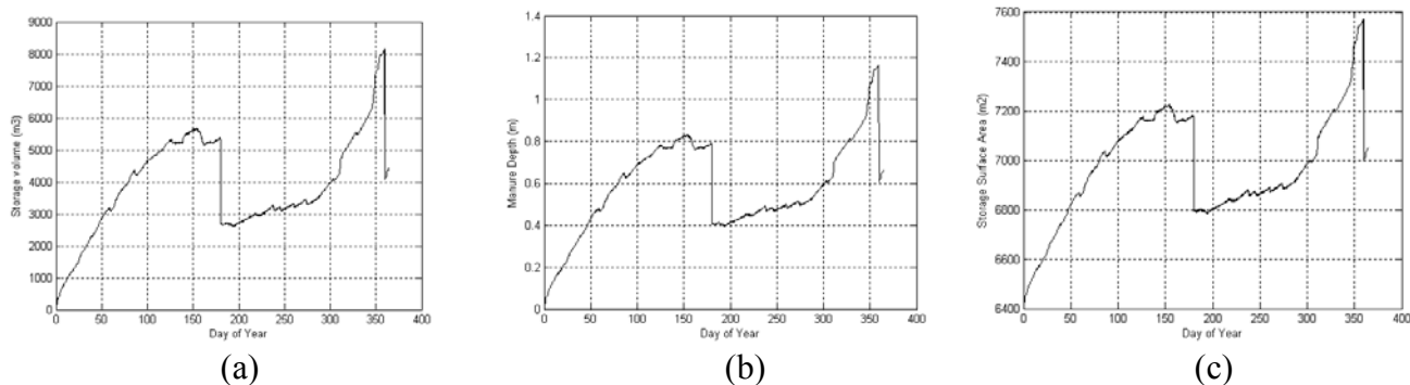
Figure 11. Predicted manure volume (a), depth (b), and surface area (c) in storage over one year period.
