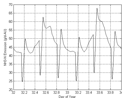
Figure 4. Predicted ammonia emission rate for two days in February.
