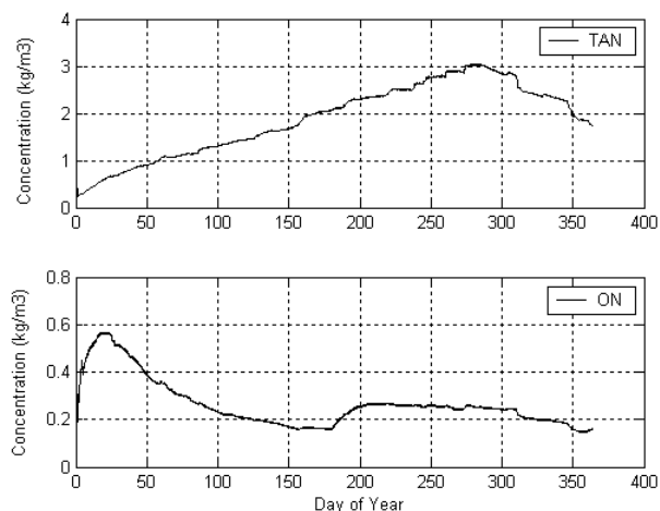
Figure 10. Predicted ammoniacal nitrogen (TAN) and organic nitrogen (ON) concentrations in storage over one-year period.
