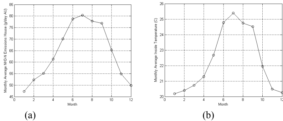
Figure 6. Predicted ammonia emission rate as monthly averages (a) in comparison with monthly average temperature inside the house (b).
