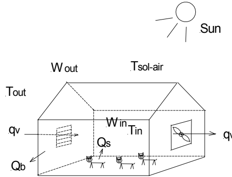
Figure 3. Swine housing model for ventilation rate and indoor temperature calculations.
