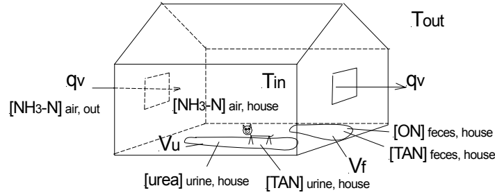
Figure 2. Swine housing model for ammonia emission calculations.
