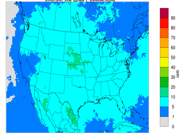
Natural Contrib. to CAMx Daily Max 8-Hour Ozone \geq 0 ppb
