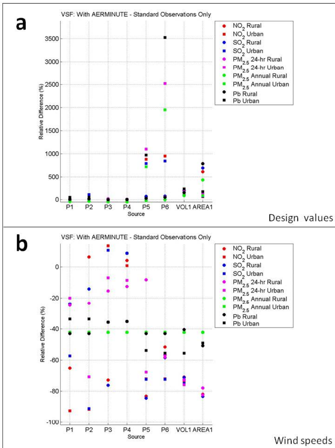
Figure B-2. VSF relative differences (AERMINUTE-standard observations only) for \text{NO}_2 , \text{SO}_2 , 24-hour and annual \text{PM}_{2.5} and lead: a) design values and b) mean wind speeds associated with design values.
