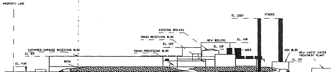
EAST ELEVATION
