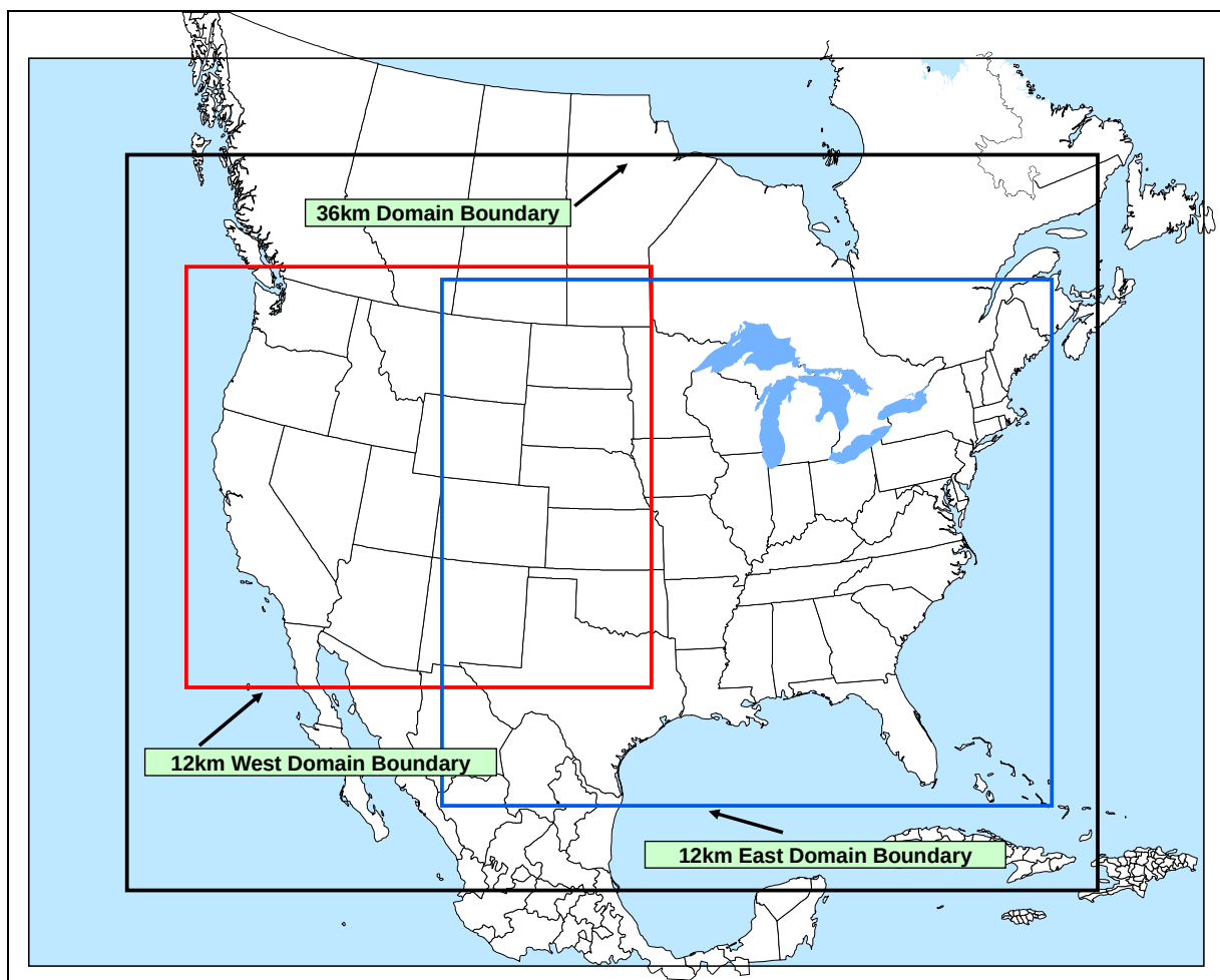
Figure 3-1. CMAQ modeling domains
