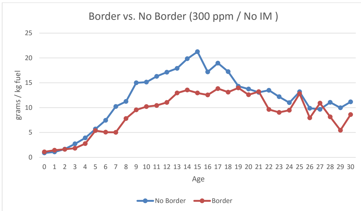
Figure 13: Border Effect for Passenger Car NO
