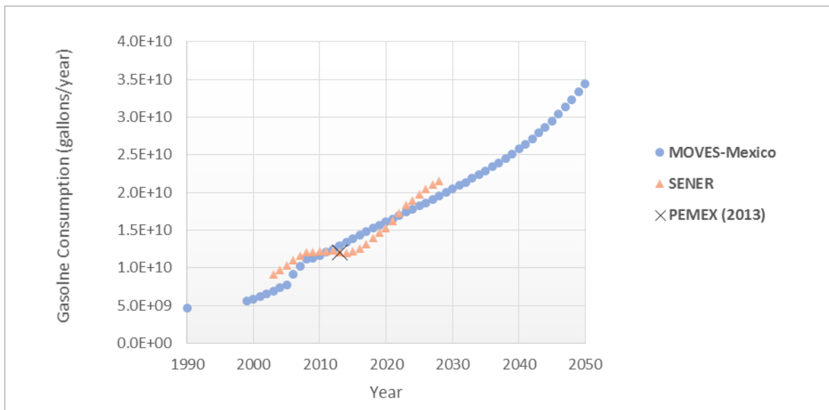
Figure 24: Gasoline Fuel Consumption
