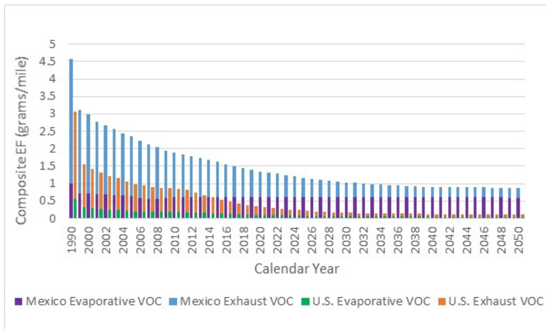
Figure 26: National Onroad VOC Emissions Per Mile Trend
