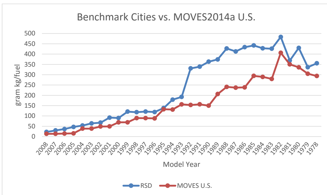
Figure 17: Benchmark RSD vs. MOVES U.S. (Passenger Car CO, inc. Taxis)
