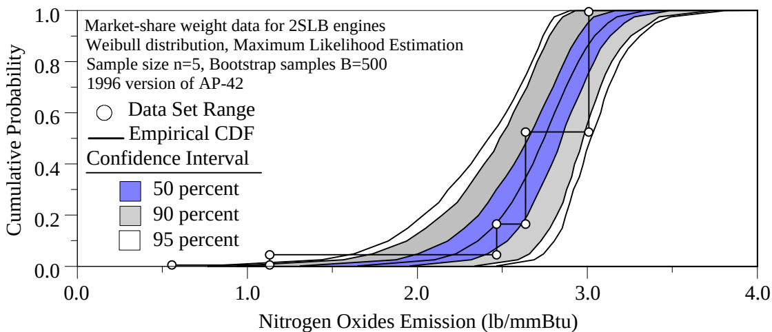
Figure 5. Comparison of the Empirical Distribution Bootstrap Simulation Results Based Upon a Weibull Distribution, Market-Share Weighted \text{NO}_x Emissions Rates, Treated as Unweighted data, Uncontrolled 2-Cycle Lean Burn Engines Based Upon October 1996 AP-42
