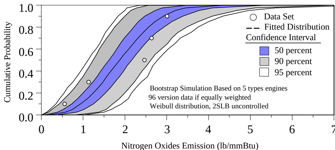
Figure 5. Comparison of the Empirical Distribution Bootstrap Simulation Results Based Upon a Weibull Distribution, Market-Share Weighted \text{NO}_x Emissions Rates, Treated as Unweighted data, Uncontrolled 2-Cycle Lean Burn Engines Based Upon October 1996 AP-42
