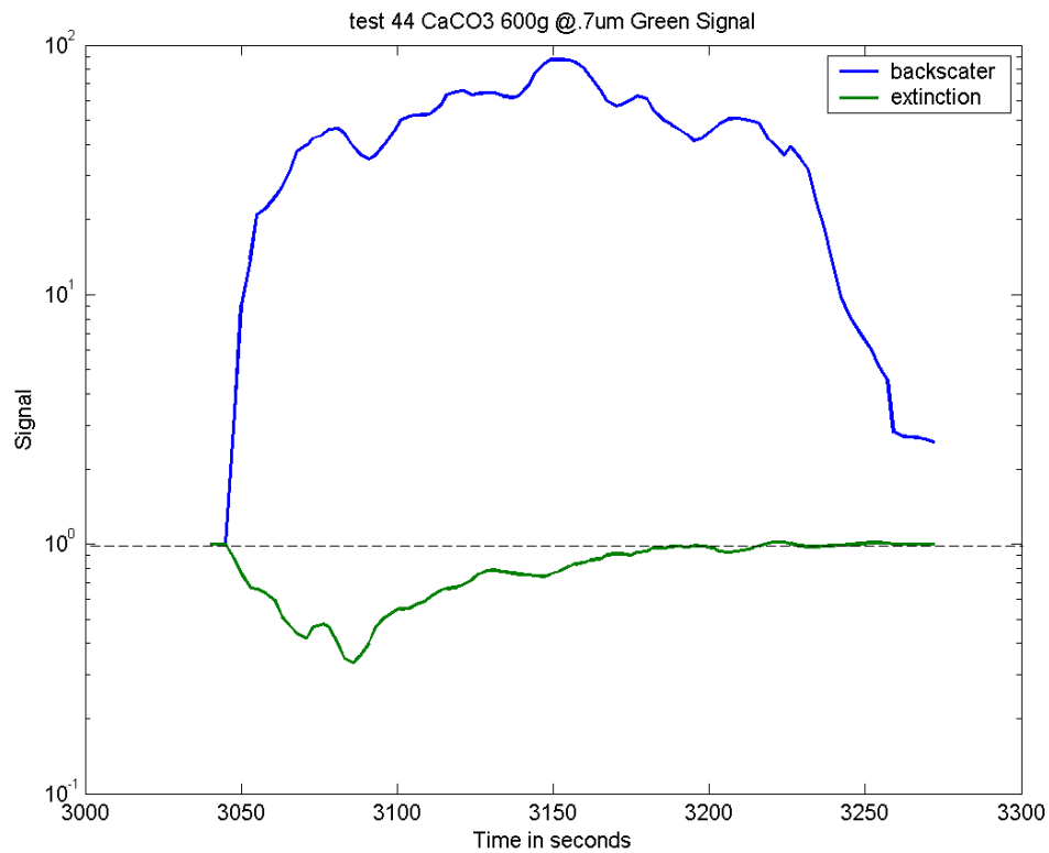
Figure 8. The open air time sequence of the lidar backscatter peak values and extinction values are shown for profiles of Test #44 on 19 December 2001 for the 0.7 \mu\text{m} CaCO 3 600 g sample.
