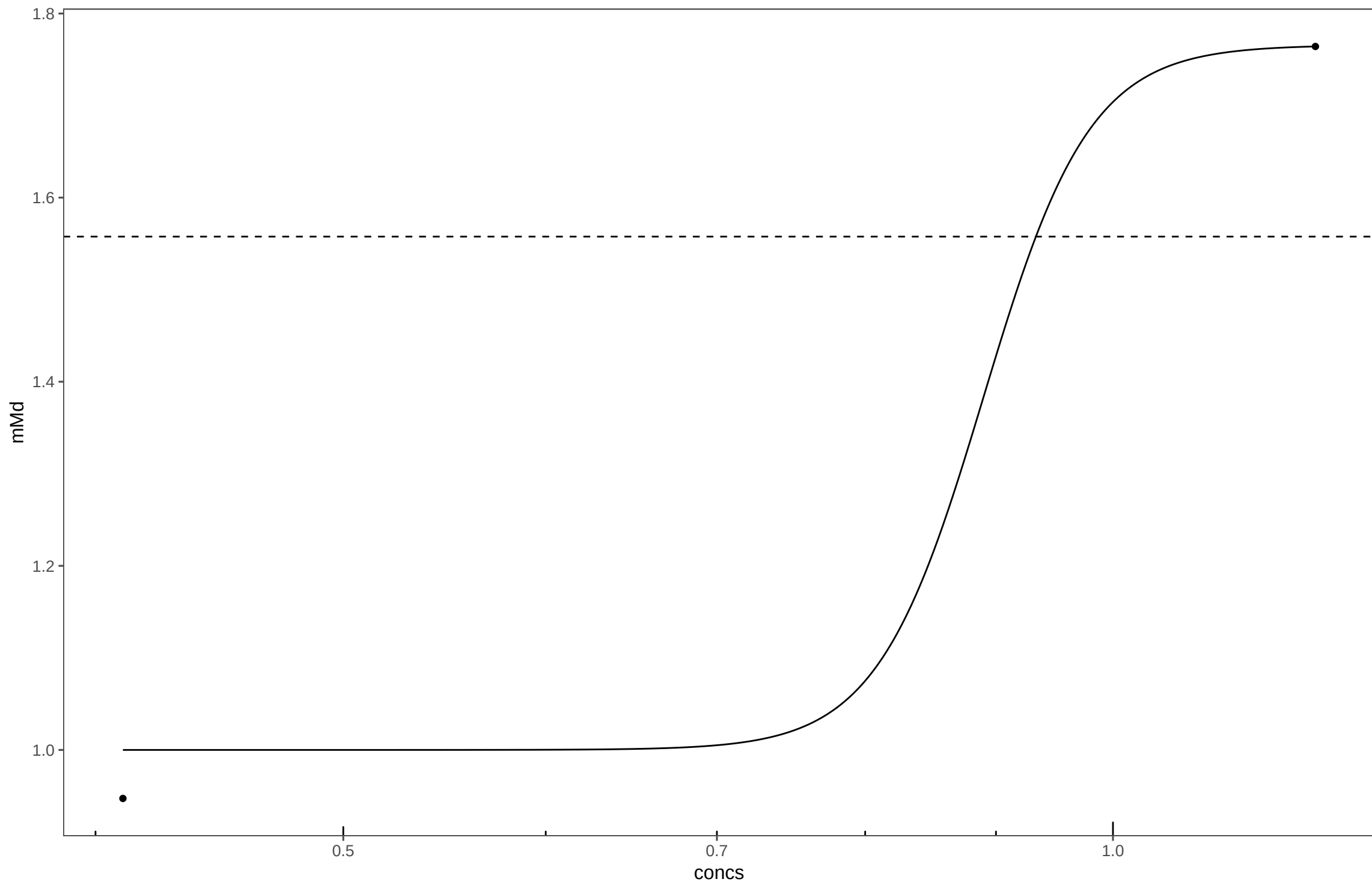
20140409_N,N'-Disalicylidene-1,2-diaminopropane_Plate17
