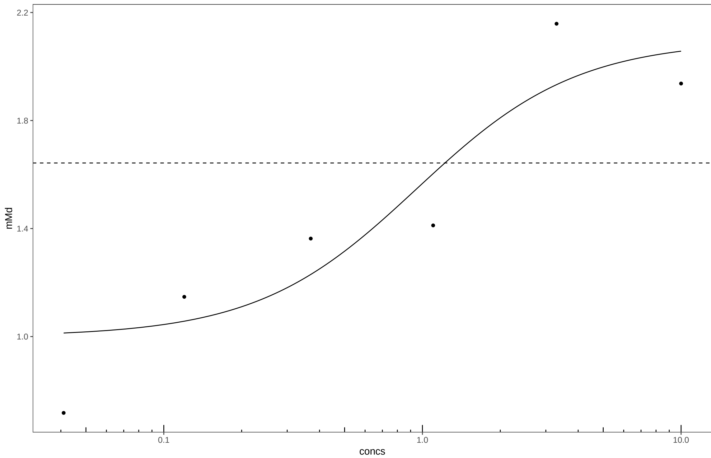
20150610_Z-Tetrachlorvinphos_Plate18
