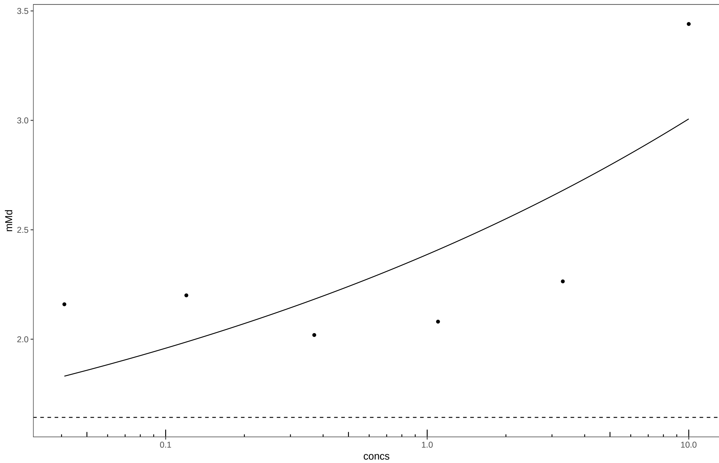
20130320_Tefluthrin_Plate7
