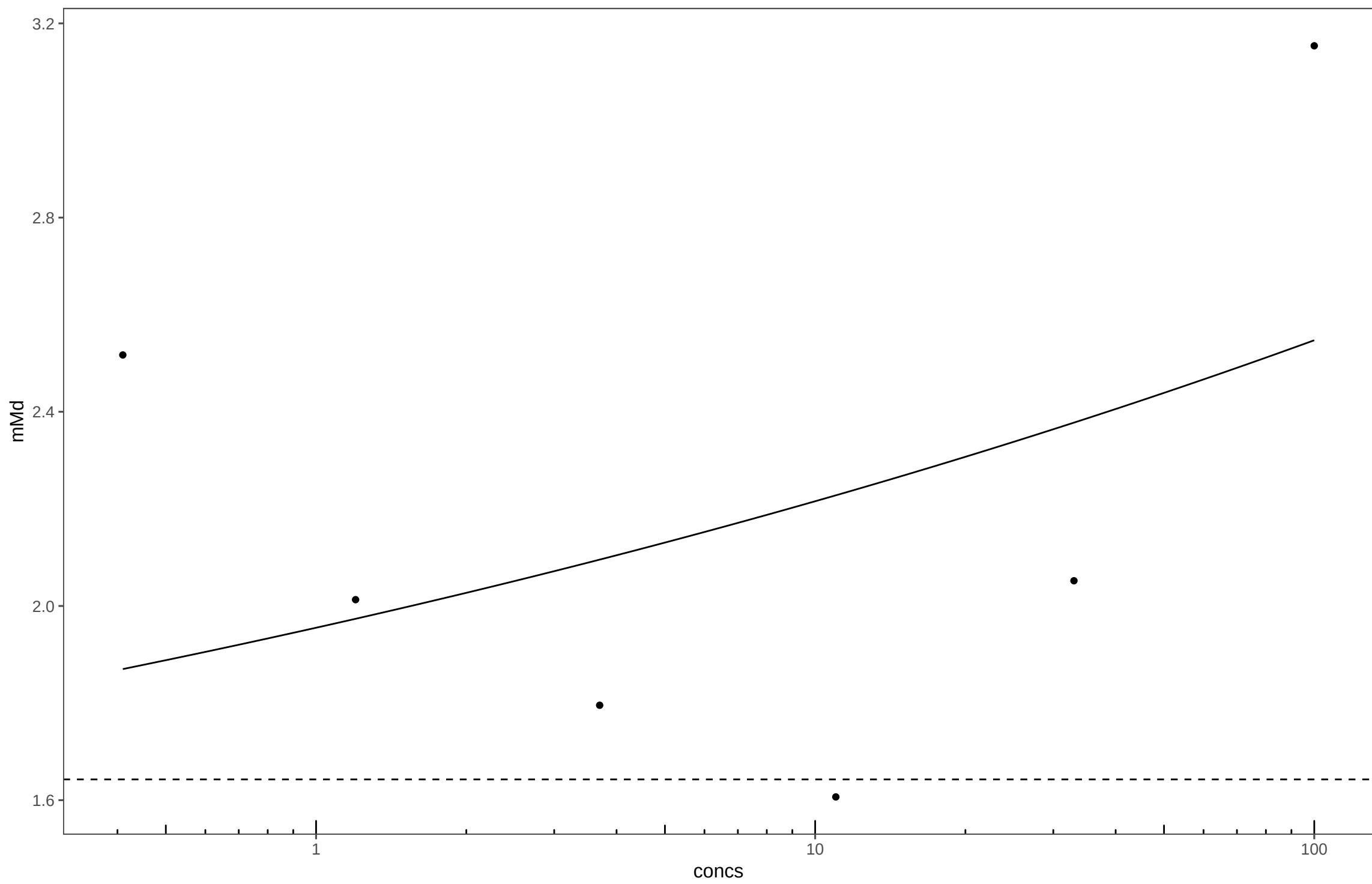
20150610_3-Hydroxy-2-pyridone_Plate23
