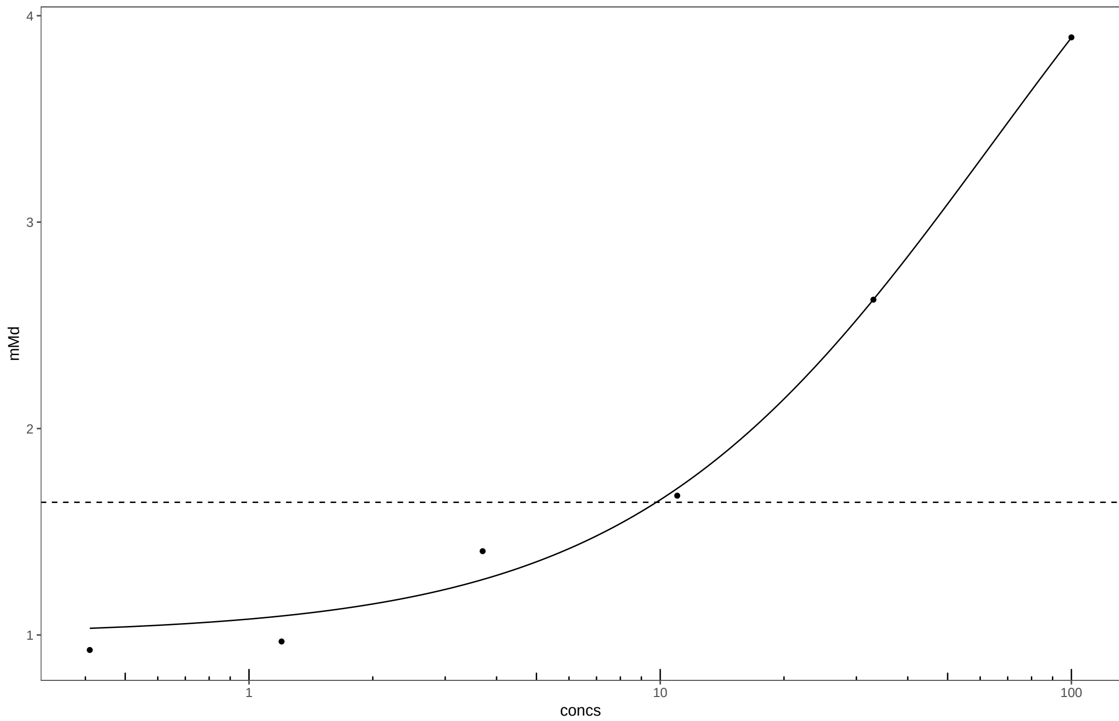
20170411_2,6-Dibromo-4-nitroaniline_Plate21
