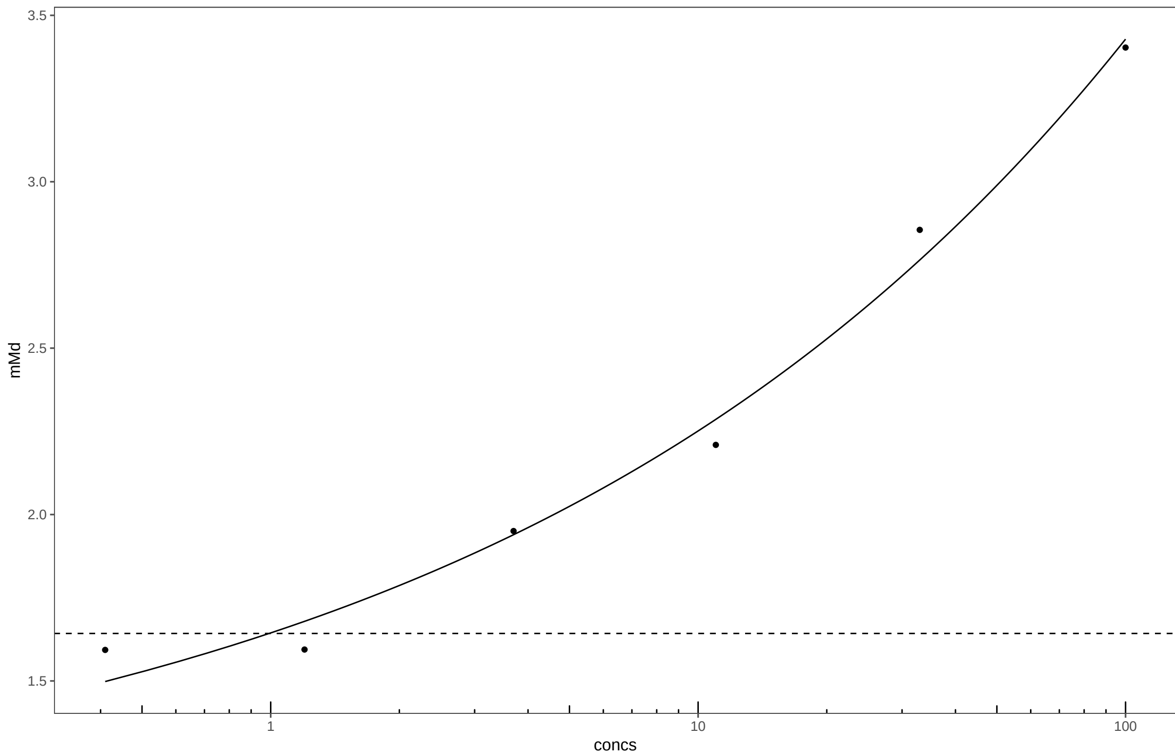
20150610_2,3-Dihydroxynaphthalene_Plate36
