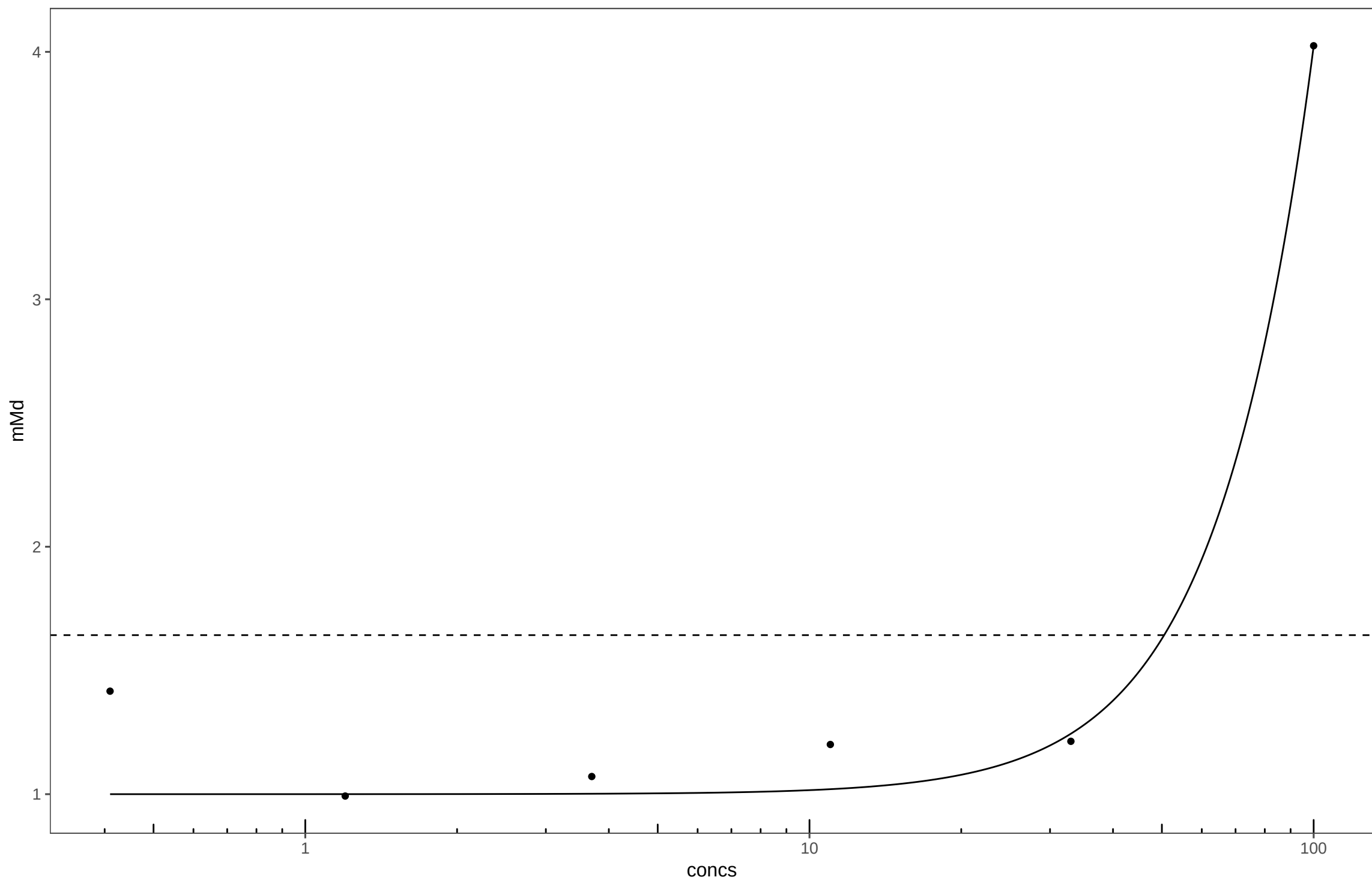
20140402_2,4,7,9-Tetramethyl-5-decyne-4,7-diol_Plate22
