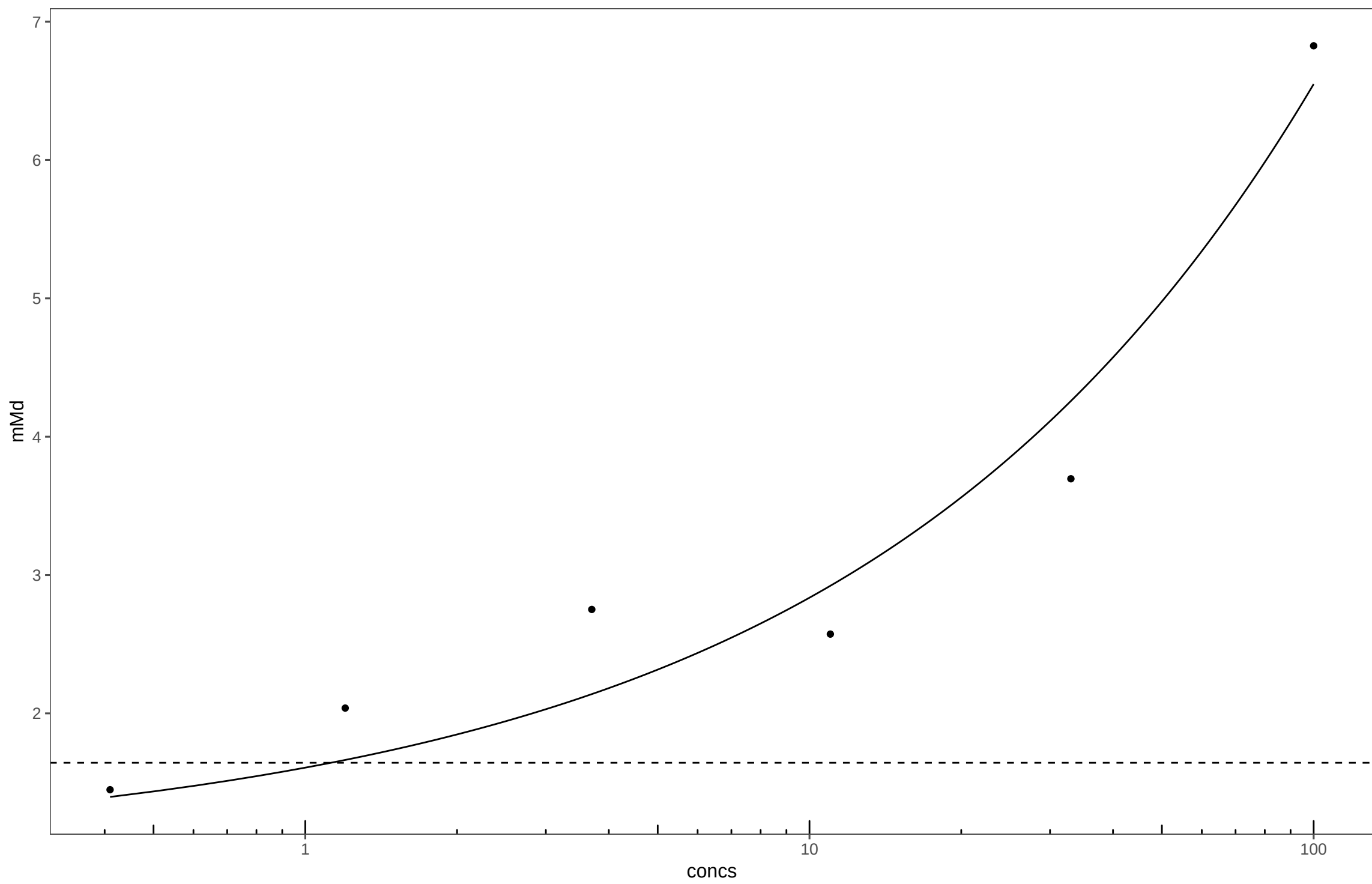
20150610_2-Chloro-5-nitroaniline_Plate39
