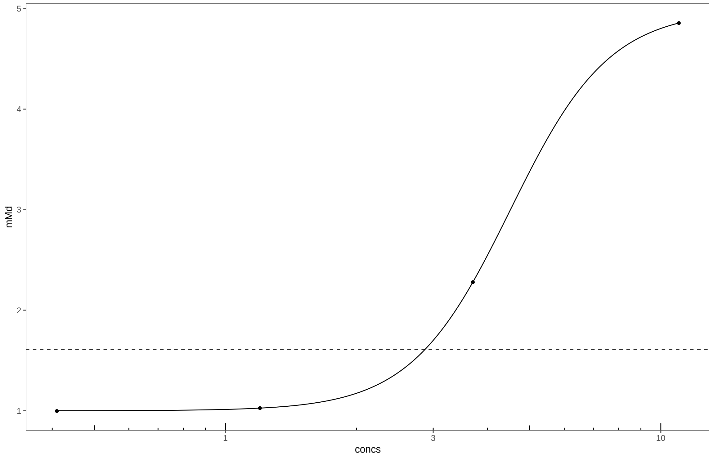
20170411_Diphenylmercury(II)_Plate19
