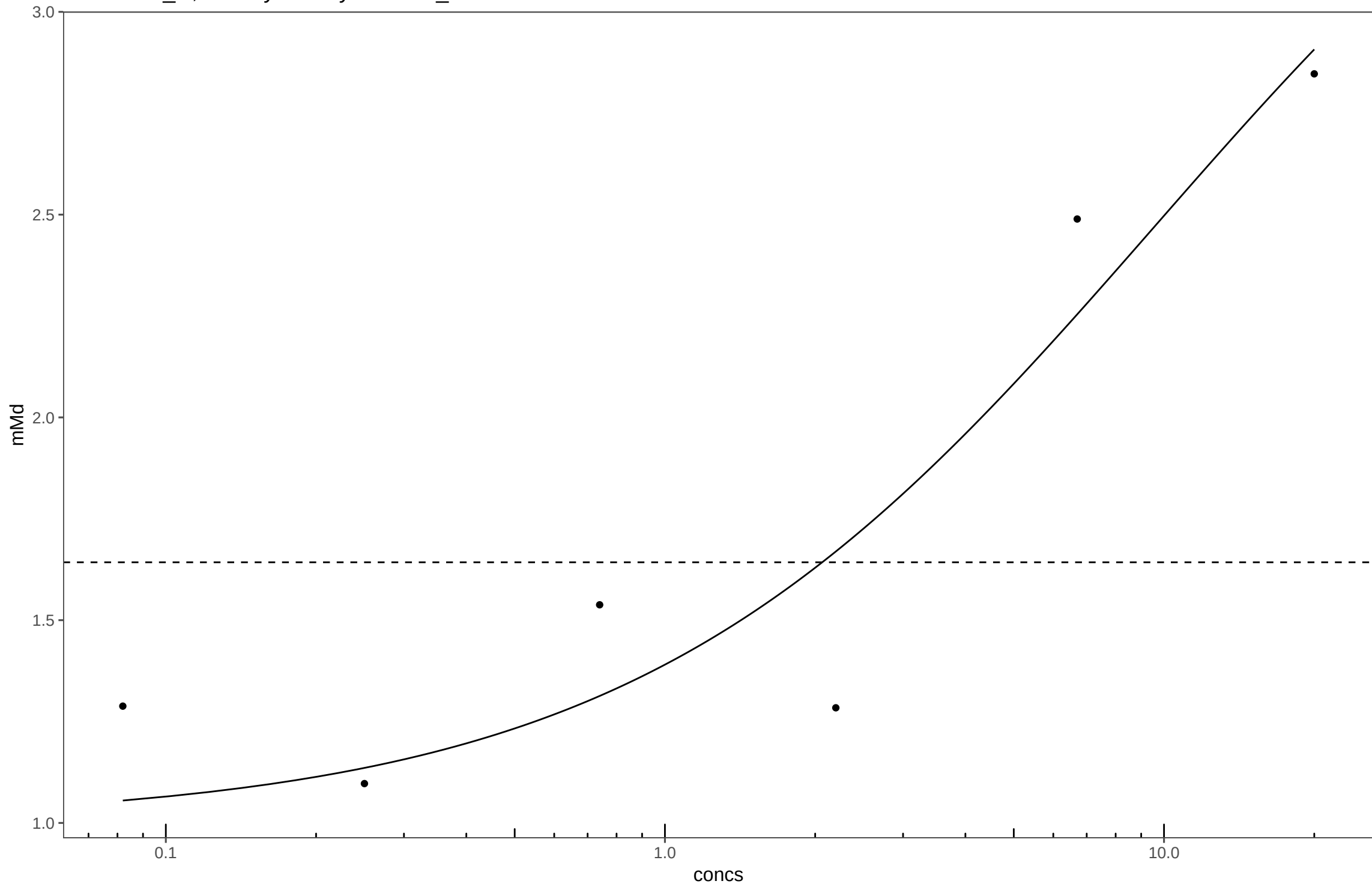
20140903_N,N'-Dicyclohexylthiourea_Plate19
