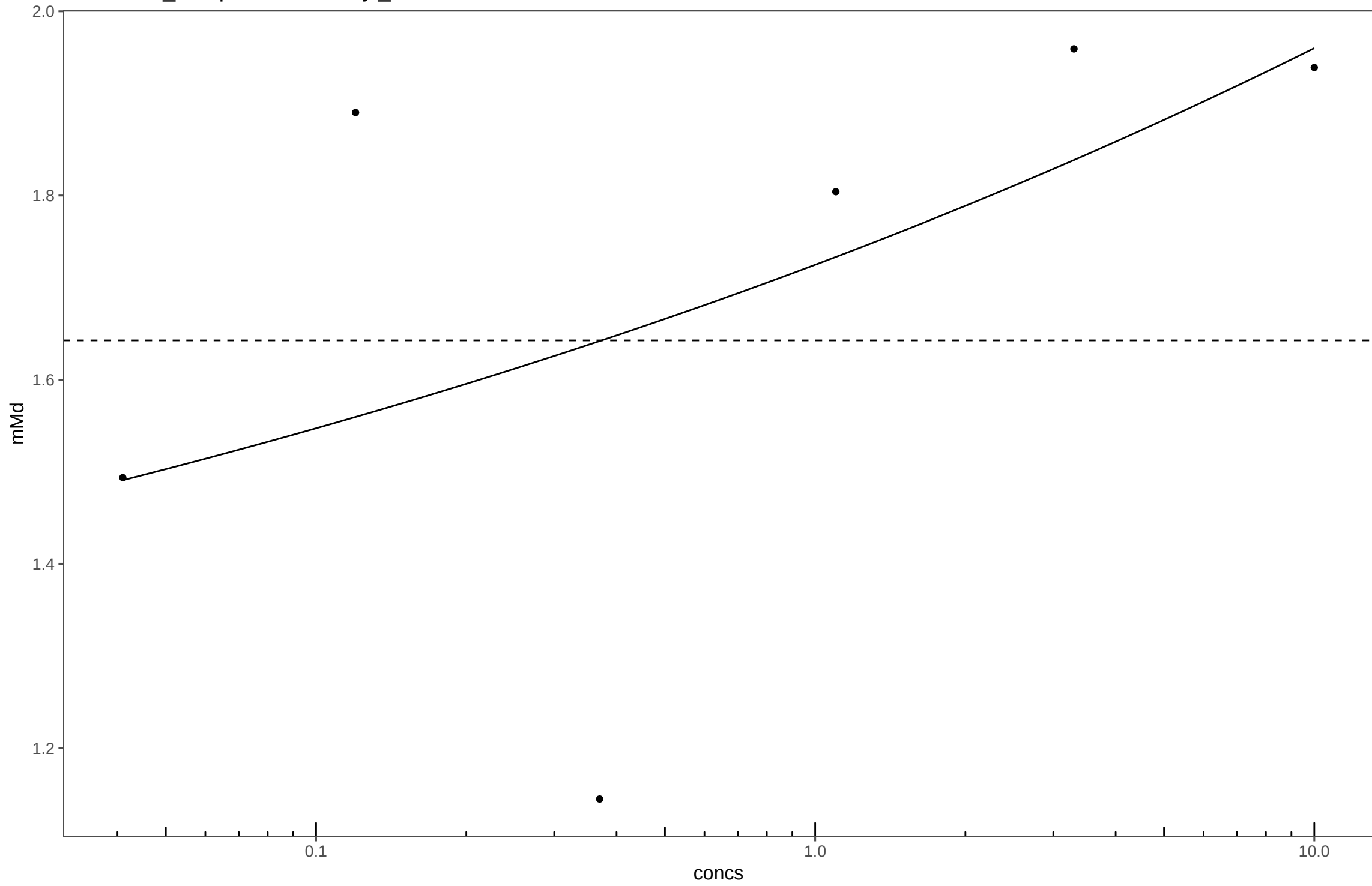
20150610_Thiophanate-methyl_Plate1
