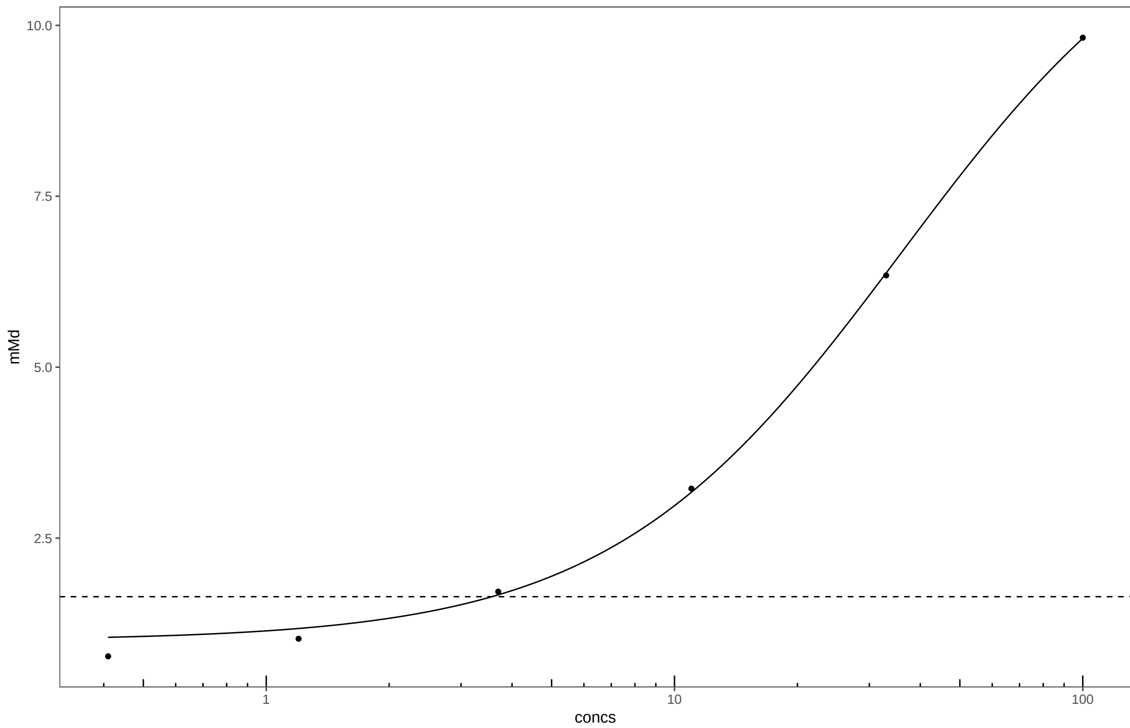
20140326_4-tert-Butylphenol_Plate11
