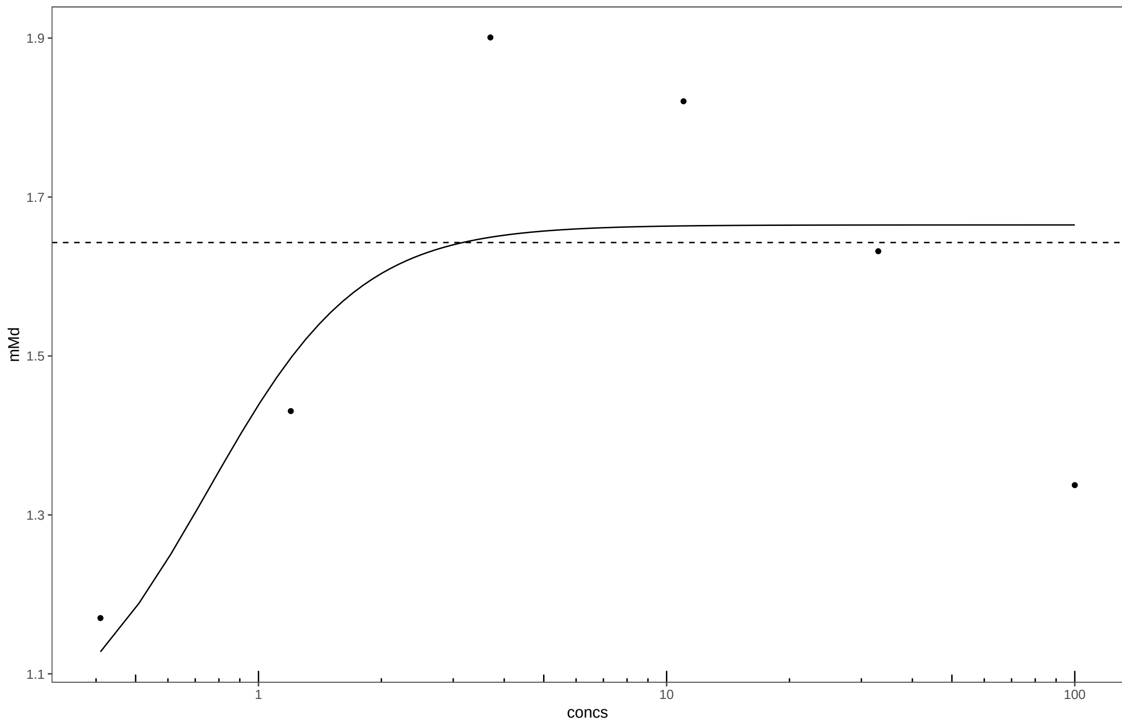
20150610_O,O-Dimethyl phosphoramidothioate_Plate29
