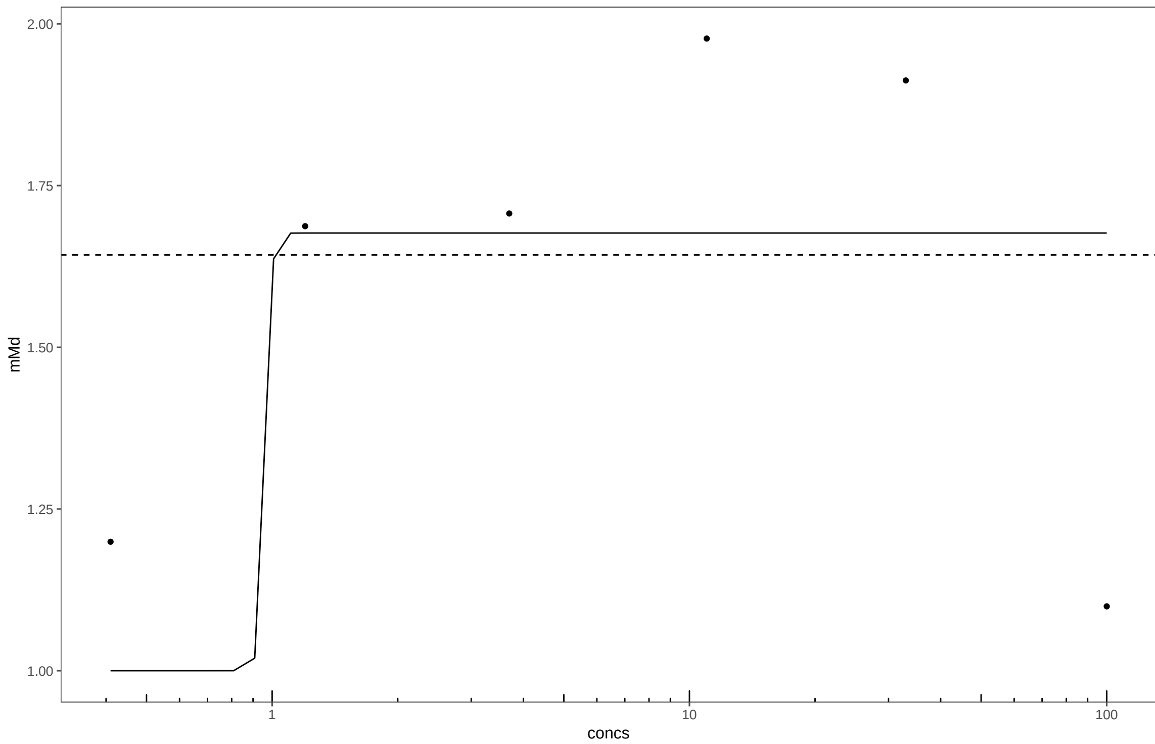
20150610_2,6-Dimethylpyridine_Plate29
