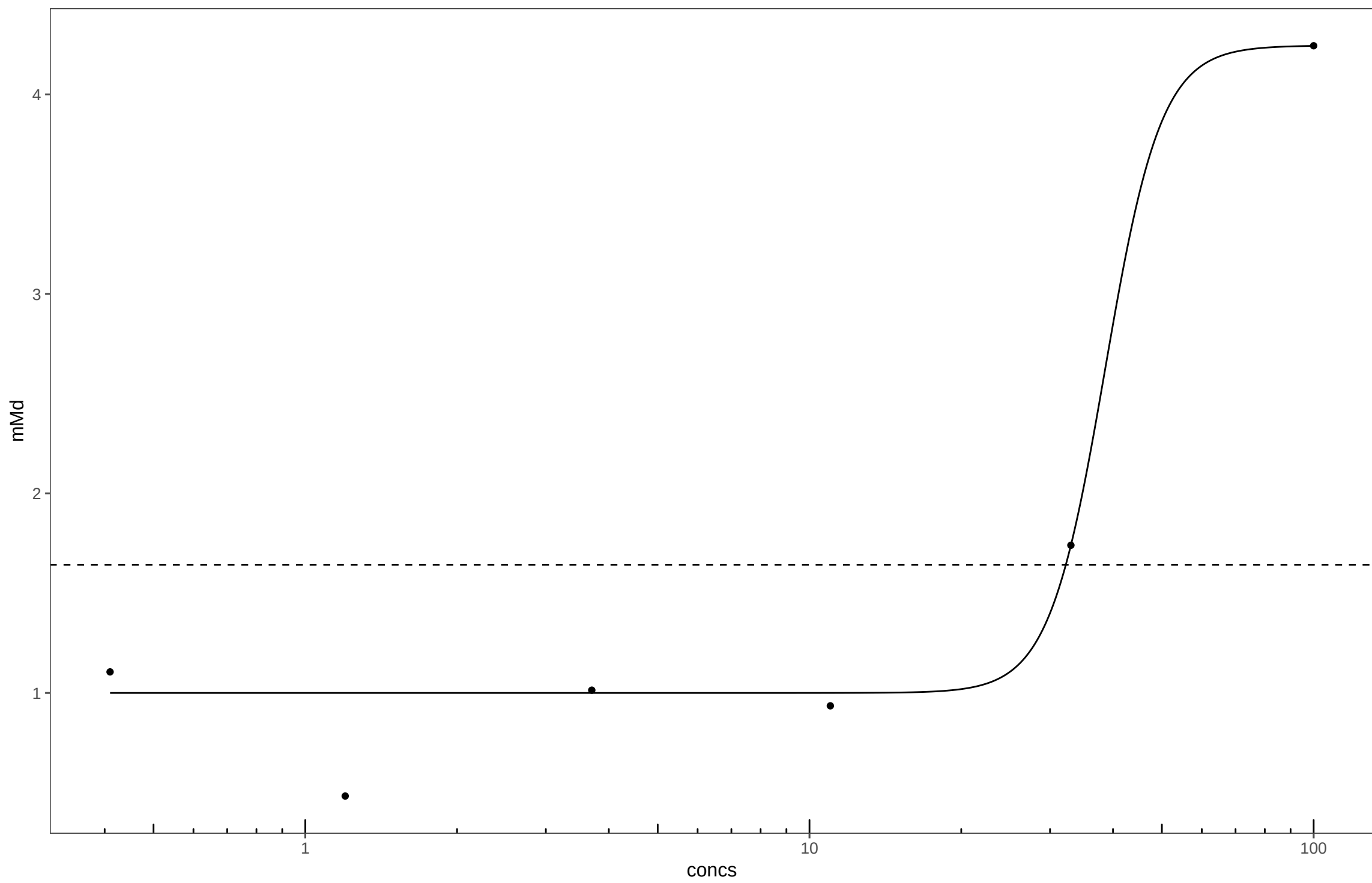
20140326_Oxytetracycline hydrochloride_Plate15
