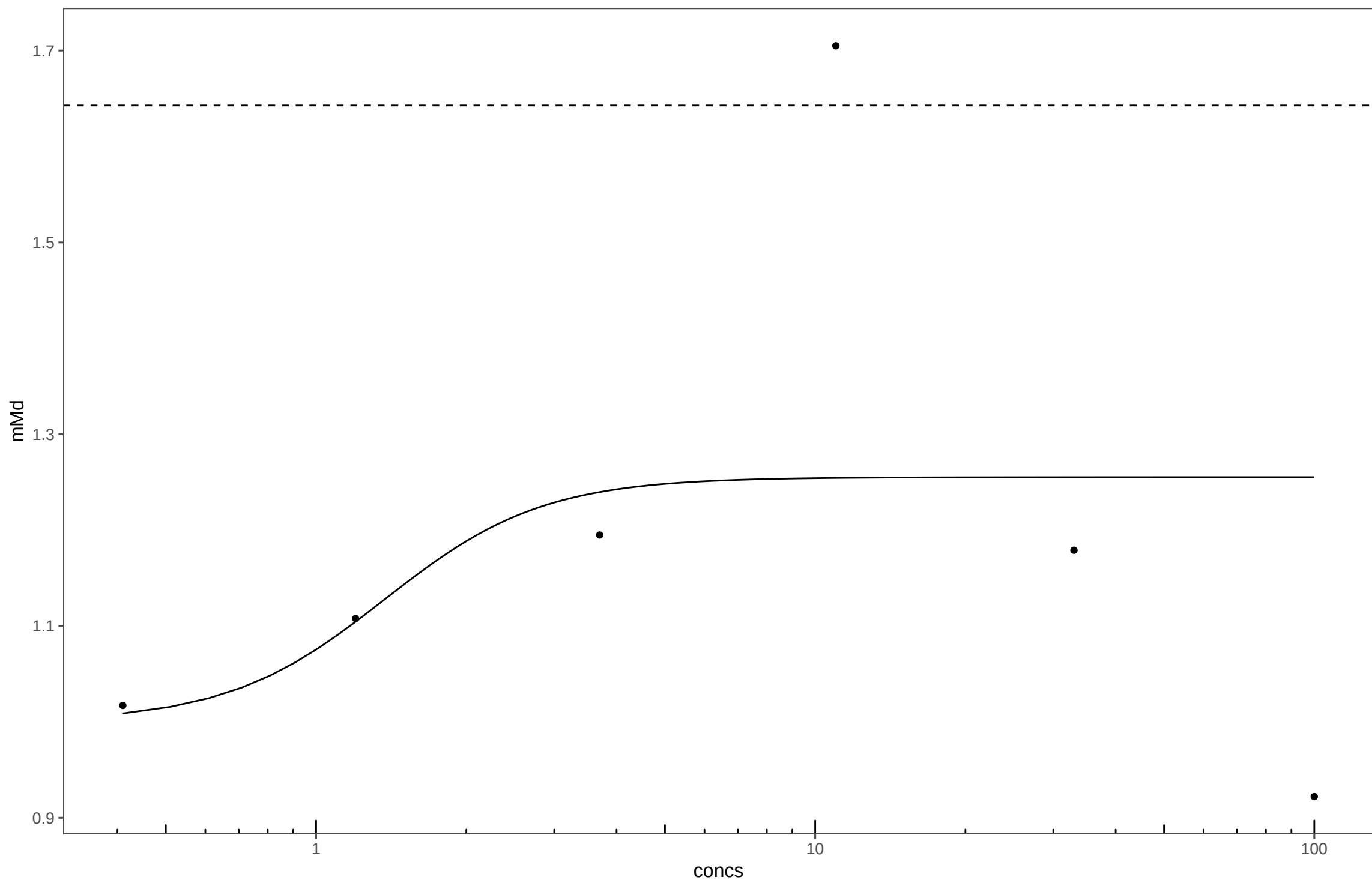
20150610_beta-(3,4-Epooxycyclohexyl)ethyltrimethoxysilane_Plate33
