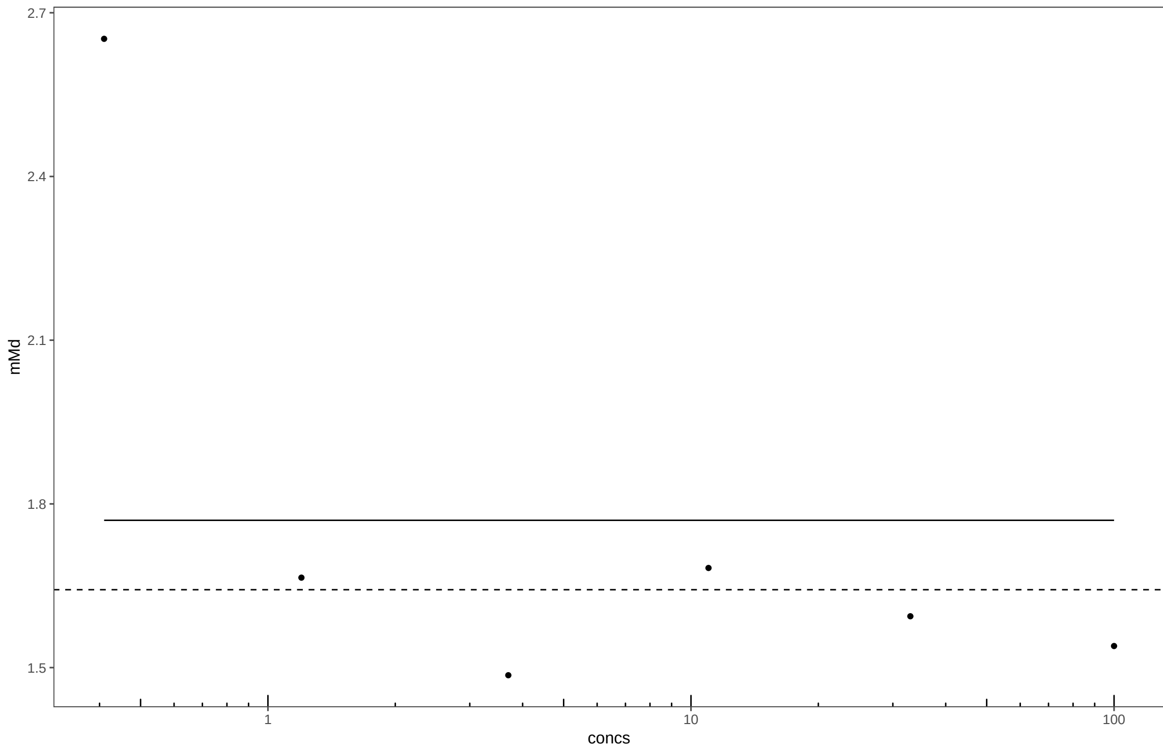
20140903_N,N,3-Trimethylaniline_Plate10
