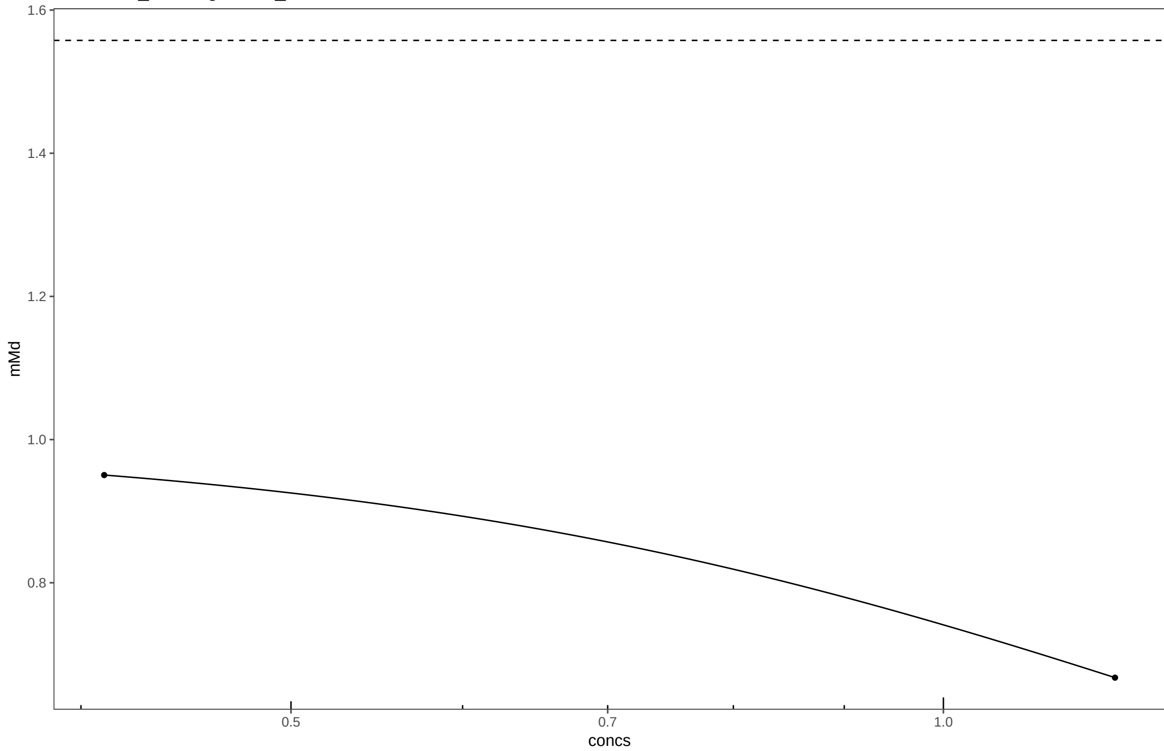
20170411_6-Thioguanine_Plate9
