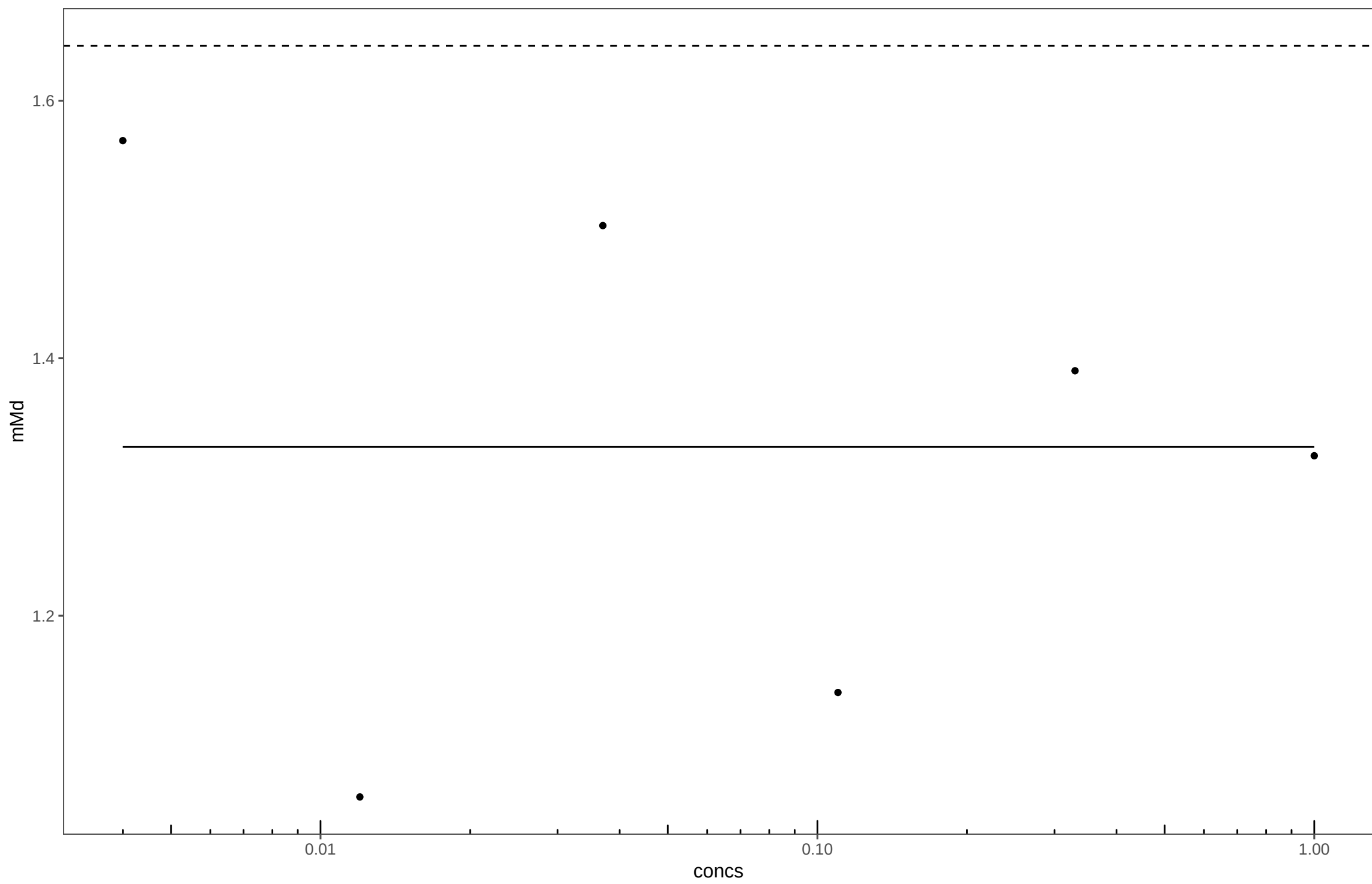
20150610_Triclosan_Plate1
