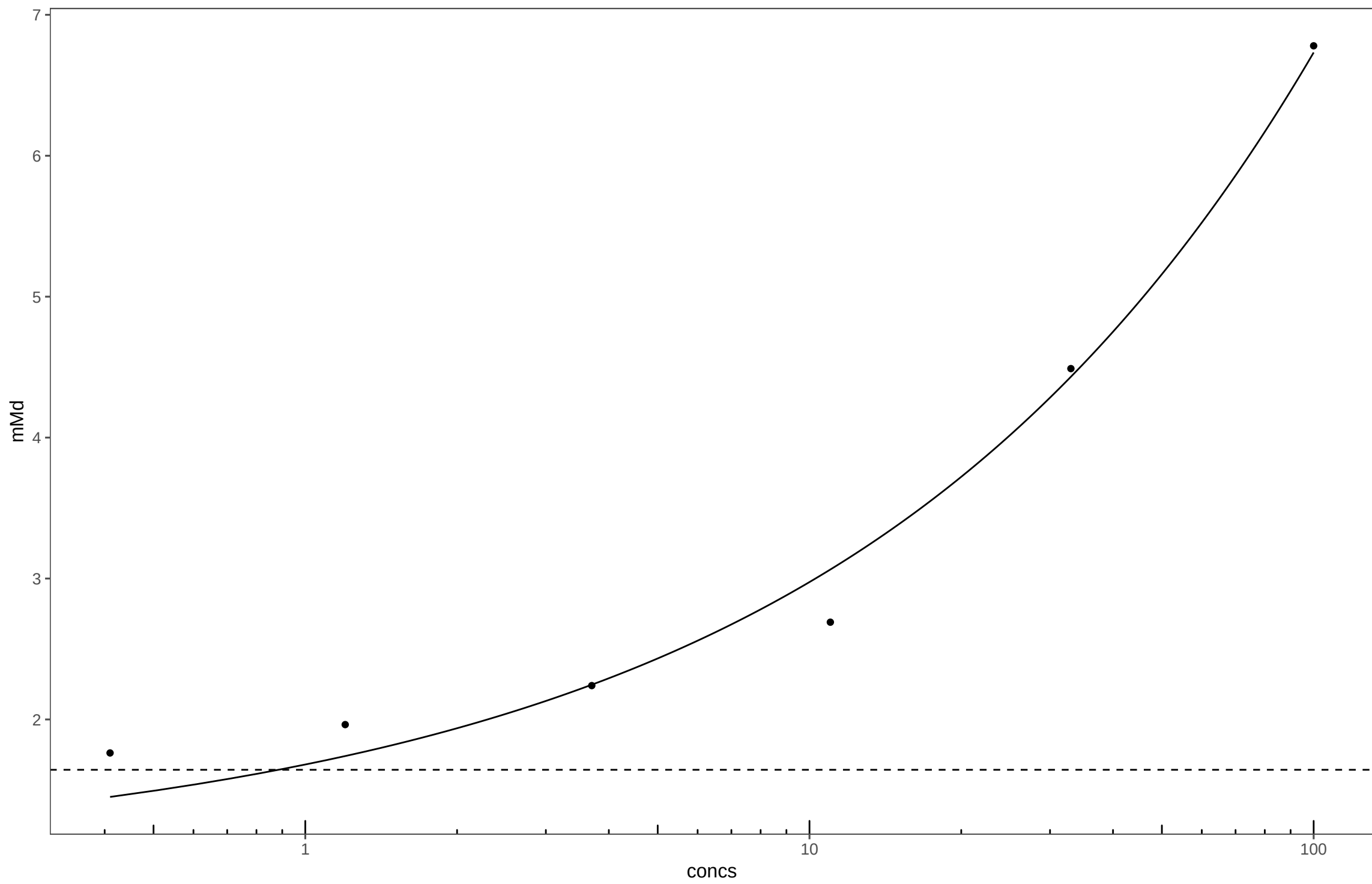
20150610_4-Chloro-2-methylphenol_Plate20
