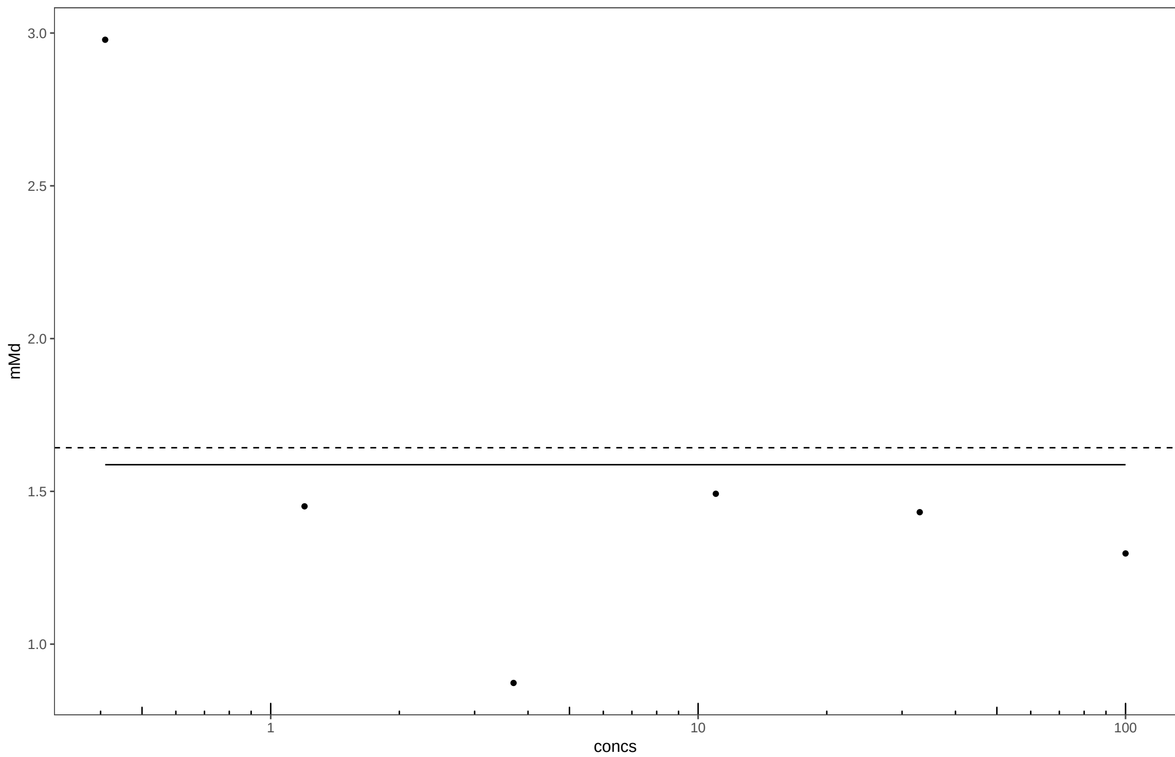
20140903_beta-(3,4-Epoxy cyclohexyl)ethyltrimethoxysilane_Plate13
