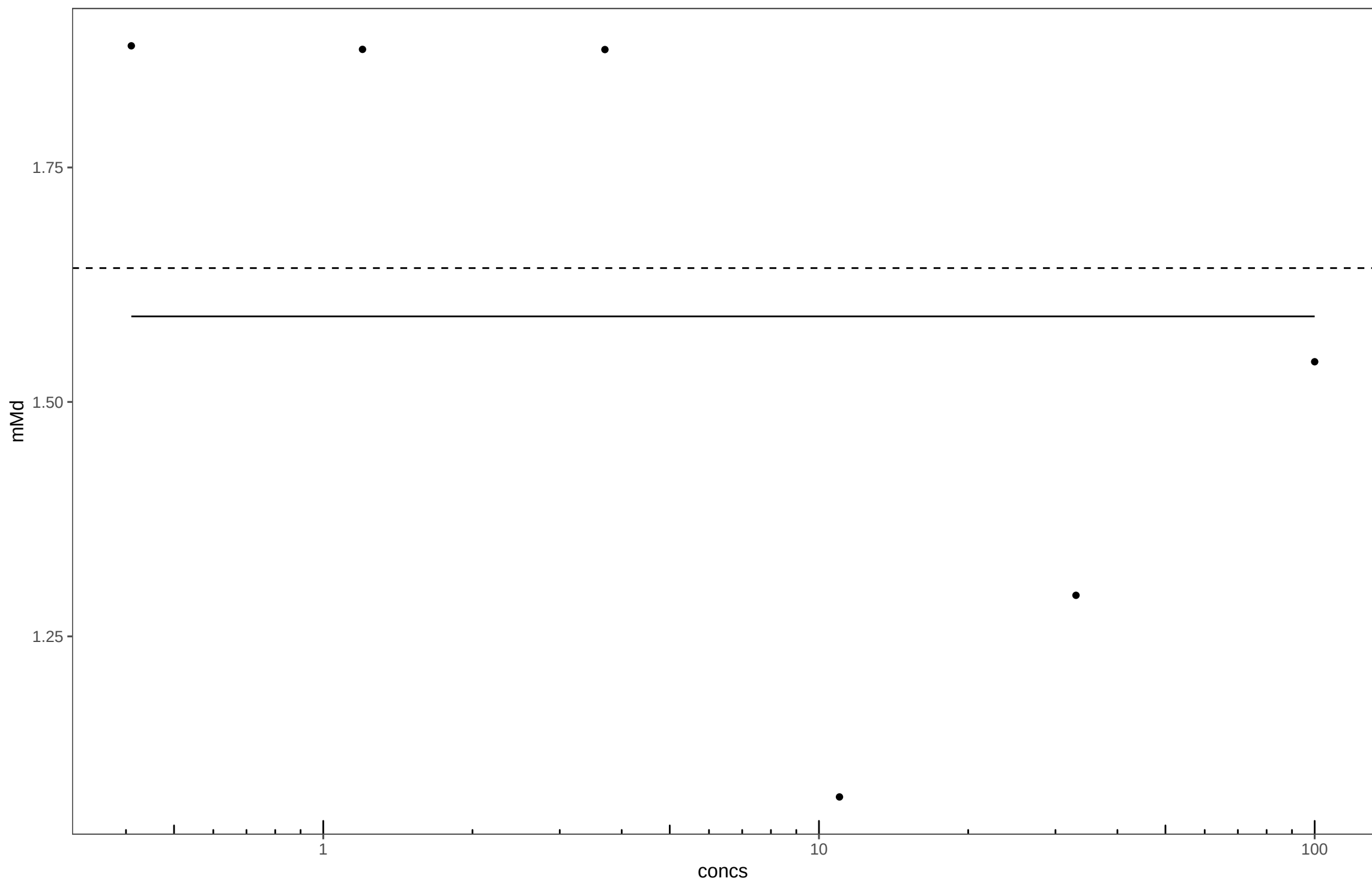
20140903_2,6-Dimethylpyridine_Plate10
