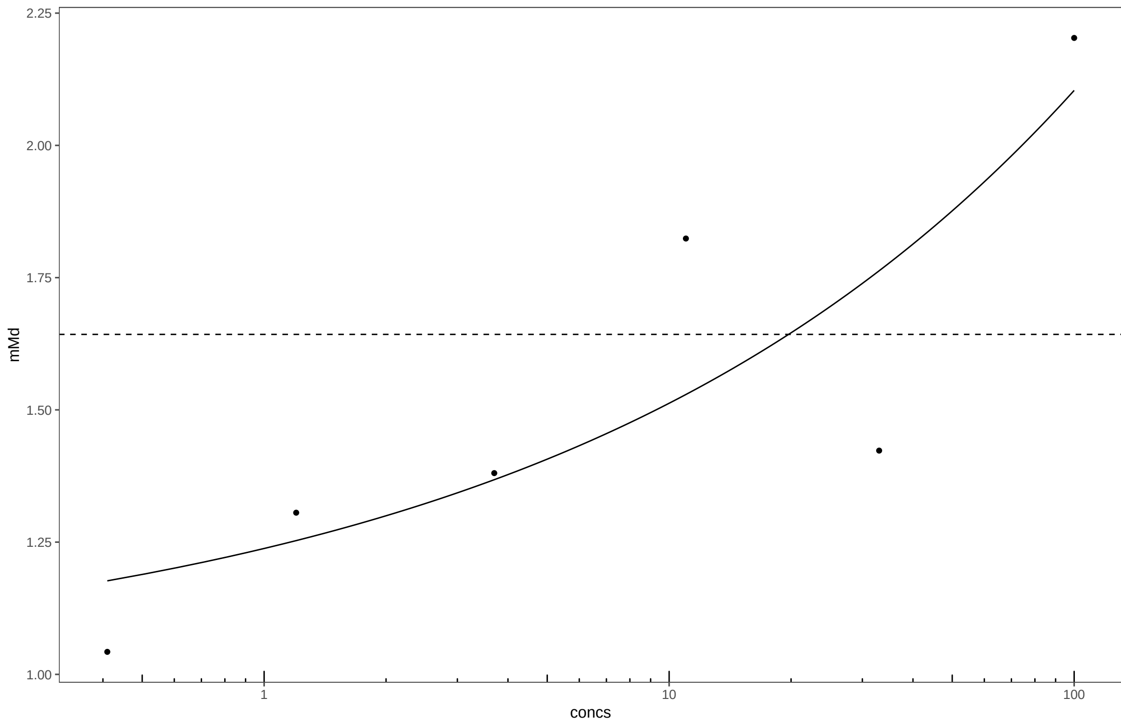
20150610_1,2,3-Trimethylbenzene_Plate31
