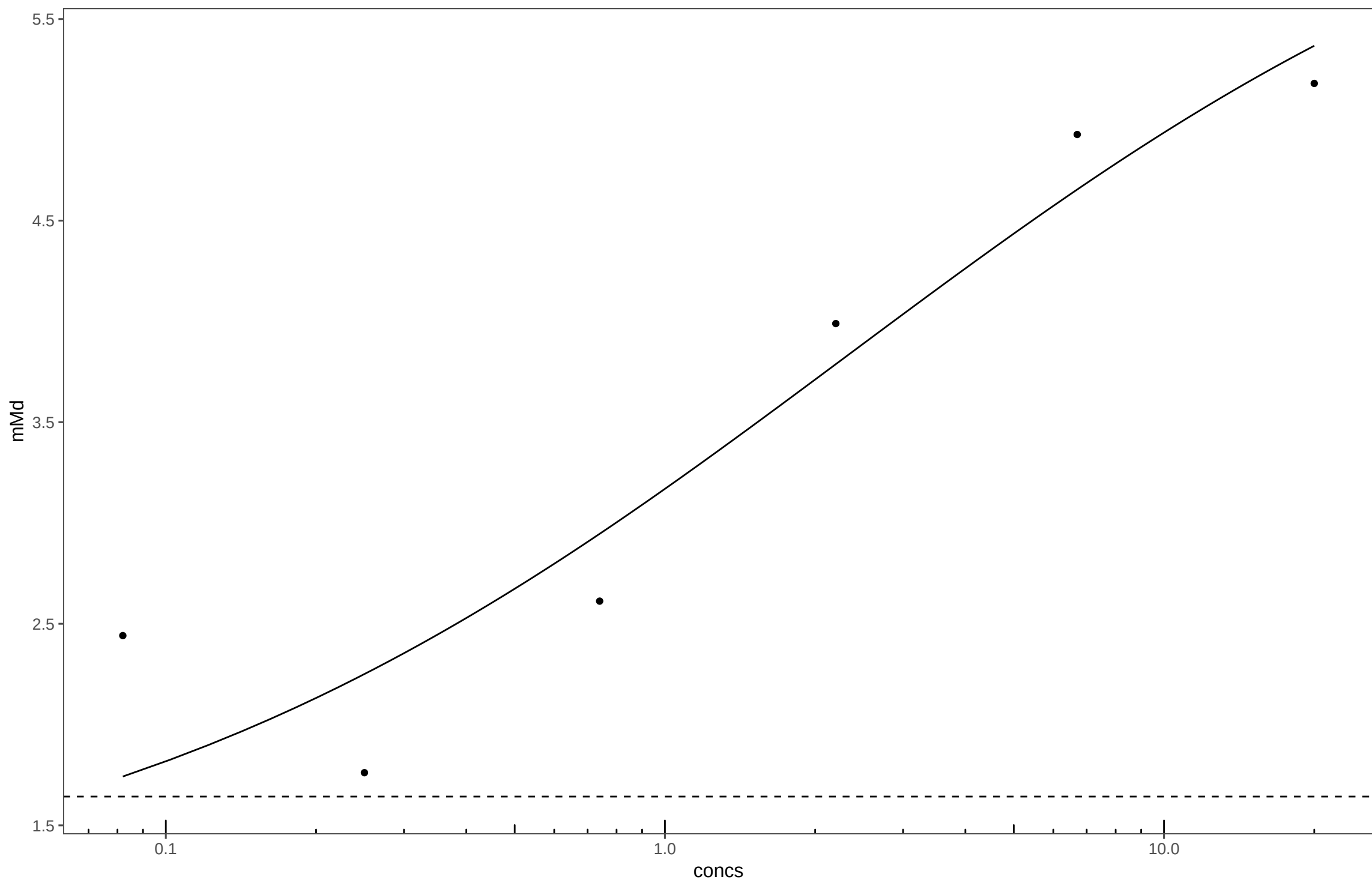
20130320_Spirodiclofen_Plate6
