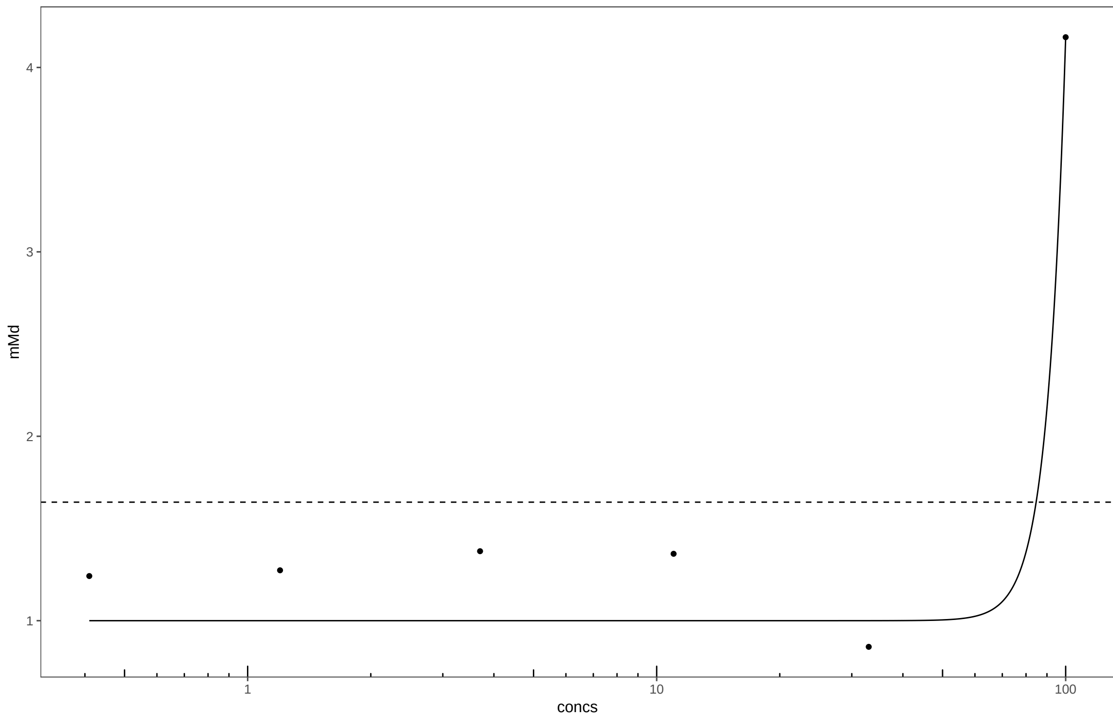
20170411_1,3,5,7-Tetramethyl-1,3,5,7-tetravinylcyclotetrasiloxane_Plate16
