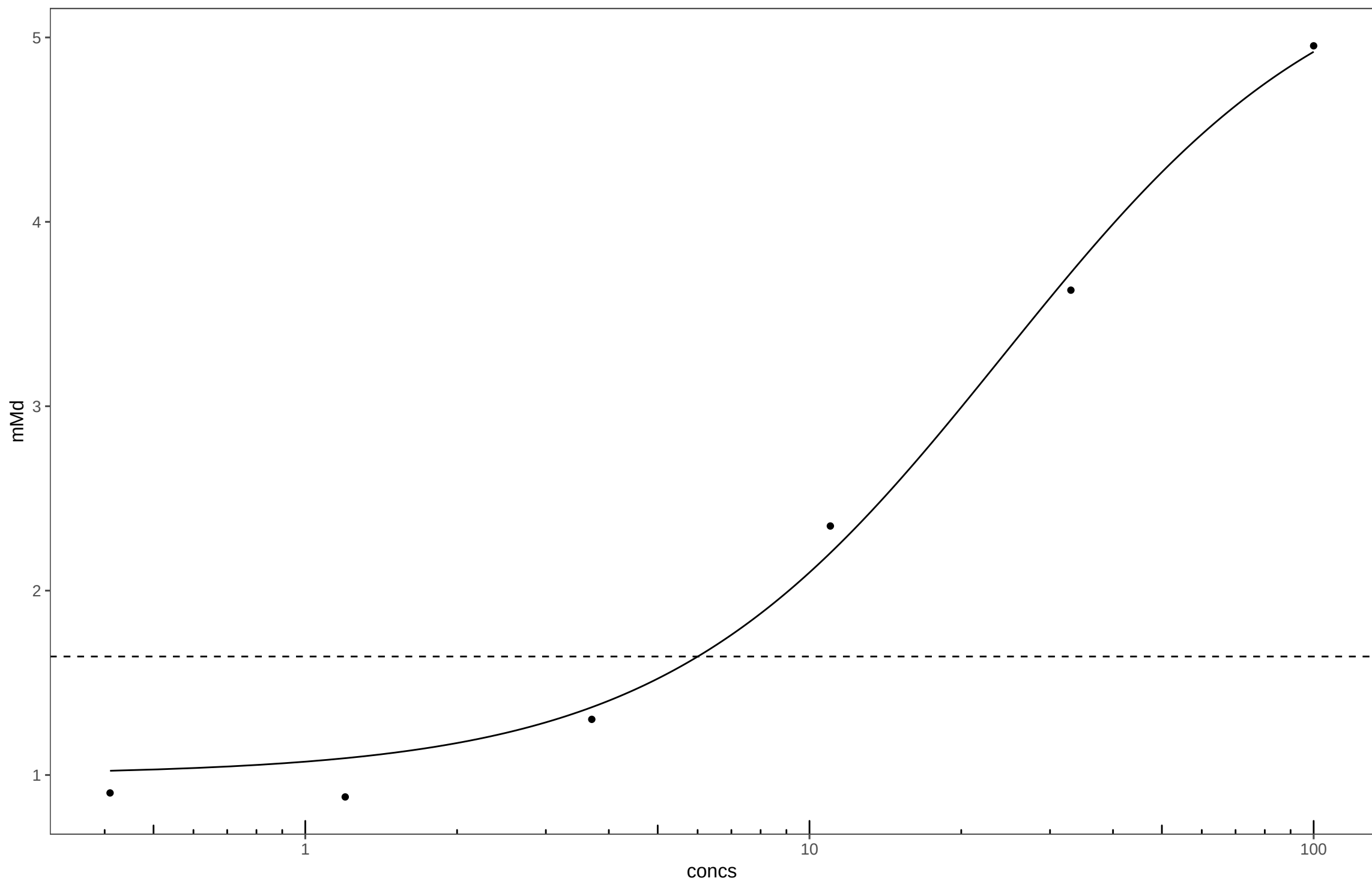
20170411_Rimsulfuron_Plate16
