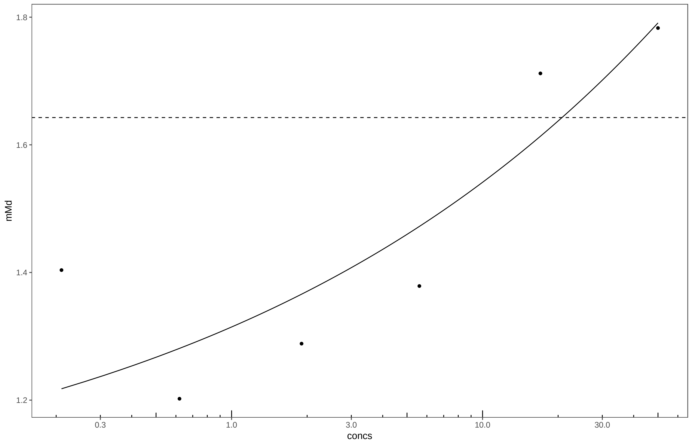
20140409_Tris(2-butoxyethyl) phosphate_Plate15
