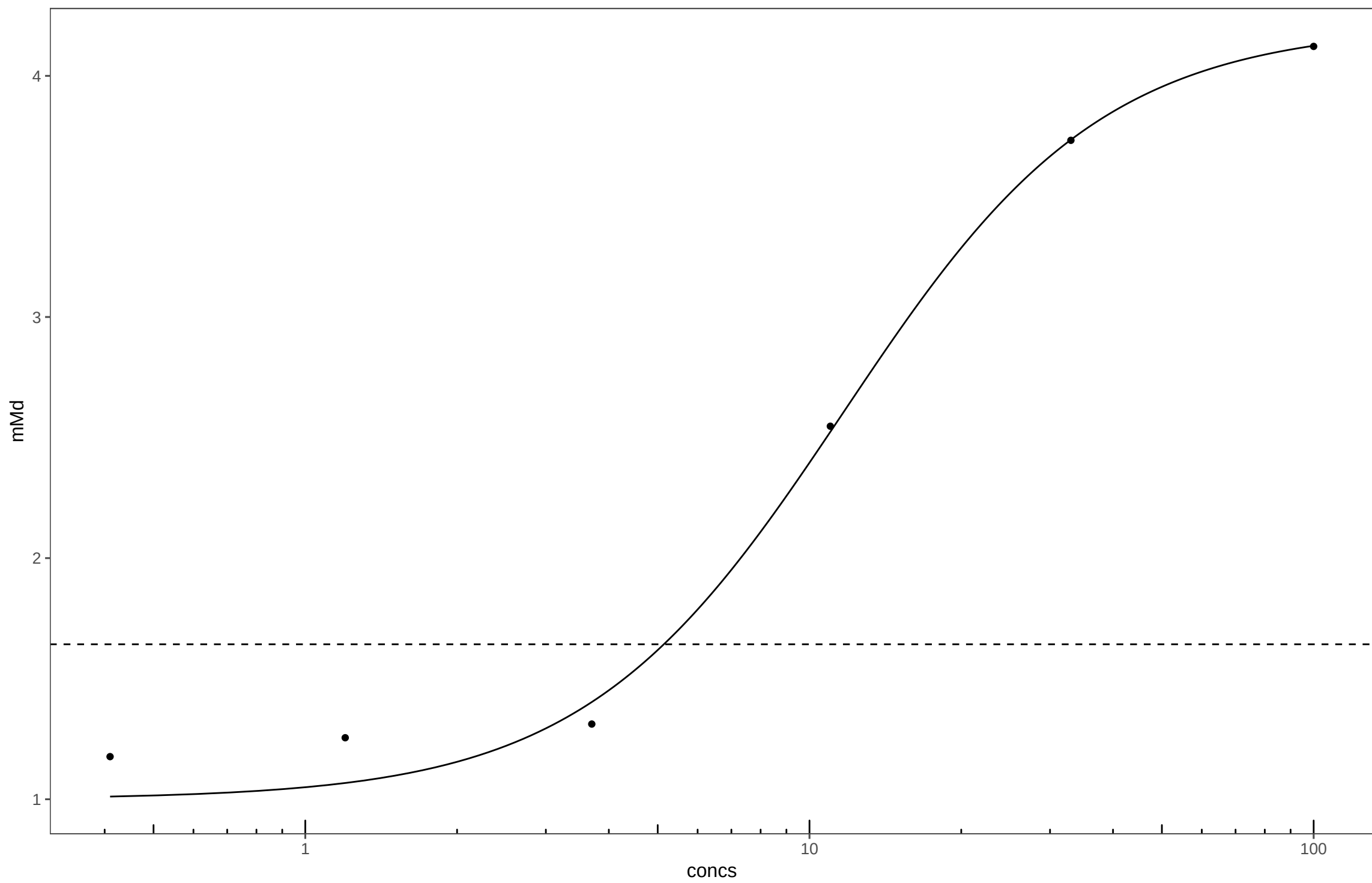
20150610_4-(N-Methyl-N-nitrosamino)-1-(3-pyridyl)-1-butanone_Plate34
