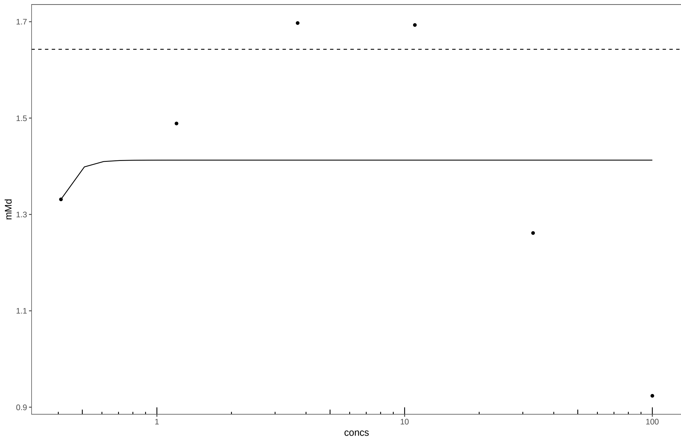
20150610_Methomyl_Plate3
