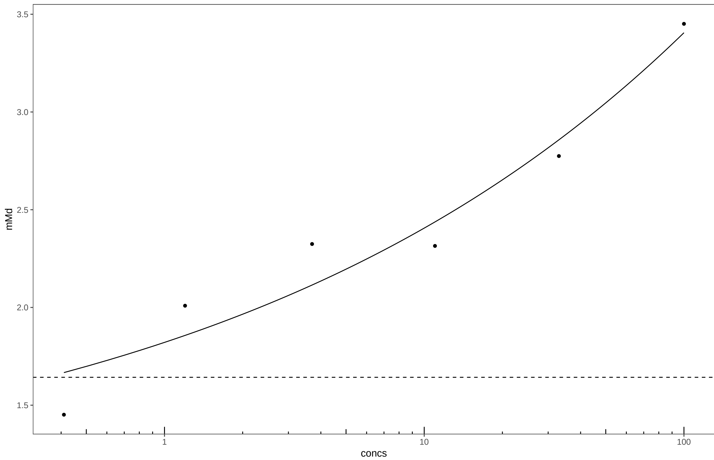
20150610_N-Octyl-2-pyrrolidone_Plate18
