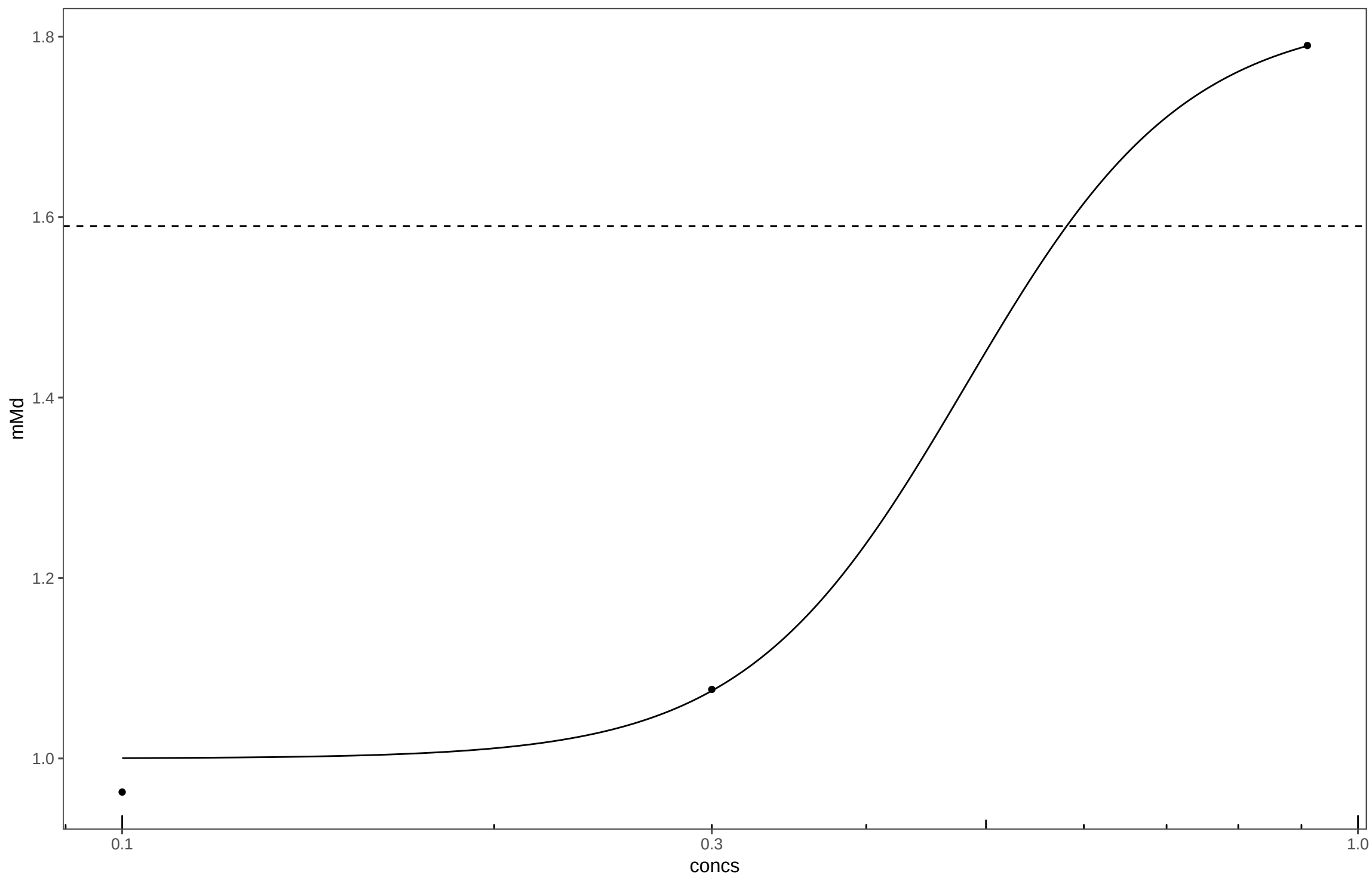
20170411_Tetrakis(hydroxymethyl)phosphonium sulfate_Plate22
