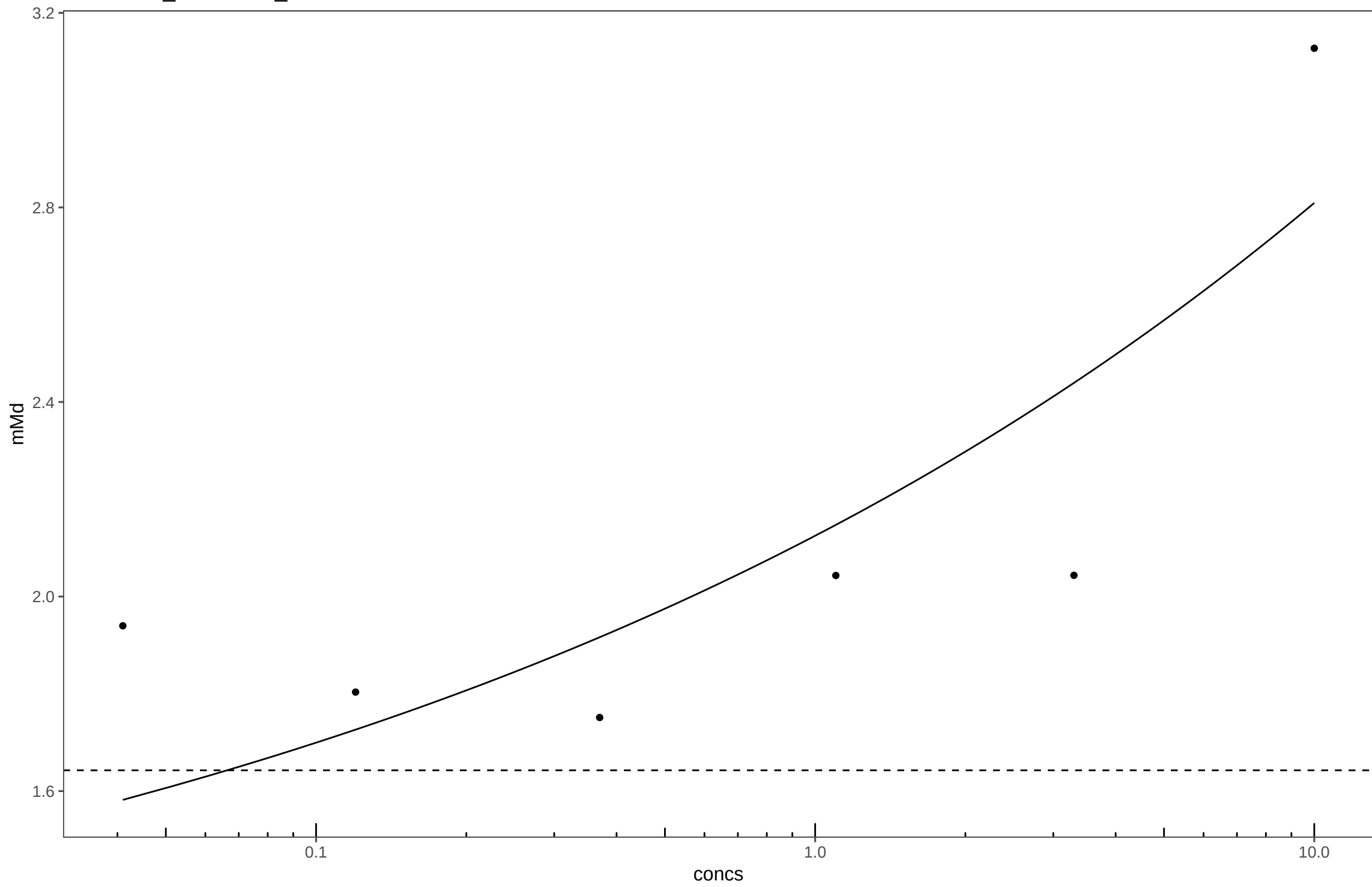
20140402_Disulfiram_Plate3
