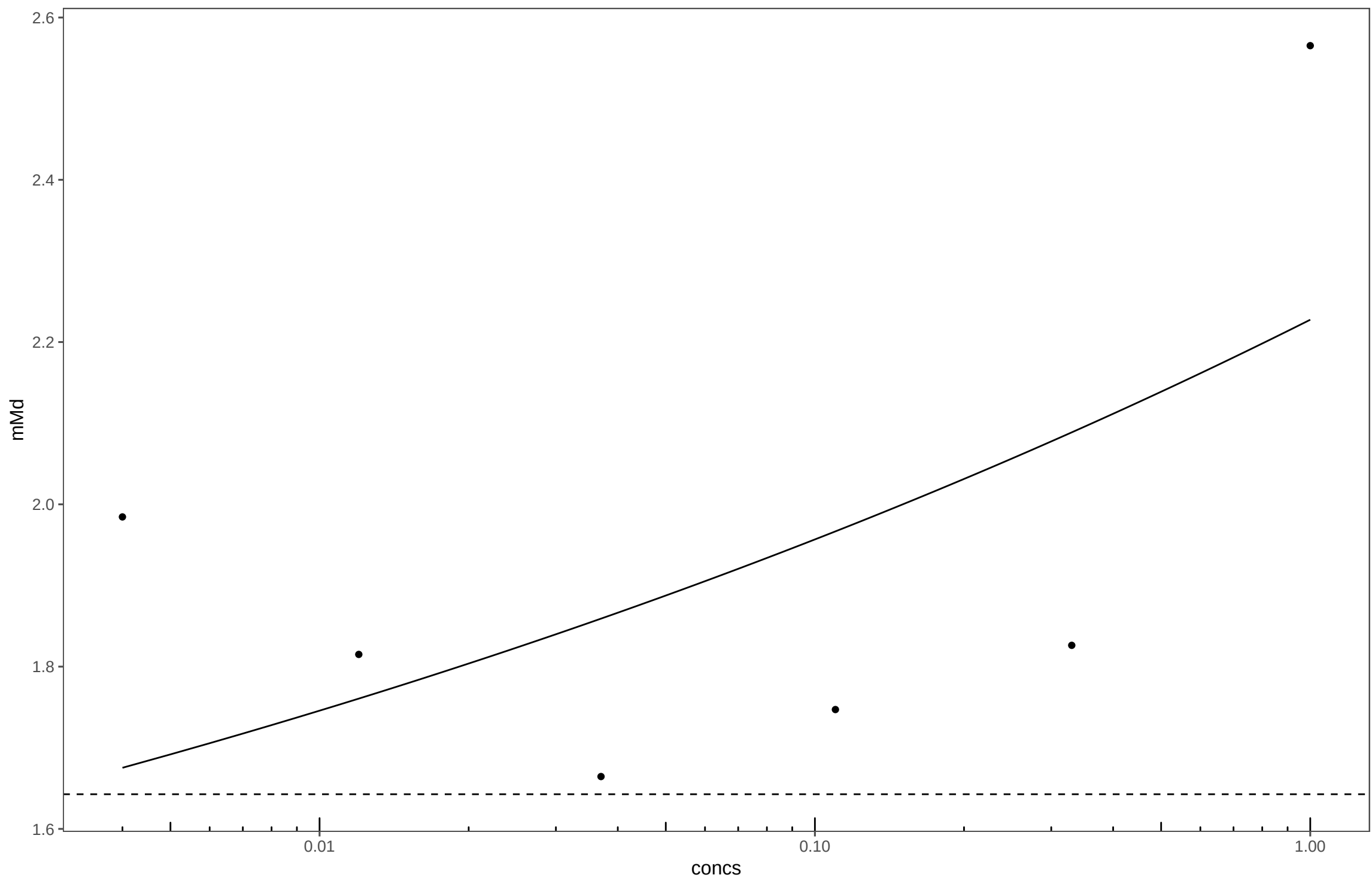
20140402_Triclosan_Plate3
