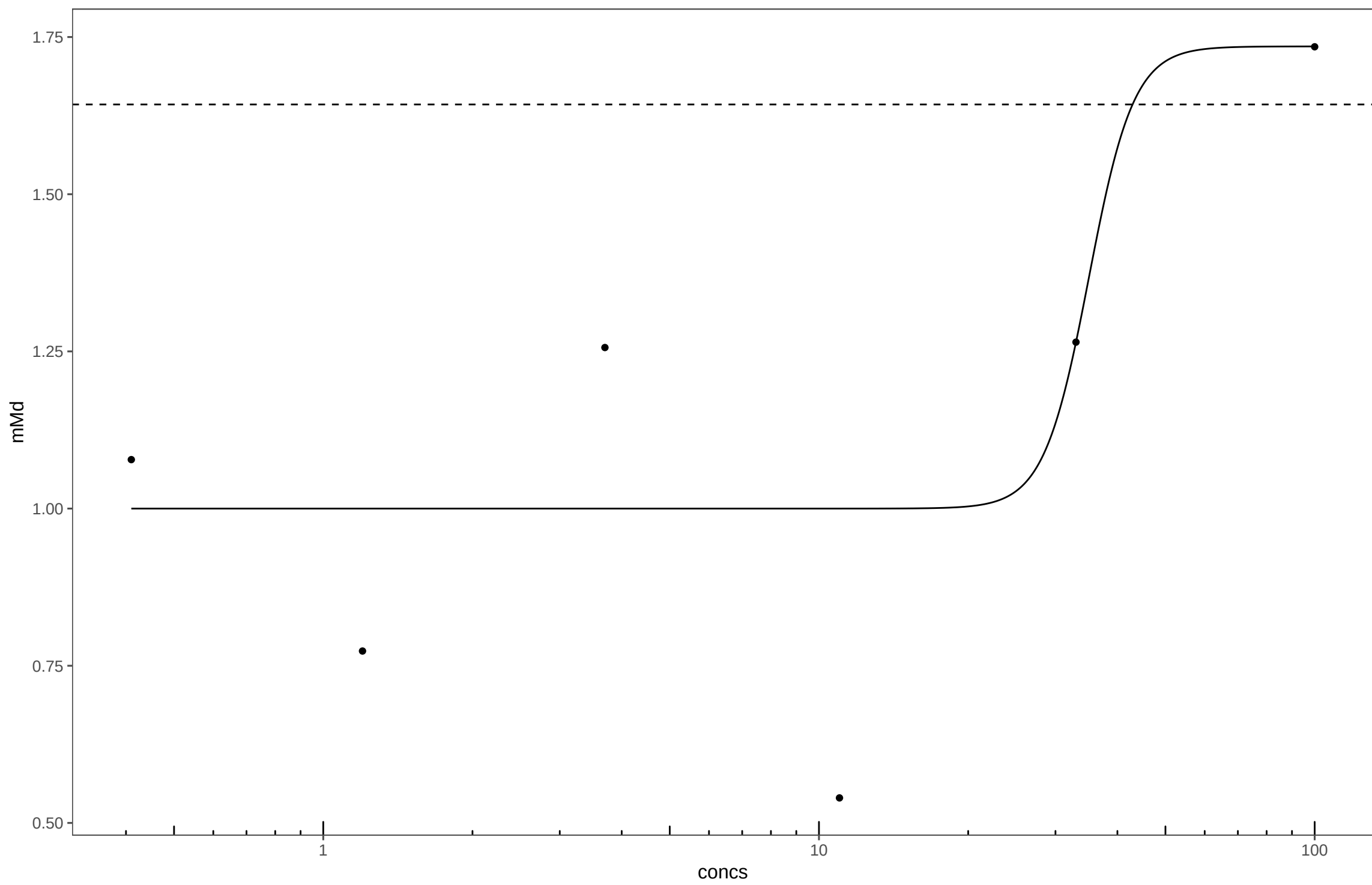
20140409_Isophorone diisocyanate_Plate1
