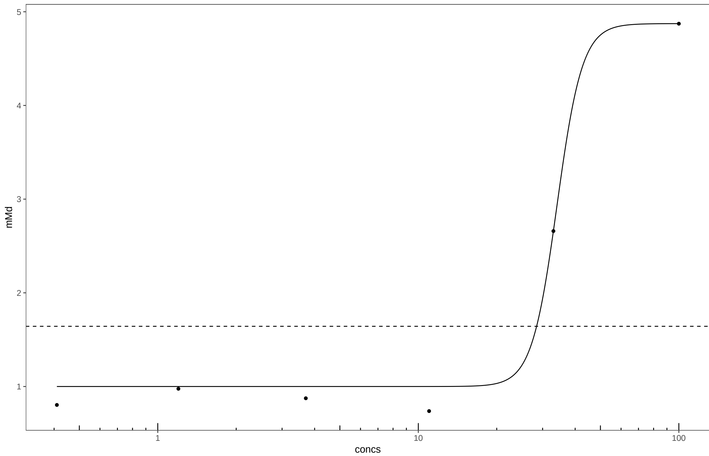
20130321_2-Phenylphenol_Plate2
