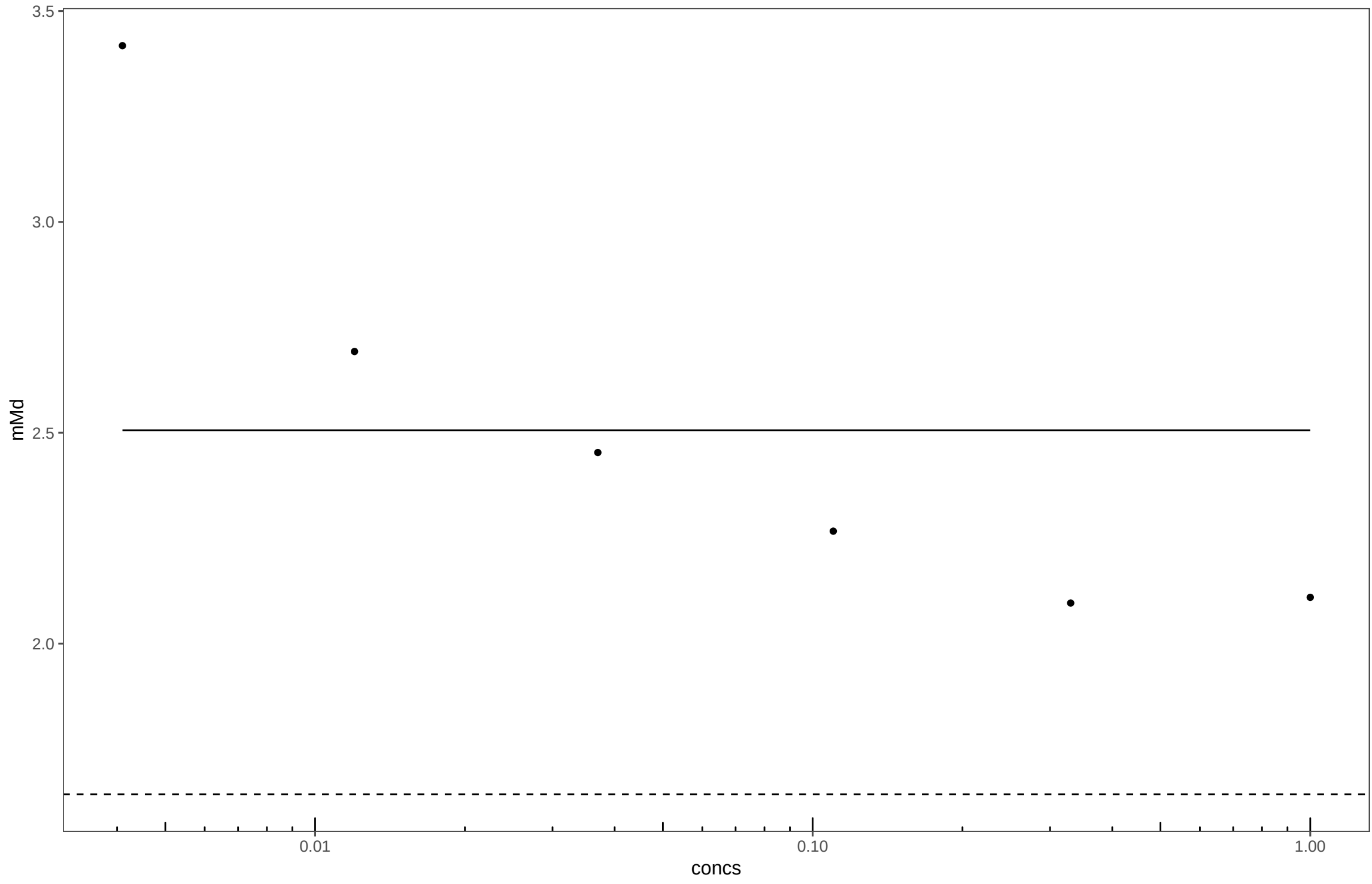
20140402_Dodecyltrimethylammonium chloride_Plate4
