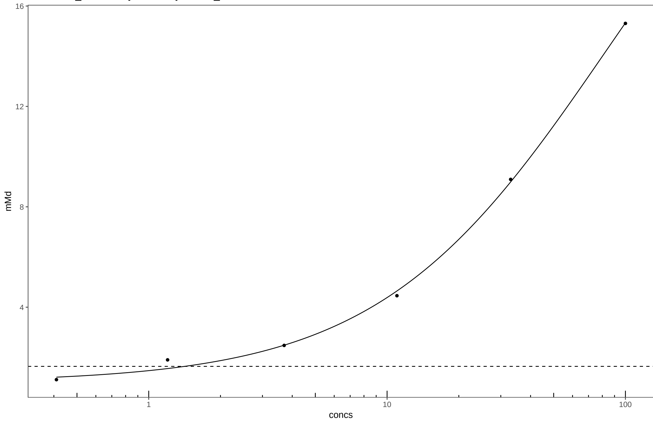
20140326_2-Methoxy-5-methylaniline_Plate16
