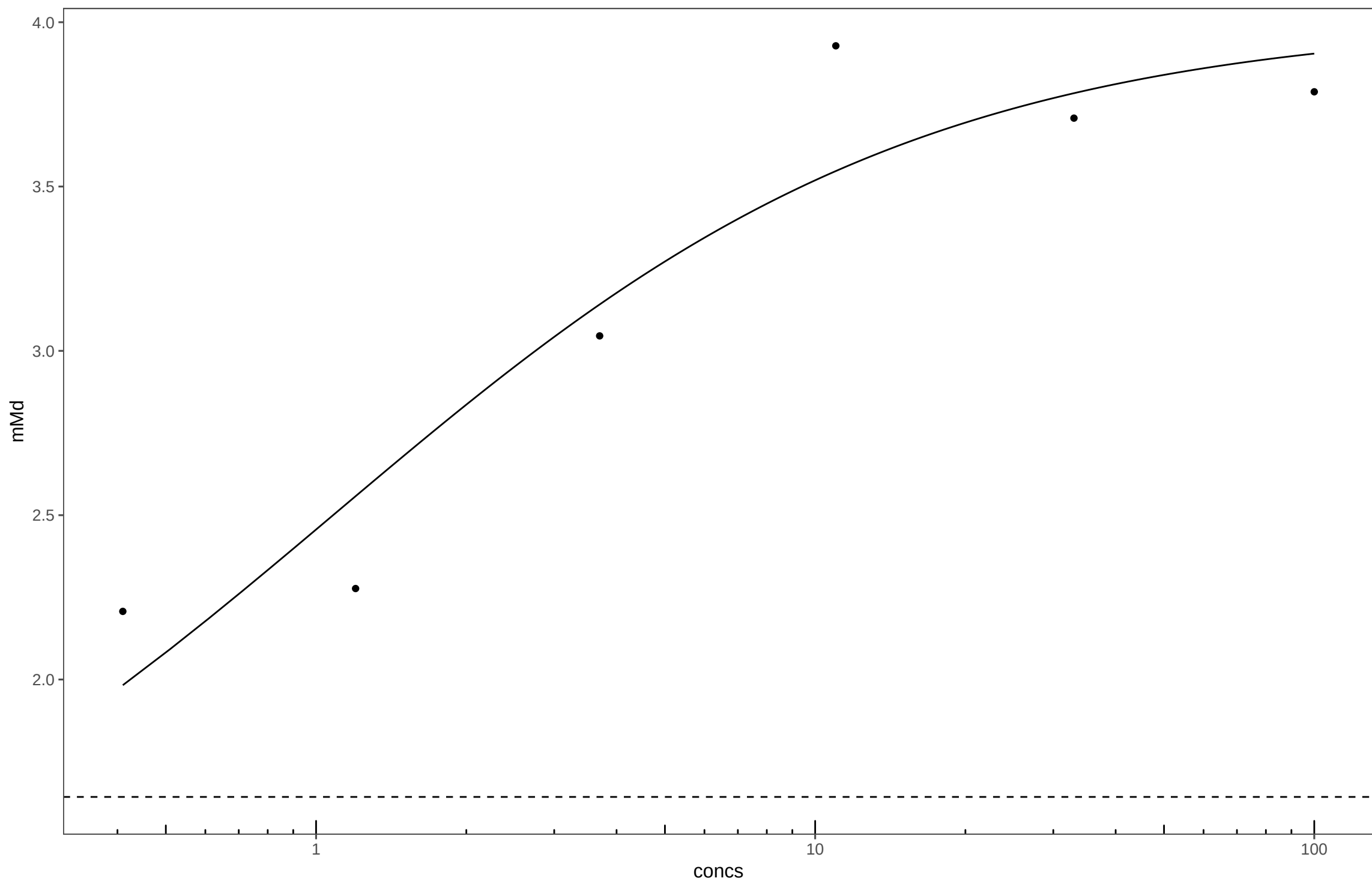
20130320_Prometryn_Plate13
