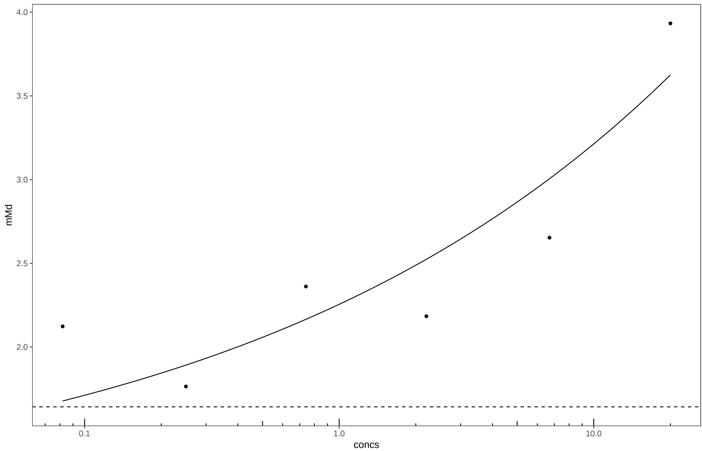
20150610_Prothioconazole_Plate23
