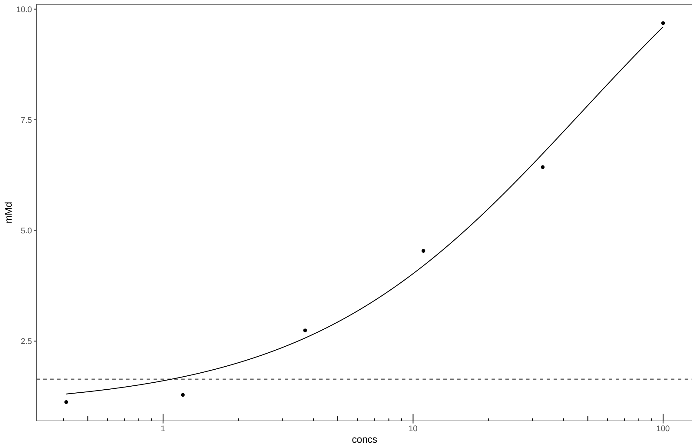
20170411_4-Pentylaniline_Plate17
