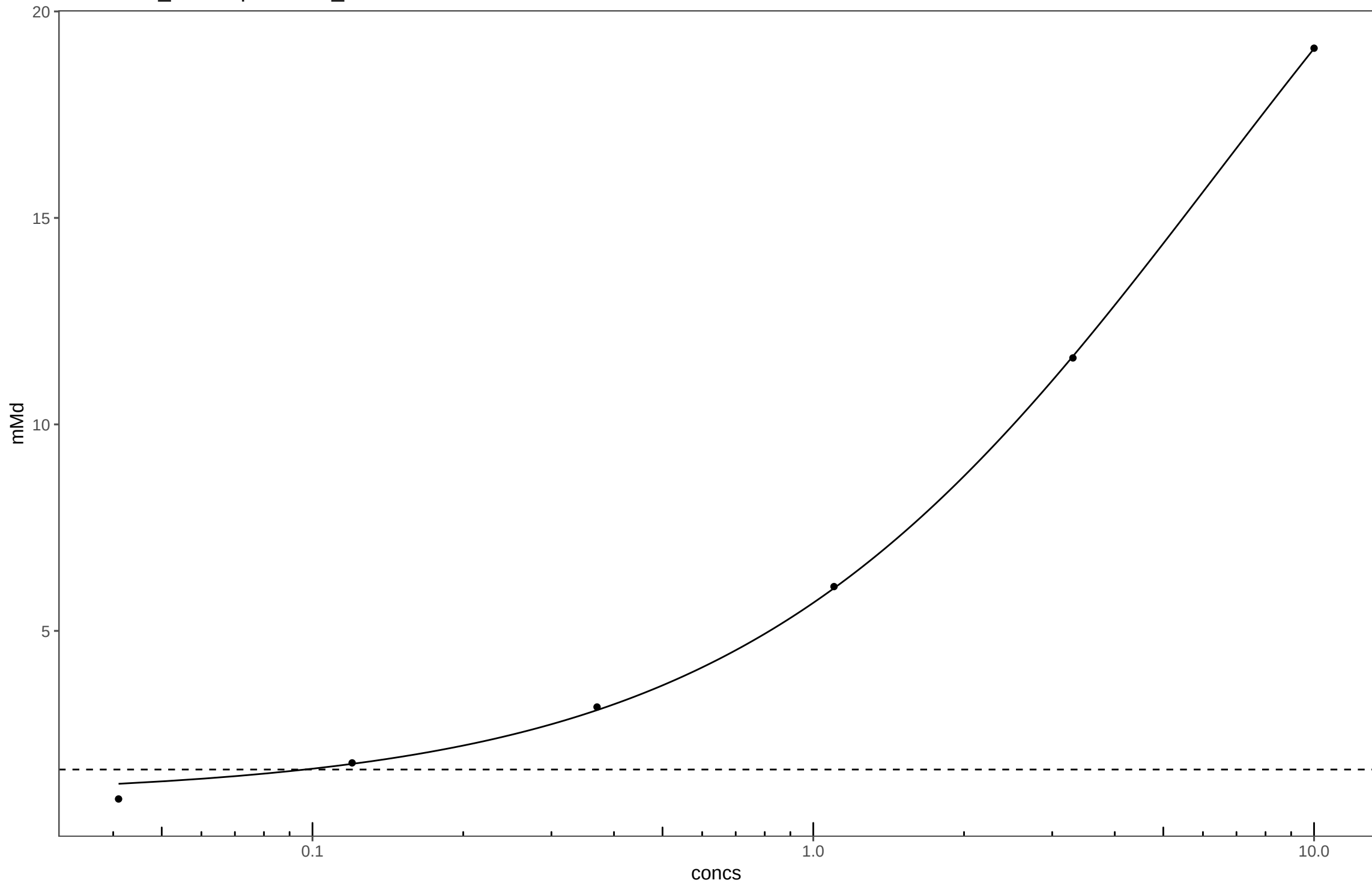
20140402_Phenolphthalein_Plate2
