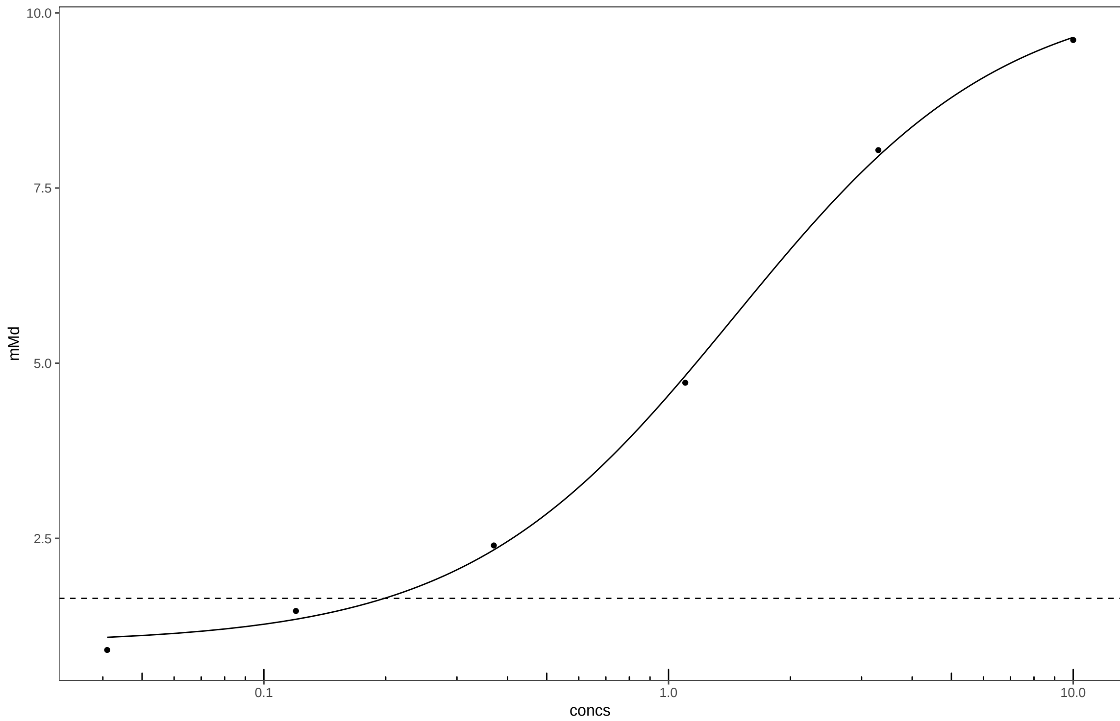
20140326_Spironolactone_Plate10
