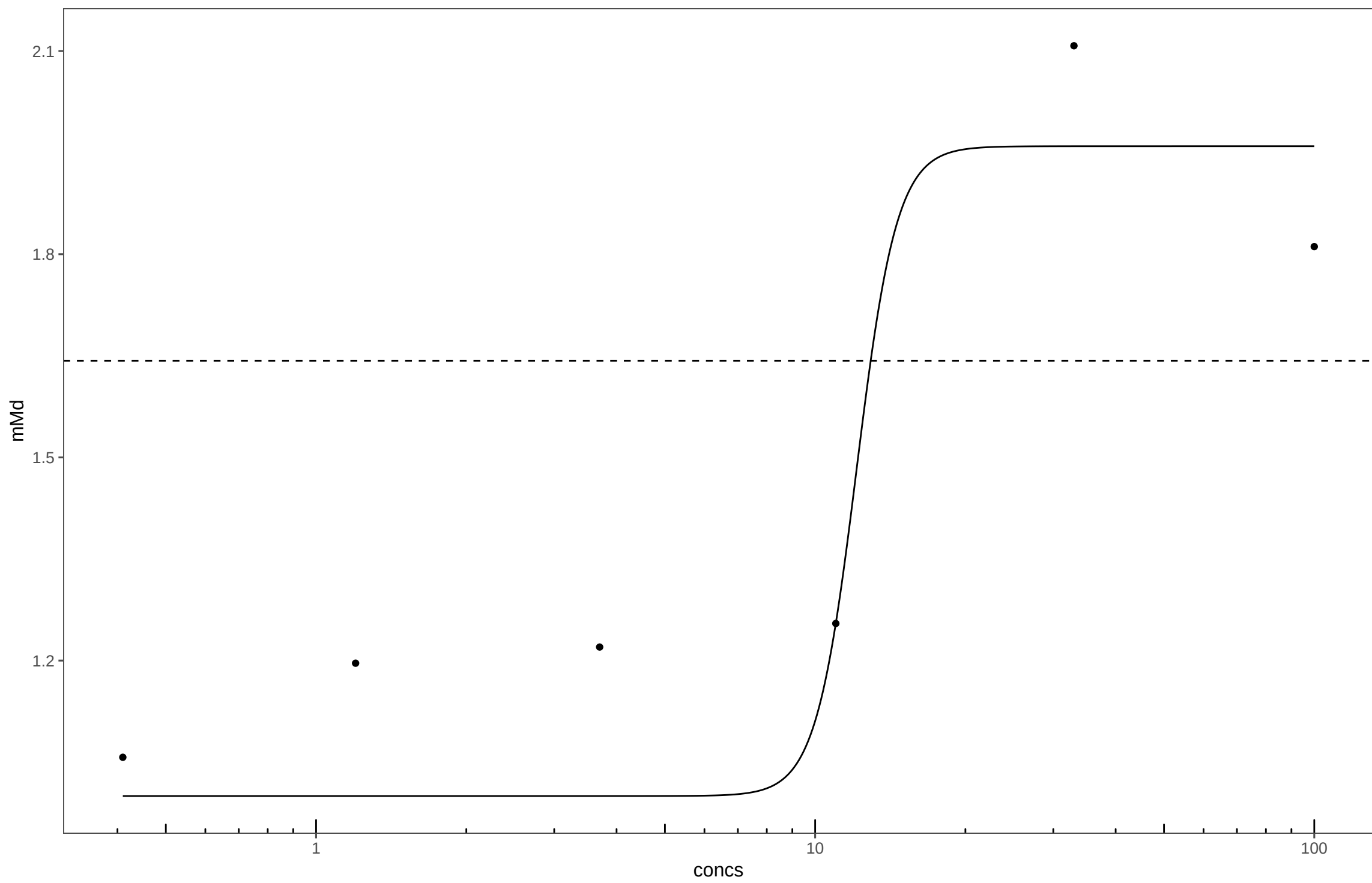
20170411_Methyl dihydrojasmonate_Plate14
