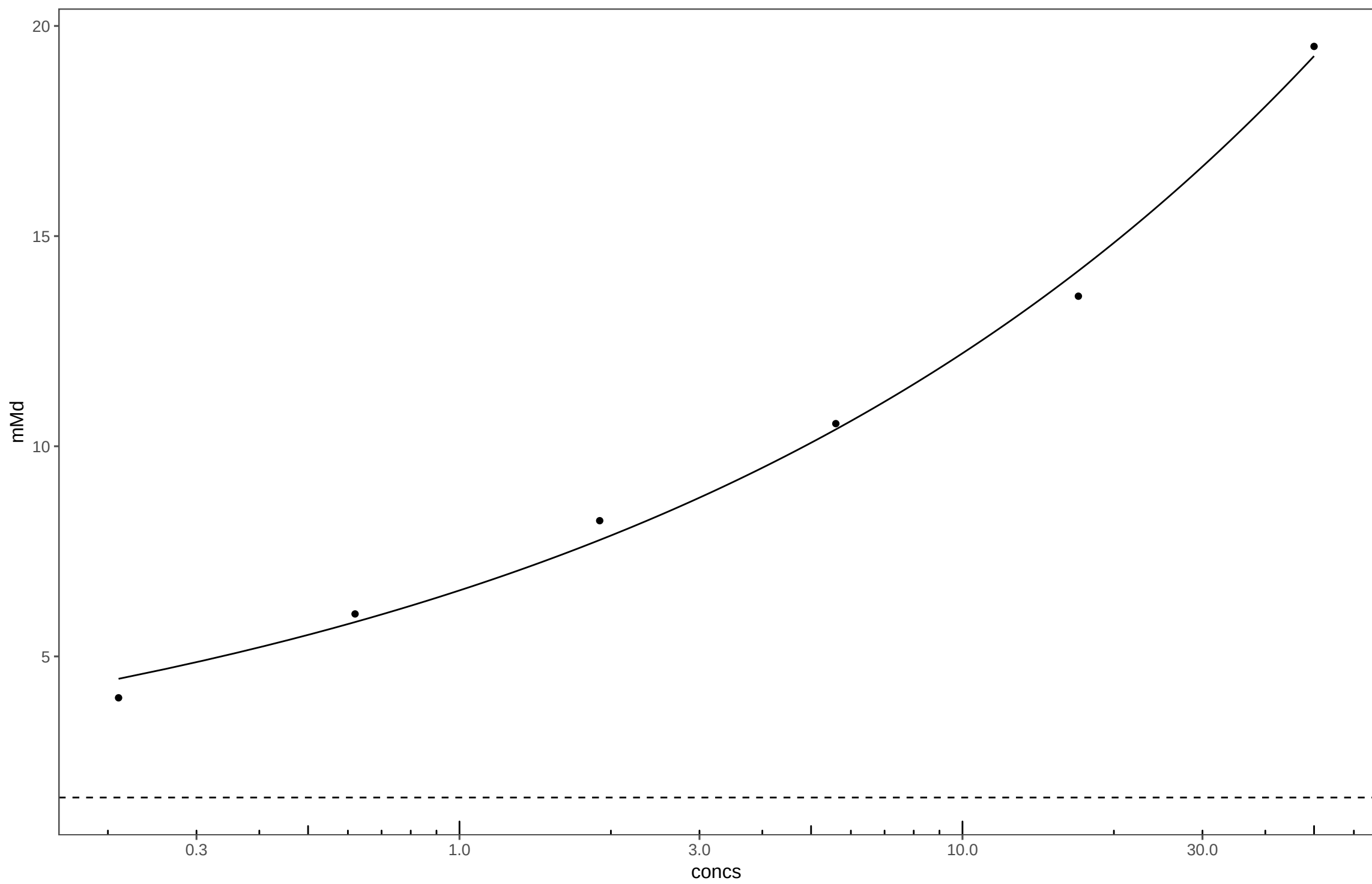
20140409_Phenolphthalin_Plate9
