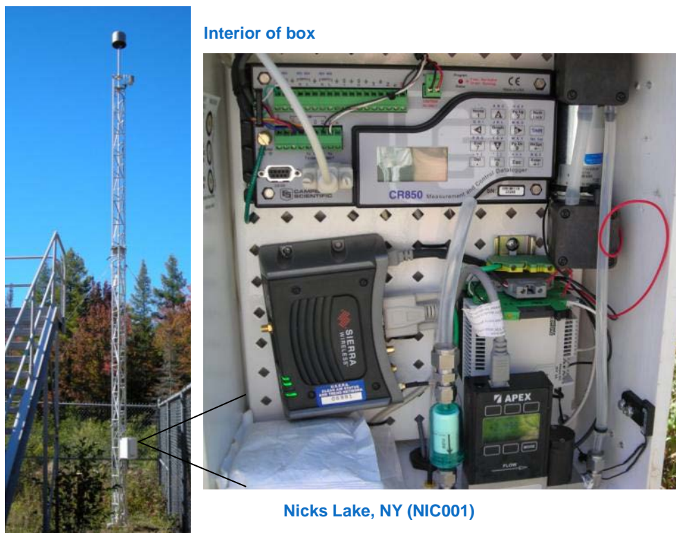
Figure 2-2. Small Footprint Site Operated at Nicks Lake, NY
