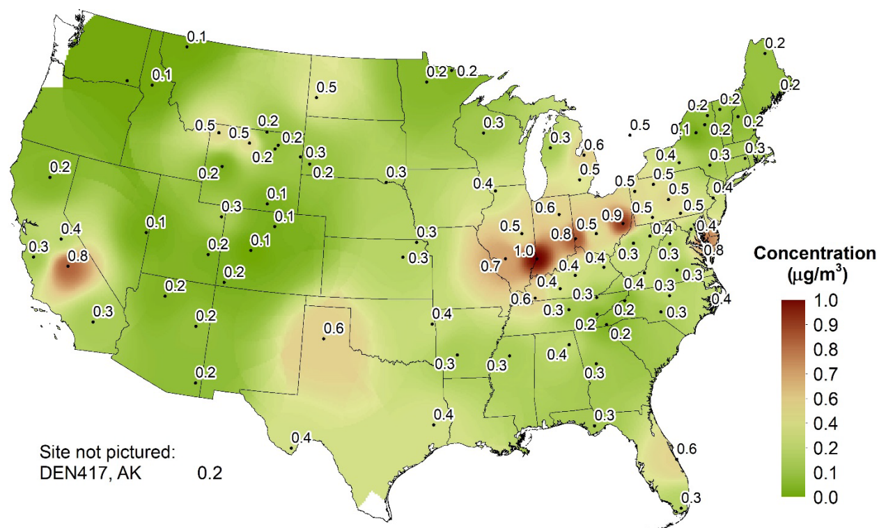
Figure 1-7. Annual Mean SO 2 Concentrations ( \mu\text{g}/\text{m}^3 ) for 2020
