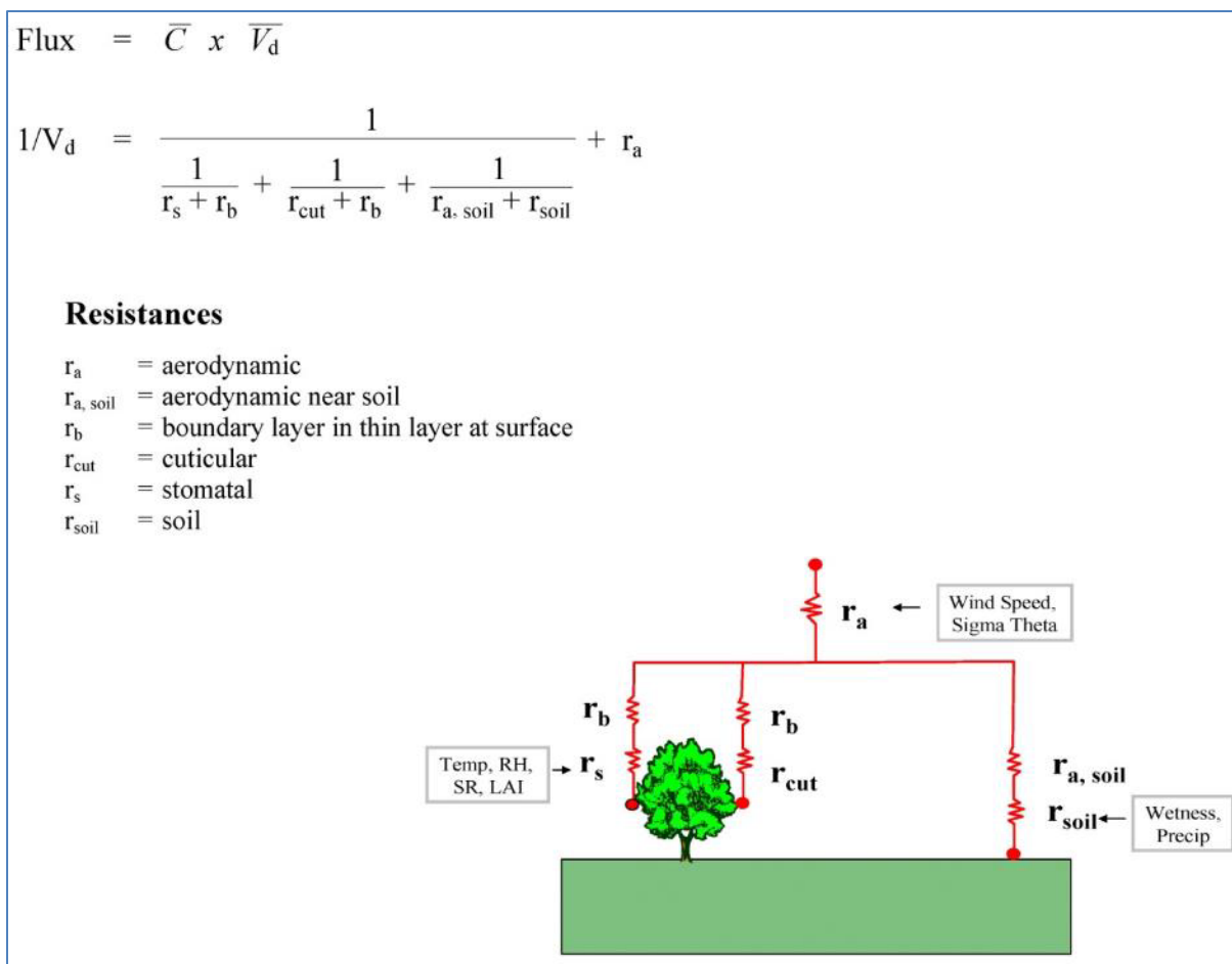
Figure 4-12. Multi-Layer Model
