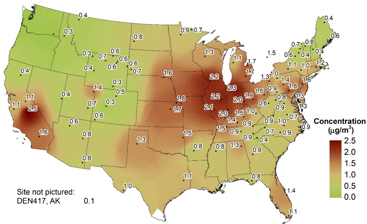
Figure 1-8. Annual Mean Total Nitrate Concentrations ( \mu\text{g}/\text{m}^3 ) for 2020
