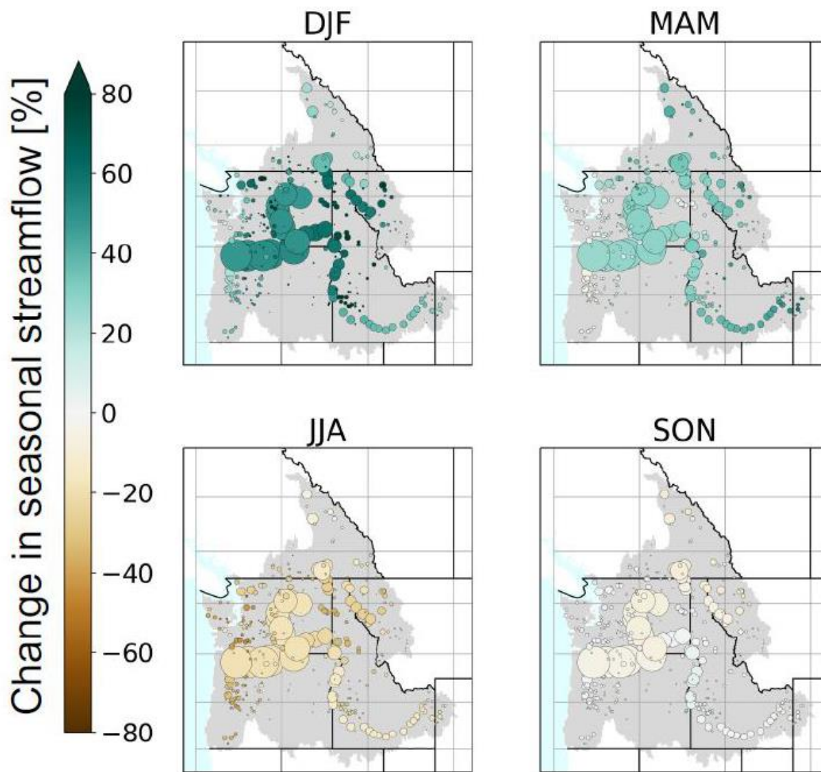
Figure 3-1 Predicted changes in seasonal streamflow between current (1976-2005) and 2030s (2020-2049) (from River Management Joint Operating Committee, 2018)
