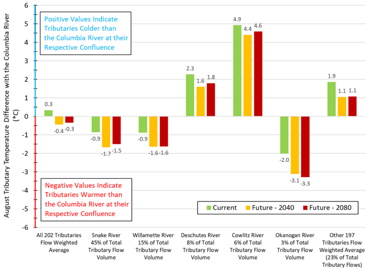
Figure 3-2 Tributary temperatures relative to mainstem Columbia River temperatures at their respective confluences at current, 2040, and 2080 conditions
