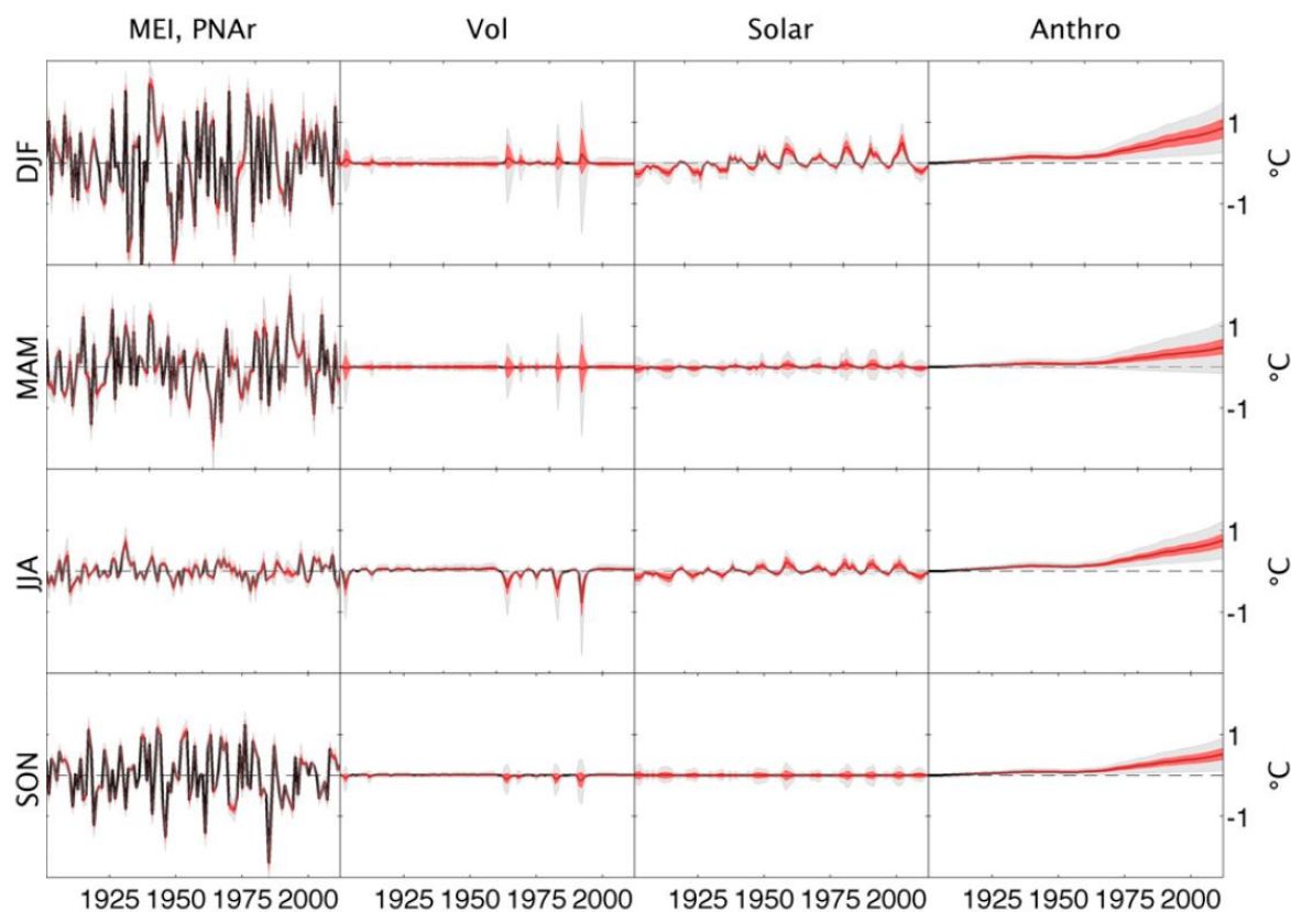
Figure 2-4 Influences of various factors on air temperature variations during the 20th century, by season (adapted from Abatzoglou et al. 2014)
