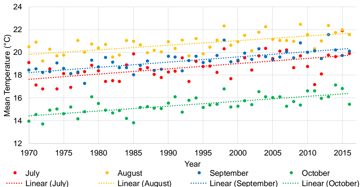
Figure 2-5 Trend in monthly mean temperatures at Bonneville Dam
