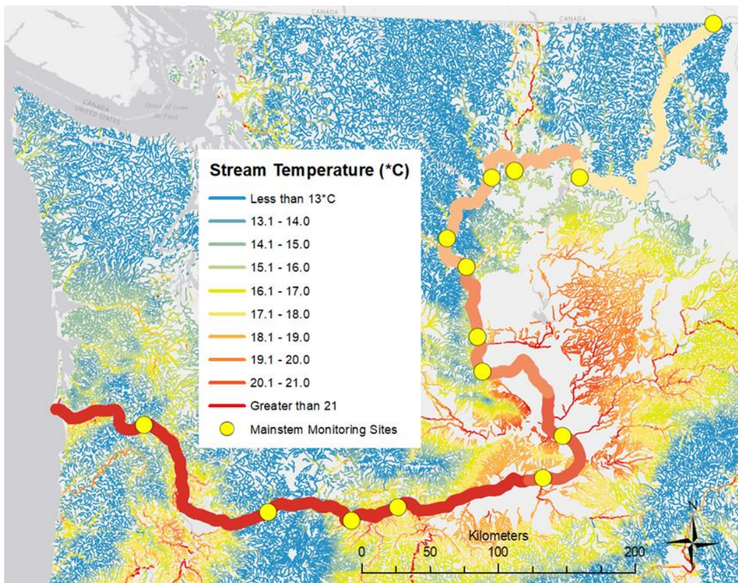
Figure 3-3 Estimated current August mean temperature in the Columbia River and tributaries
