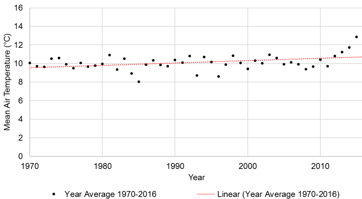
Figure 2-2 Trend for annual average air temperature at Yakima, Oregon
