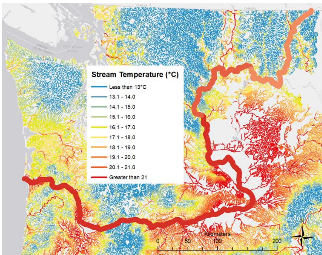
Figure 3-4 Estimated 2080 August Mean temperature in the Columbia River and tributaries
