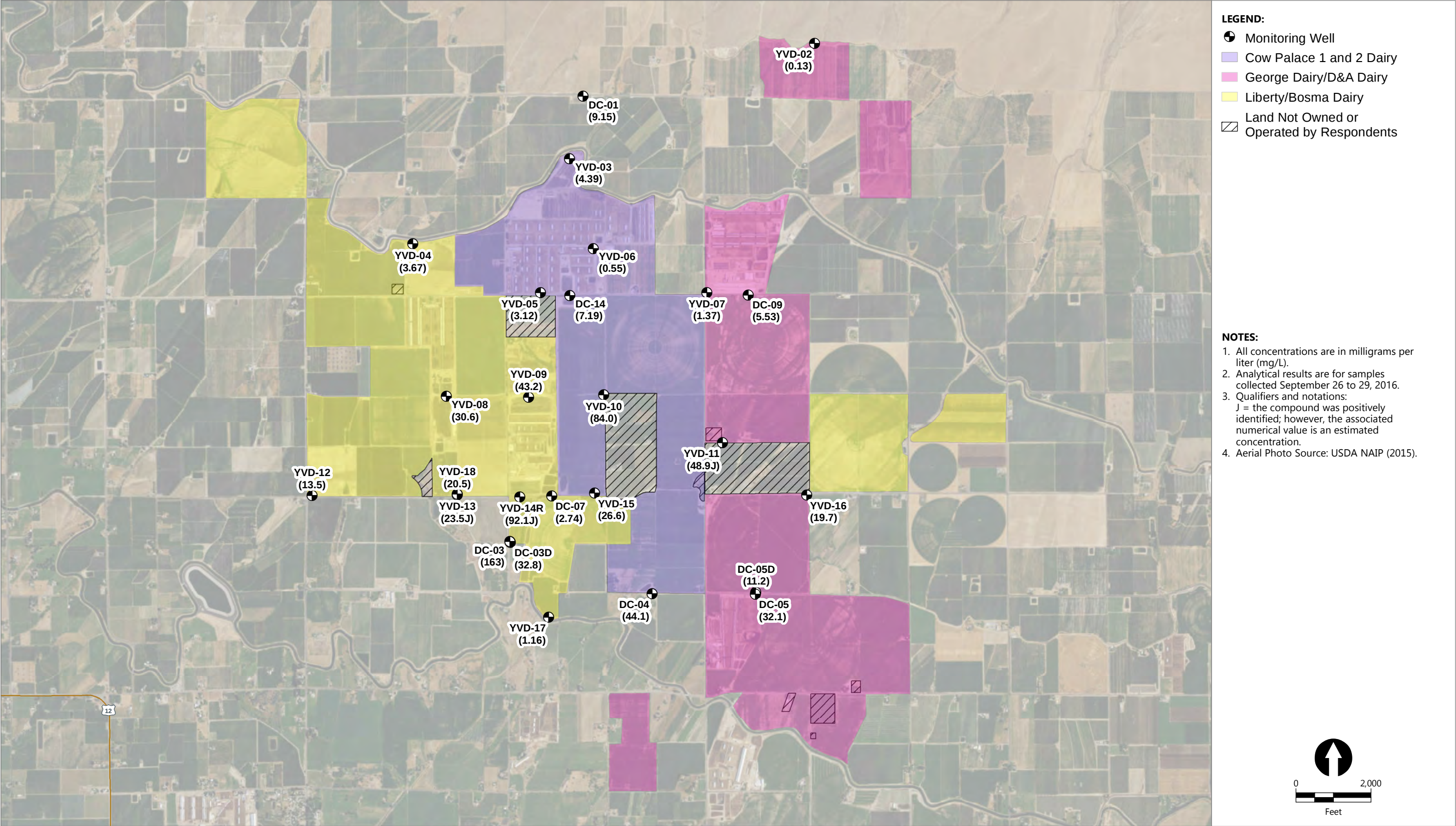
Figure 16A Nitrate Concentrations in Groundwater Third Quarter 2016 Groundwater Monitoring Data Report Third Quarter 2016 Yakima Valley Dairies
