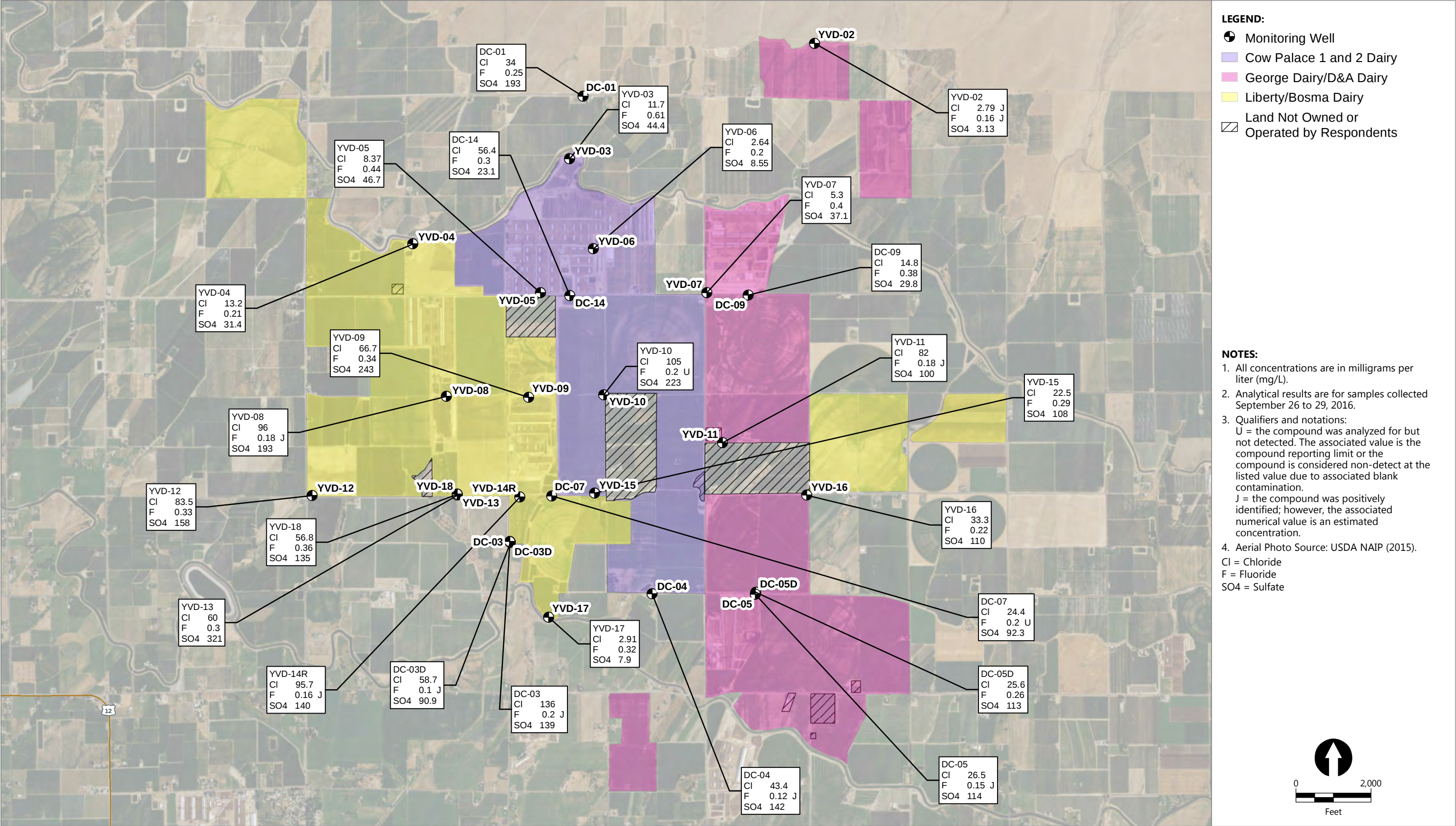
Figure 24 Anion Concentrations in Groundwater Third Quarter 2016 Groundwater Monitoring Data Report Third Quarter 2016 Yakima Valley Dairies
