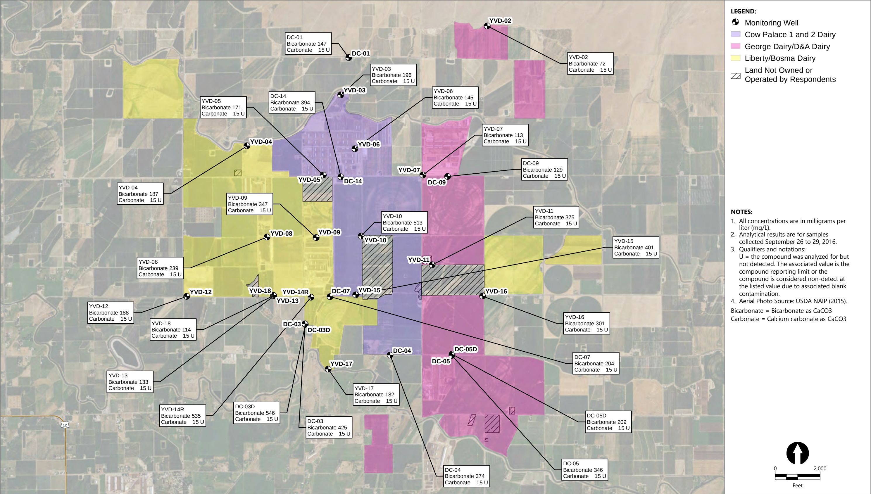
Figure 26 Alkalinity Concentrations in Groundwater Third Quarter 2016 Groundwater Monitoring Data Report Third Quarter 2016 Yakima Valley Dairies
