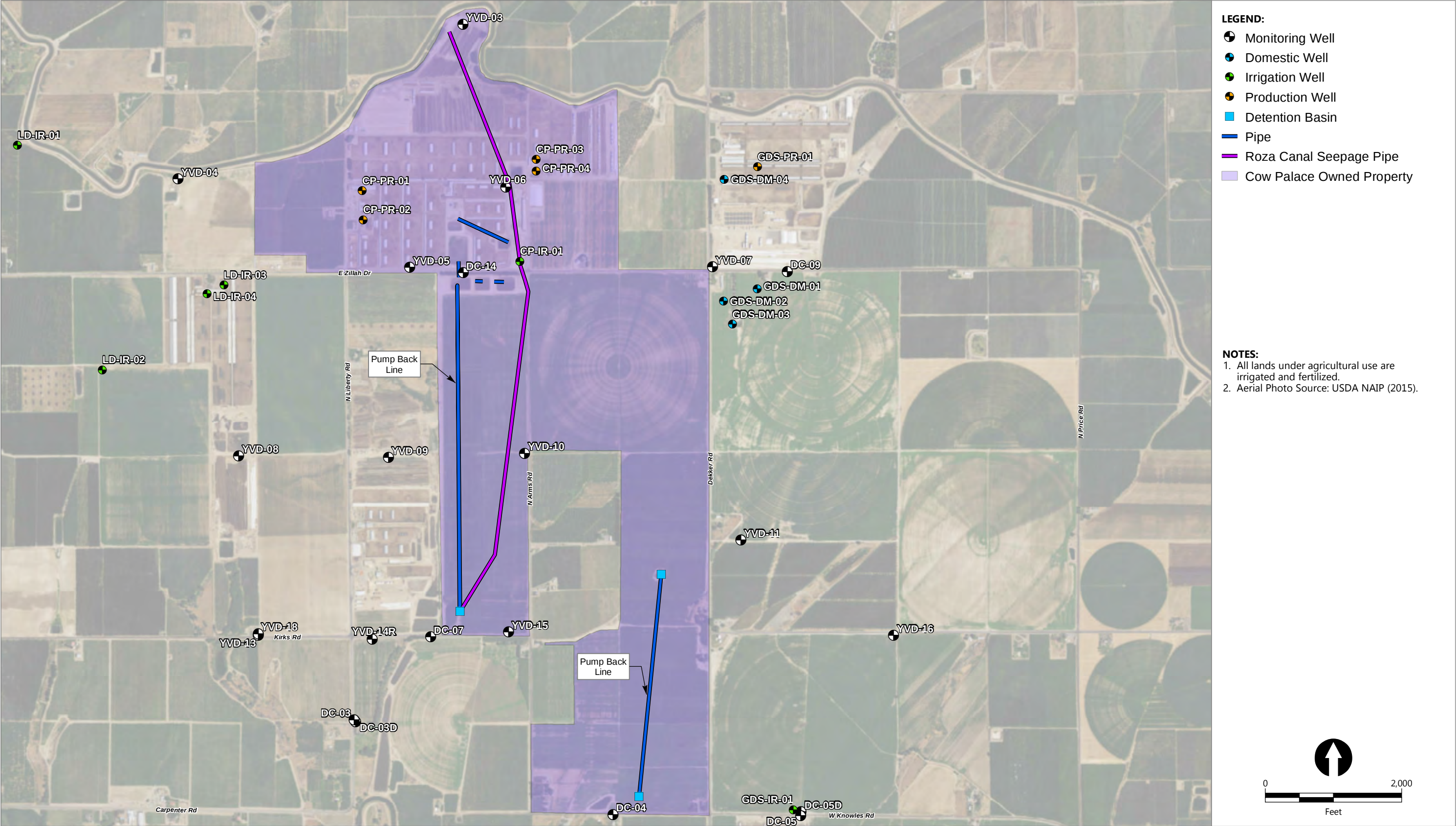
Figure 3B Facility Plan – Cow Palace Dairy Groundwater Monitoring Data Report Third Quarter 2016 Yakima Valley Dairies
