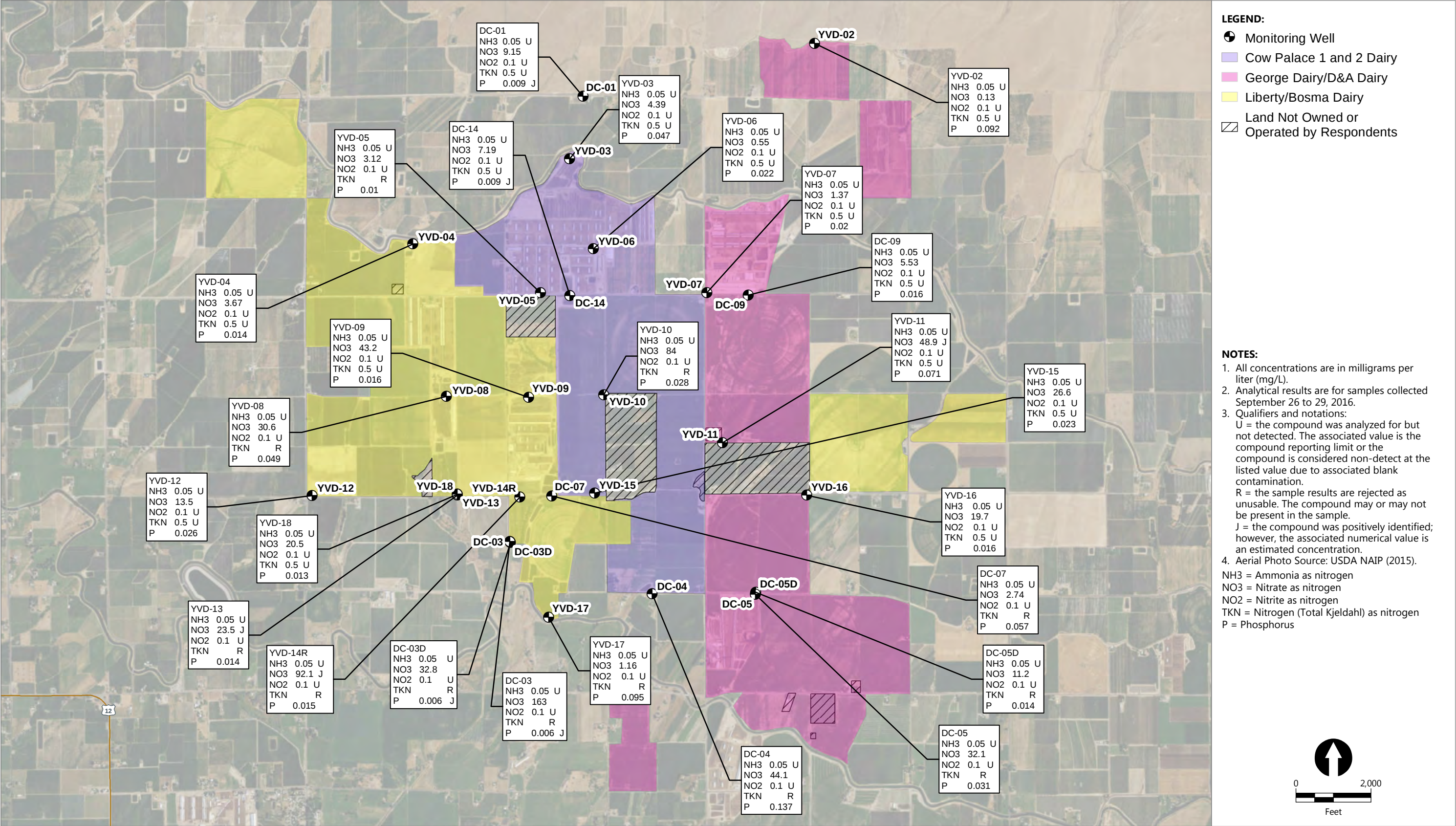
Figure 23 Nutrient Concentrations in Groundwater Third Quarter 2016 Groundwater Monitoring Data Report Third Quarter 2016 Yakima Valley Dairies
