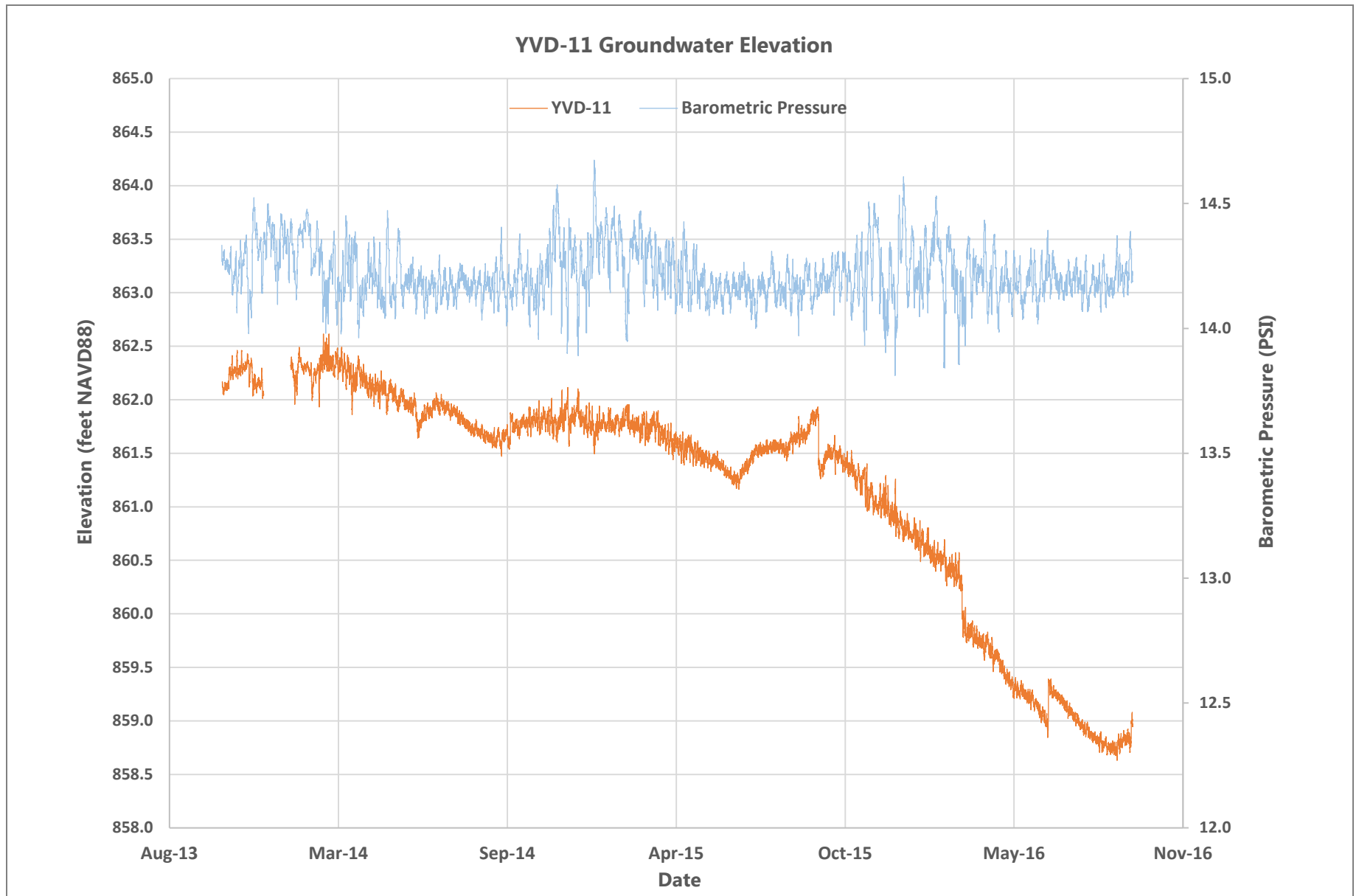
Figure 15G Groundwater Hydrograph – Well YVD-11 Groundwater Monitoring Data Report Third Quarter 2016 Yakima Valley Dairies
