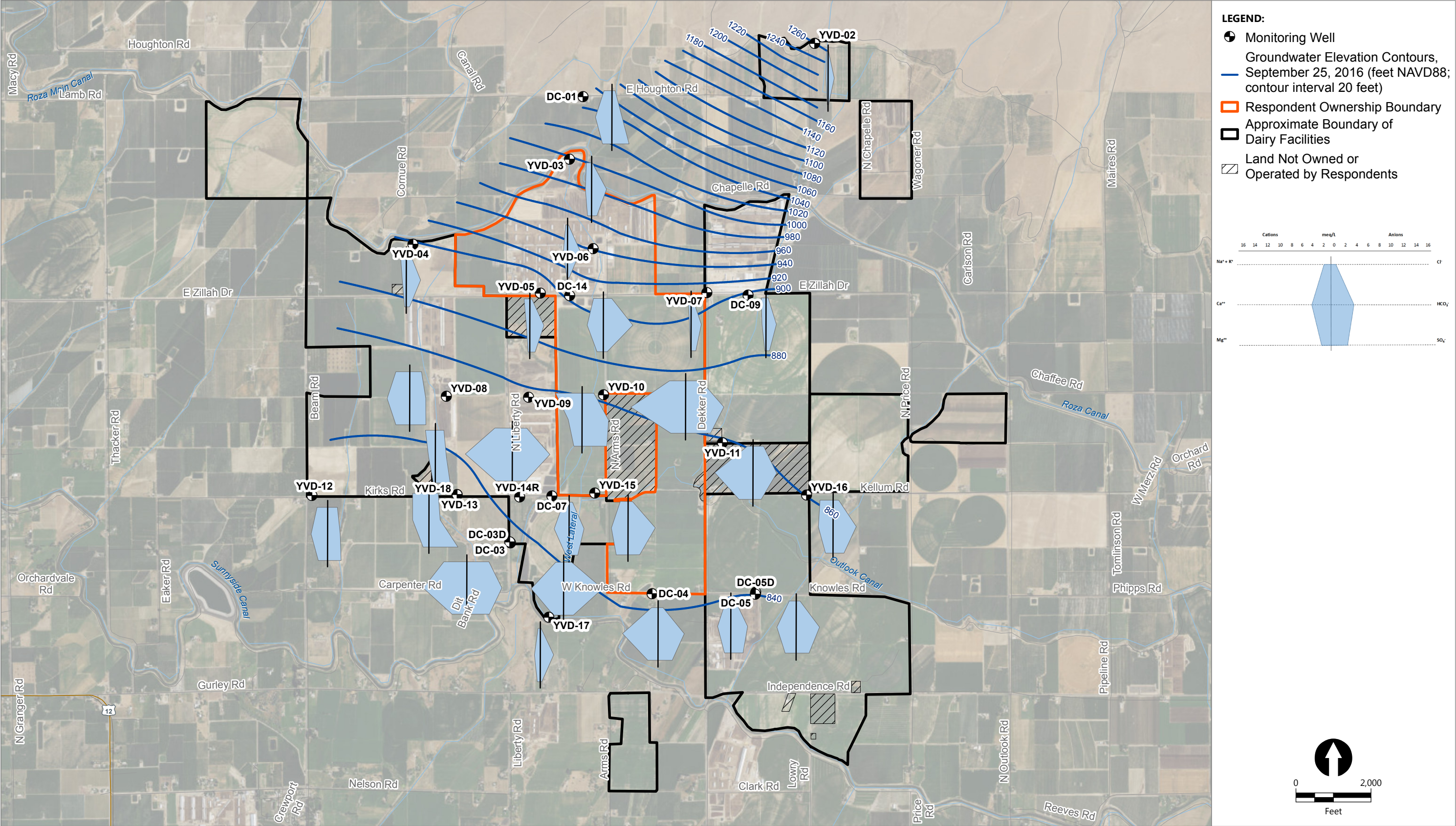
Figure 28 Stiff Diagrams and Groundwater Elevation Contour Map Groundwater Monitoring Data Report Third Quarter 2016 Yakima Valley Dairies
