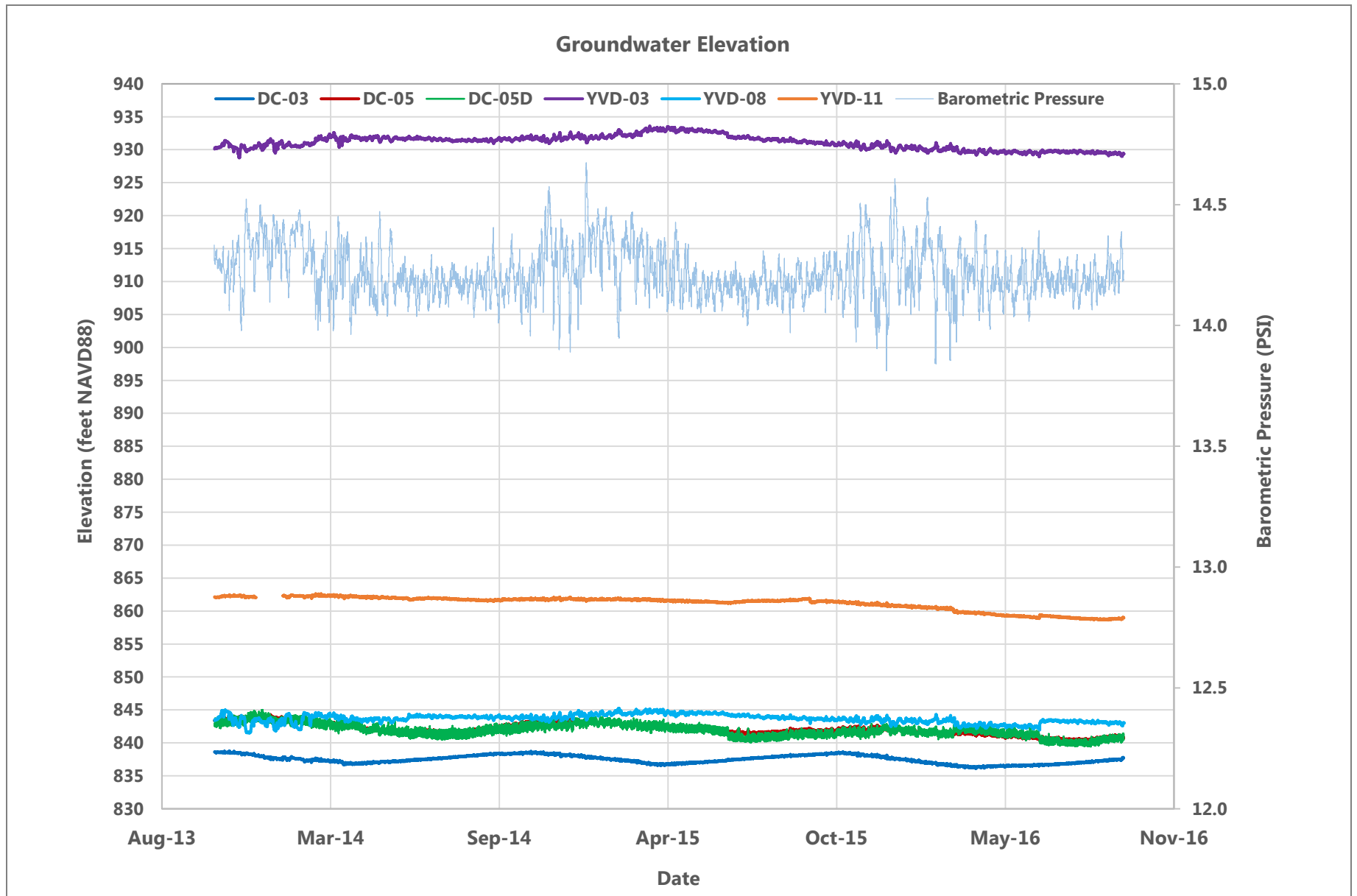
Figure 15A Groundwater Hydrographs – All Transducers Groundwater Monitoring Data Report Third Quarter 2016 Yakima Valley Dairies
