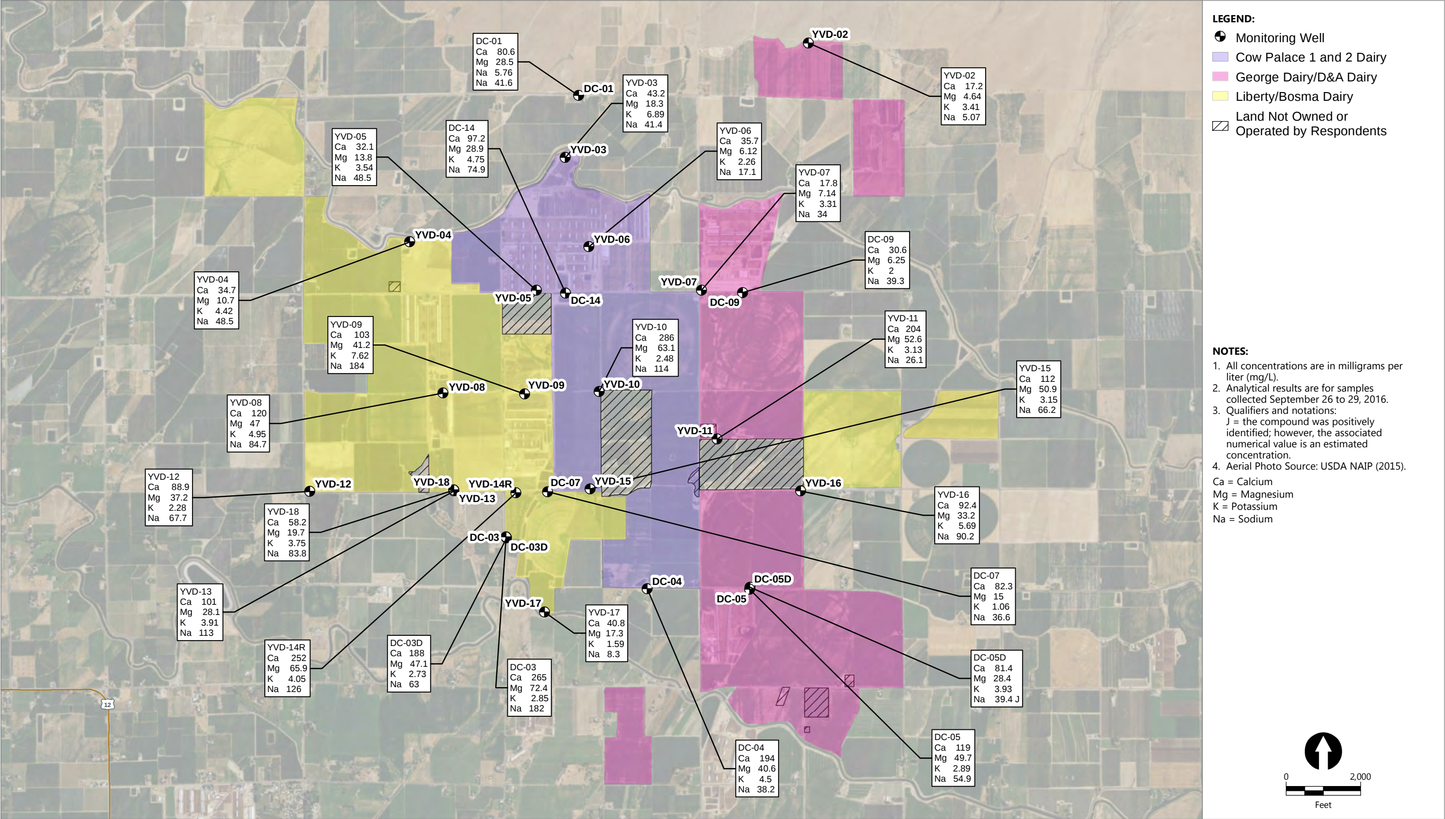
Figure 25 Metals Concentrations in Groundwater Third Quarter 2016 Groundwater Monitoring Data Report Third Quarter 2016 Yakima Valley Dairies
