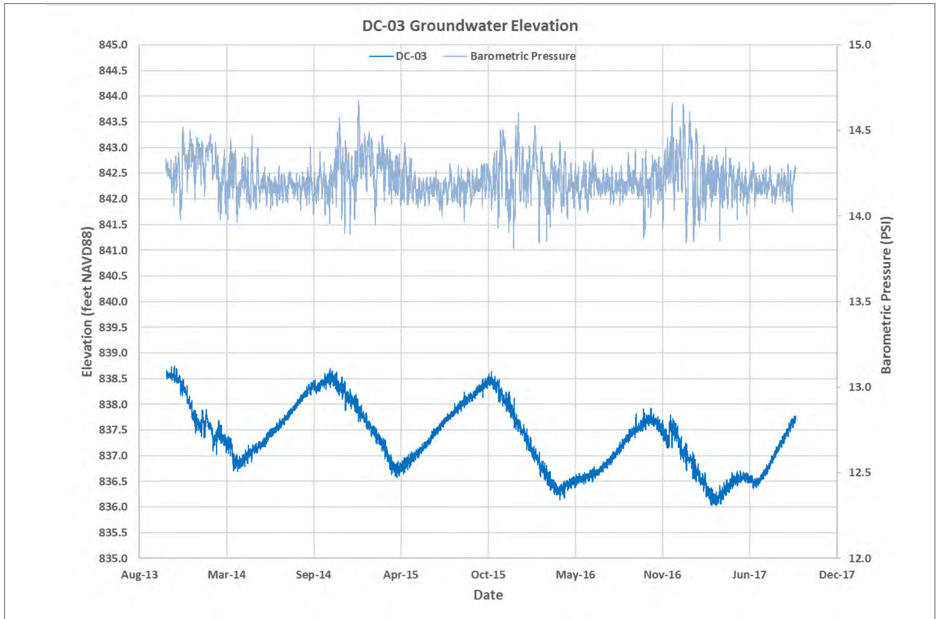
Figure 16B Groundwater Hydrographs – DC-03 Groundwater Monitoring Data Report – Third Quarter 2017 Yakima Valley Dairies
