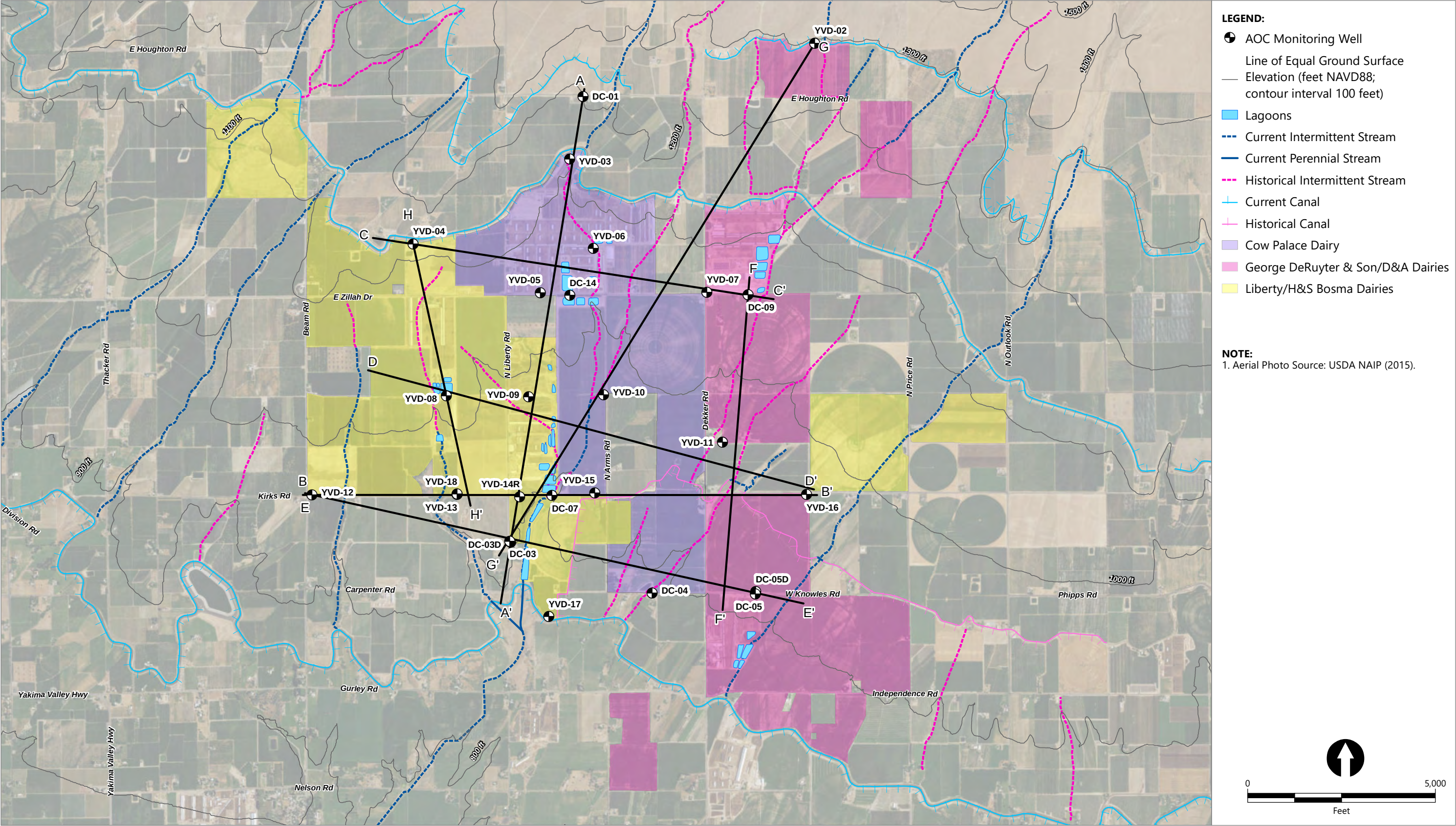
Figure 6 Cross Section Location Map Groundwater Monitoring Data Report – Third Quarter 2017 Yakima Valley Dairies
