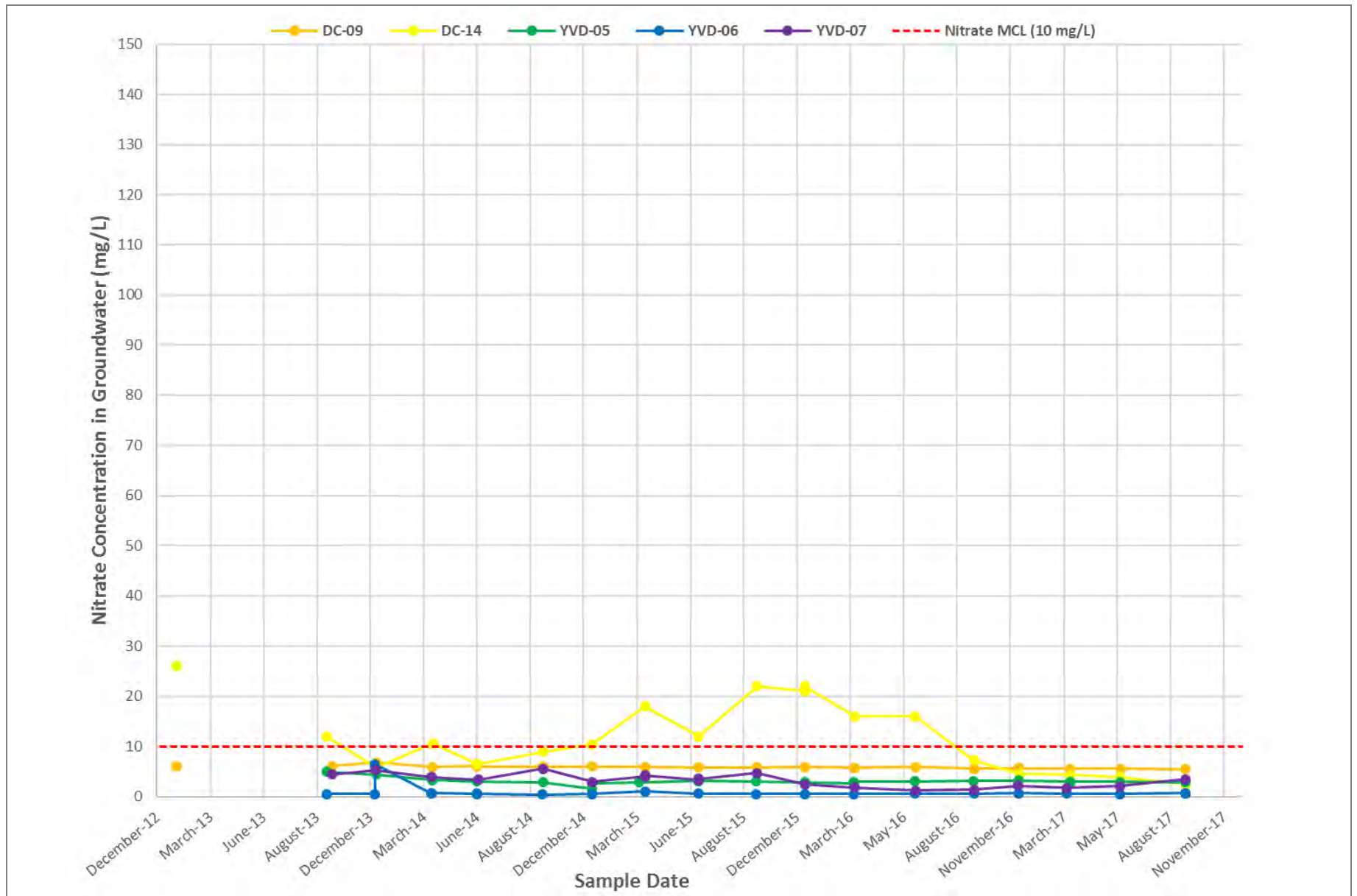
Figure 21 Nitrate Concentrations – Northern Wells Groundwater Monitoring Data Report – Third Quarter 2017 Yakima Valley Dairies
