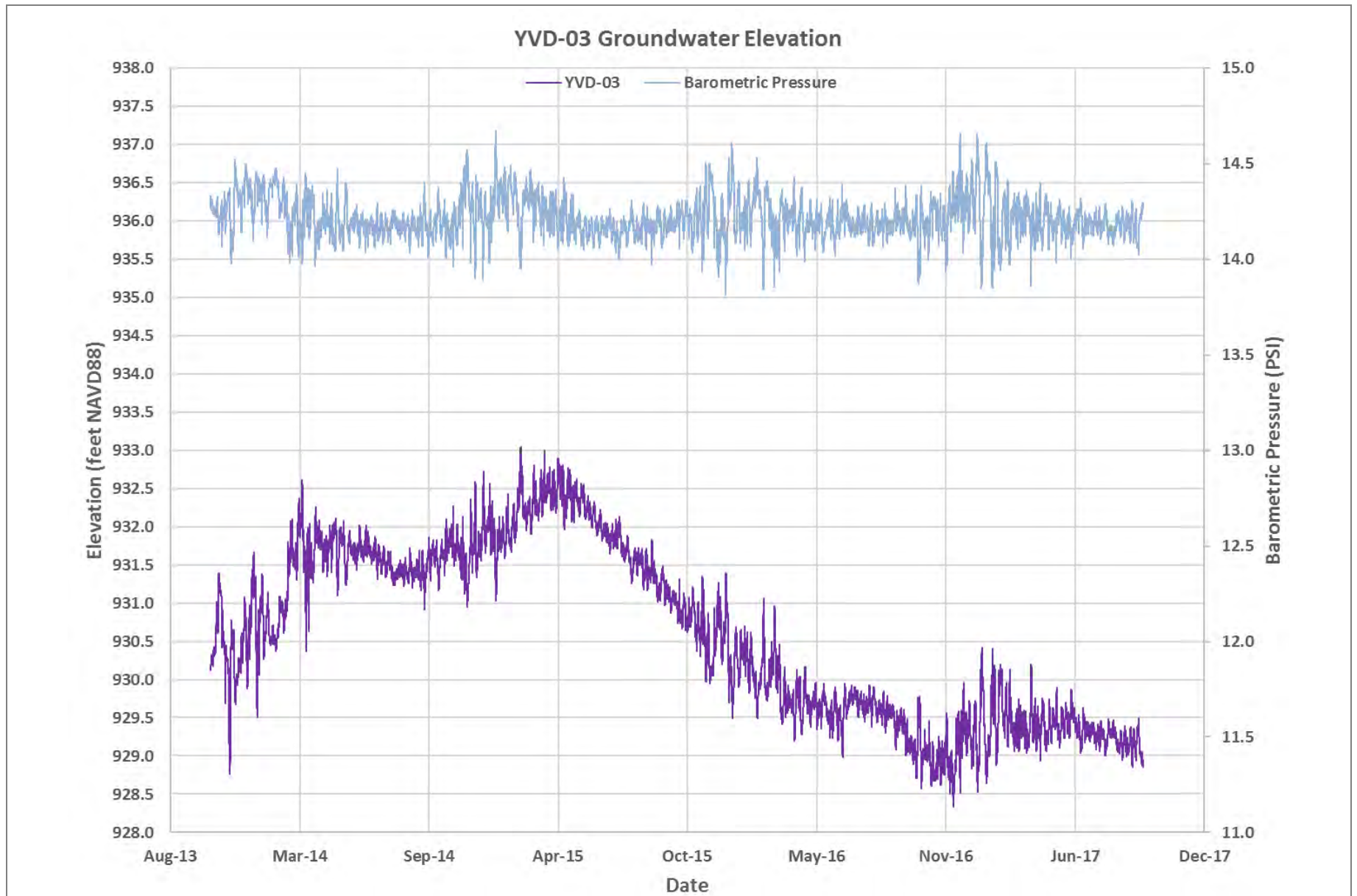
Figure 16E Groundwater Hydrographs – YVD-03 Groundwater Monitoring Data Report – Third Quarter 2017 Yakima Valley Dairies
