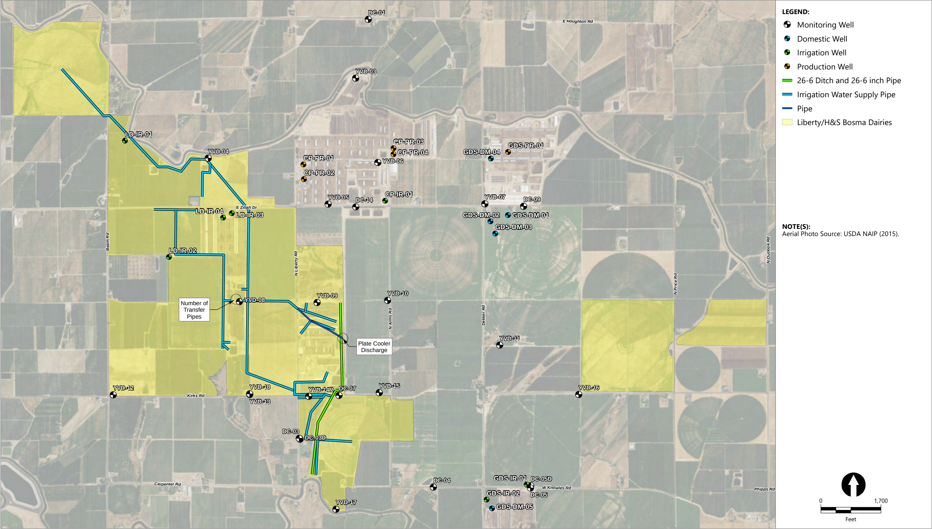
Figure 3D Facility Plan – Liberty/H&S Bosma Dairies Groundwater Monitoring Data Report – Third Quarter 2017 Yakima Valley Dairies
