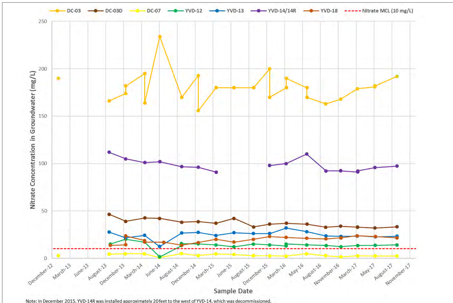
Figure 19 Nitrate Concentrations – West Downgradient Wells Groundwater Monitoring Data Report – Third Quarter 2017 Yakima Valley Dairies
