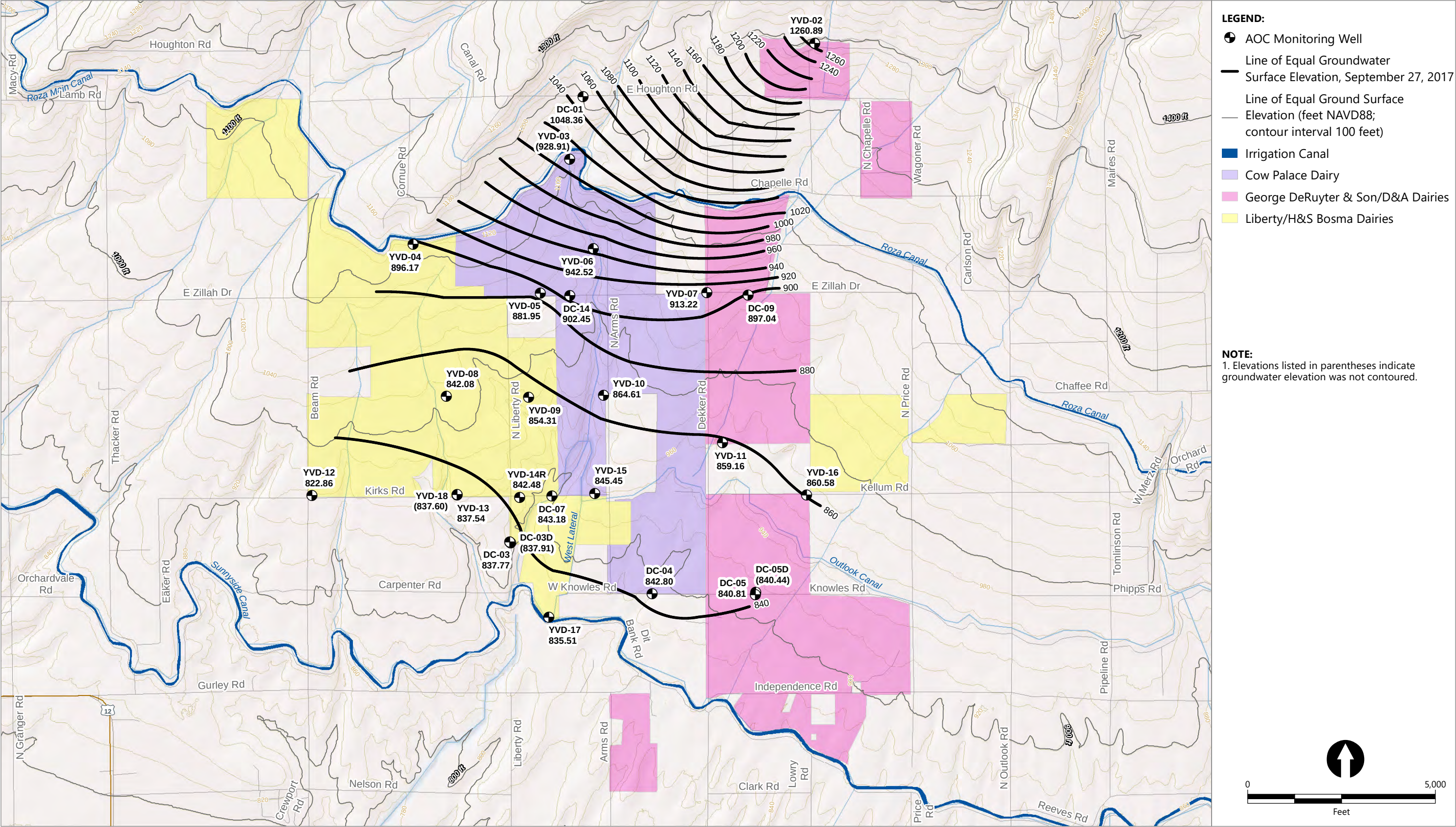
Figure 15 Surficial Aquifer Groundwater Elevation Contour Map Groundwater Monitoring Data Report – Third Quarter 2017 Yakima Valley Dairies
