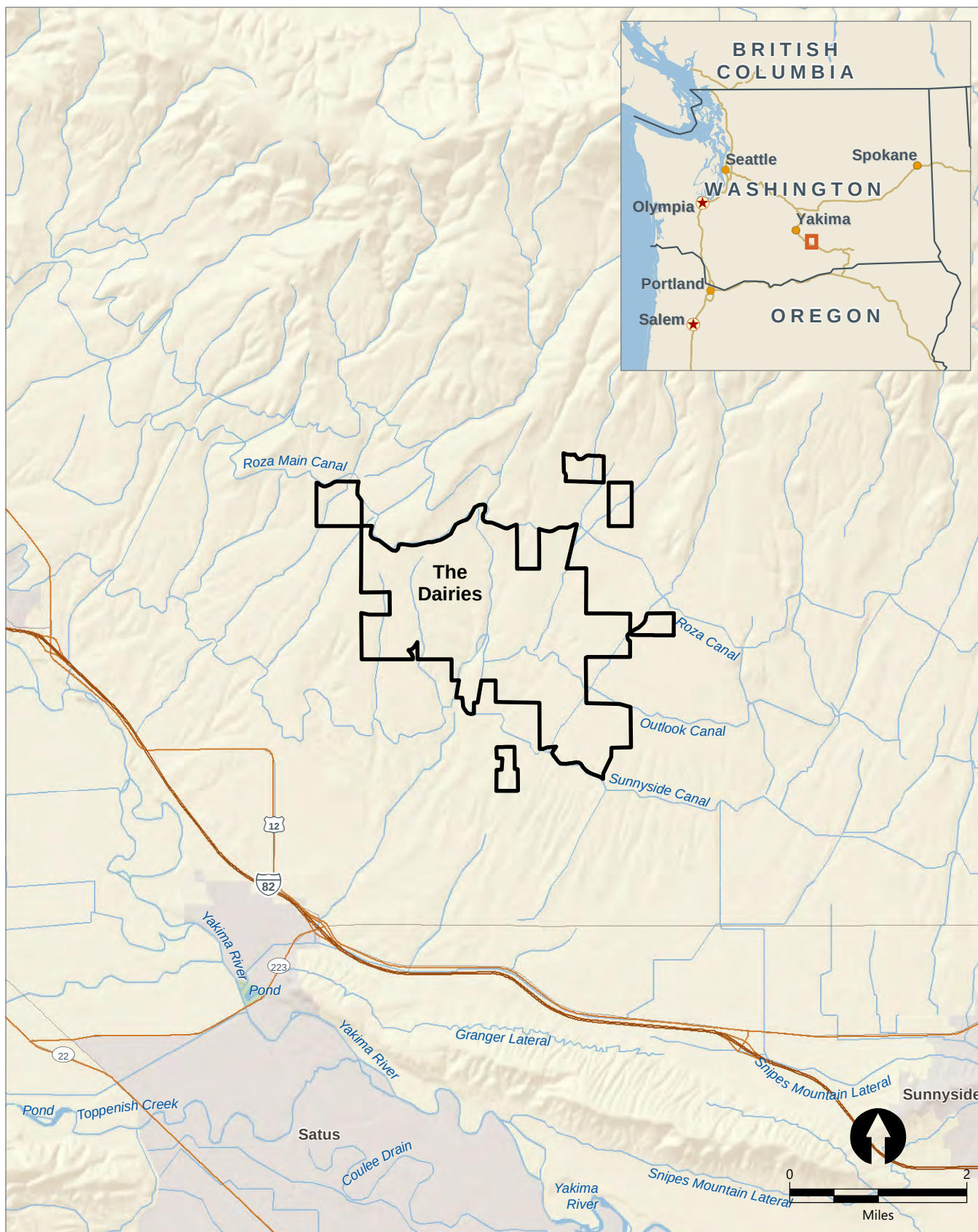
Figure 1 Site Vicinity Map Groundwater Monitoring Data Report – Third Quarter 2017 Yakima Valley Dairies
