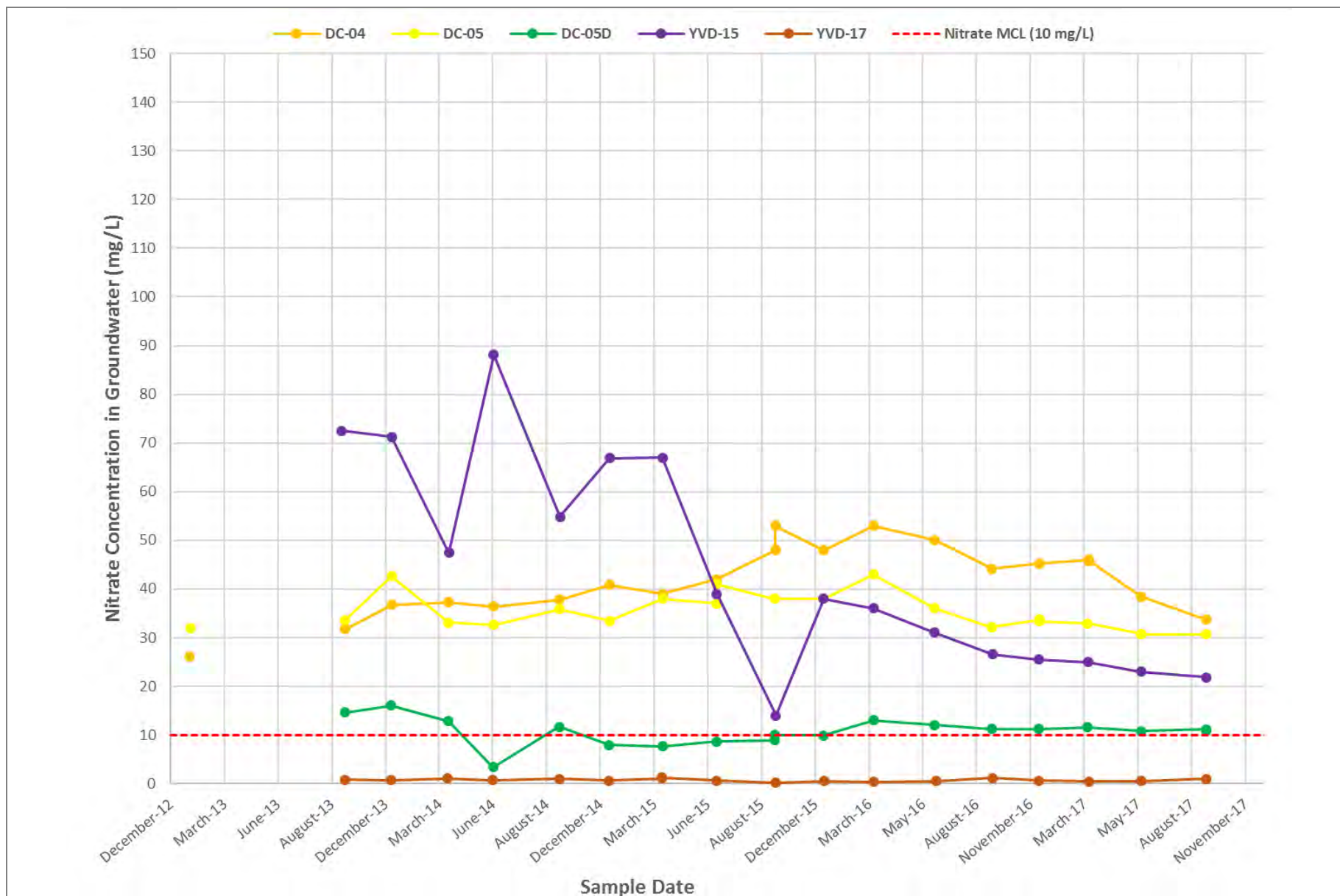
Figure 18 Nitrate Concentrations – East Downgradient Wells Groundwater Monitoring Data Report – Third Quarter 2017 Yakima Valley Dairies
