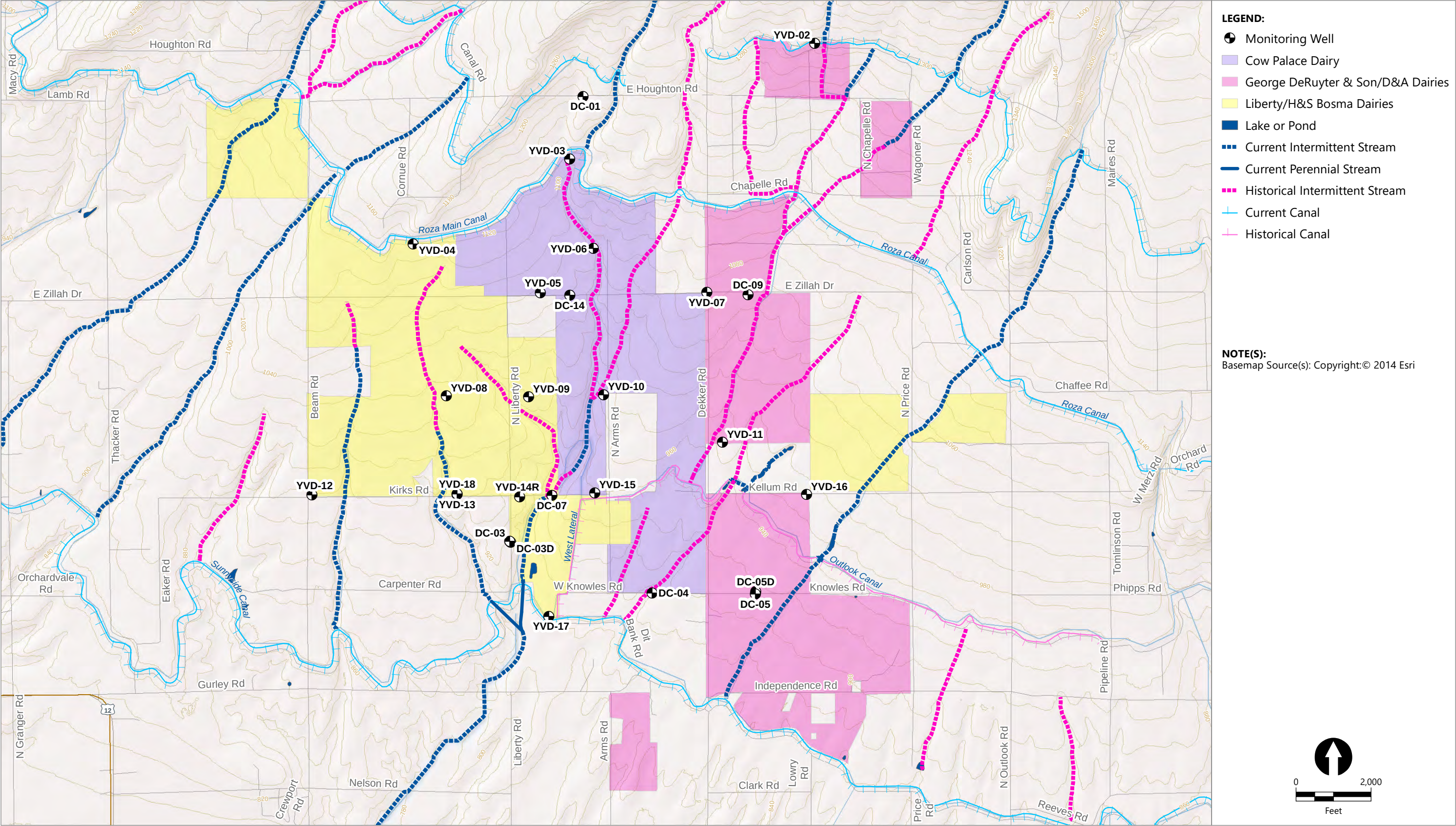
Figure 2A Site Map Groundwater Monitoring Data Report – Third Quarter 2017 Yakima Valley Dairies
