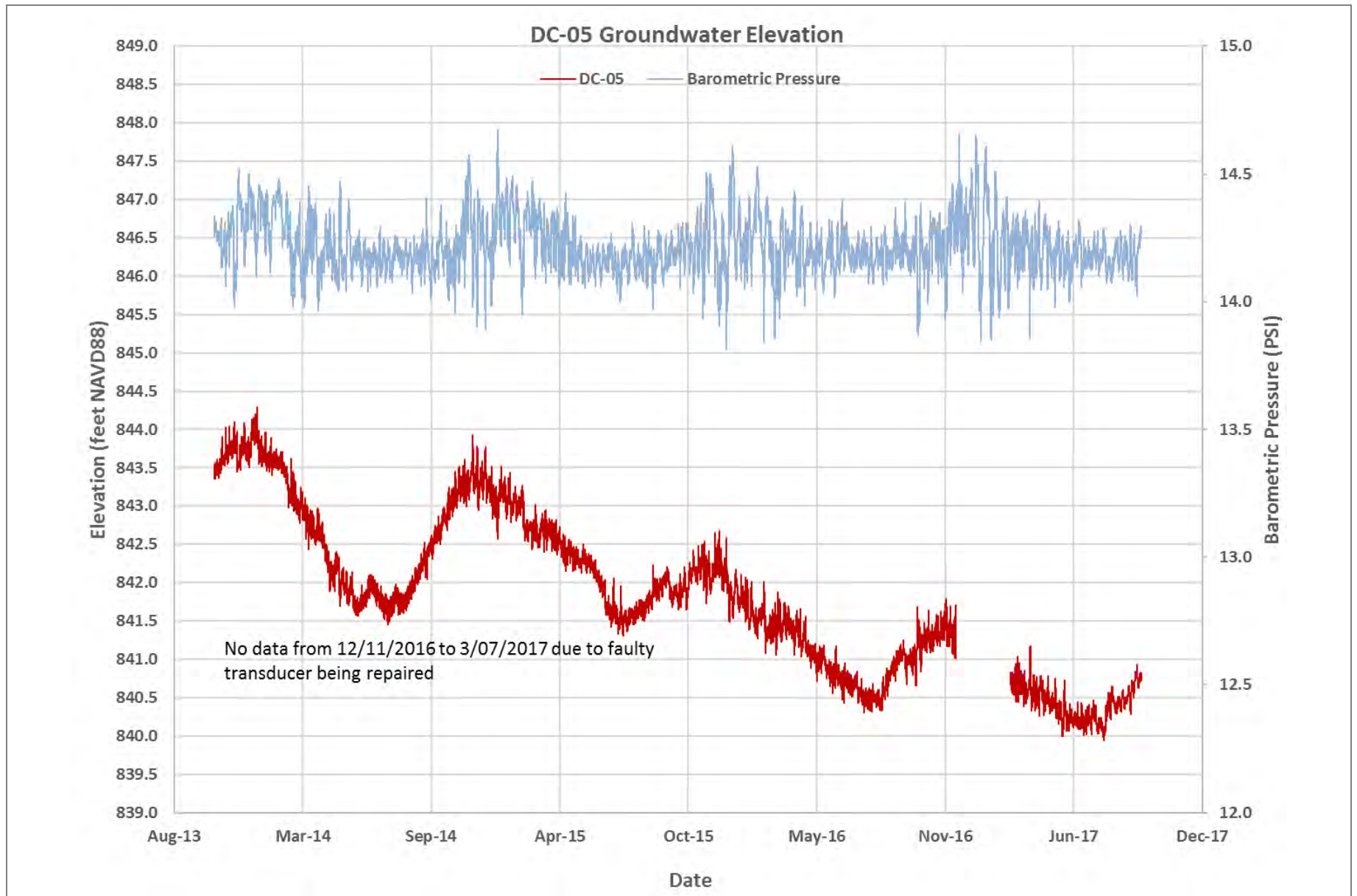
Figure 16C Groundwater Hydrographs – DC-05 Groundwater Monitoring Data Report – Third Quarter 2017 Yakima Valley Dairies
