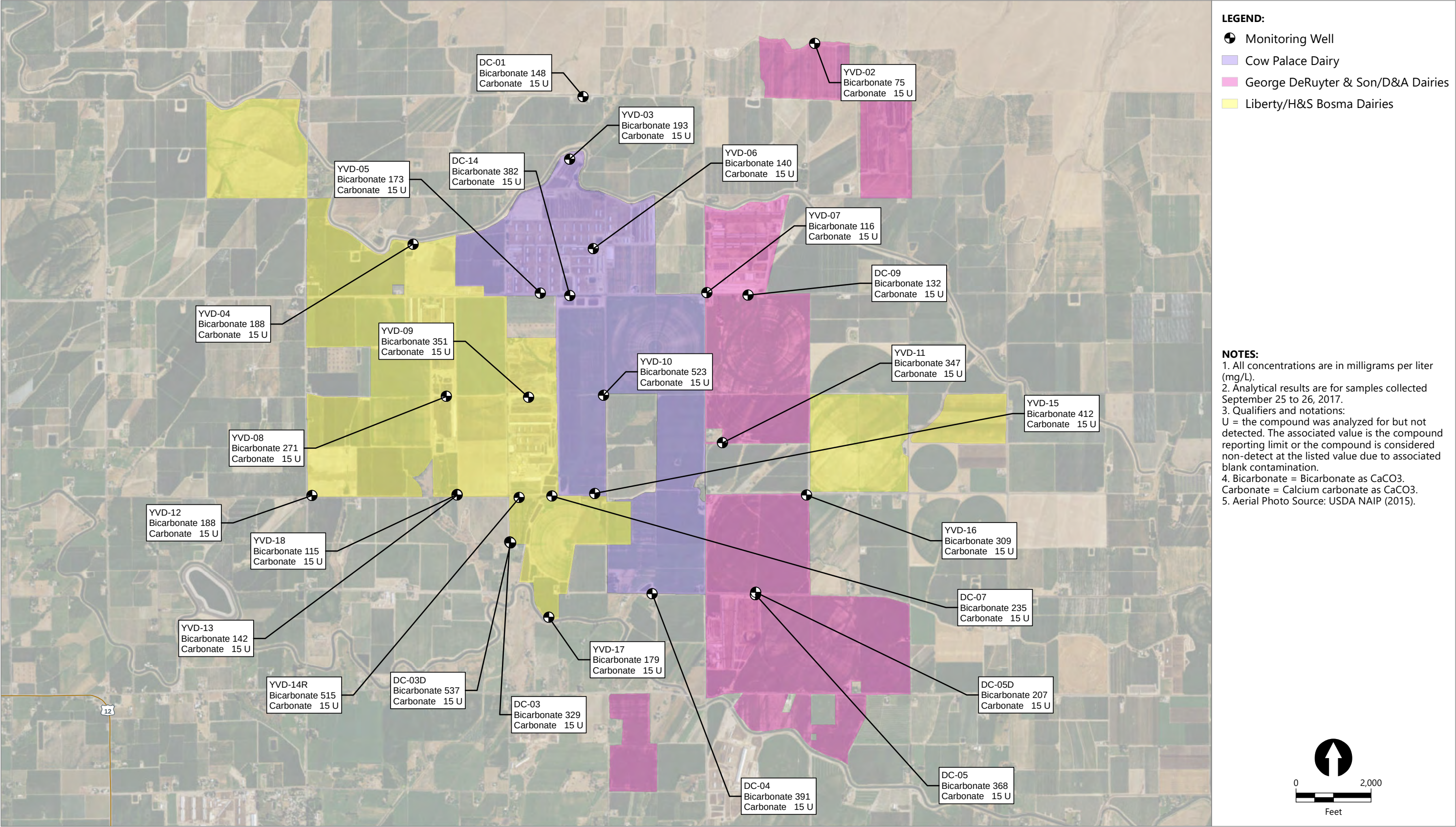
Figure 27 Alkalinity Concentrations in Groundwater Third Quarter 2017 Groundwater Monitoring Data Report – Third Quarter 2017 Yakima Valley Dairies
