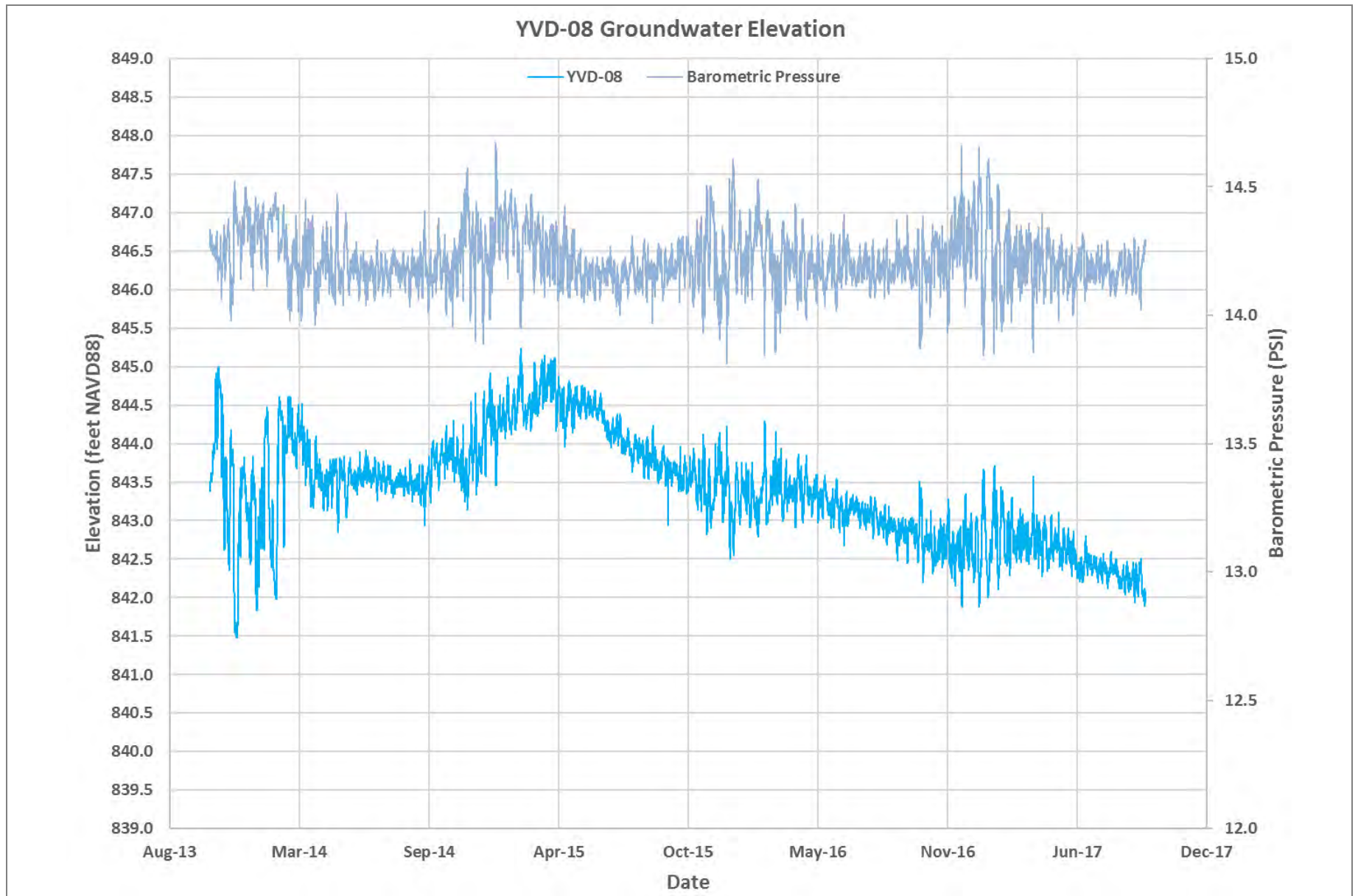
Figure 16F Groundwater Hydrographs – YVD-08 Groundwater Monitoring Data Report – Third Quarter 2017 Yakima Valley Dairies
