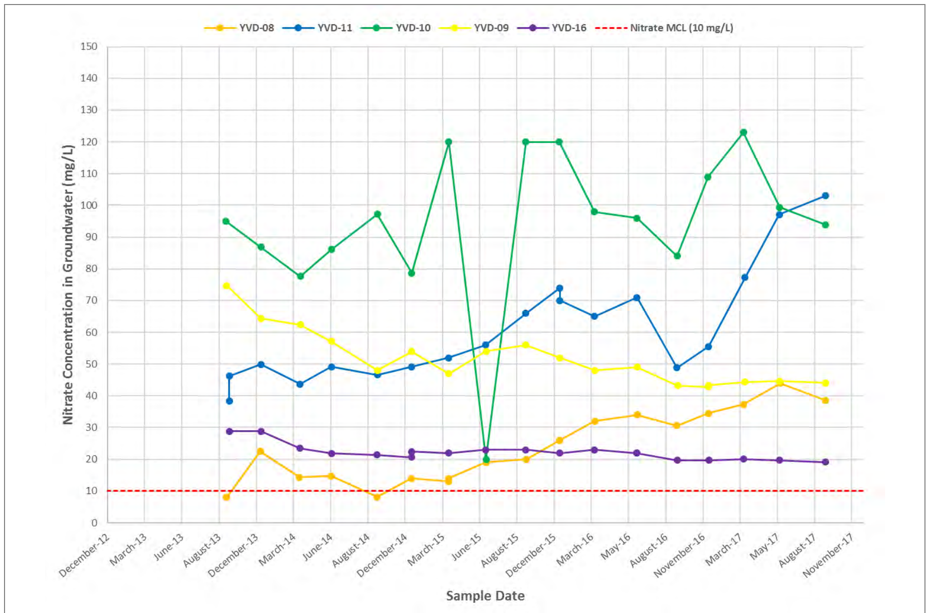
Figure 20 Nitrate Concentrations – Central Wells Groundwater Monitoring Data Report – Third Quarter 2017 Yakima Valley Dairies
