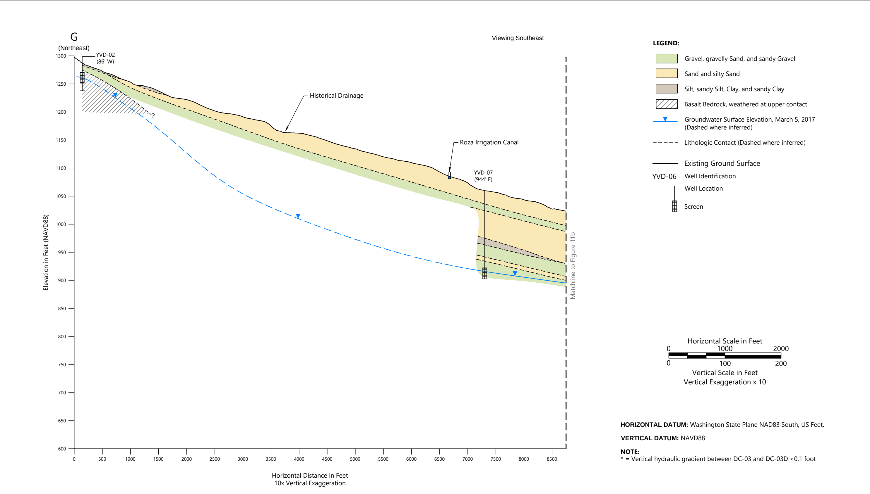
Figure 13A Cross Section G-G'
