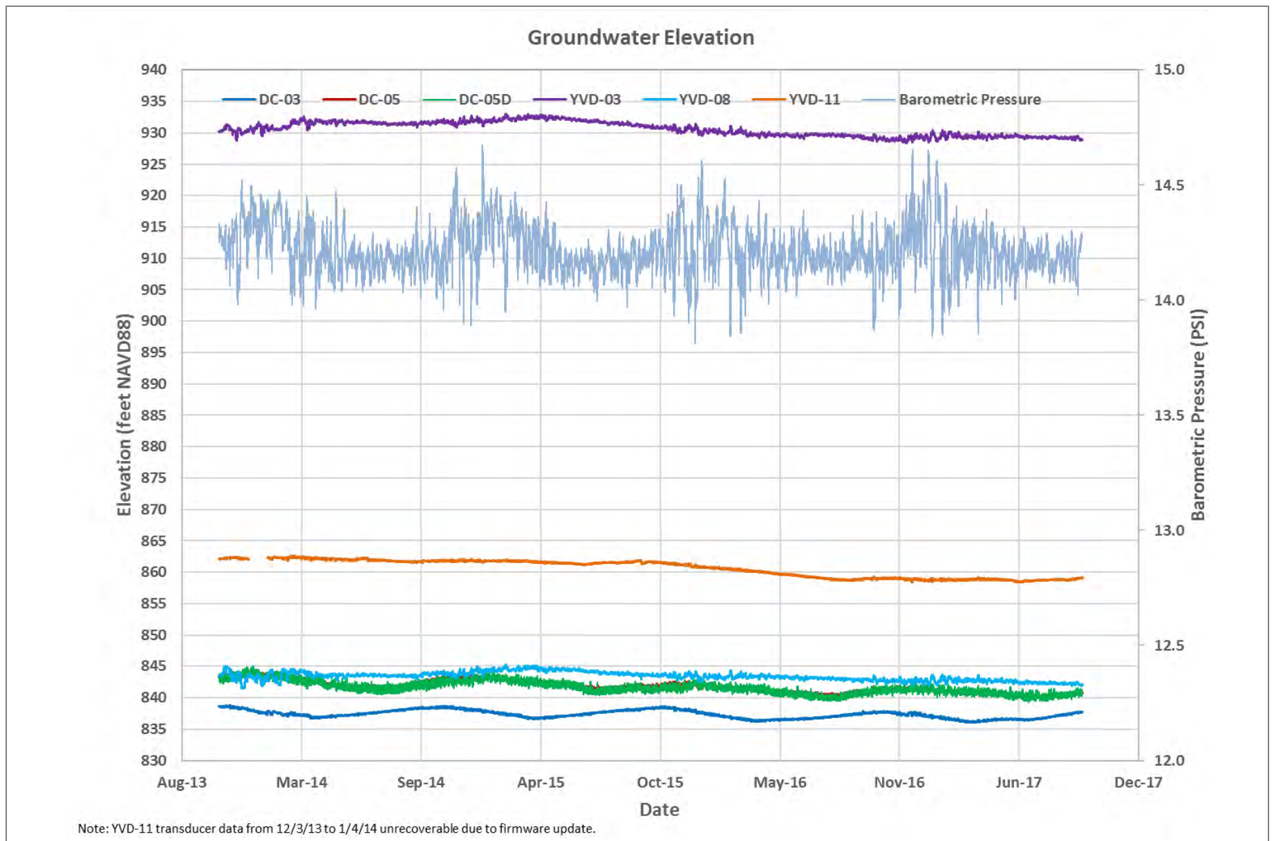
Figure 16A Groundwater Hydrographs – All Transducers Groundwater Monitoring Data Report – Third Quarter 2017 Yakima Valley Dairies
