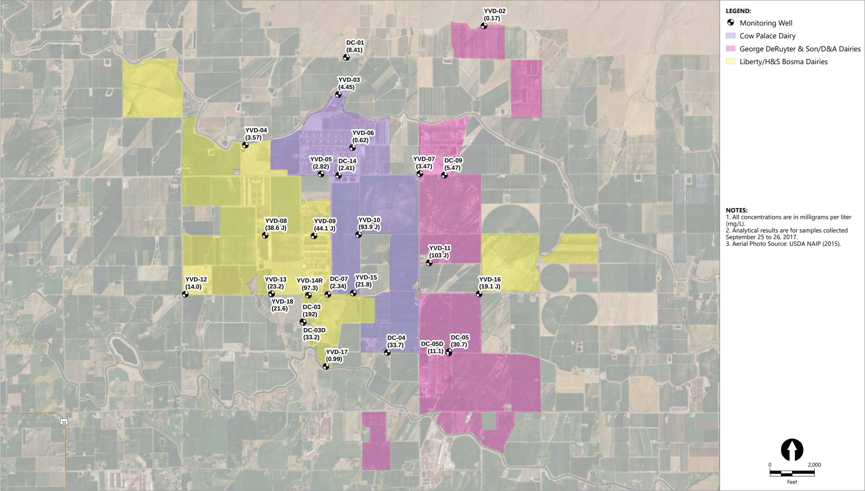
Figure 17A Nitrate Concentrations in Groundwater Third Quarter 2017 Groundwater Monitoring Data Report – Third Quarter 2017 Yakima Valley Dairies
