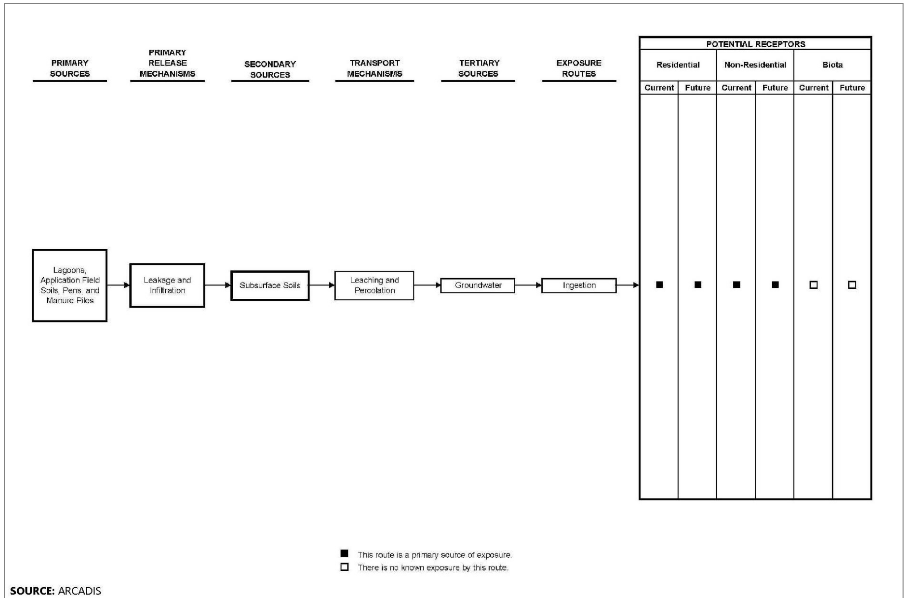
Figure 4 Conceptual Site Model Flow Chart Groundwater Monitoring Data Report – Third Quarter 2017 Yakima Valley Dairies
