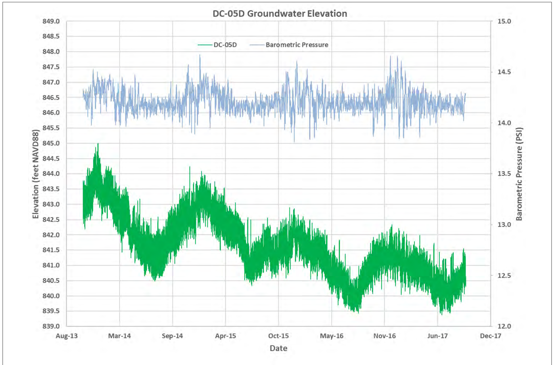
Figure 16D Groundwater Hydrographs – DC-05D Groundwater Monitoring Data Report – Third Quarter 2017 Yakima Valley Dairies
