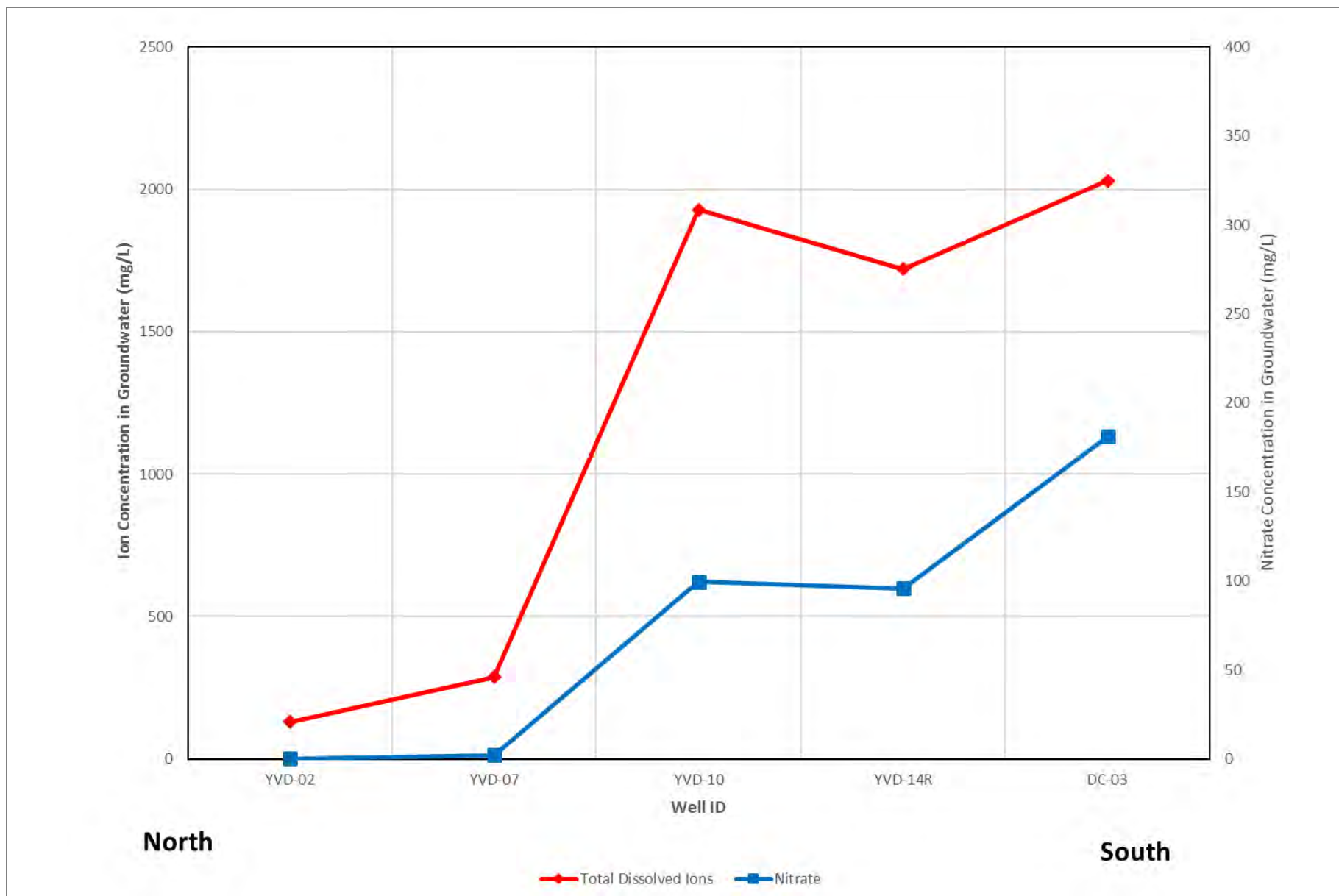
Figure 23 Nitrate and Total Dissolved Ion Concentration along Cross Section G-G' Transect Groundwater Monitoring Data Report – Third Quarter 2017 Yakima Valley Dairies
