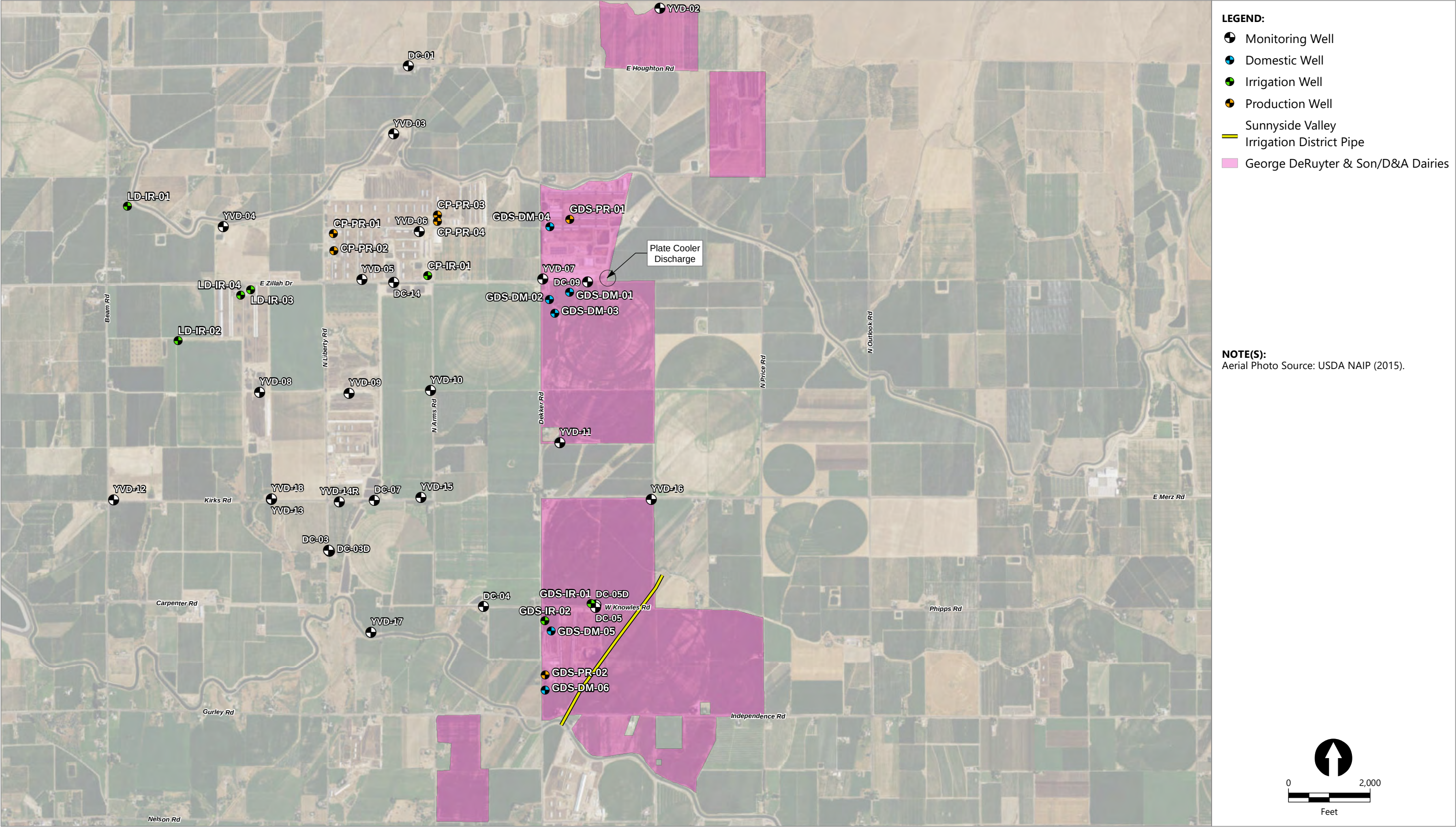
Figure 3C Facility Plan – George DeRuyter & Son/D&A Dairies Groundwater Monitoring Data Report – Third Quarter 2017 Yakima Valley Dairies
