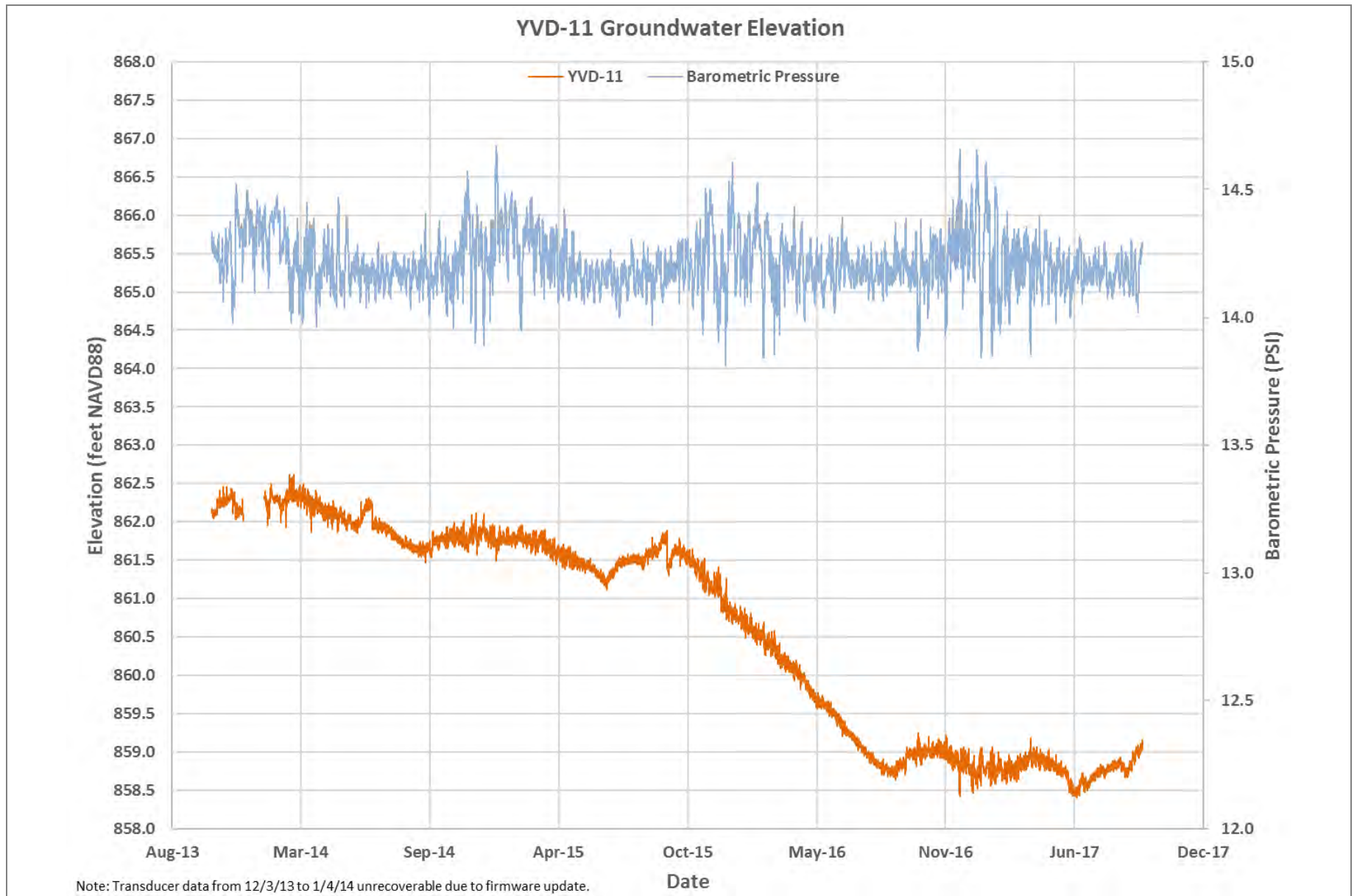
Figure 16G Groundwater Hydrographs – YVD-11 Groundwater Monitoring Data Report – Third Quarter 2017 Yakima Valley Dairies
