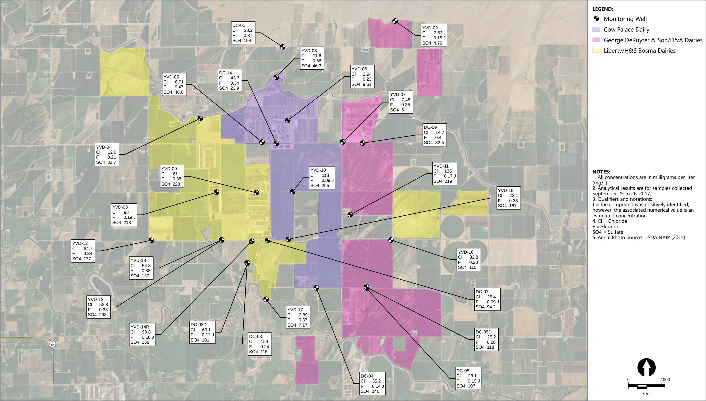
Figure 25 Anion Concentrations in Groundwater Third Quarter 2017 Groundwater Monitoring Data Report – Third Quarter 2017 Yakima Valley Dairies
