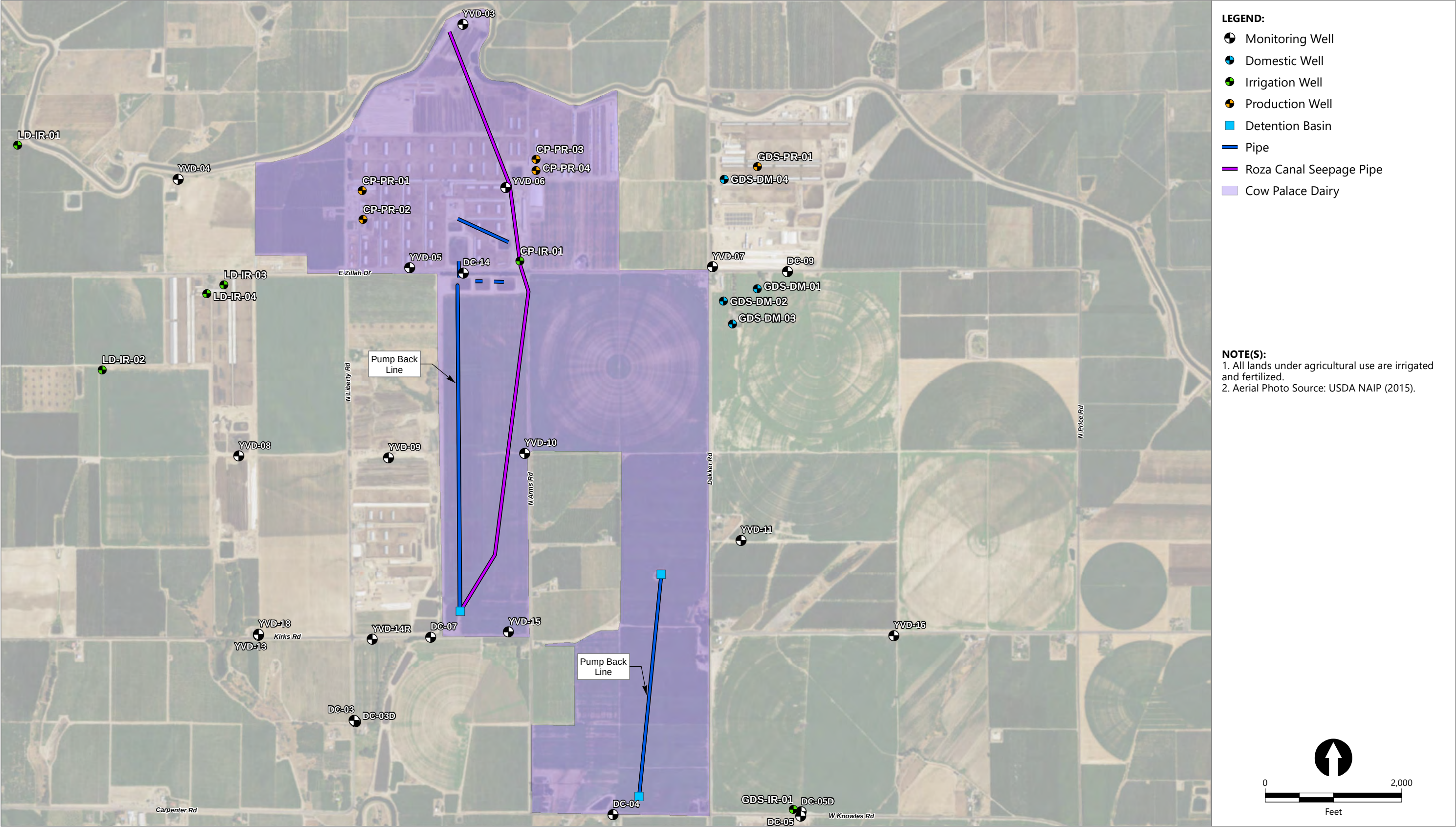
Figure 3B Facility Plan – Cow Palace Dairy Groundwater Monitoring Data Report – Third Quarter 2017 Yakima Valley Dairies
