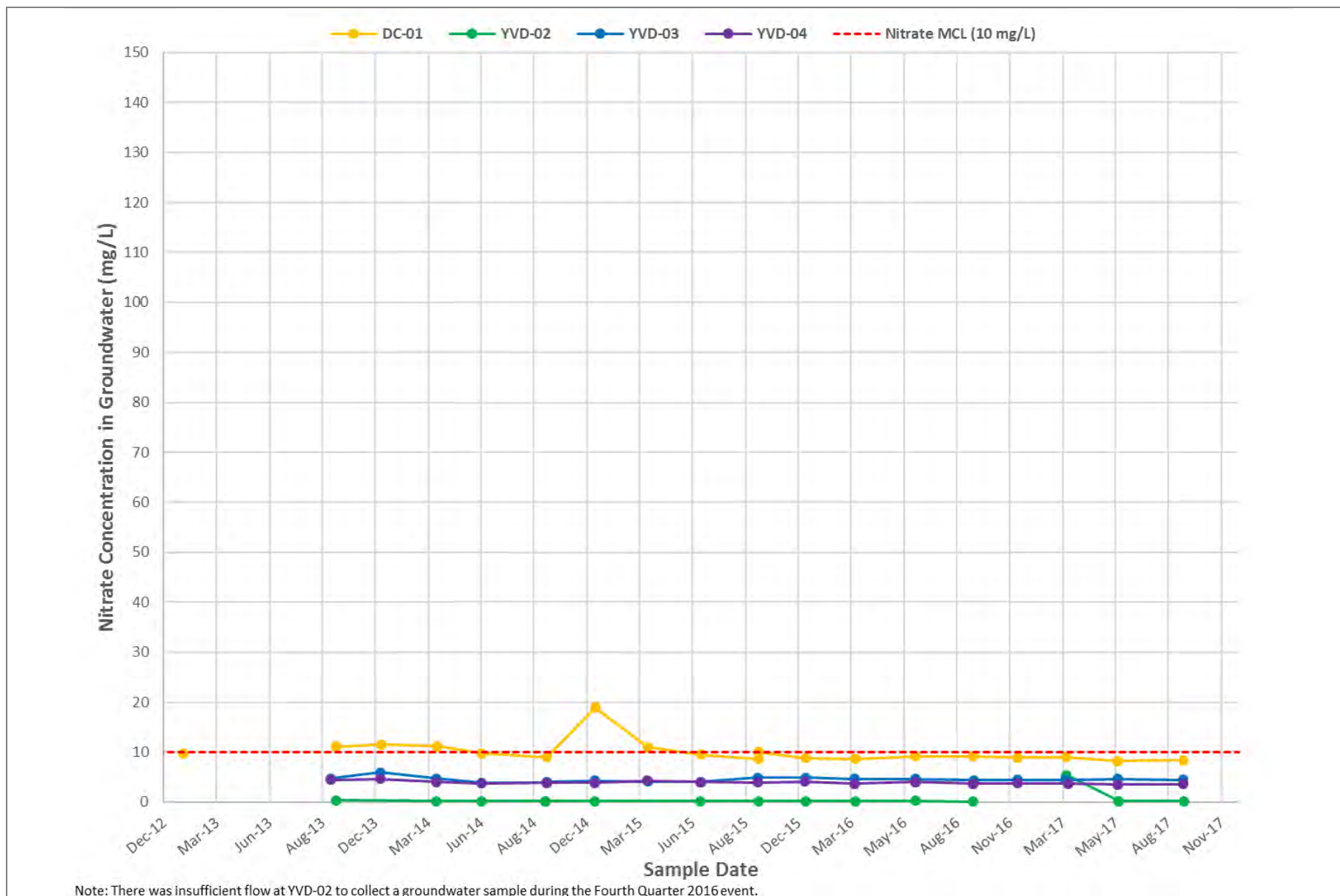
Figure 22 Nitrate Concentrations – Upgradient Wells Groundwater Monitoring Data Report – Third Quarter 2017 Yakima Valley Dairies
