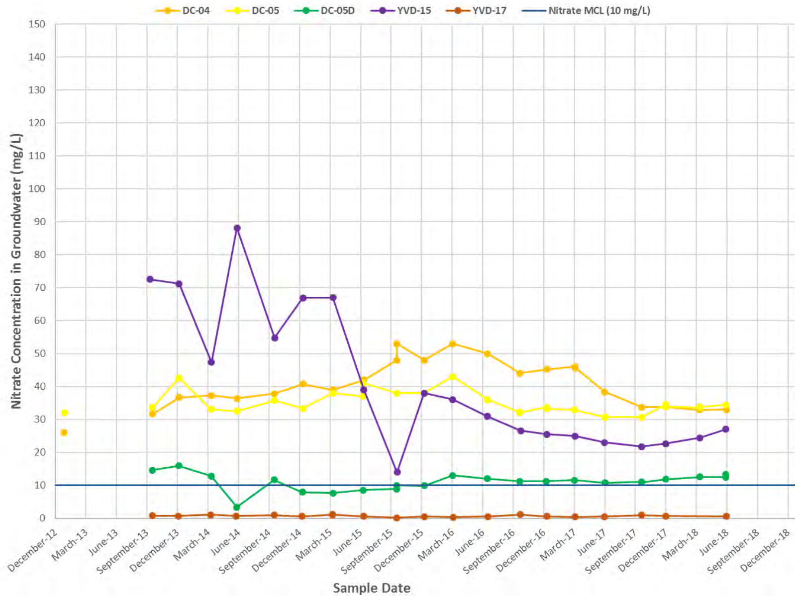
Figure 18 Nitrate Concentrations – East Downgradient Wells Groundwater Monitoring Data Report – Second Quarter 2018 Yakima Valley Dairies
