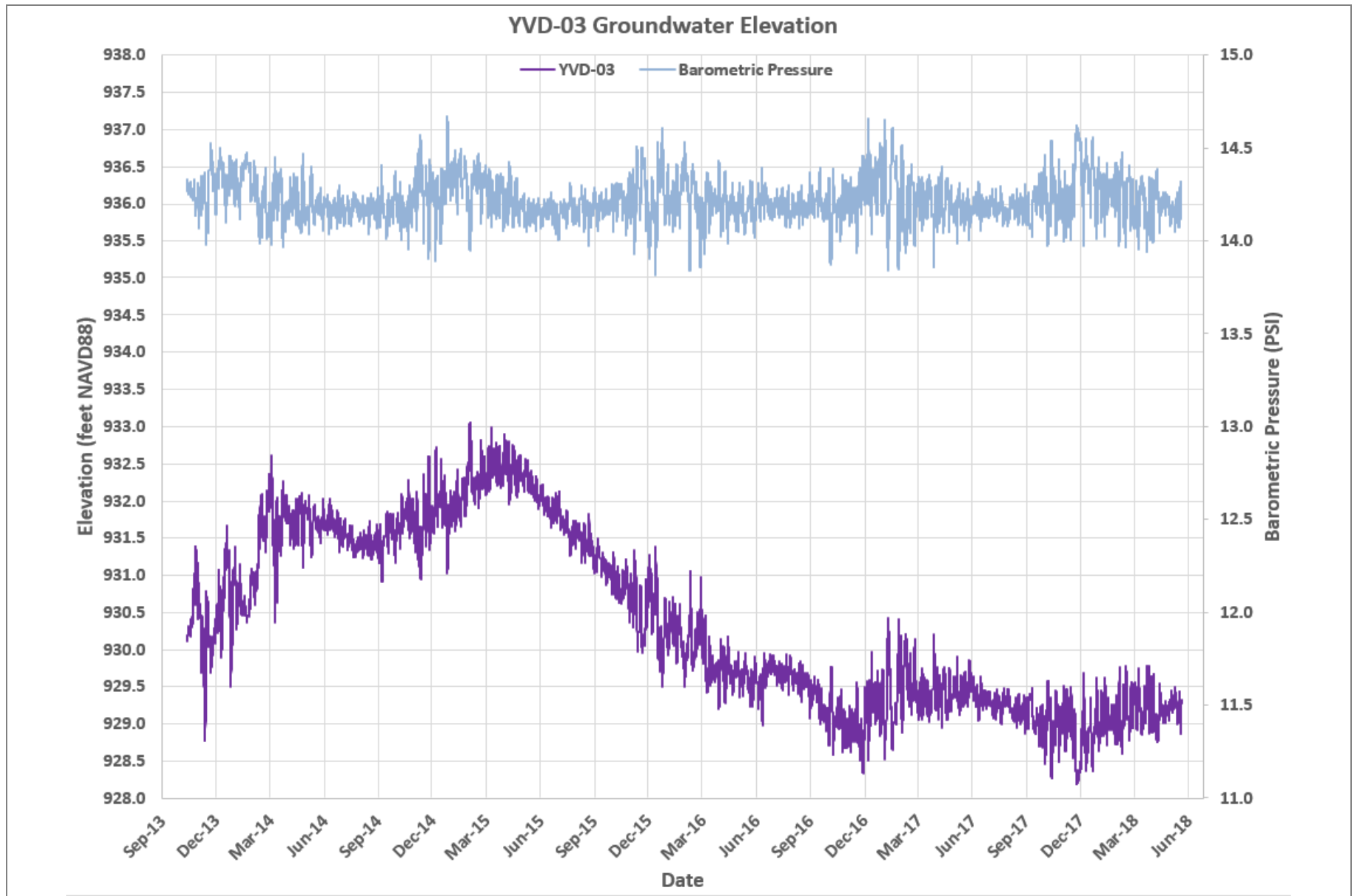
Figure 16E Groundwater Hydrographs – YVD-03 Groundwater Monitoring Data Report – Second Quarter 2018 Yakima Valley Dairies
