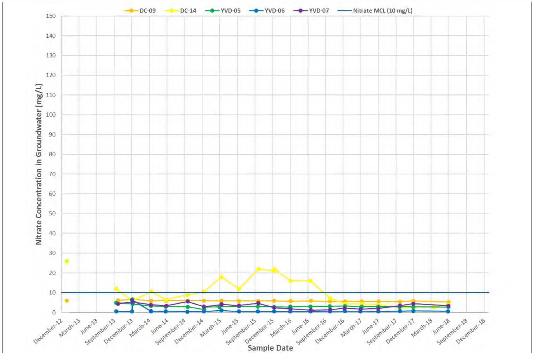
Figure 21 Nitrate Concentrations – Northern Wells Groundwater Monitoring Data Report – Second Quarter 2018 Yakima Valley Dairies
