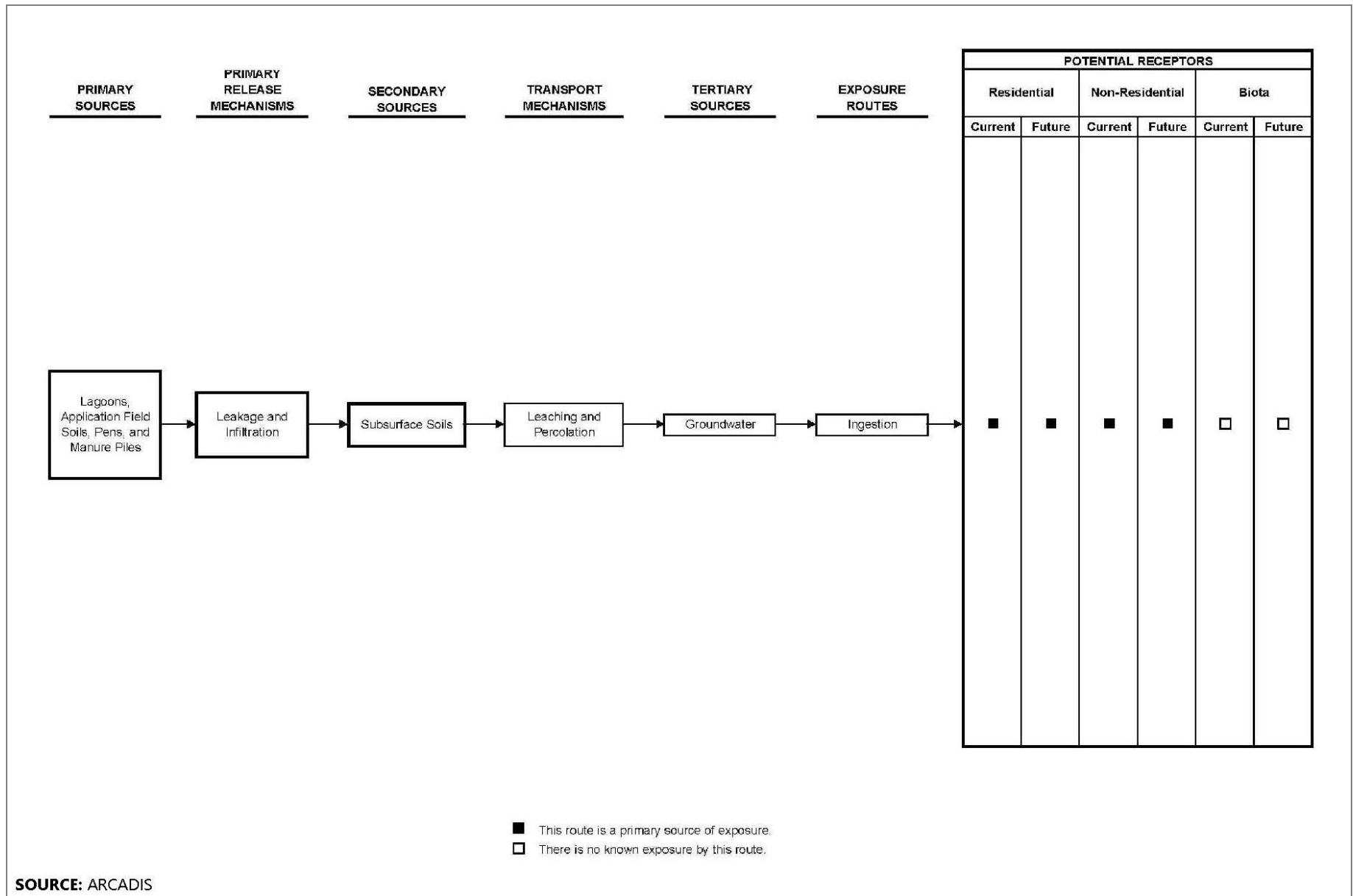
Figure 4 Conceptual Site Model Flow Chart Groundwater Monitoring Data Report – Second Quarter 2018 Yakima Valley Dairies
