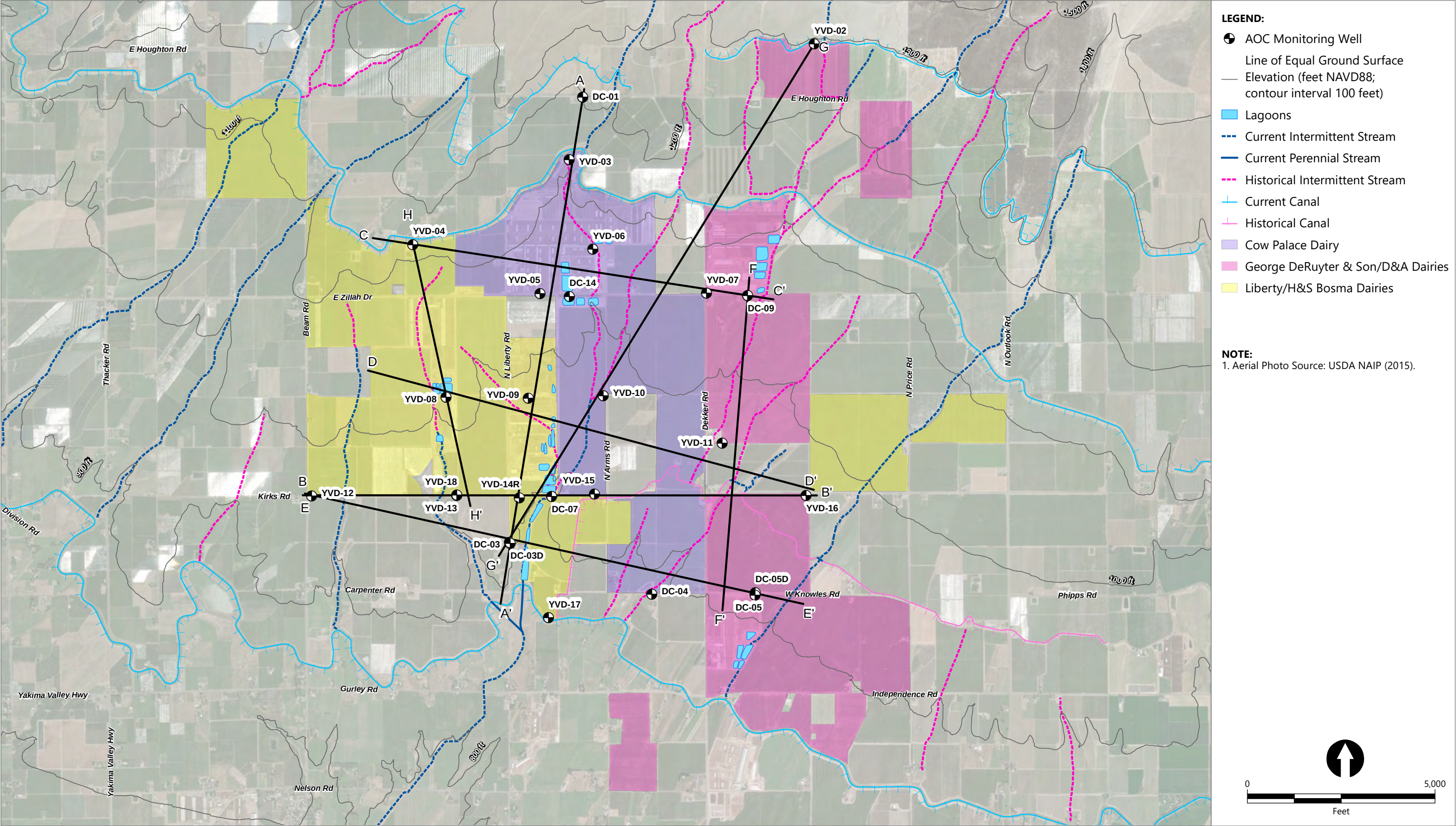
Figure 6 Cross Section Location Map Groundwater Monitoring Data Report – Second Quarter 2018 Yakima Valley Dairies
