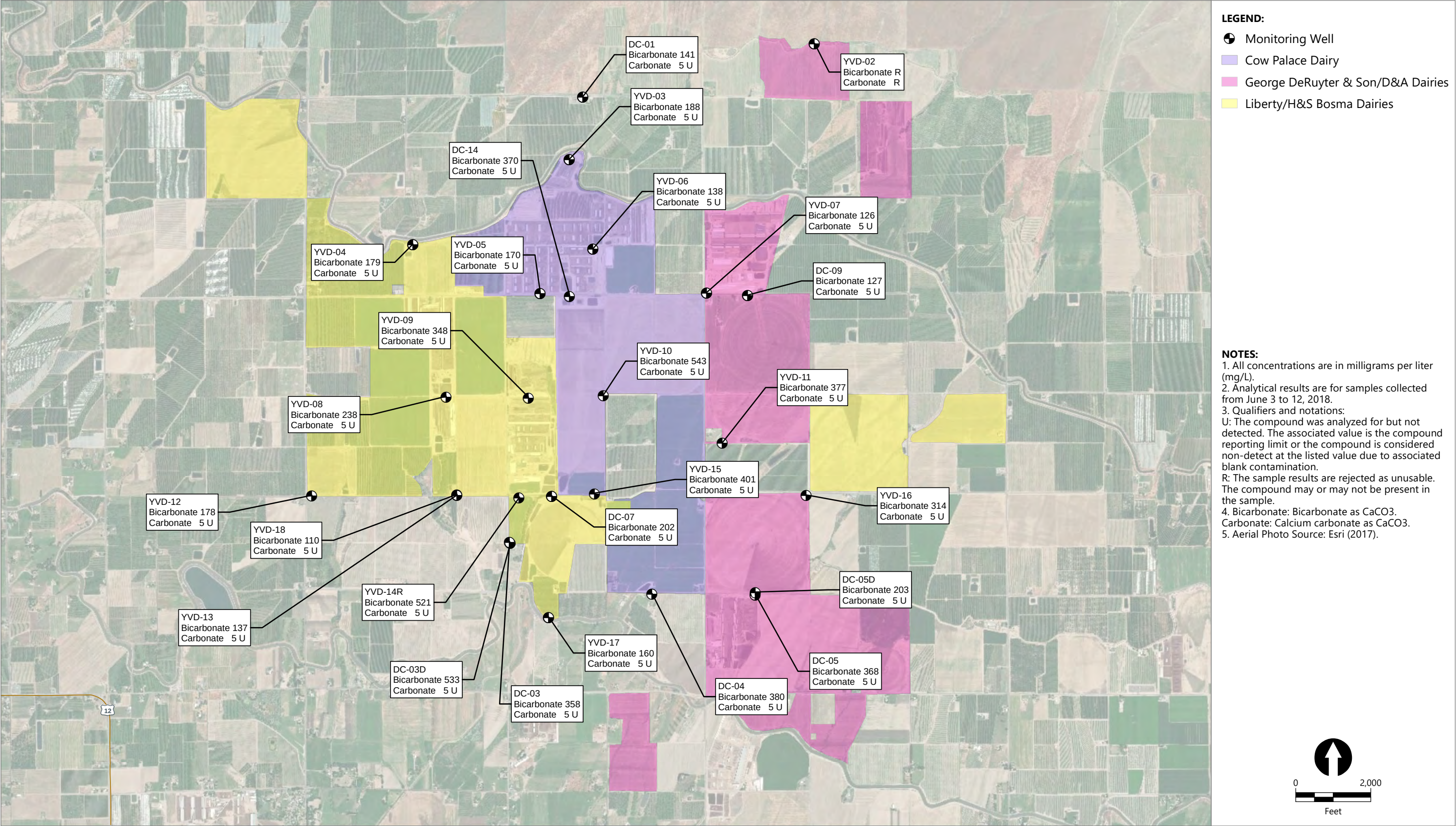
Figure 27 Alkalinity Concentrations in Groundwater Second Quarter 2018 Groundwater Monitoring Data Report – Second Quarter 2018 Yakima Valley Dairies
