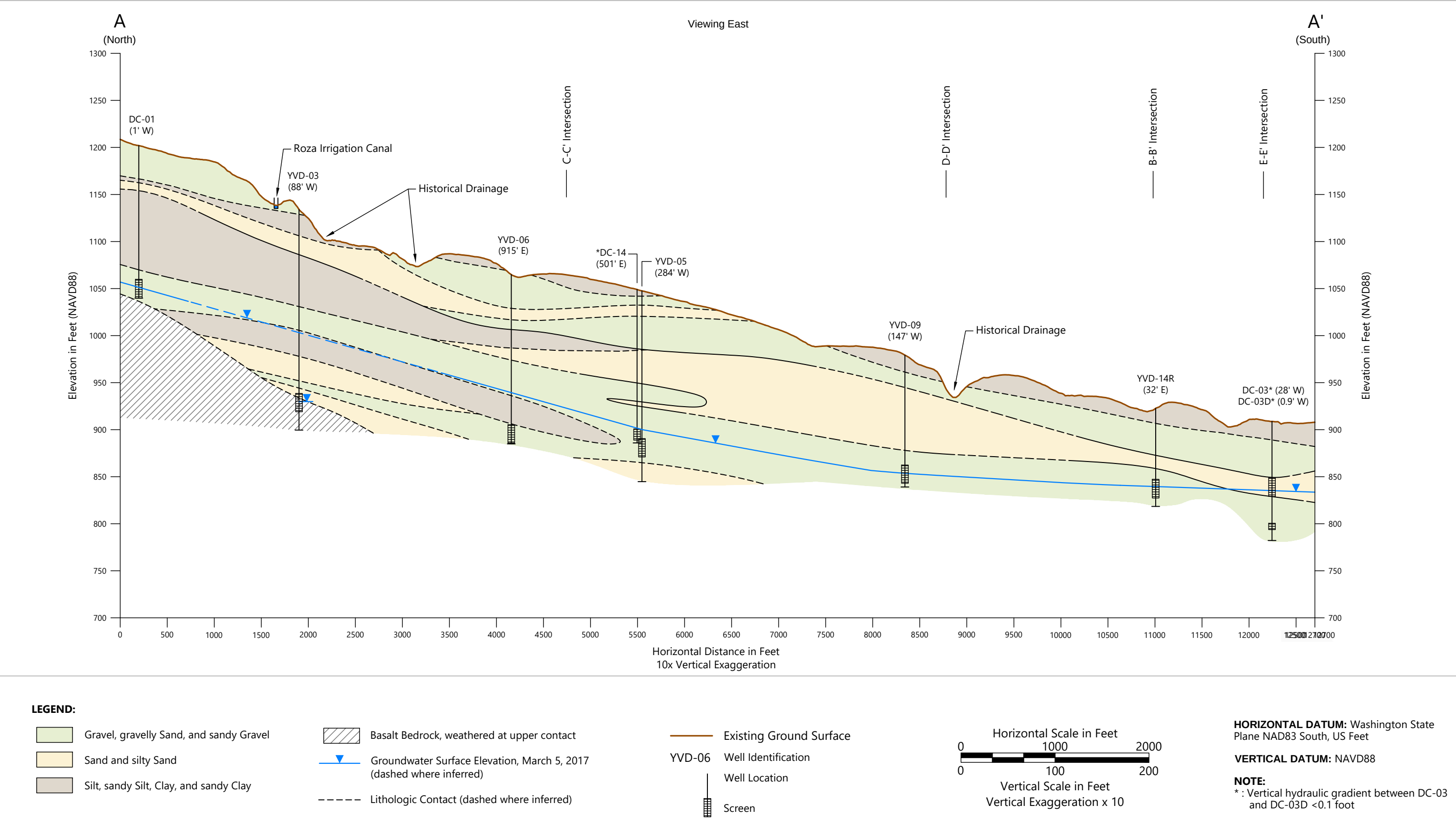
Figure 7 Geologic Cross Section A-A' Groundwater Monitoring Data Report – Second Quarter 2018 Yakima Valley Dairies
