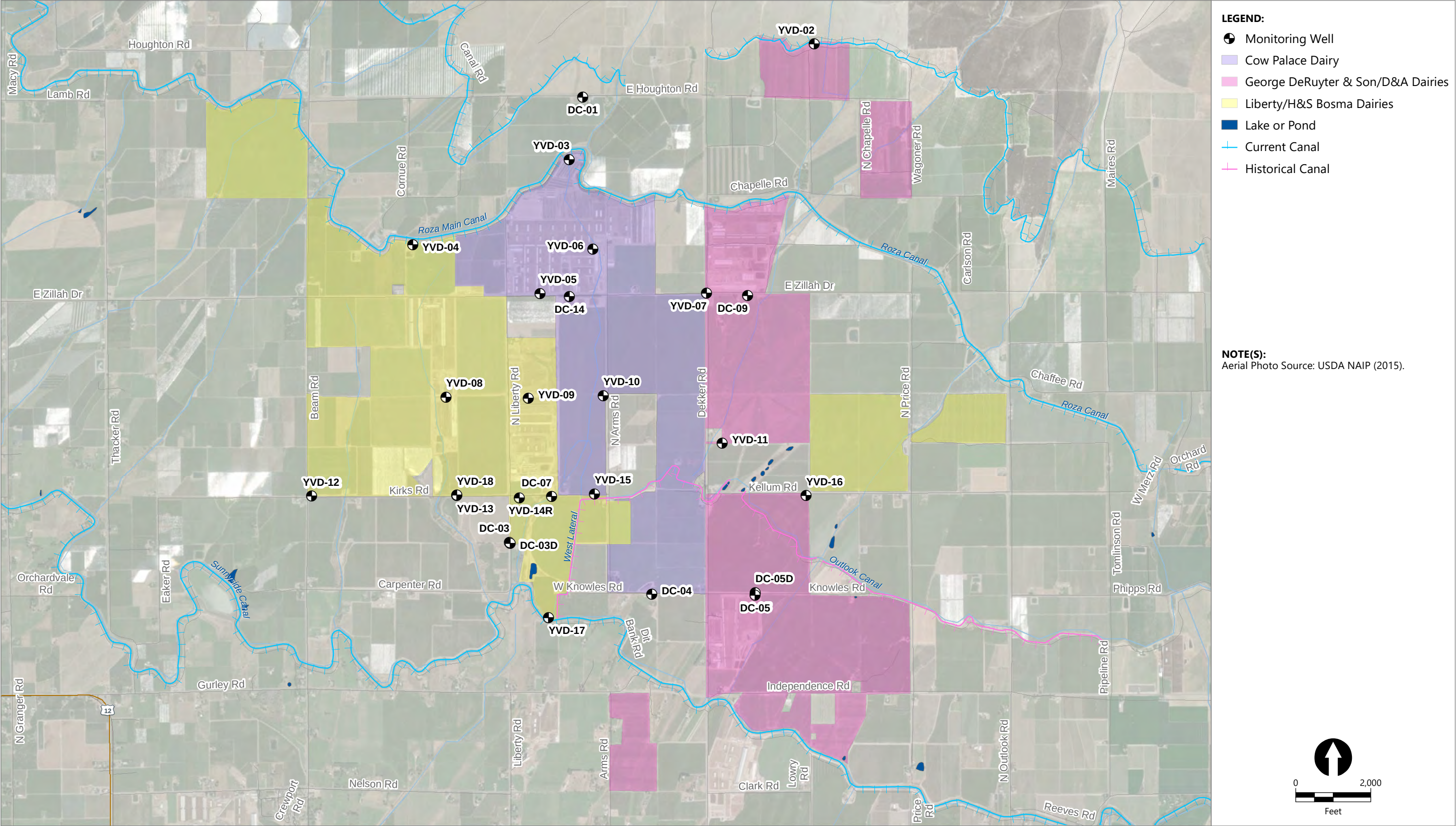
Figure 2B Aerial Photograph Groundwater Monitoring Data Report – Second Quarter 2018 Yakima Valley Dairies
