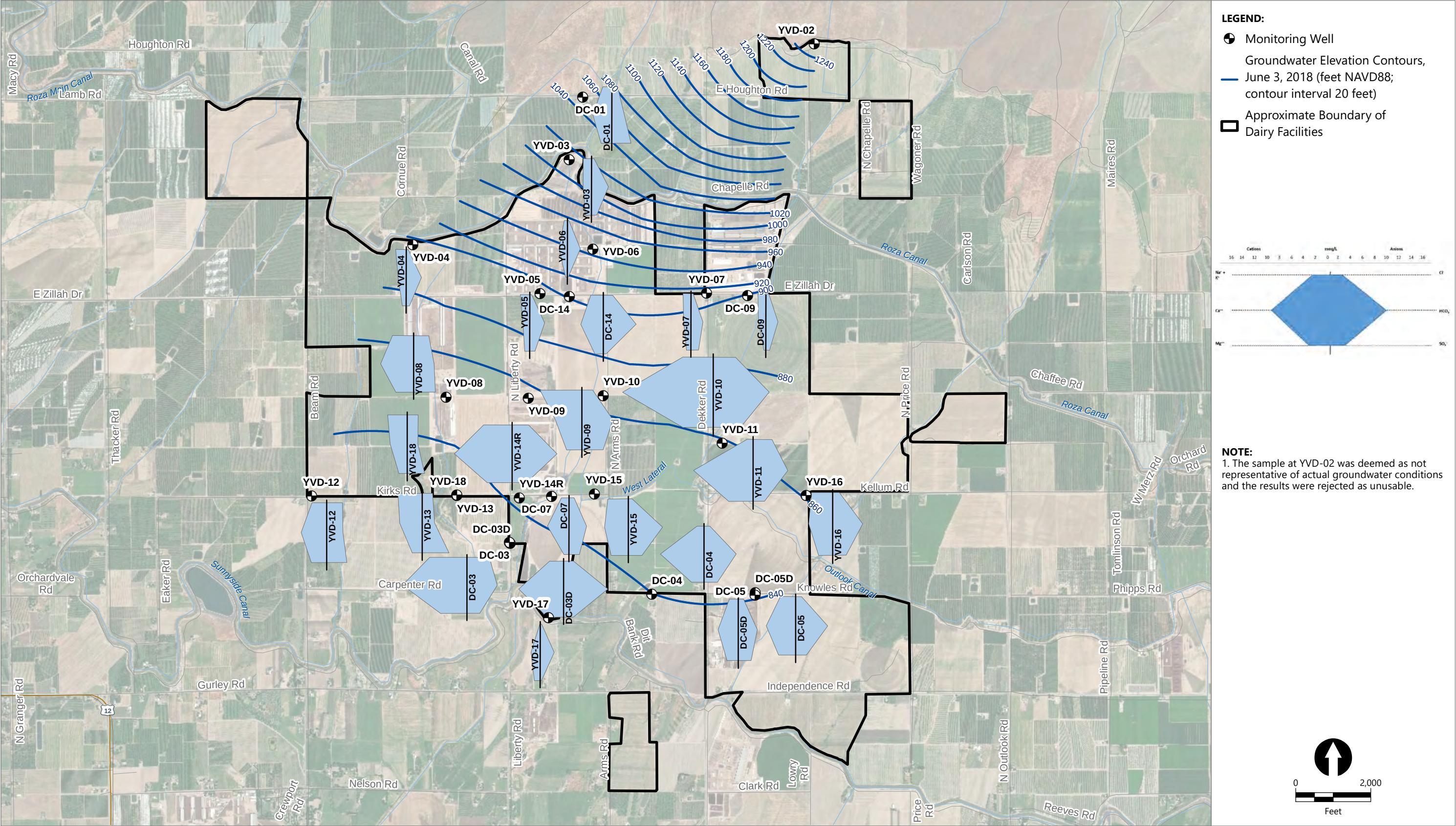
Figure 29 Stiff Diagrams and Groundwater Elevation Contour Map Groundwater Monitoring Data Report – Second Quarter 2018 Yakima Valley Dairies
