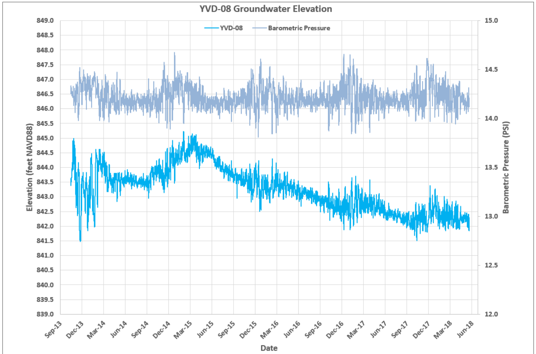
Figure 16F Groundwater Hydrographs – YVD-08 Groundwater Monitoring Data Report – Second Quarter 2018 Yakima Valley Dairies
