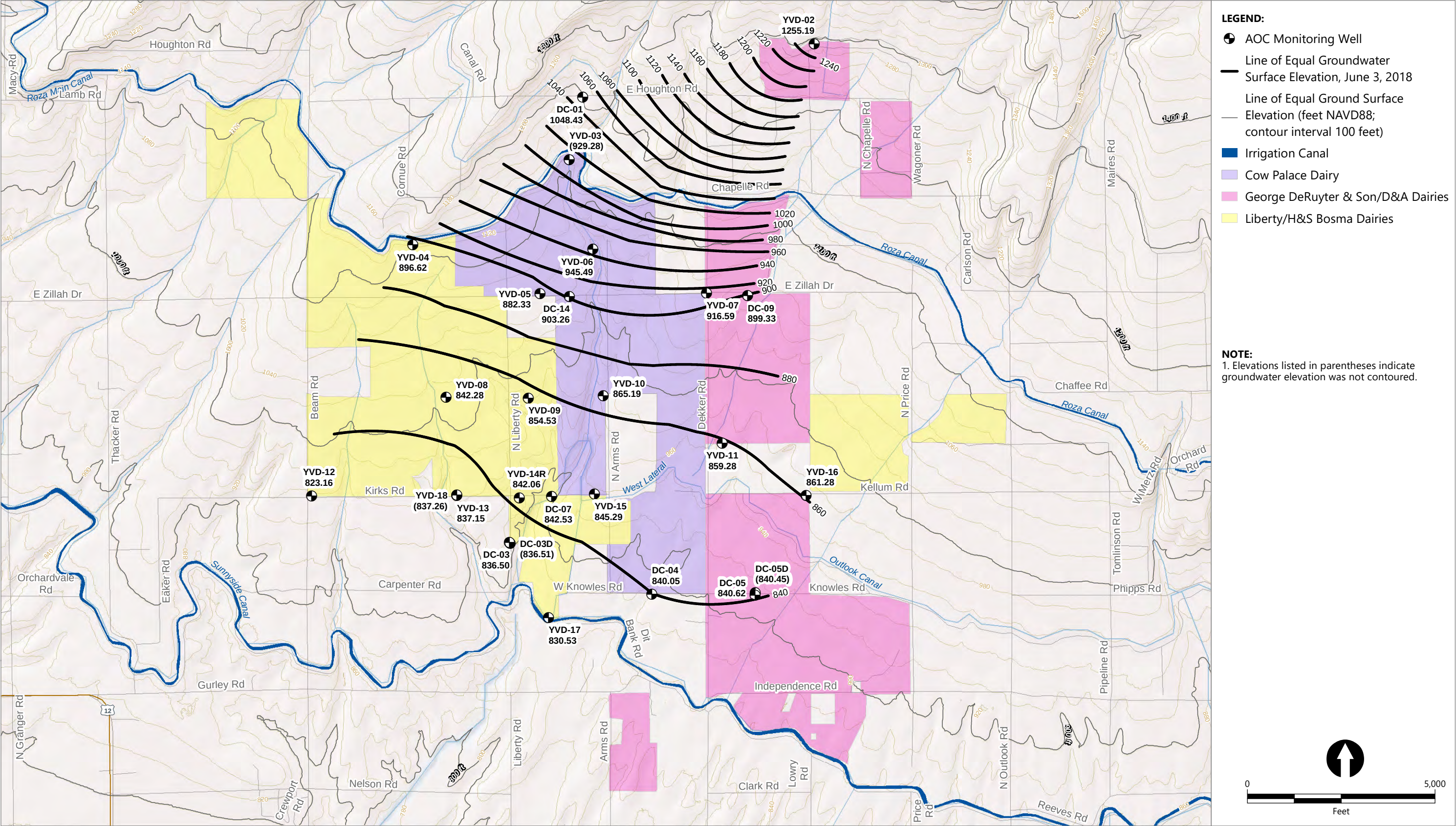
Figure 15 Surficial Aquifer Groundwater Elevation Contour Map Second Quarter 2018 Groundwater Monitoring Data Report – Second Quarter 2018 Yakima Valley Dairies
