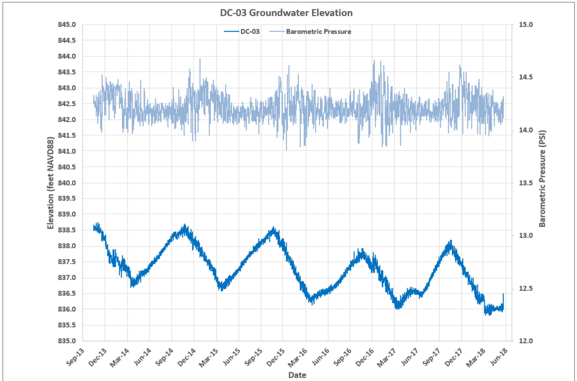
Figure 16B Groundwater Hydrographs – DC-03 Groundwater Monitoring Data Report – Second Quarter 2018 Yakima Valley Dairies
