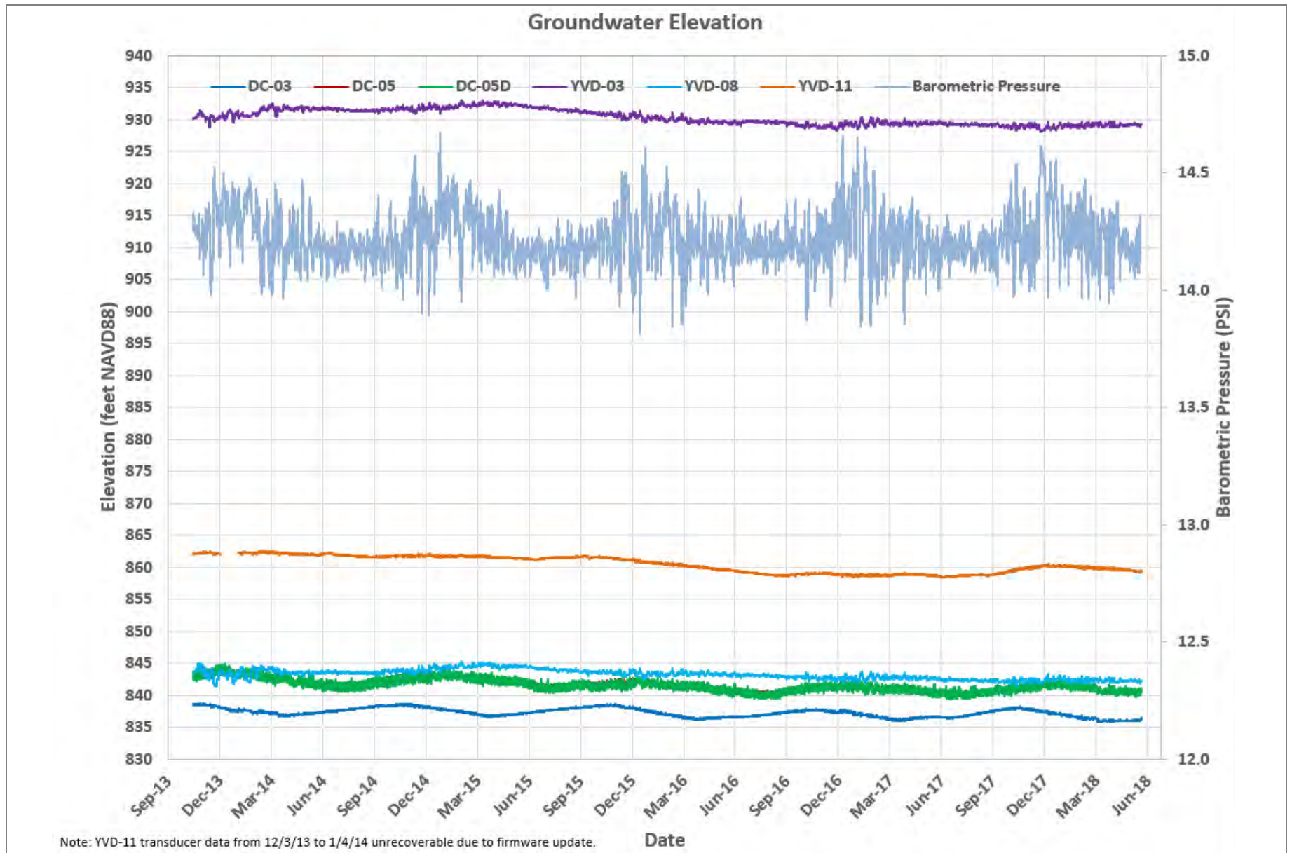
Figure 16A Groundwater Hydrographs – All Transducers Groundwater Monitoring Data Report – Second Quarter 2018 Yakima Valley Dairies
