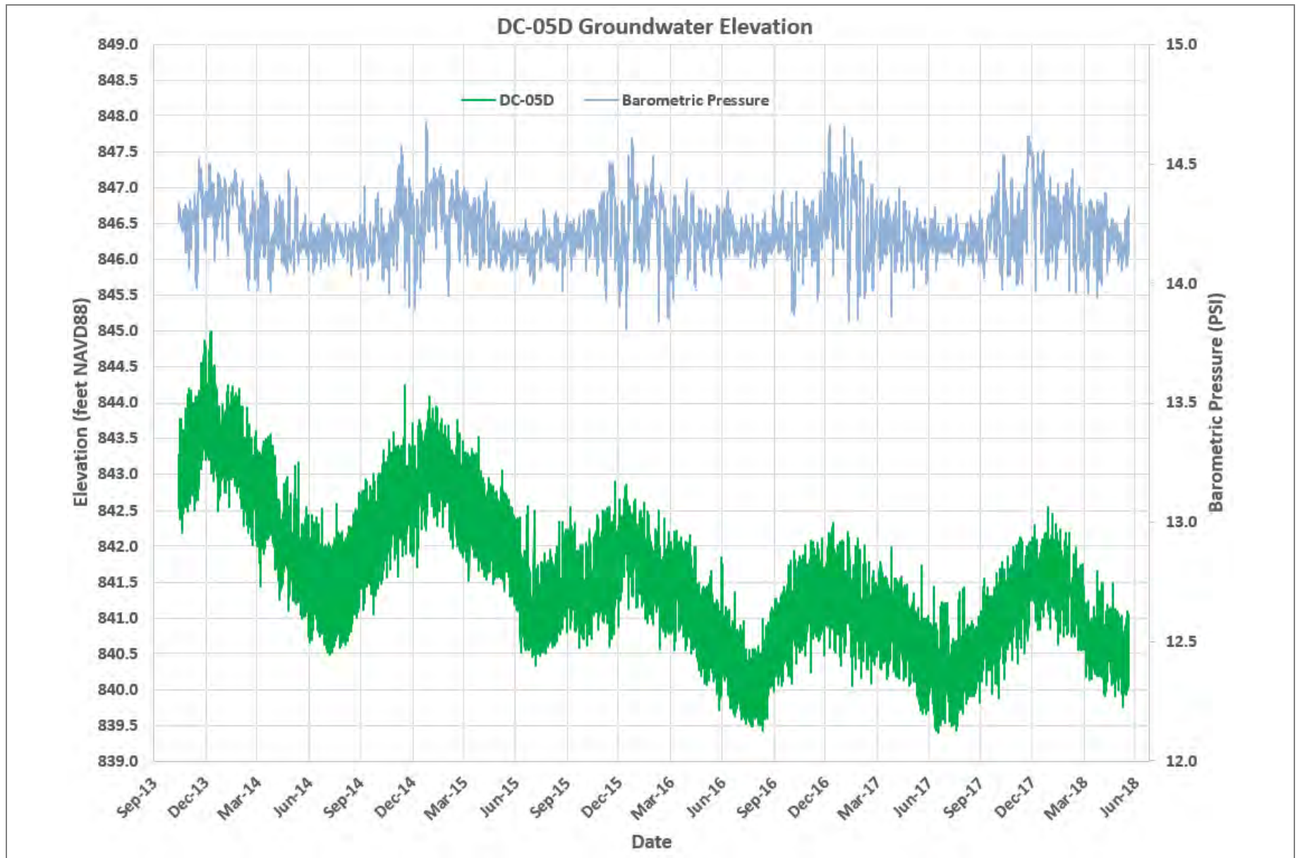
Figure 16D Groundwater Hydrographs – DC-05D Groundwater Monitoring Data Report – Second Quarter 2018 Yakima Valley Dairies
