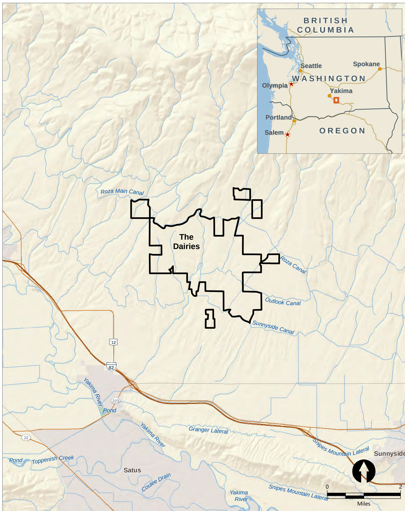
Figure 1 Site Vicinity Map Groundwater Monitoring Data Report – Second Quarter 2018 Yakima Valley Dairies
