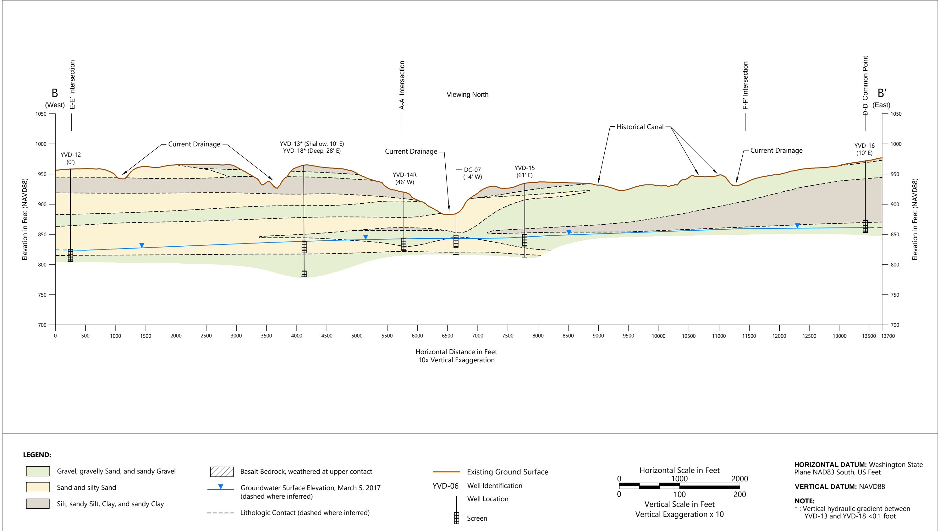
Figure 8 Geologic Cross Section B-B' Groundwater Monitoring Data Report – Second Quarter 2018 Yakima Valley Dairies
