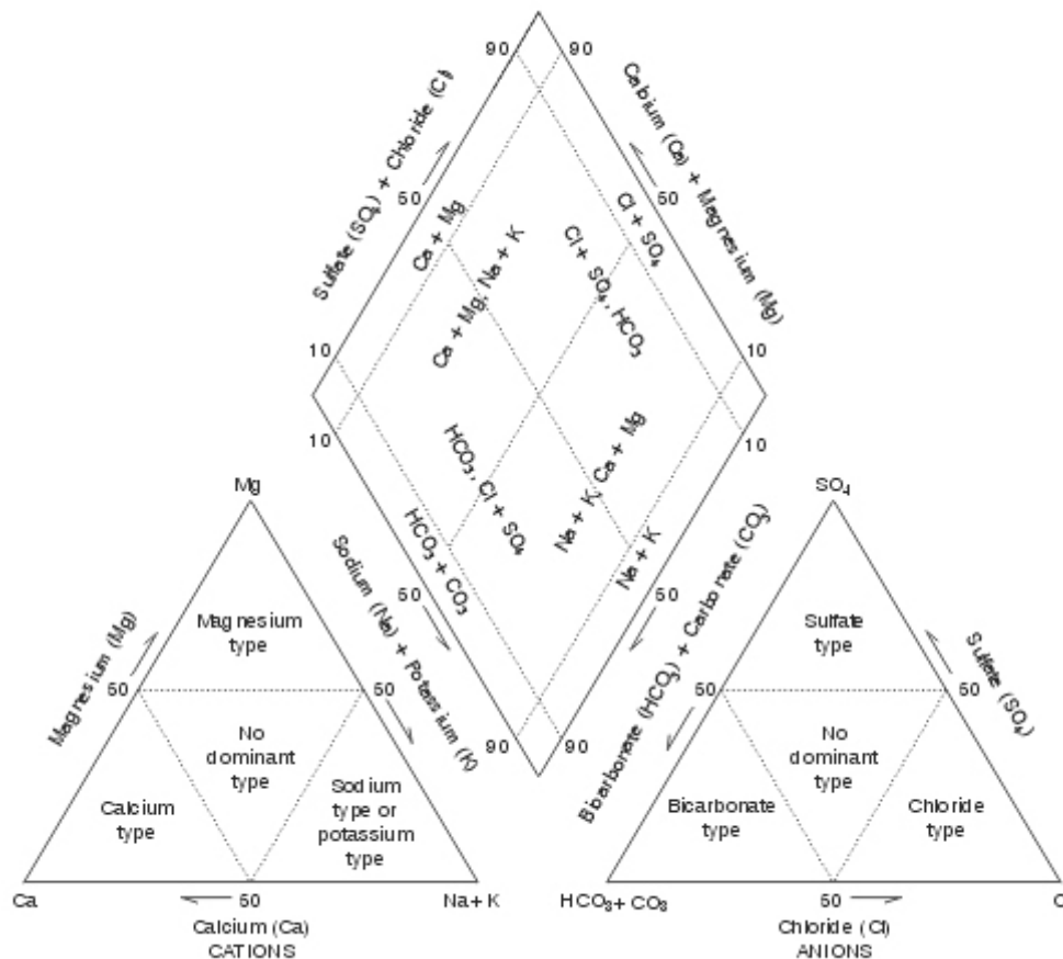
Chart 1 Piper Diagram Displaying Relative Ion Composition (Bartos and Ogle 2002)
