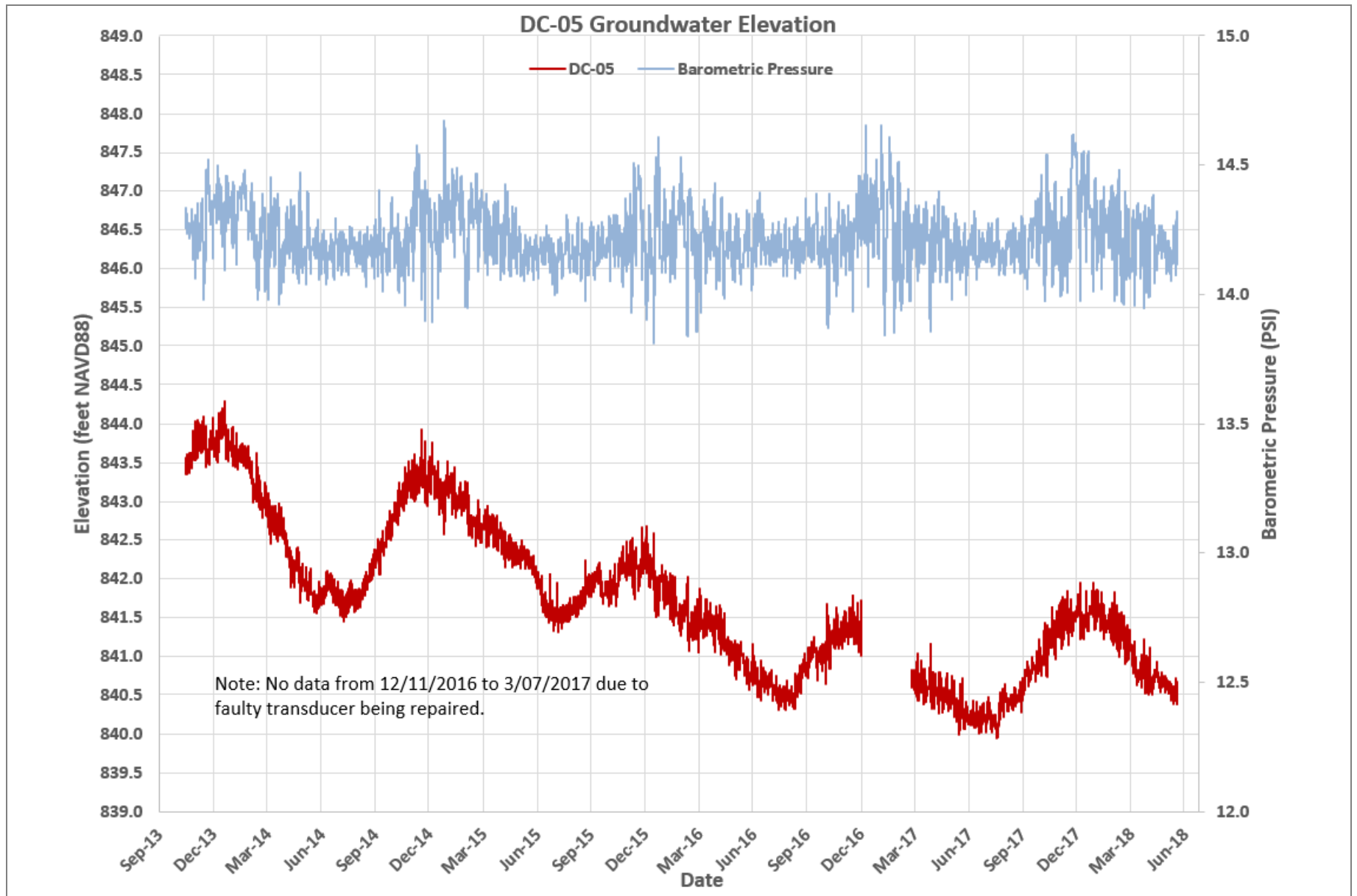
Figure 16C Groundwater Hydrographs – DC-05 Groundwater Monitoring Data Report – Second Quarter 2018 Yakima Valley Dairies
