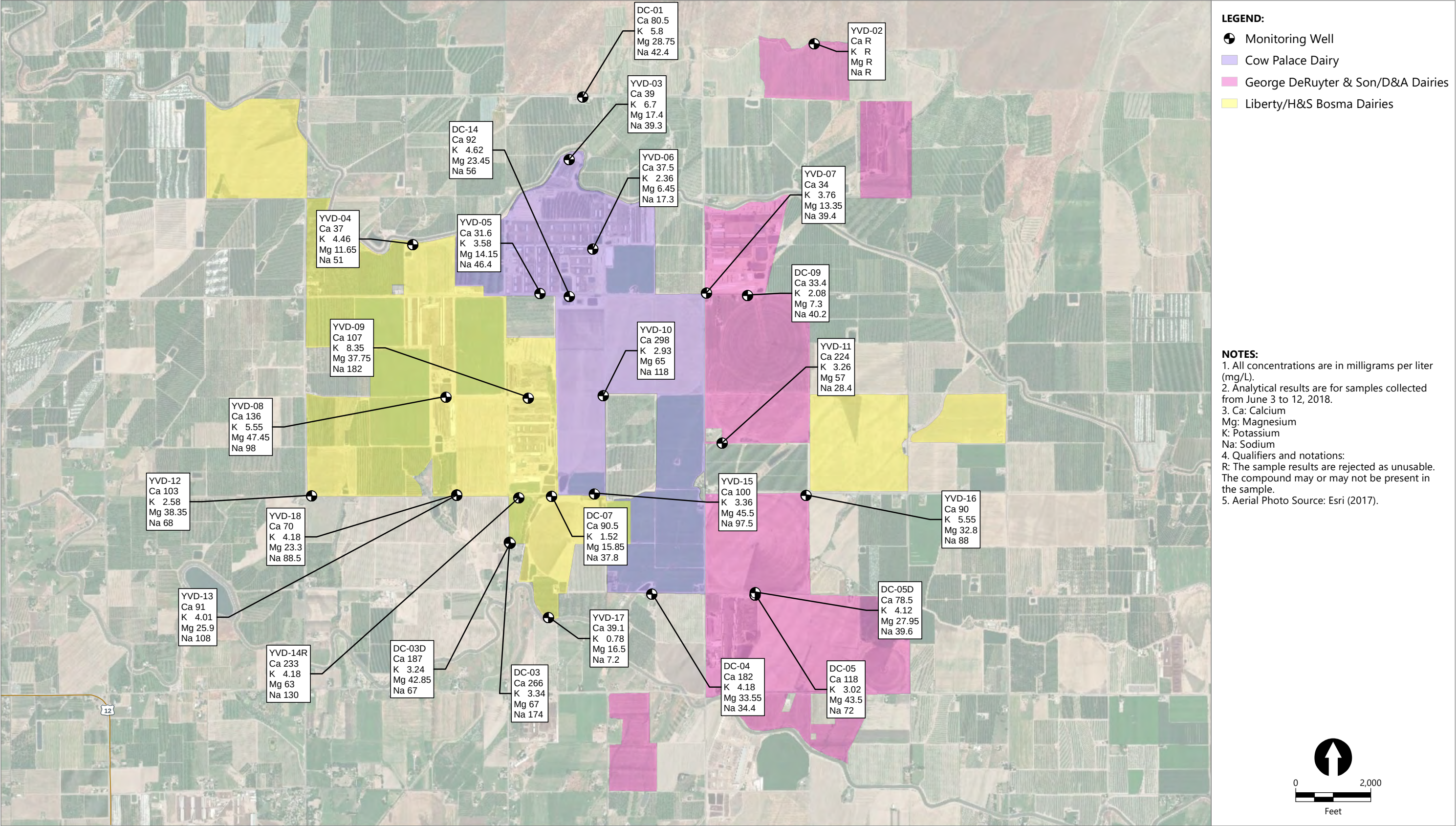
Figure 26 Metals Concentrations in Groundwater Second Quarter 2018 Groundwater Monitoring Data Report – Second Quarter 2018 Yakima Valley Dairies
