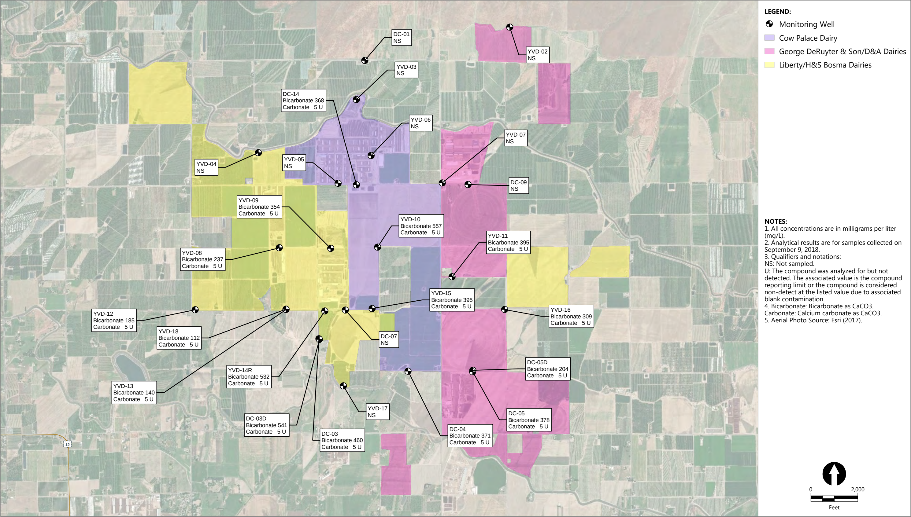
Figure 5 Alkalinity Concentrations in Groundwater Third Quarter 2018 Groundwater Monitoring Data Report – Third Quarter 2018 Yakima Valley Dairies
