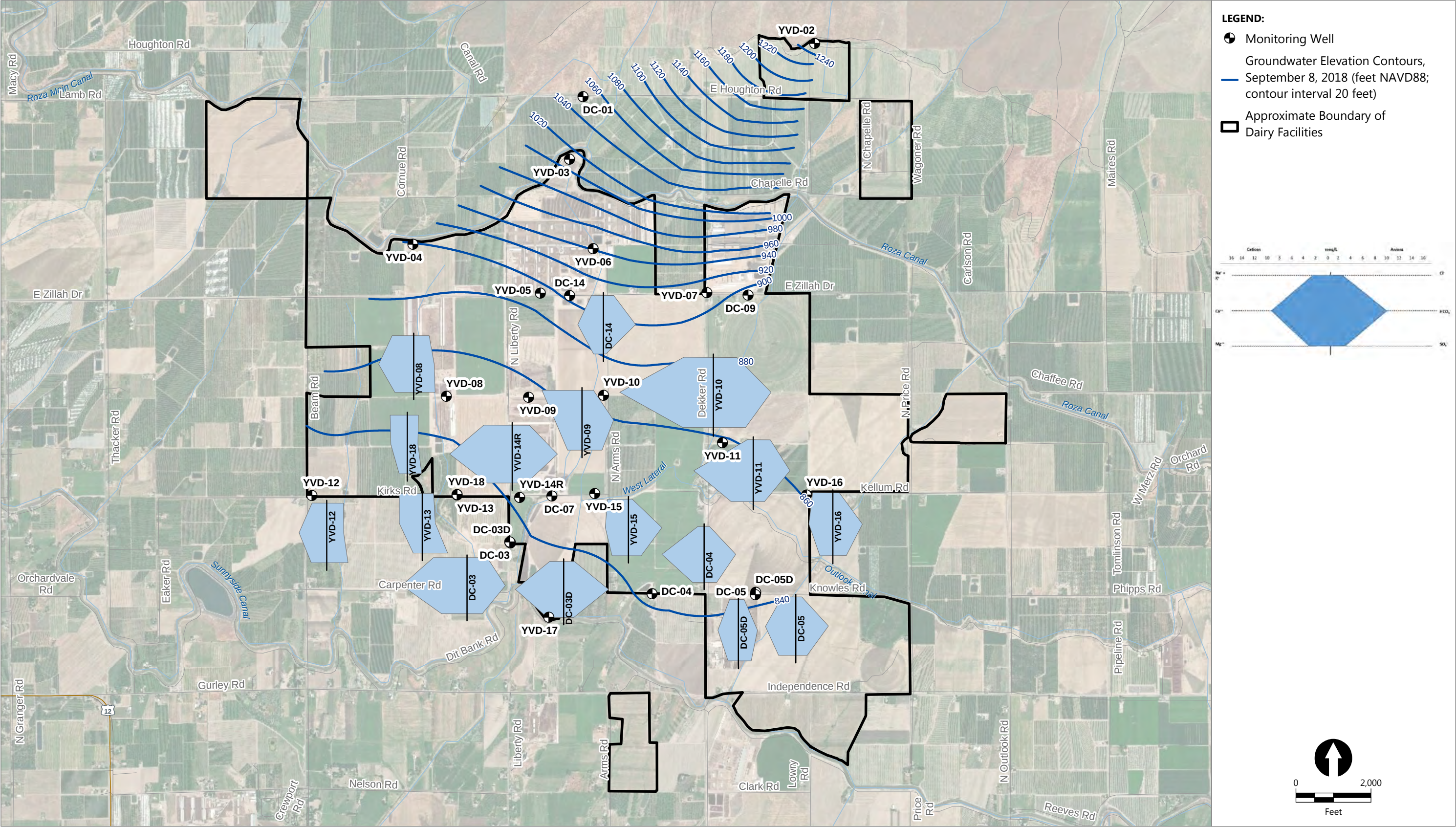
Figure 13 Stiff Diagrams and Groundwater Elevation Contour Map Groundwater Monitoring Data Report – Third Quarter 2018 Yakima Valley Dairies
