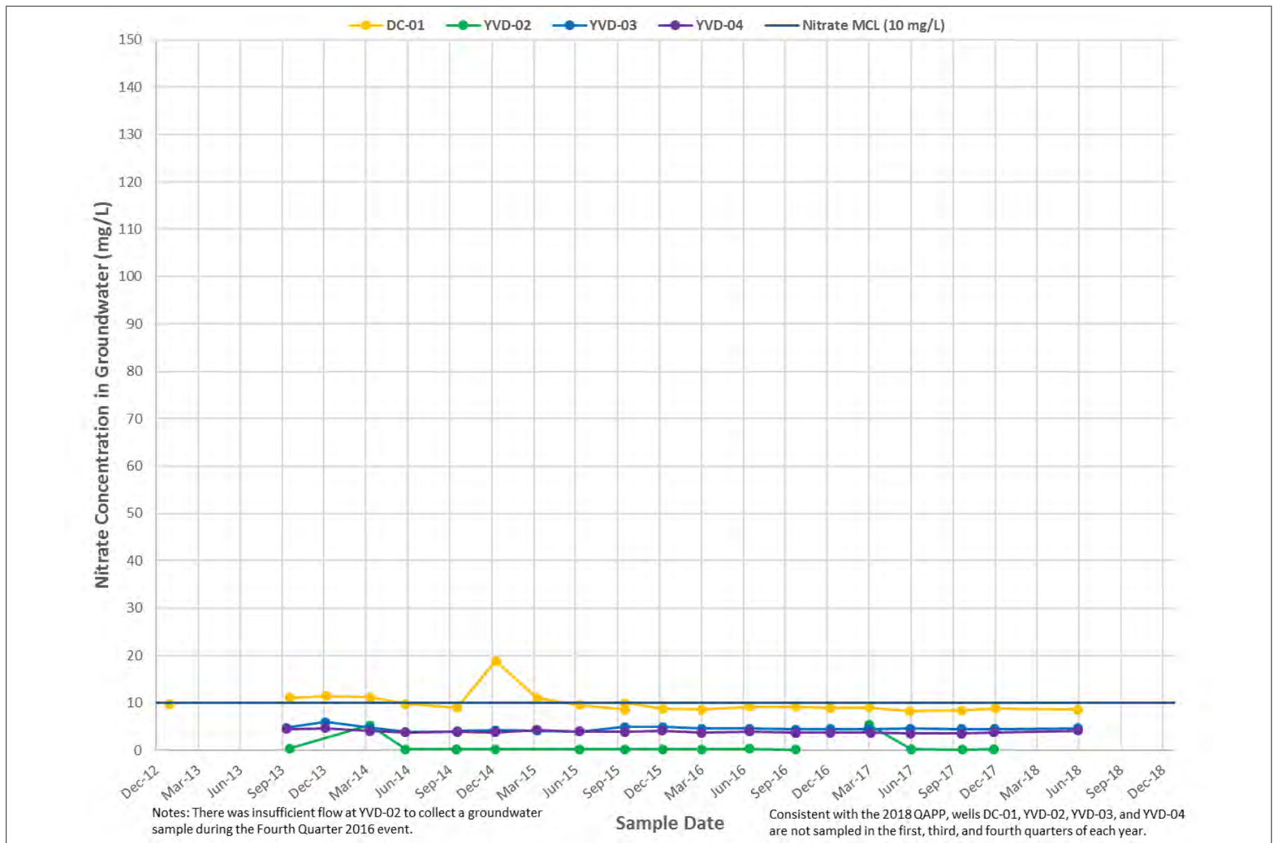
Figure 11 Nitrate Concentrations – Upgradient Wells Groundwater Monitoring Data Report – Third Quarter 2018 Yakima Valley Dairies
