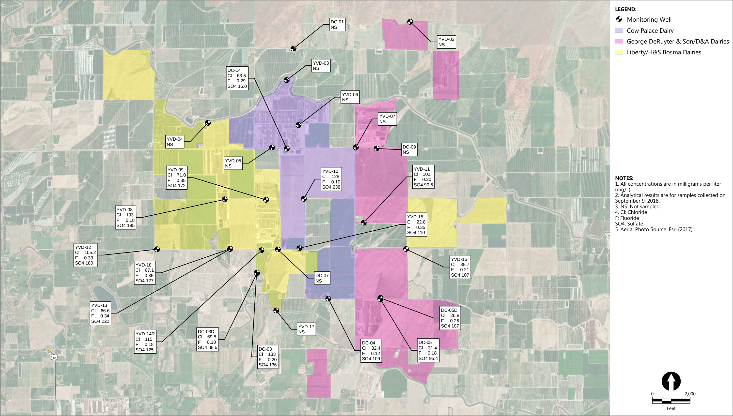
Figure 3 Anion Concentrations in Groundwater Third Quarter 2018 Groundwater Monitoring Data Report – Third Quarter 2018 Yakima Valley Dairies
