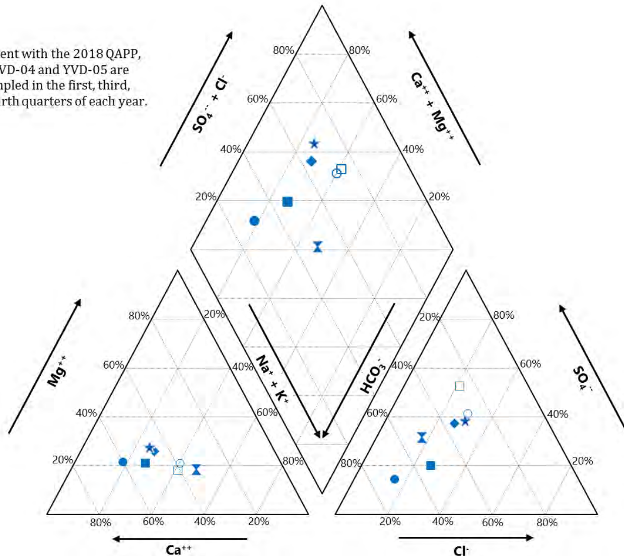
Figure 16 Piper Diagram – Group 1 Wells Groundwater Monitoring Data Report – Third Quarter 2018 Yakima Valley Dairies
