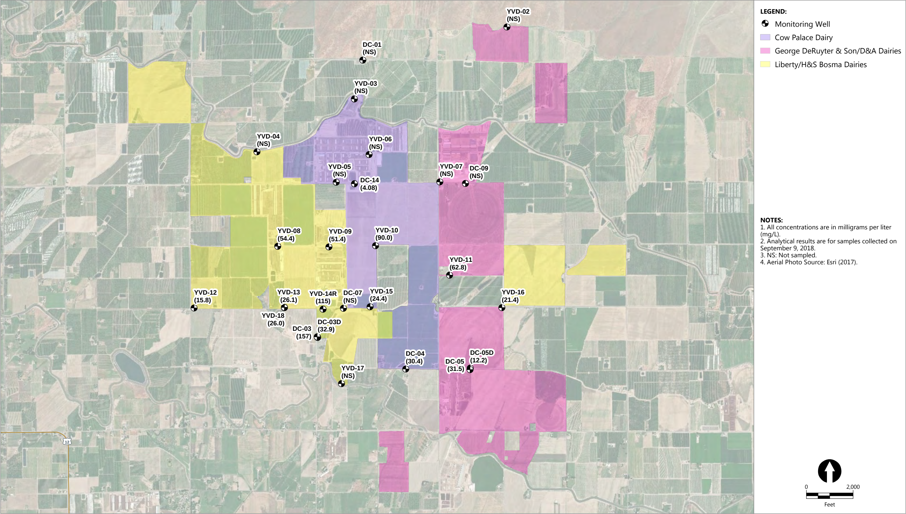
Figure 6A Nitrate Concentrations in Groundwater Third Quarter 2018 Groundwater Monitoring Data Report – Third Quarter 2018 Yakima Valley Dairies
