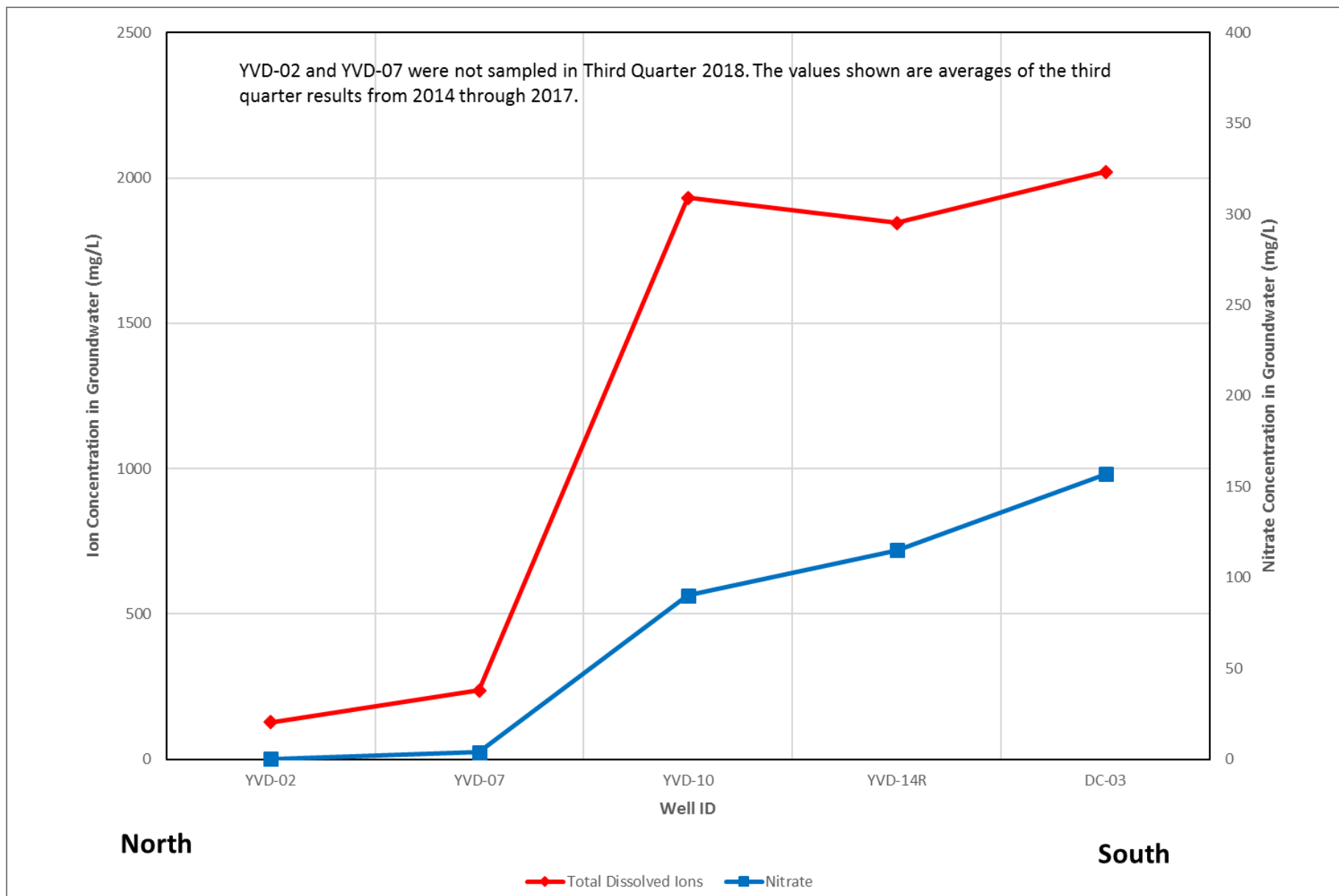
Figure 14 Nitrate and Total Dissolved Ion Concentration Along North-South Transect Groundwater Monitoring Data Report – Third Quarter 2018 Yakima Valley Dairies
