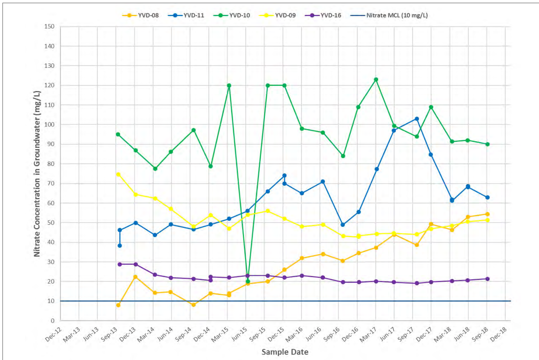
Figure 9 Nitrate Concentrations – Central Wells Groundwater Monitoring Data Report – Third Quarter 2018 Yakima Valley Dairies
