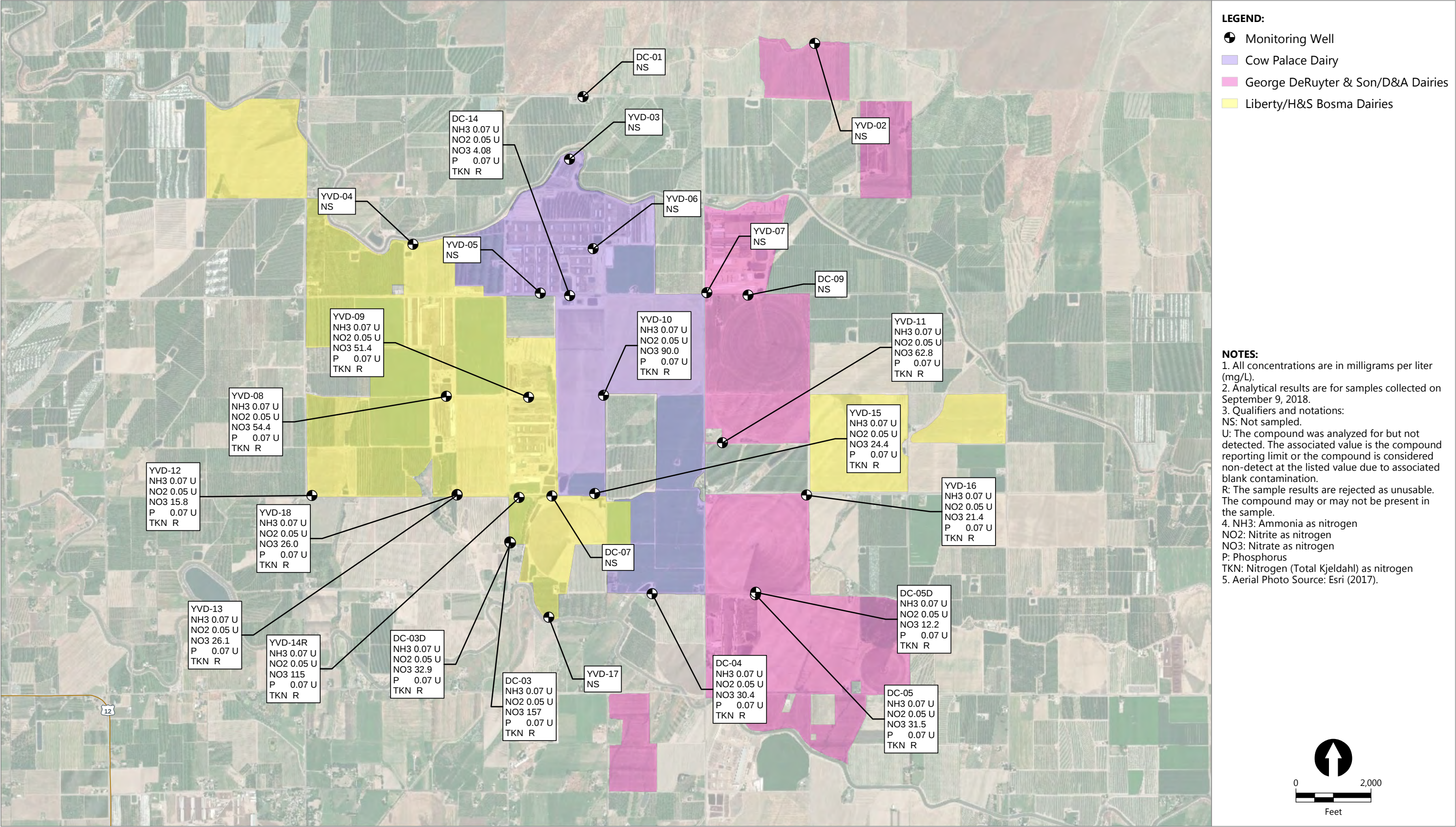
Figure 2 Nutrient Concentrations in Groundwater Third Quarter 2018 Groundwater Monitoring Data Report – Third Quarter 2018 Yakima Valley Dairies
