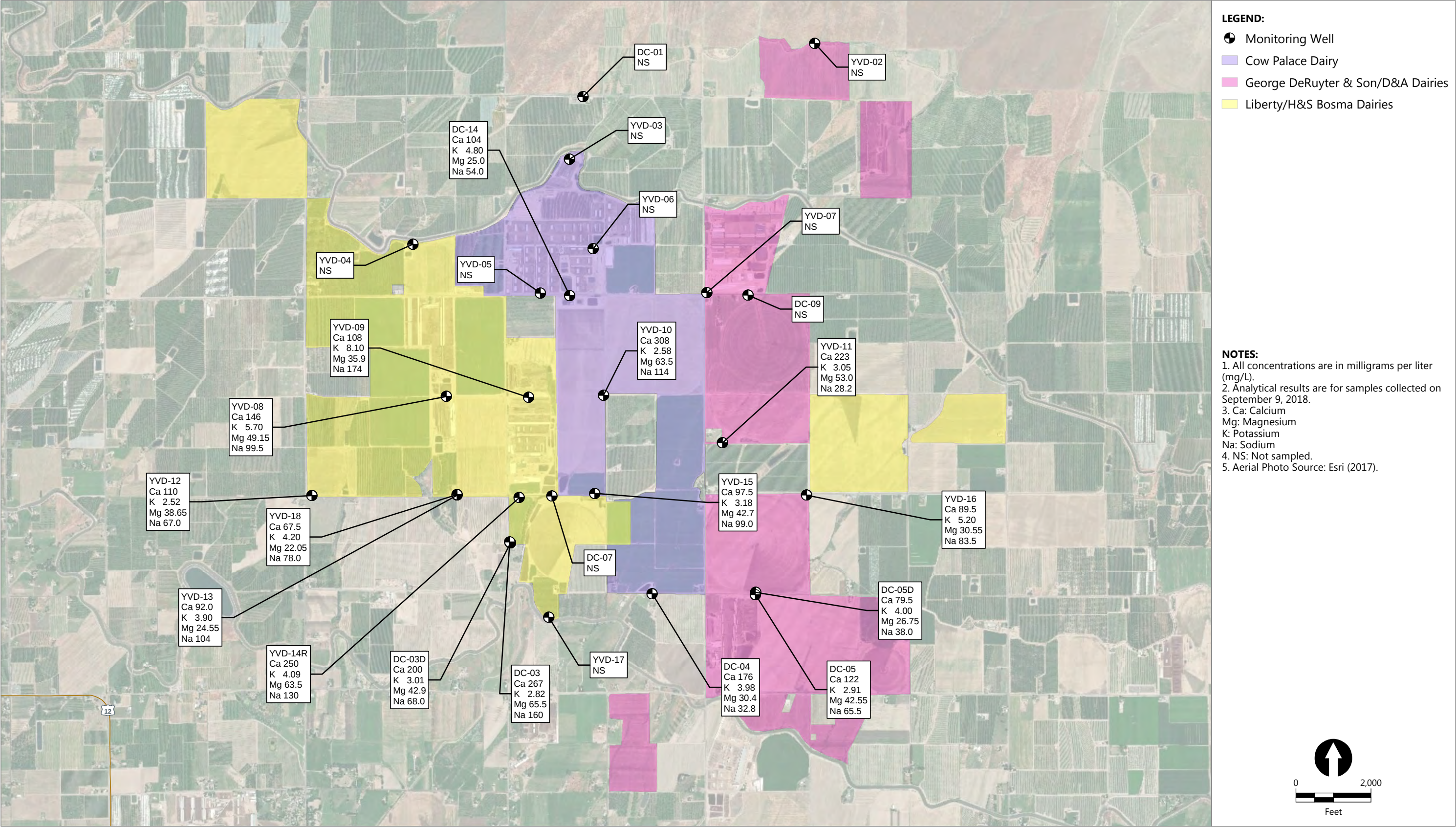
Figure 4 Metals Concentrations in Groundwater Third Quarter 2018 Groundwater Monitoring Data Report – Third Quarter 2018 Yakima Valley Dairies
