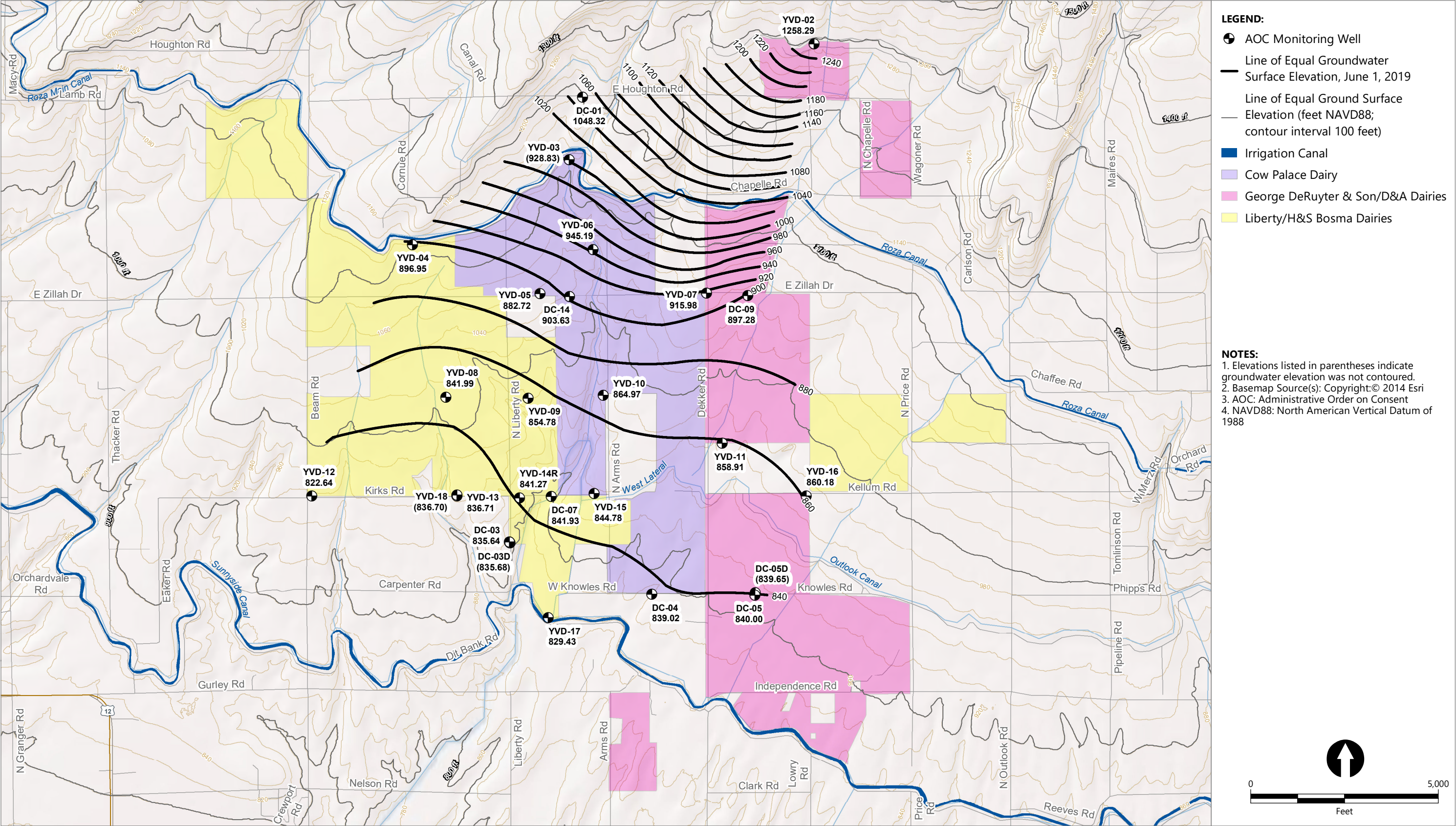
Figure 1 Surficial Aquifer Groundwater Elevation Contour Map Second Quarter 2019 Groundwater Monitoring Data Report – Second Quarter 2019 Yakima Valley Dairies
