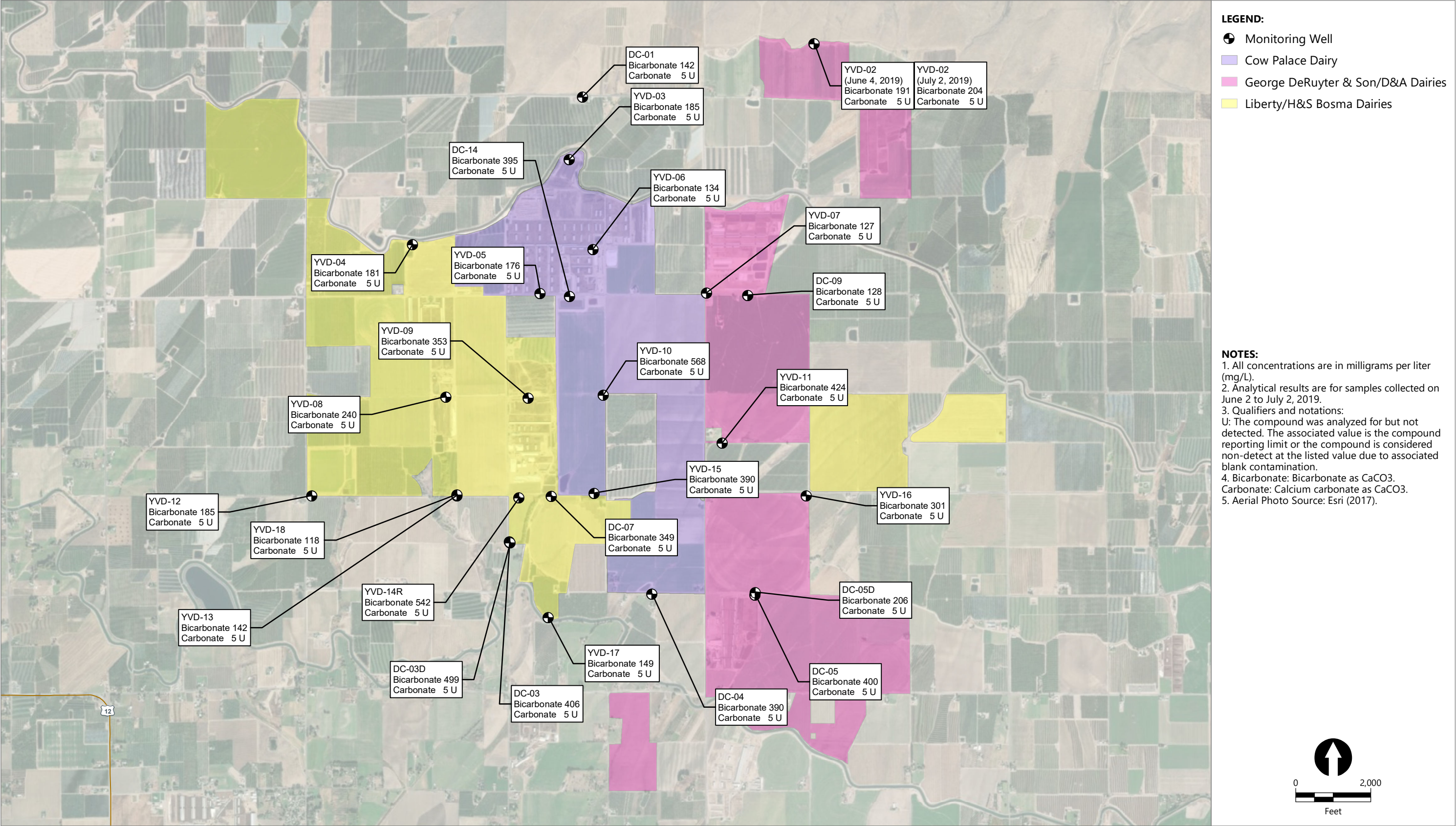
Figure 5 Alkalinity Concentrations in Groundwater Second Quarter 2019 Groundwater Monitoring Data Report – Second Quarter 2019 Yakima Valley Dairies
