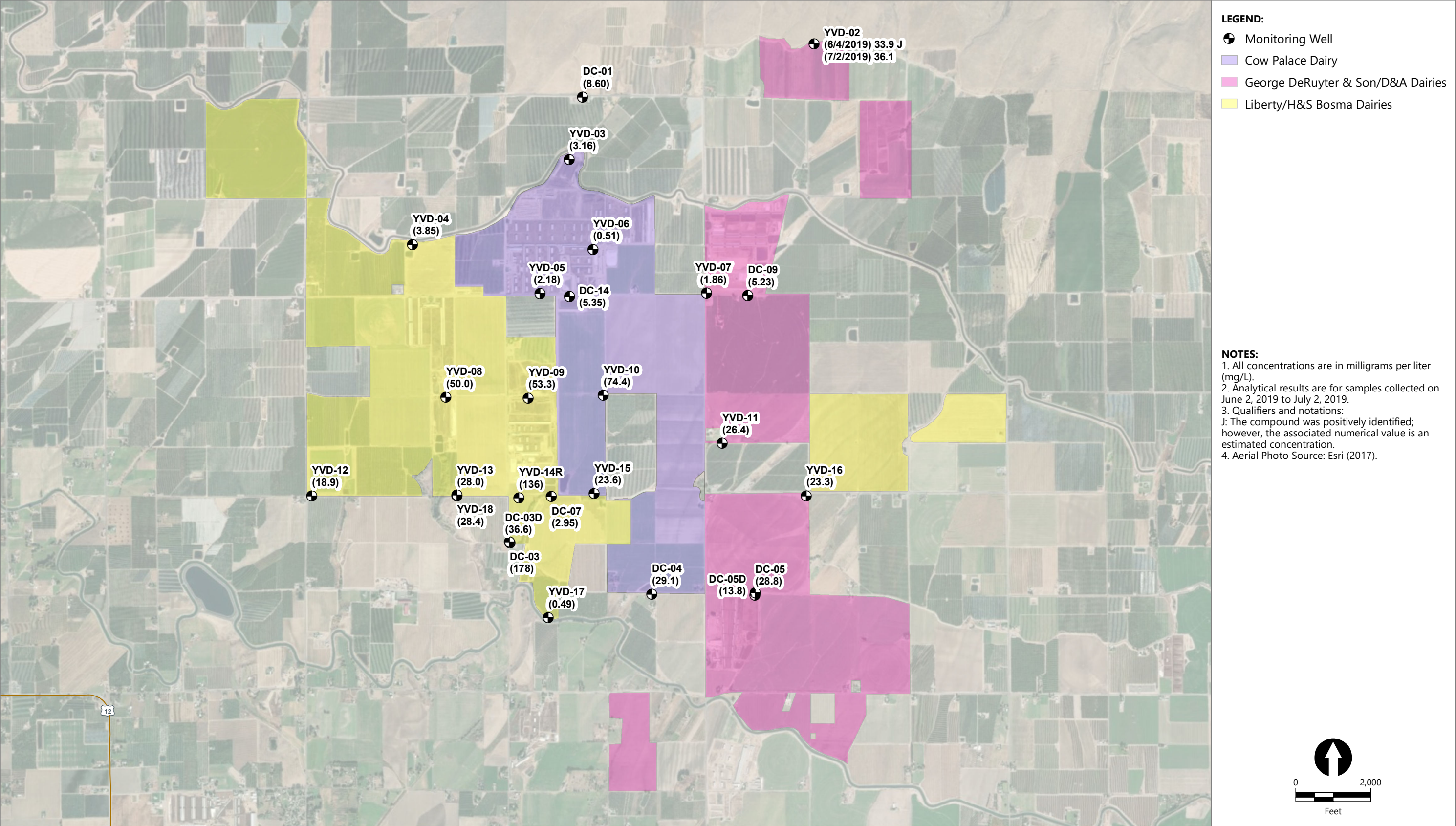
Figure 6A Nitrate Concentrations in Groundwater Second Quarter 2019 Groundwater Monitoring Data Report – Second Quarter 2019 Yakima Valley Dairies
