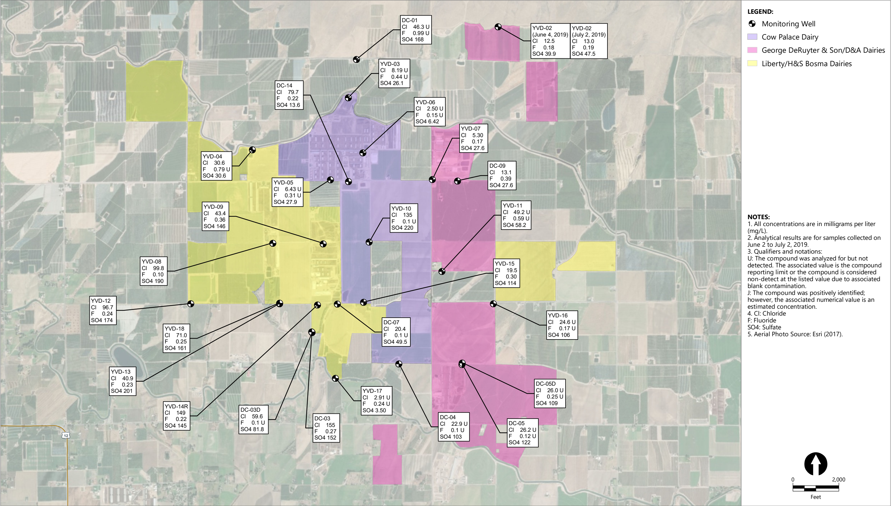
Figure 3 Anion Concentrations in Groundwater Second Quarter 2019 Groundwater Monitoring Data Report – Second Quarter 2019 Yakima Valley Dairies
