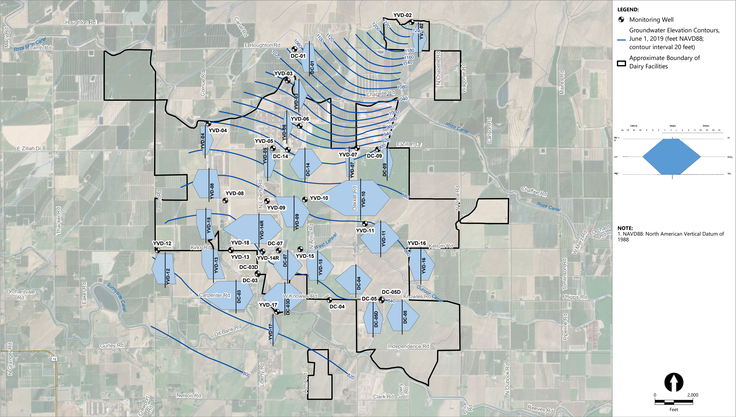
Figure 13 Stiff Diagrams and Groundwater Elevation Contour Map Groundwater Monitoring Data Report – Second Quarter 2019 Yakima Valley Dairies
