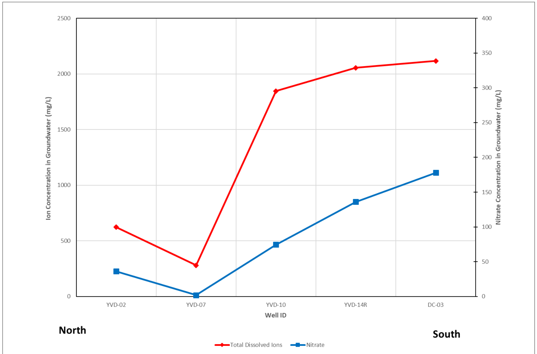
Figure 14 Nitrate and Total Dissolved Ion Concentration Along North-South Transect Groundwater Monitoring Data Report – Second Quarter 2019 Yakima Valley Dairies
