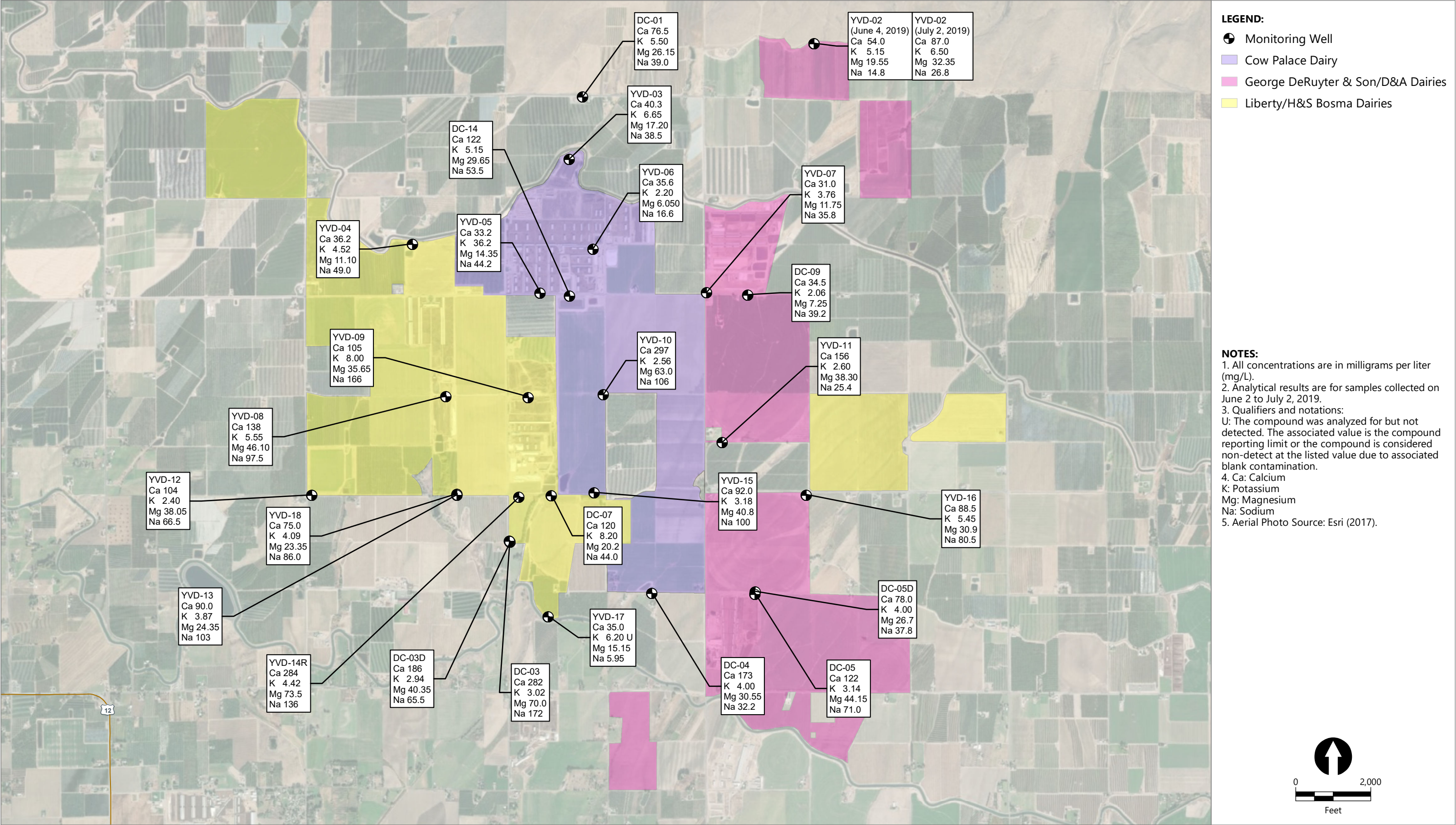
Figure 4 Metals Concentrations in Groundwater Second Quarter 2019 Groundwater Monitoring Data Report – Second Quarter 2019 Yakima Valley Dairies
