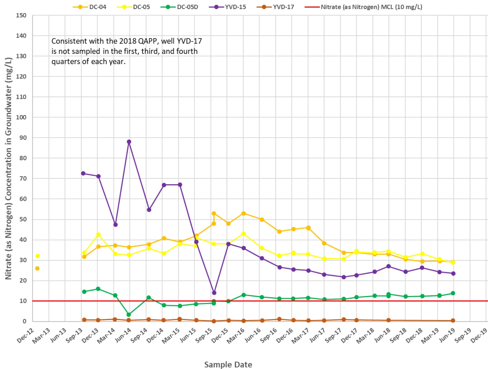
Figure 7 Nitrate Concentrations – East Downgradient Wells Groundwater Monitoring Data Report – Second Quarter 2019 Yakima Valley Dairies
