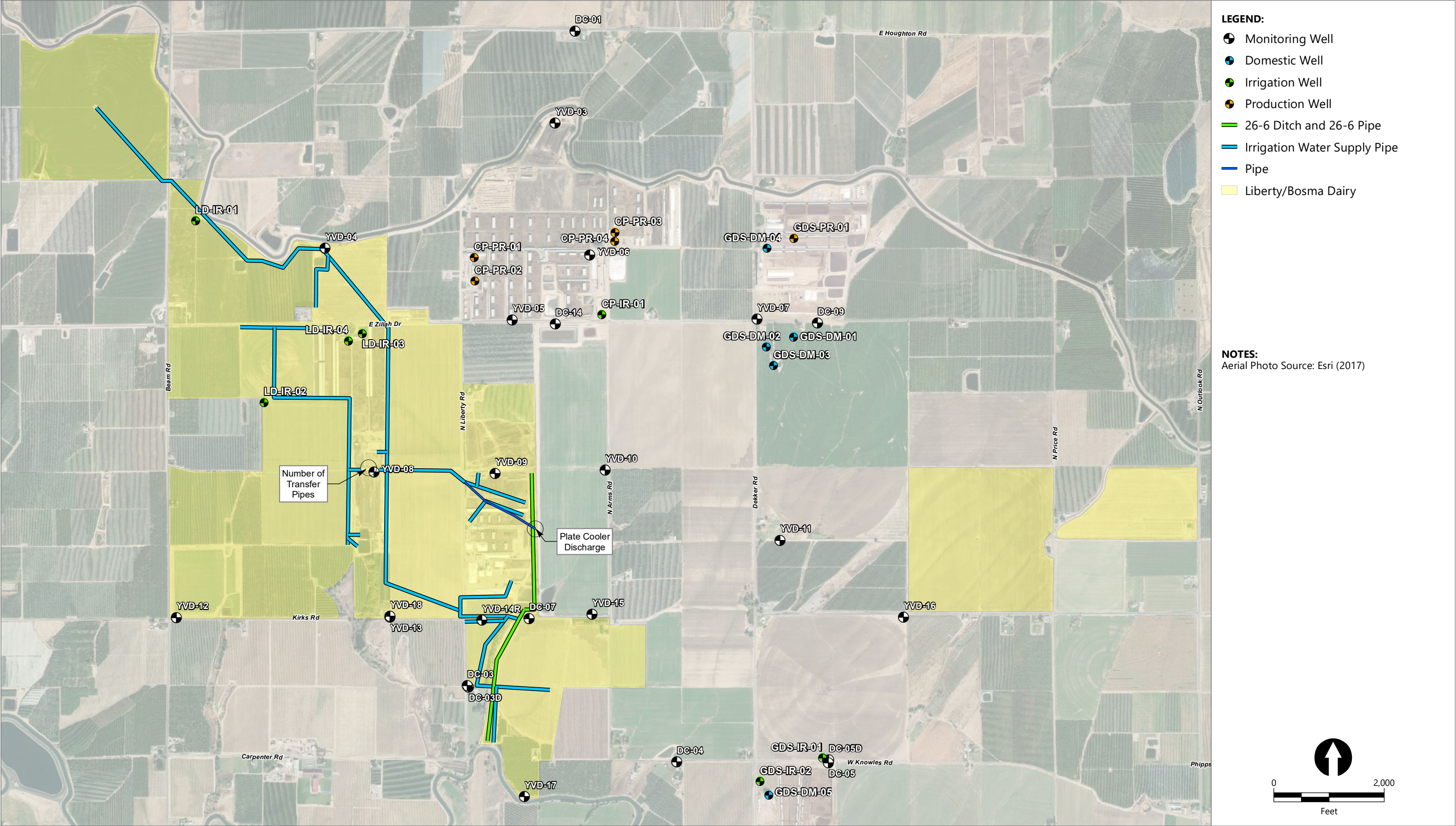
Figure 3D Facility Plan – Liberty/H&S Bosma Dairies Groundwater Monitoring Data Report – Fourth Quarter 2019 Yakima Valley Dairies
