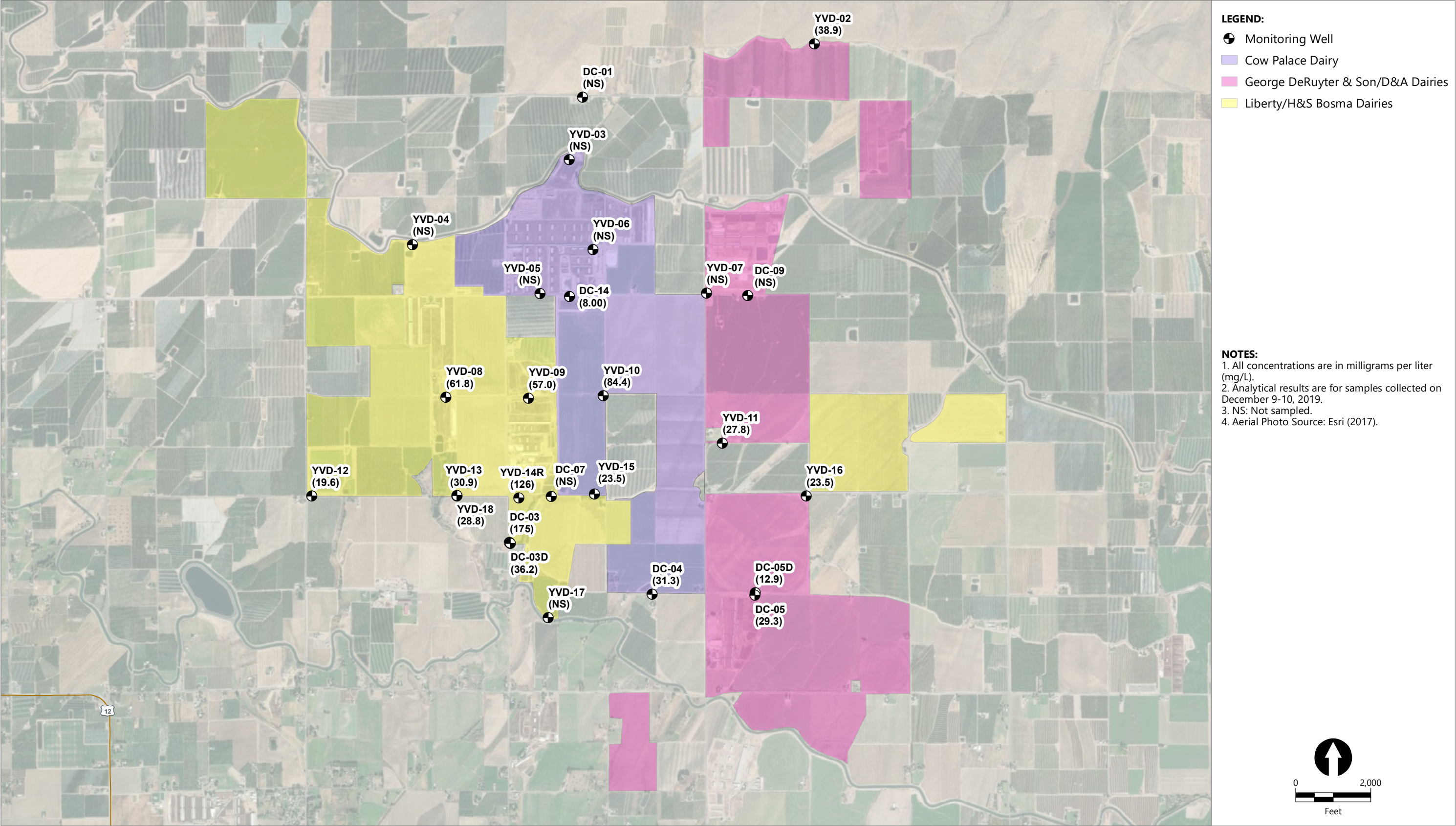
Figure 17A Nitrate Concentrations in Groundwater Fourth Quarter 2019 Groundwater Monitoring Data Report – Fourth Quarter 2019 Yakima Valley Dairies
