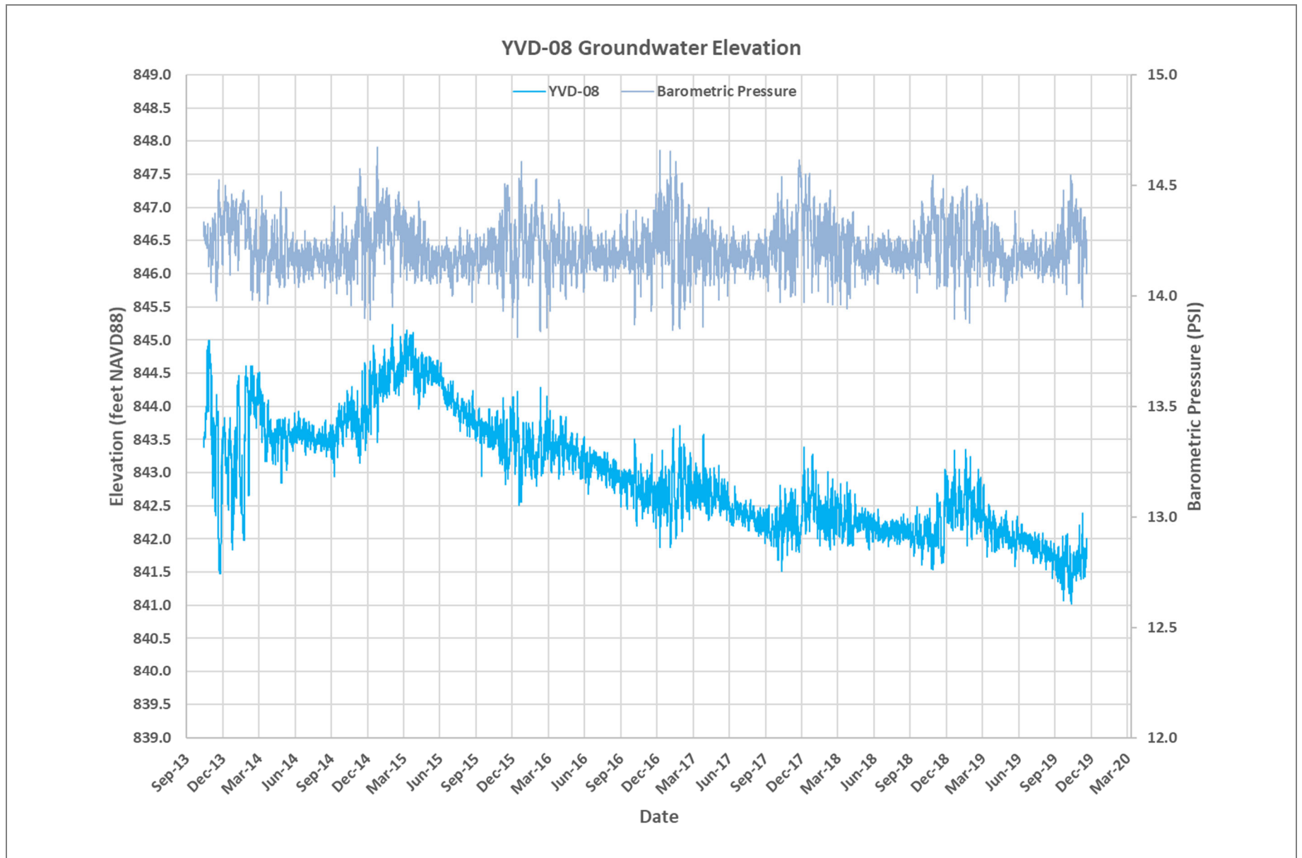
Figure 16F Groundwater Hydrographs – YVD-08 Groundwater Monitoring Data Report – Fourth Quarter 2019 Yakima Valley Dairies
