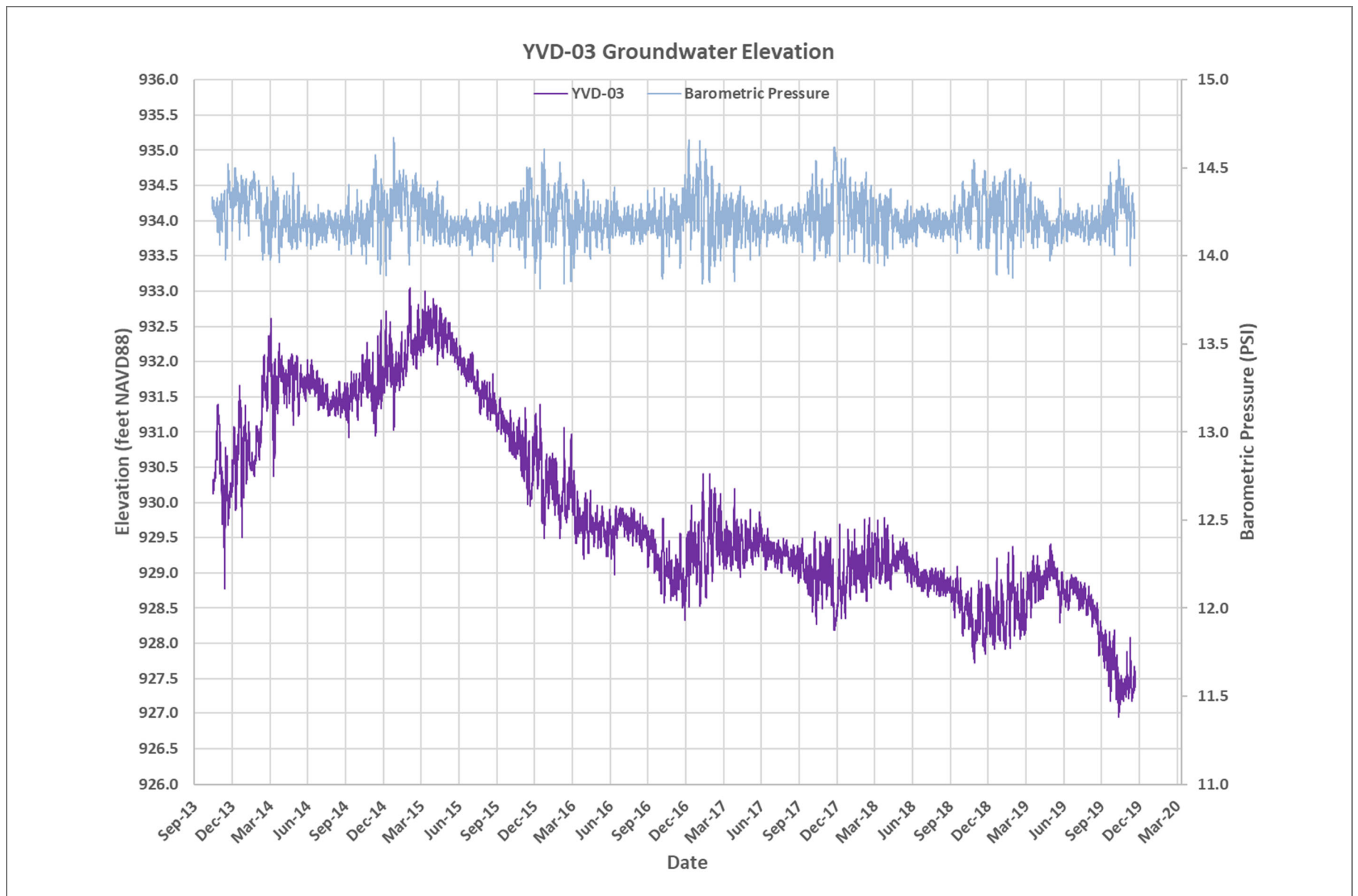
Figure 16E Groundwater Hydrographs – YVD-03 Groundwater Monitoring Data Report – Fourth Quarter 2019 Yakima Valley Dairies
