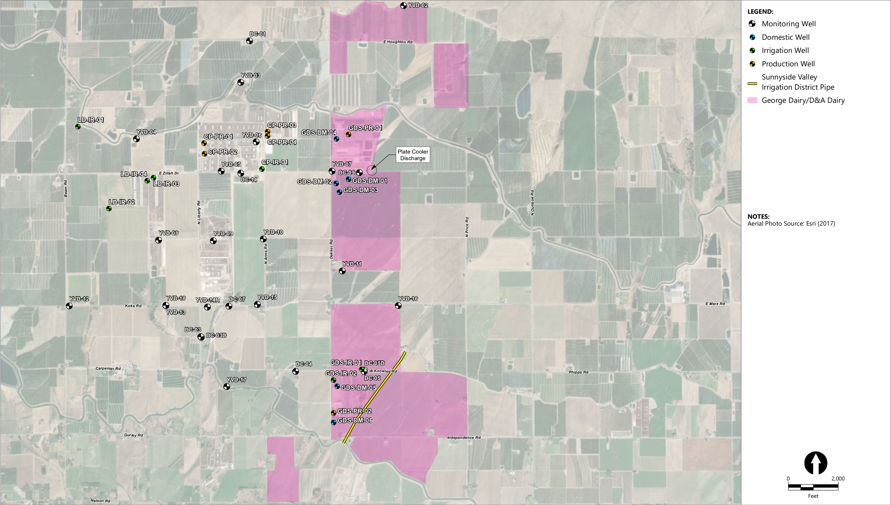
Figure 3C Facility Plan – George DeRuyter & Son/D&A Dairies Groundwater Monitoring Data Report – Fourth Quarter 2019 Yakima Valley Dairies
