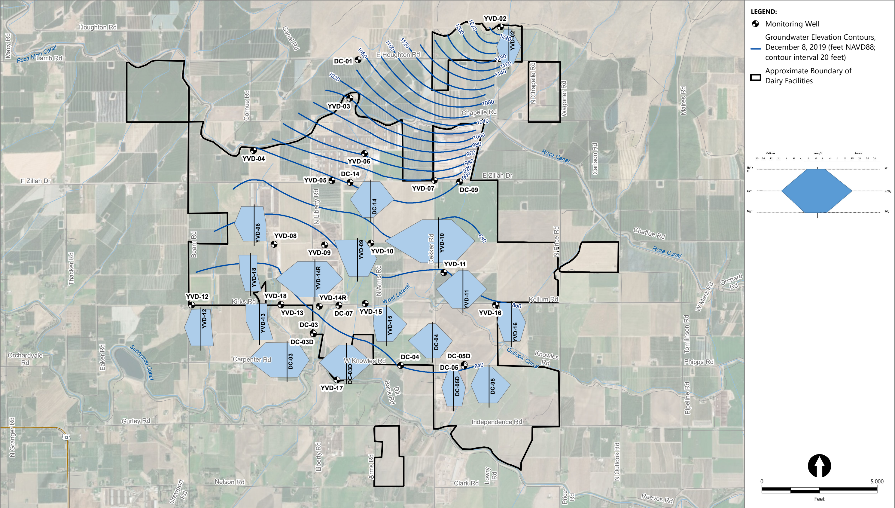
Figure 29 Stiff Diagrams and Groundwater Elevation Contour Map Groundwater Monitoring Data Report – Fourth Quarter 2019 Yakima Valley Dairies
