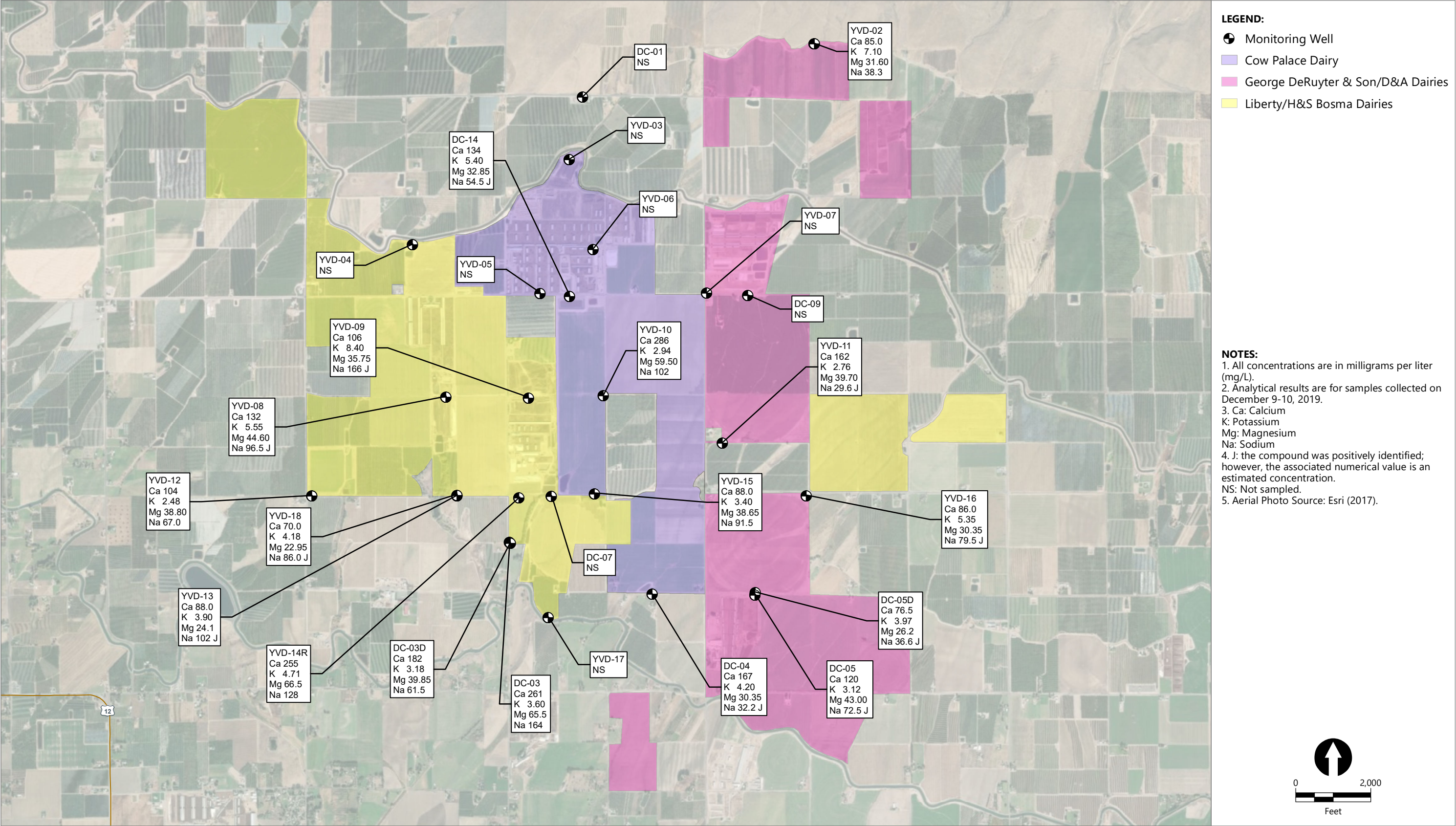
Figure 26 Metals Concentrations in Groundwater Fourth Quarter 2019 Groundwater Monitoring Data Report – Fourth Quarter 2019 Yakima Valley Dairies
