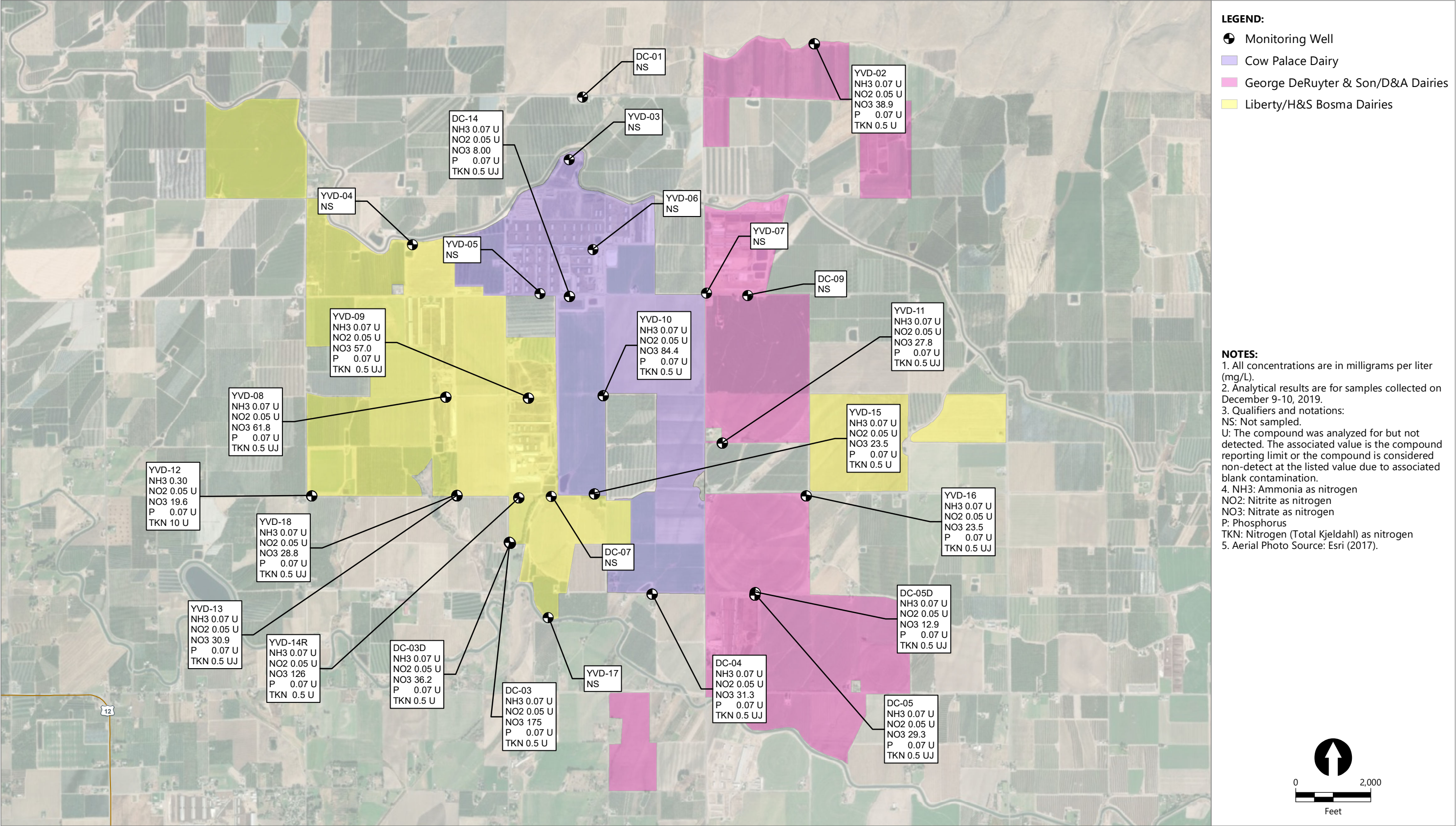
Figure 24 Nutrient Concentrations in Groundwater Fourth Quarter 2019 Groundwater Monitoring Data Report – Fourth Quarter 2019 Yakima Valley Dairies
