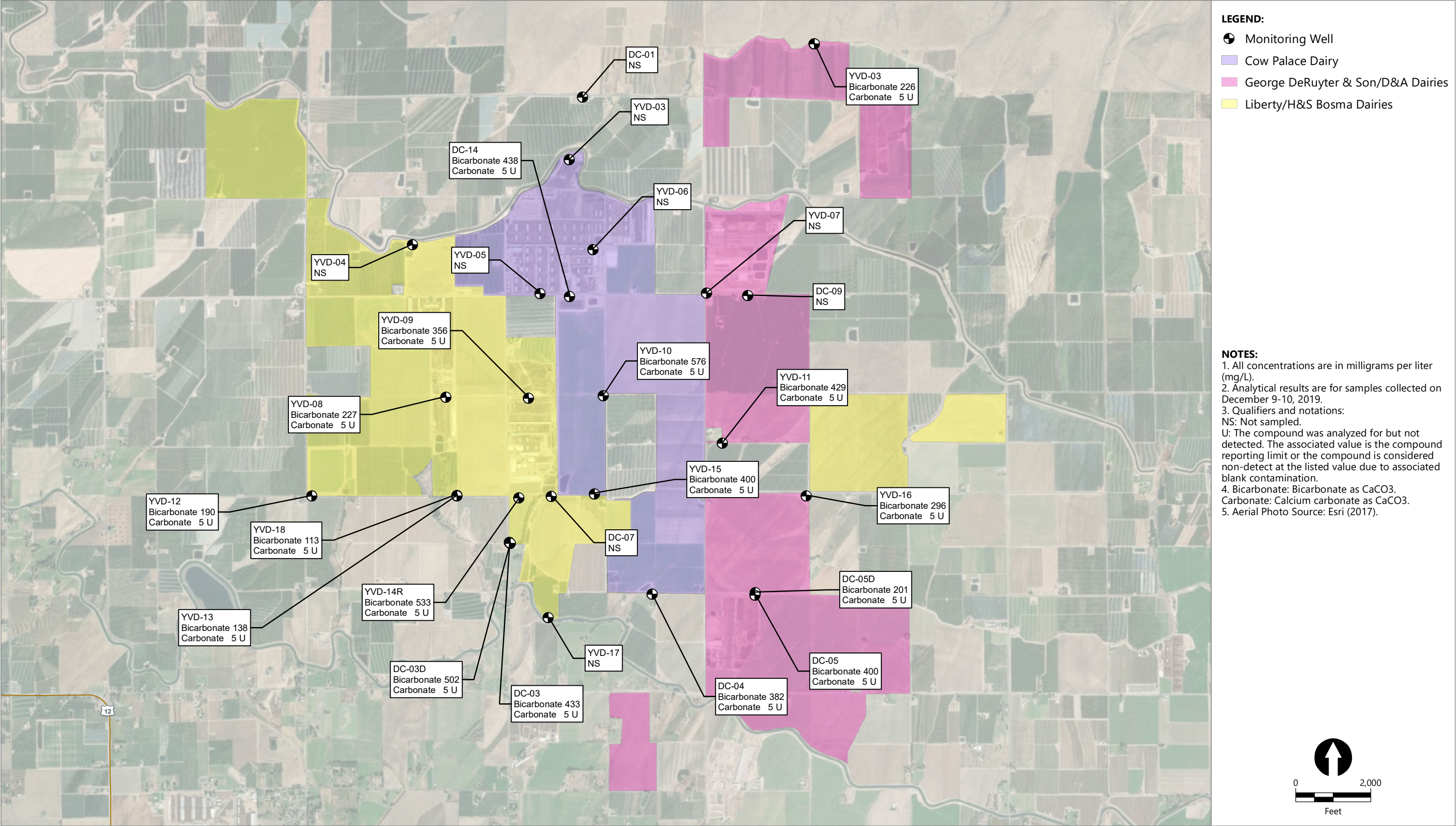
Figure 27 Alkalinity Concentrations in Groundwater Fourth Quarter 2019 Groundwater Monitoring Data Report – Fourth Quarter 2019 Yakima Valley Dairies
