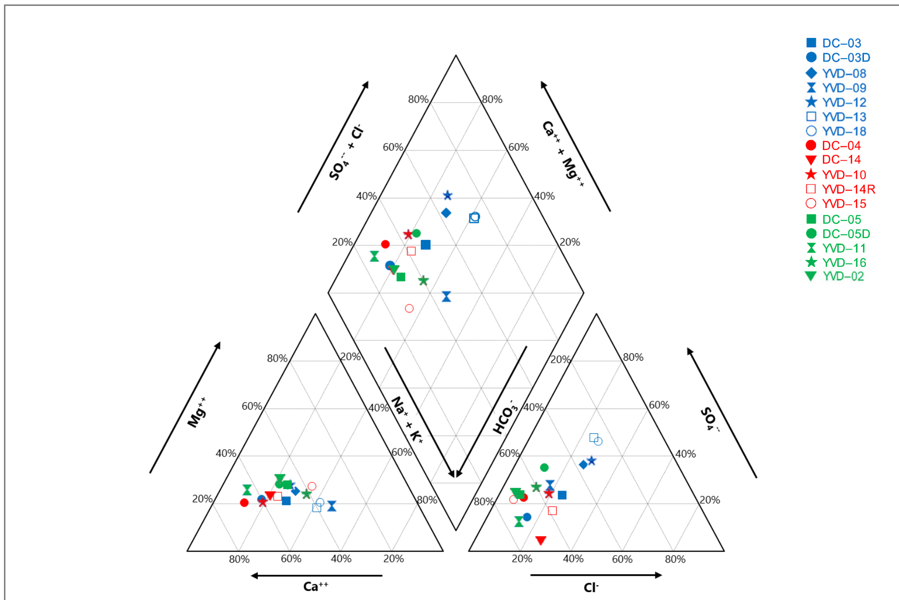
Figure 30 Piper Diagram – All Wells Groundwater Monitoring Data Report – Fourth Quarter 2019 Yakima Valley Dairies
