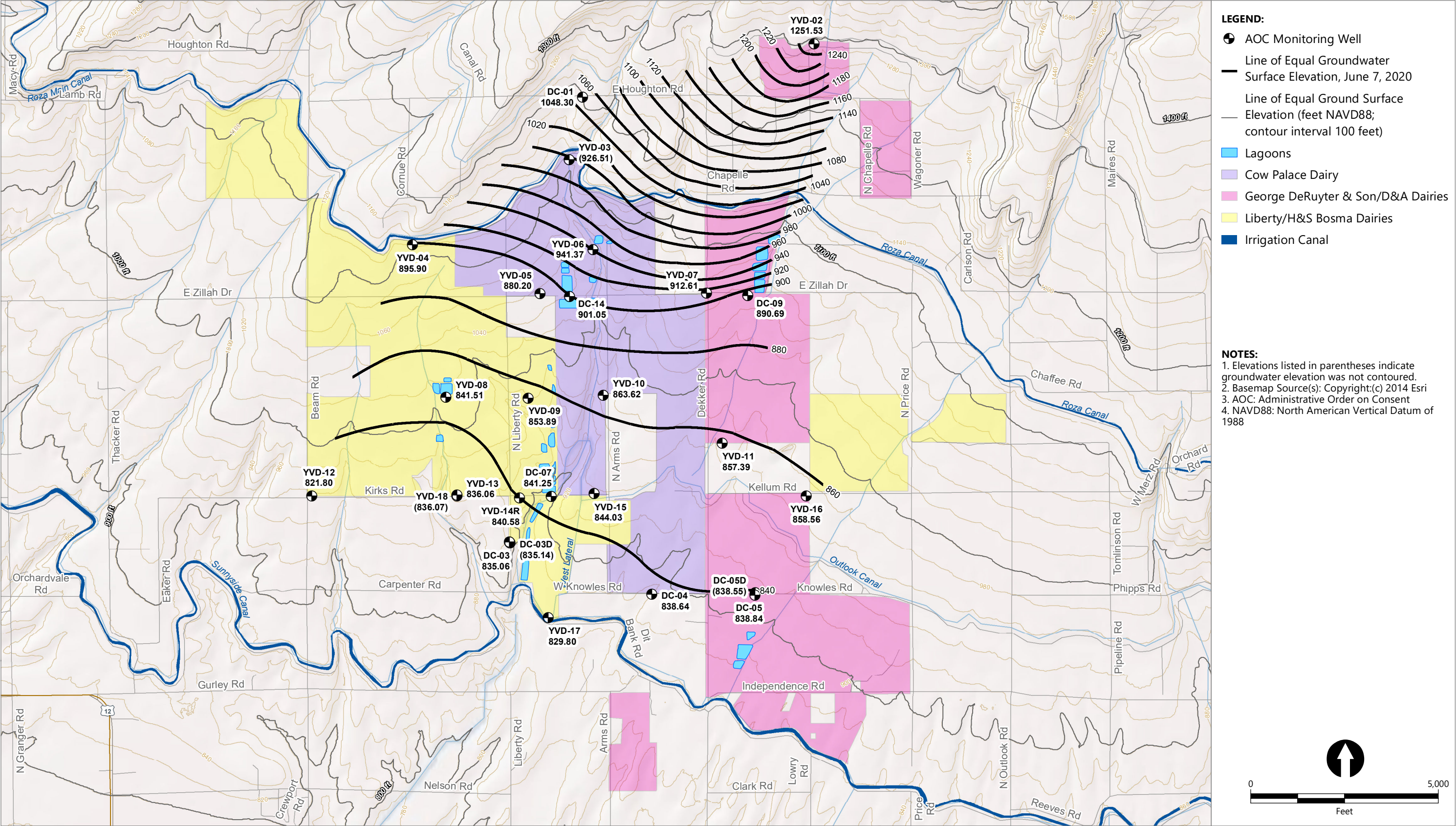
Figure 1 Surficial Aquifer Groundwater Elevation Contour Map Second Quarter 2020 Groundwater Monitoring Data Report – Second Quarter 2020 Yakima Valley Dairies
