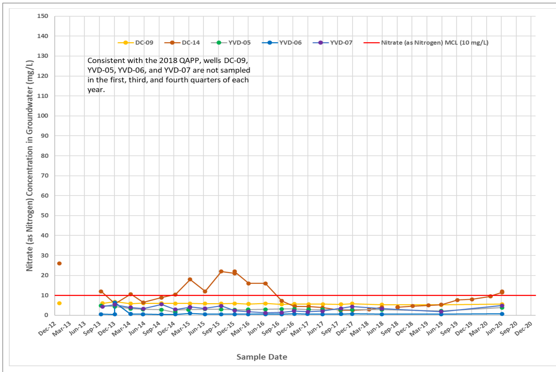
Figure 11 Nitrate Concentrations – Northern Wells Groundwater Monitoring Data Report – Second Quarter 2020 Yakima Valley Dairies
