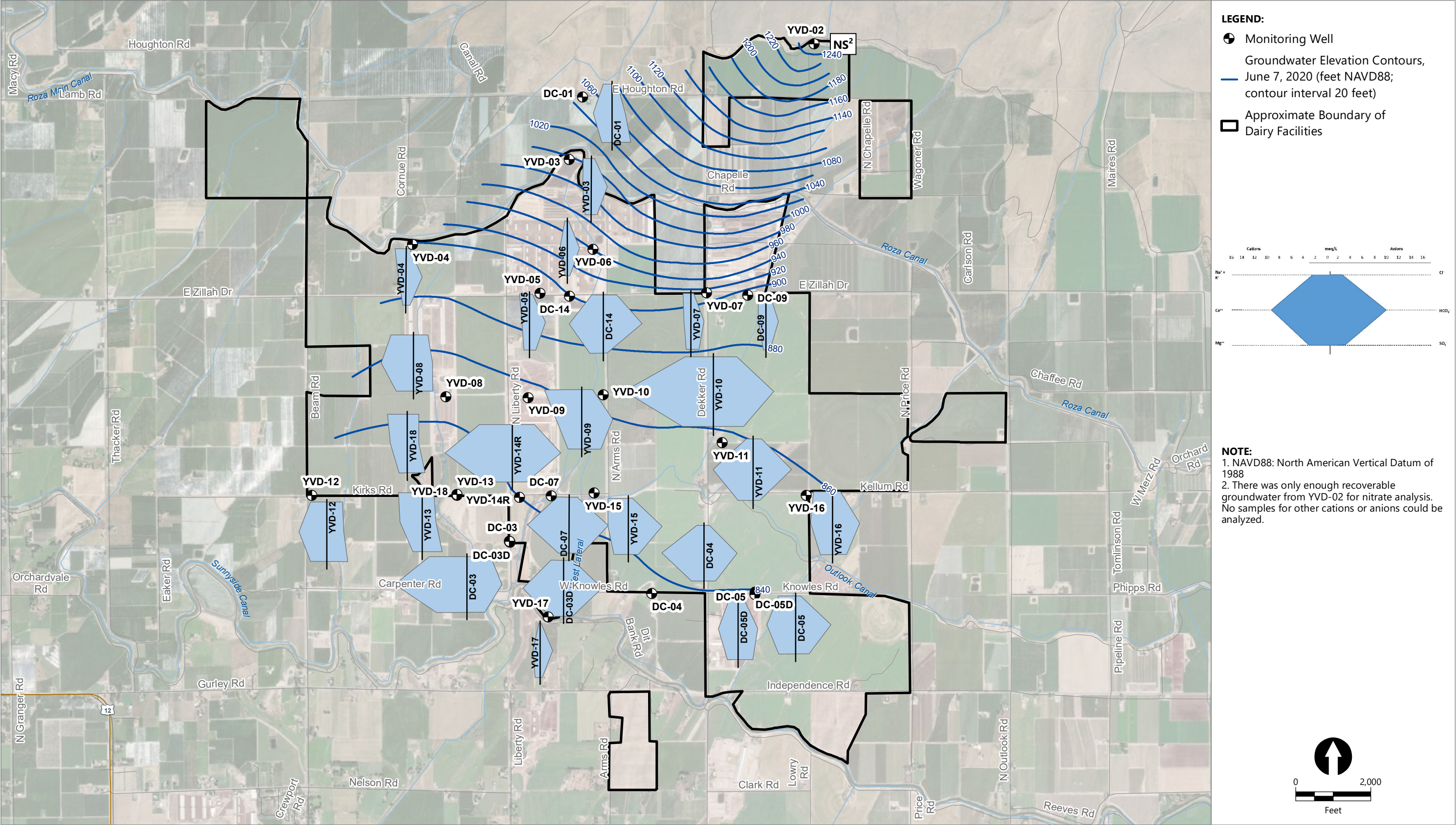
Figure 14 Stiff Diagrams and Groundwater Elevation Contour Map Groundwater Monitoring Data Report – Second Quarter 2020 Yakima Valley Dairies
