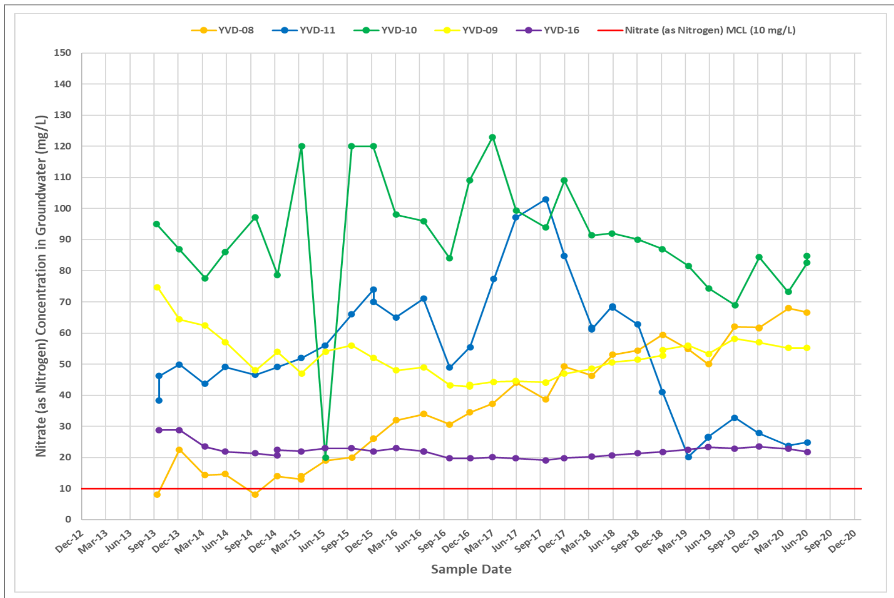
Figure 10 Nitrate Concentrations – Central Wells
