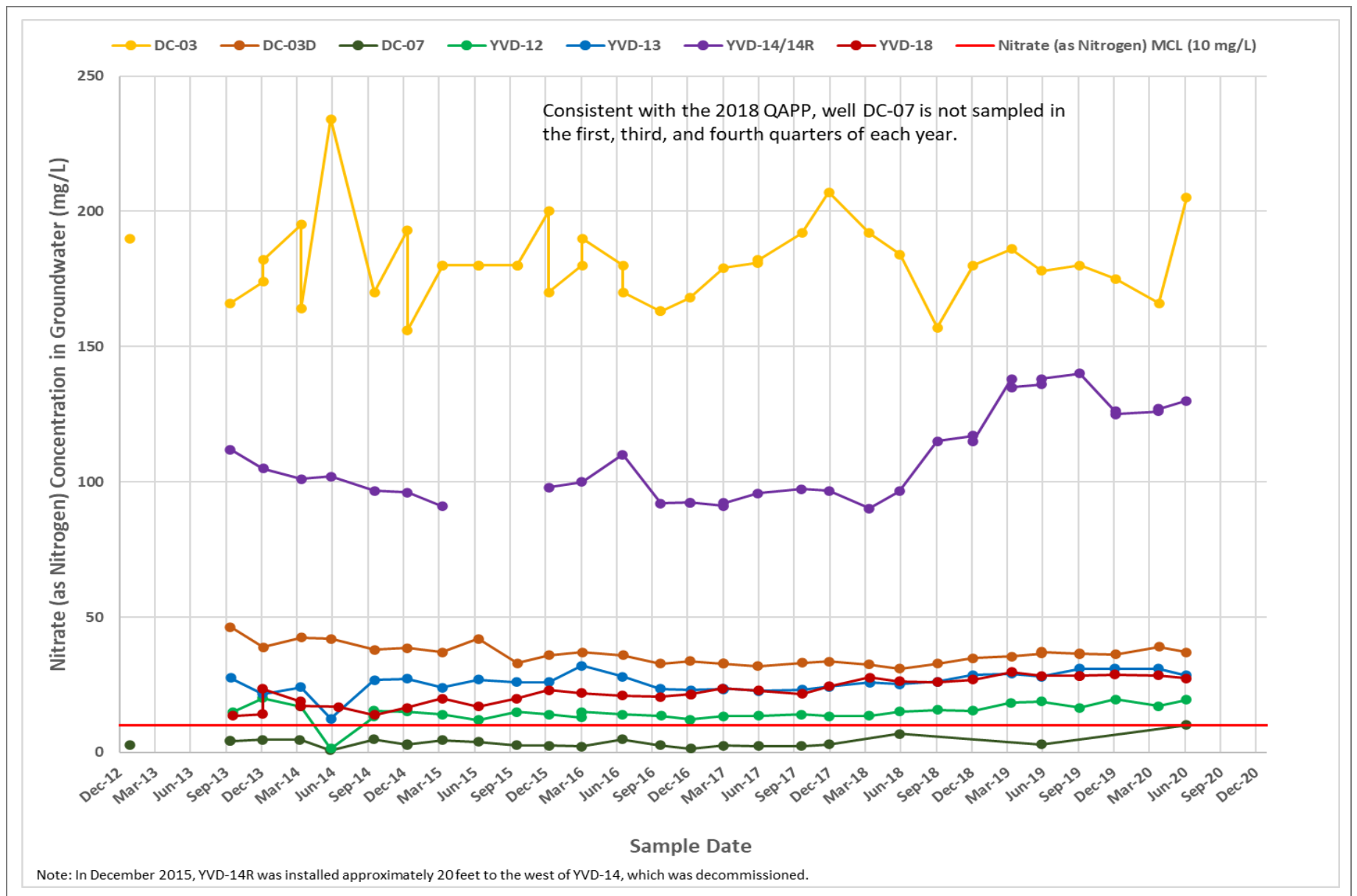
Figure 9 Nitrate Concentrations – West Downgradient Wells Groundwater Monitoring Data Report – Second Quarter 2020 Yakima Valley Dairies
