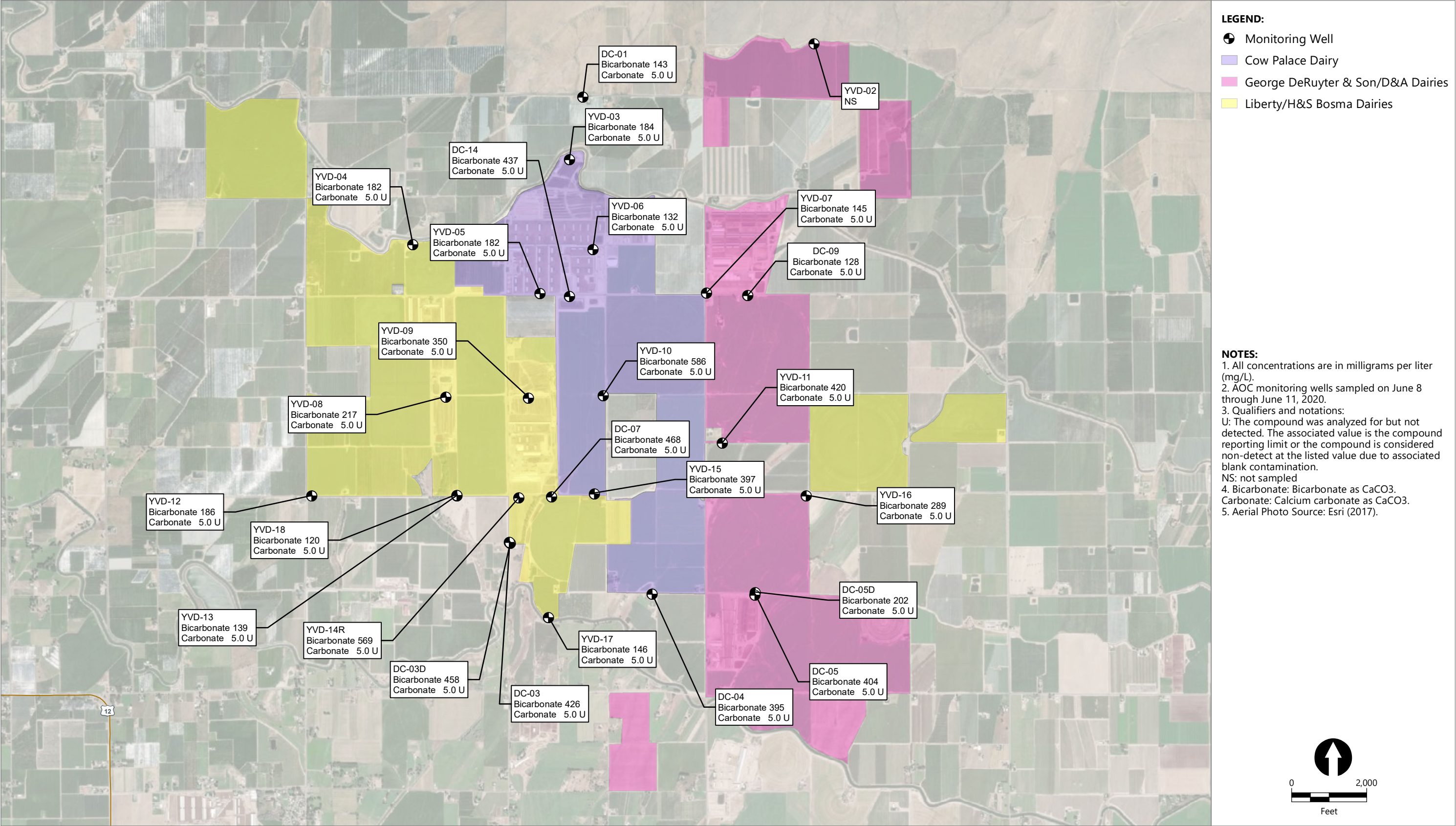
Figure 6 Alkalinity Concentrations in Groundwater Second Quarter 2020 Groundwater Monitoring Data Report – Second Quarter 2020 Yakima Valley Dairies
