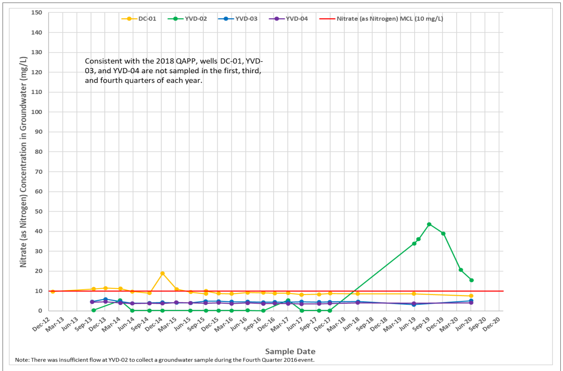
Figure 12 Nitrate Concentrations – Upgradient Wells Groundwater Monitoring Data Report – Second Quarter 2020 Yakima Valley Dairies
