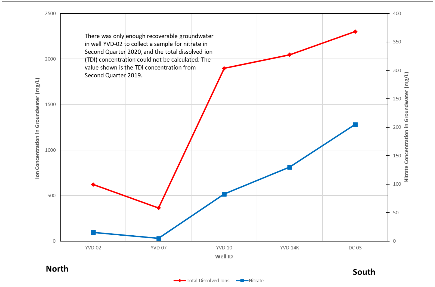
Figure 15 Nitrate and Total Dissolved Ion Concentration Along North-South Transect Groundwater Monitoring Data Report – Second Quarter 2020 Yakima Valley Dairies
