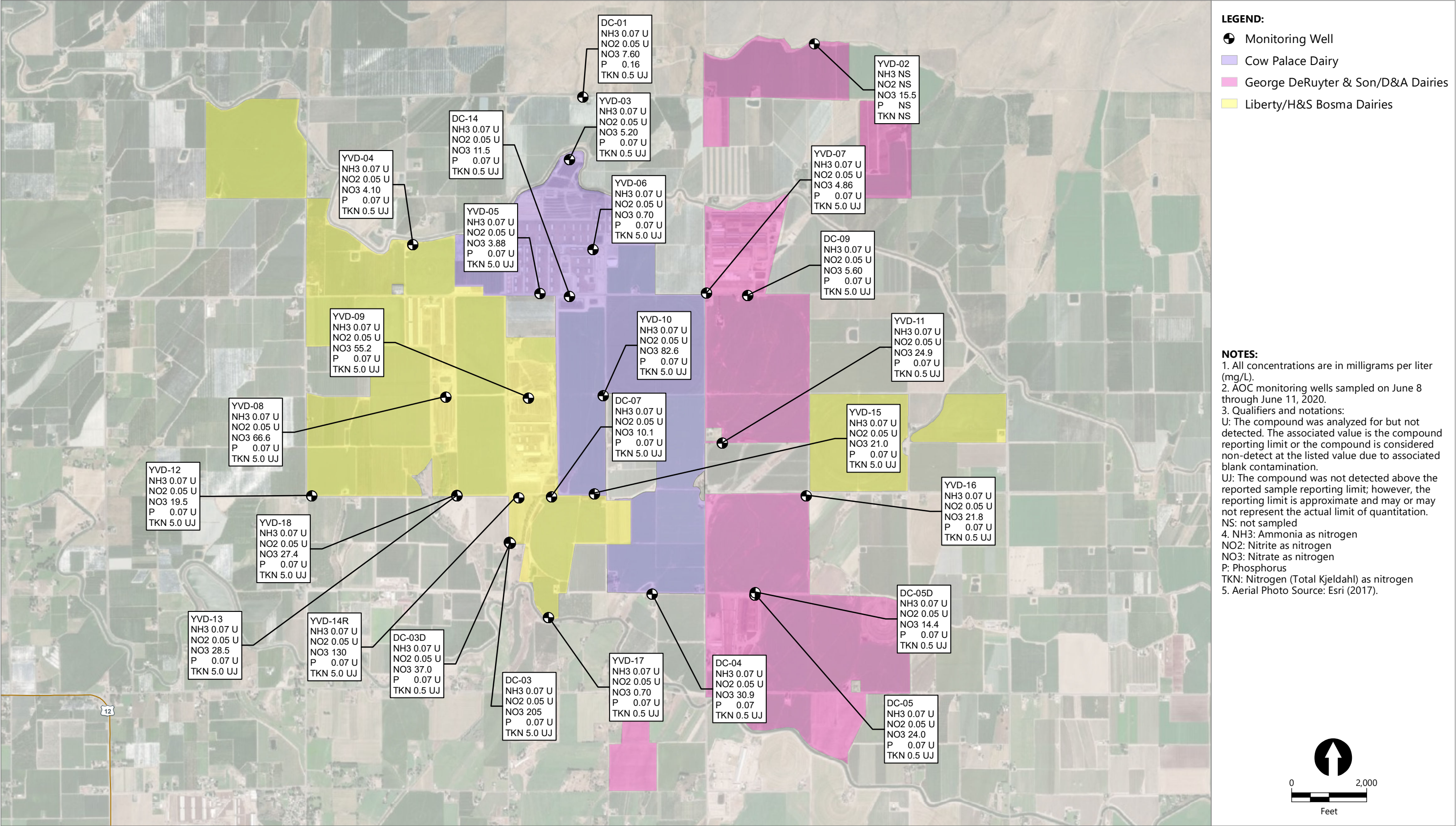
Figure 3 Nutrient Concentrations in Groundwater Second Quarter 2020 Groundwater Monitoring Data Report – Second Quarter 2020 Yakima Valley Dairies
