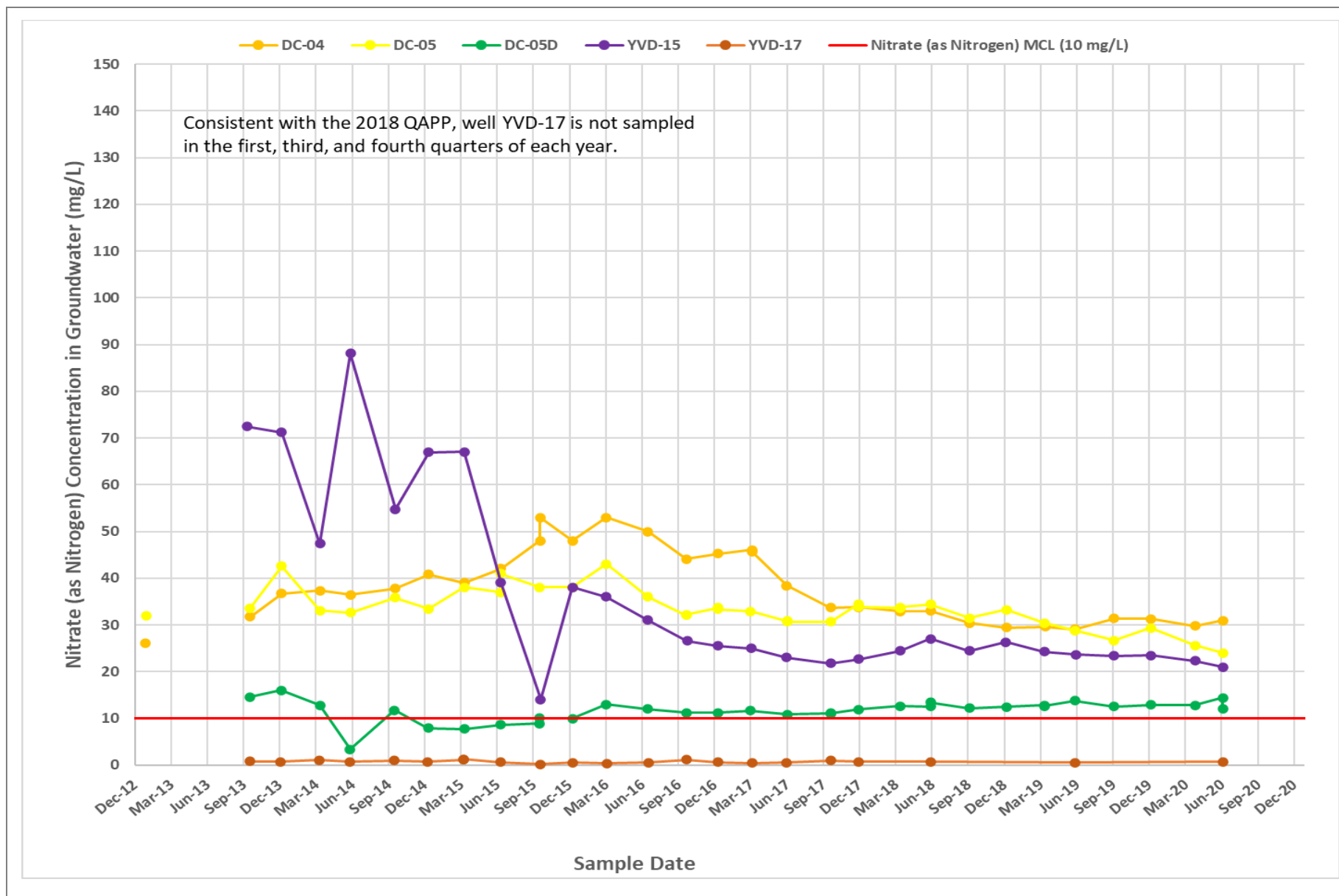
Figure 8 Nitrate Concentrations – East Downgradient Wells Groundwater Monitoring Data Report – Second Quarter 2020 Yakima Valley Dairies
