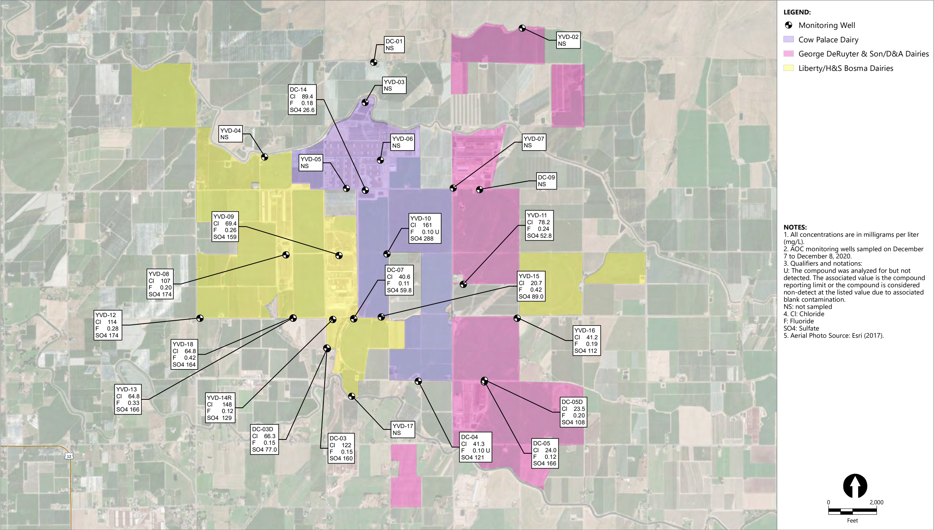
Figure 26 Anion Concentrations in Groundwater Fourth Quarter 2020 Groundwater Monitoring Data Report – Fourth Quarter 2020 Yakima Valley Dairies
