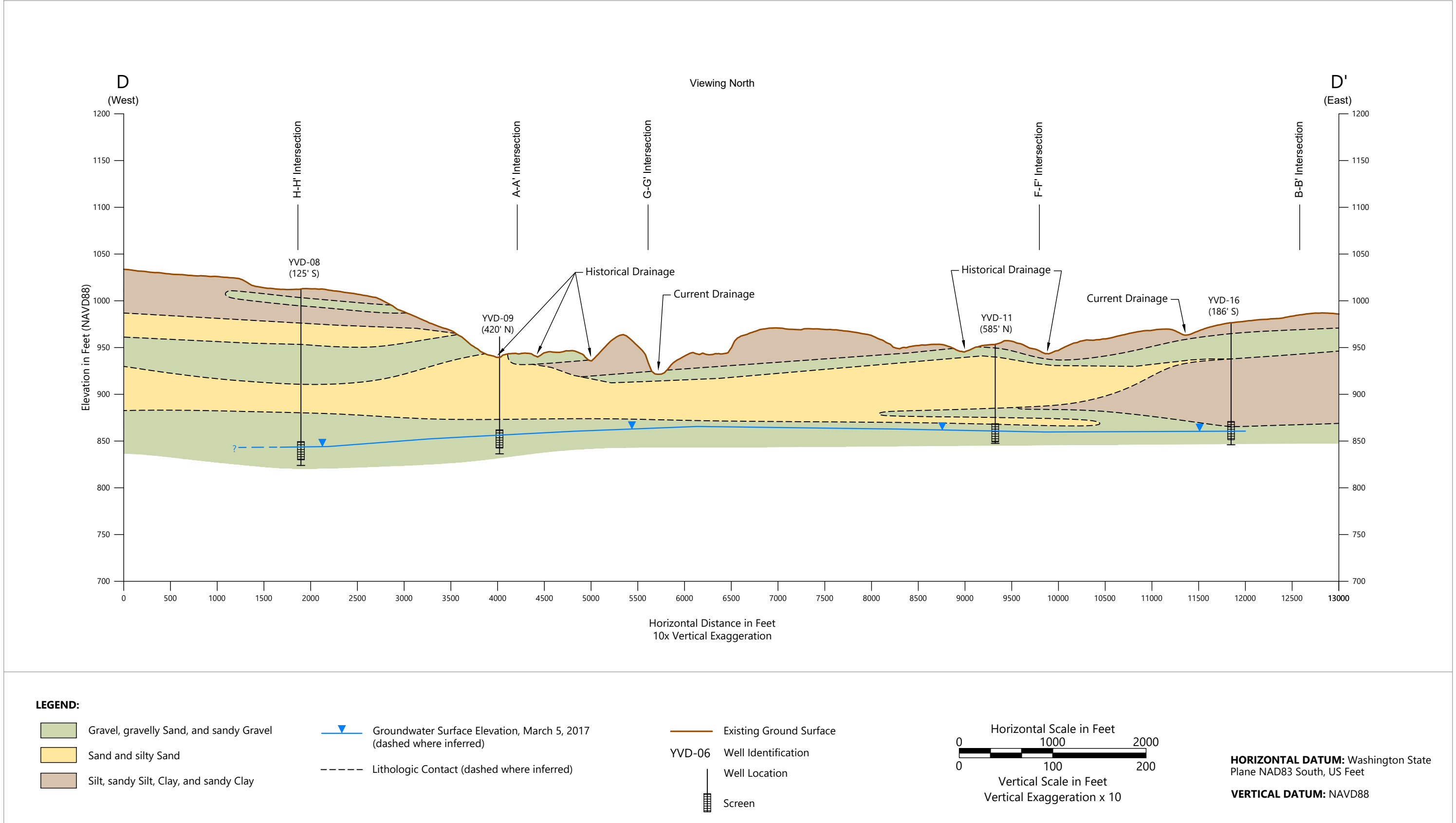
Figure 10 Geologic Cross Section D-D'
