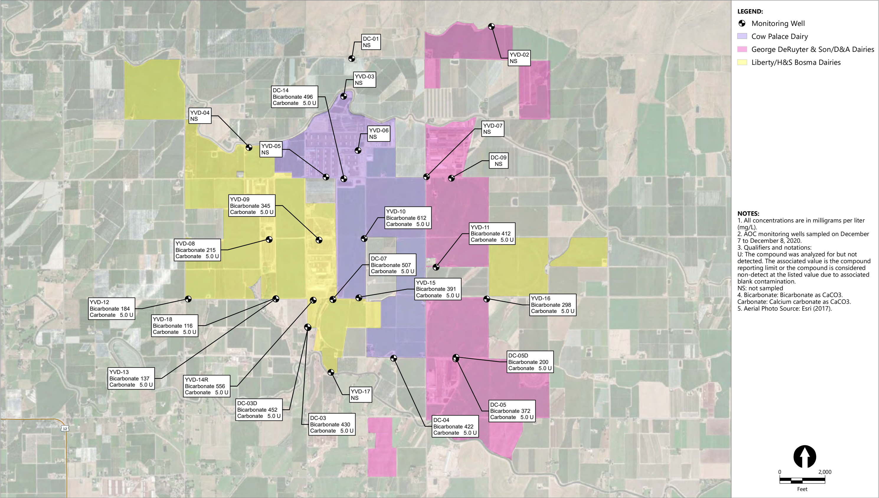
Figure 28 Alkalinity Concentrations in Groundwater Fourth Quarter 2020 Groundwater Monitoring Data Report – Fourth Quarter 2020 Yakima Valley Dairies
