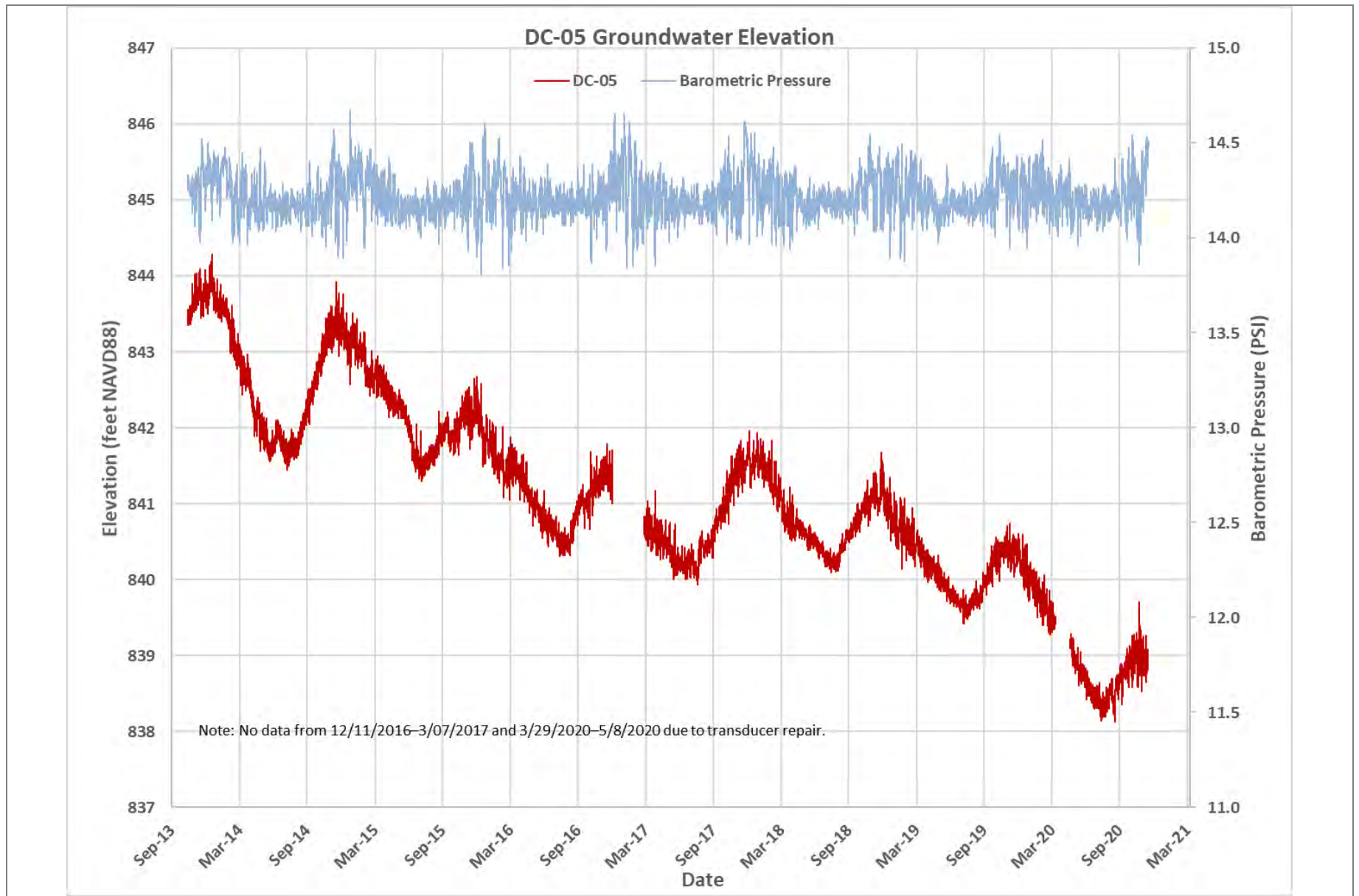
Figure 16C Groundwater Hydrographs – DC-05 Groundwater Monitoring Data Report – Fourth Quarter 2020 Yakima Valley Dairies
