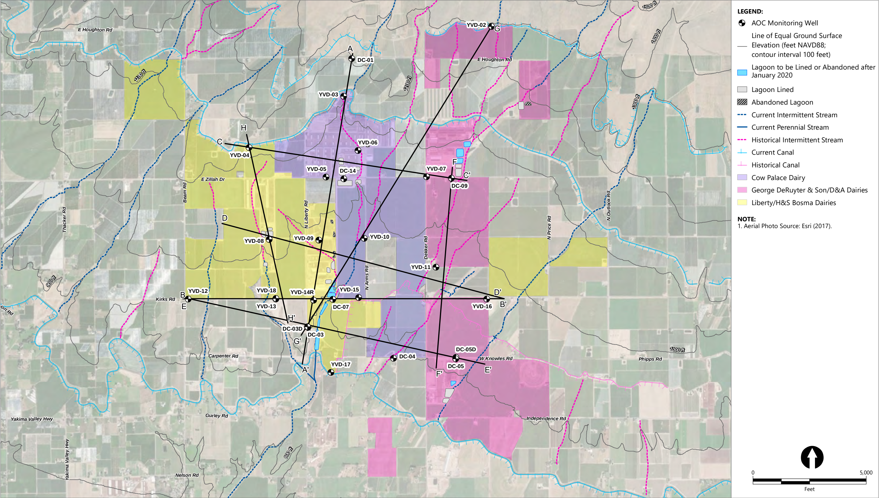
Figure 6 Cross Section Location Map Groundwater Monitoring Data Report – Fourth Quarter 2020 Yakima Valley Dairies
