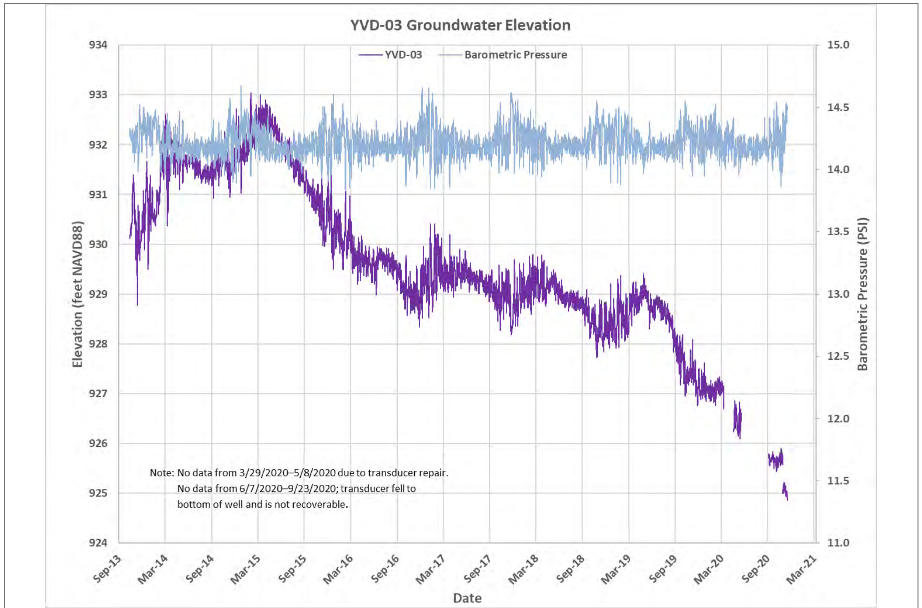
Figure 16E Groundwater Hydrographs – YVD-03 Groundwater Monitoring Data Report – Fourth Quarter 2020 Yakima Valley Dairies
