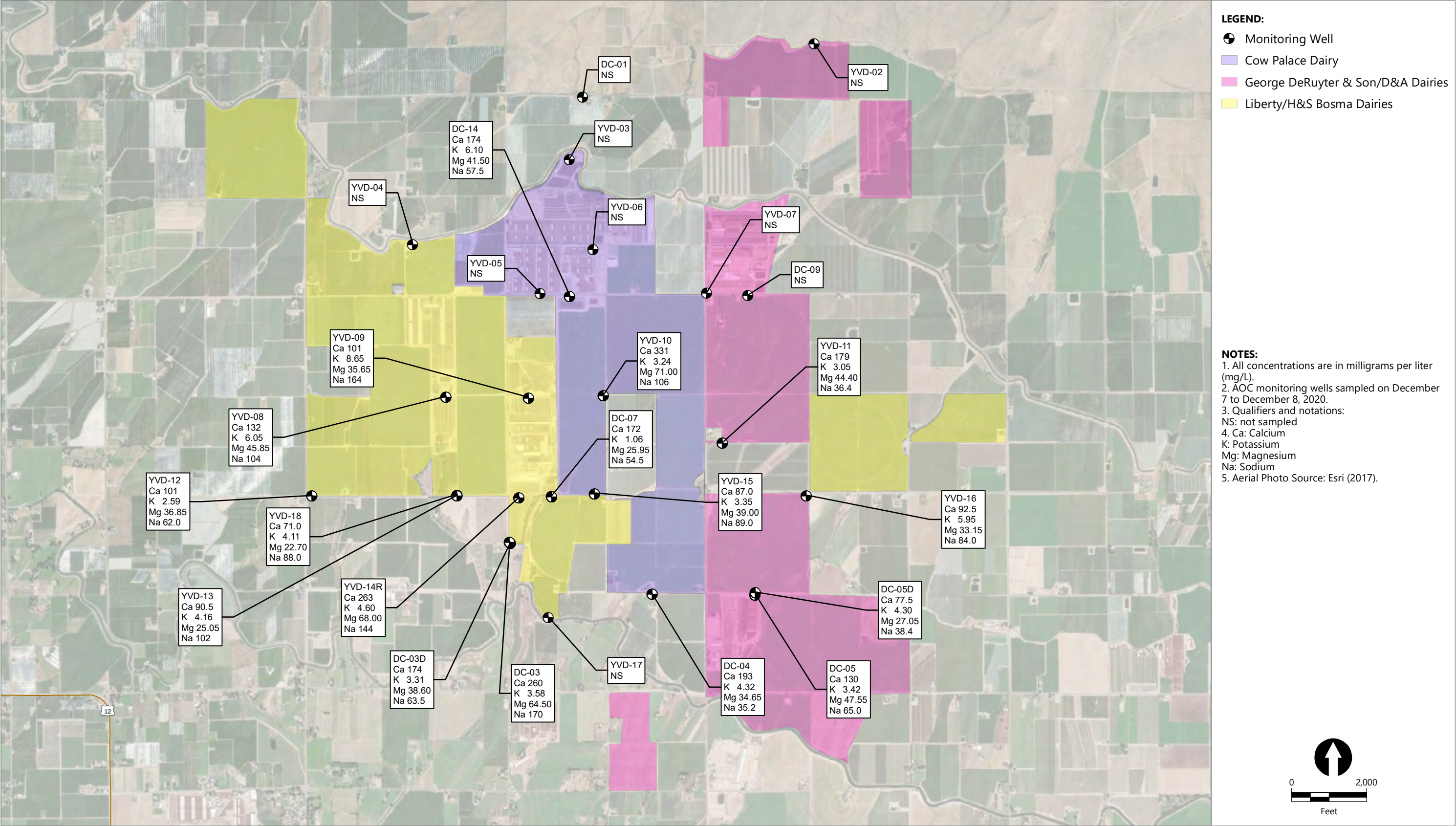
Figure 27 Metals Concentrations in Groundwater Fourth Quarter 2020 Groundwater Monitoring Data Report – Fourth Quarter 2020 Yakima Valley Dairies
