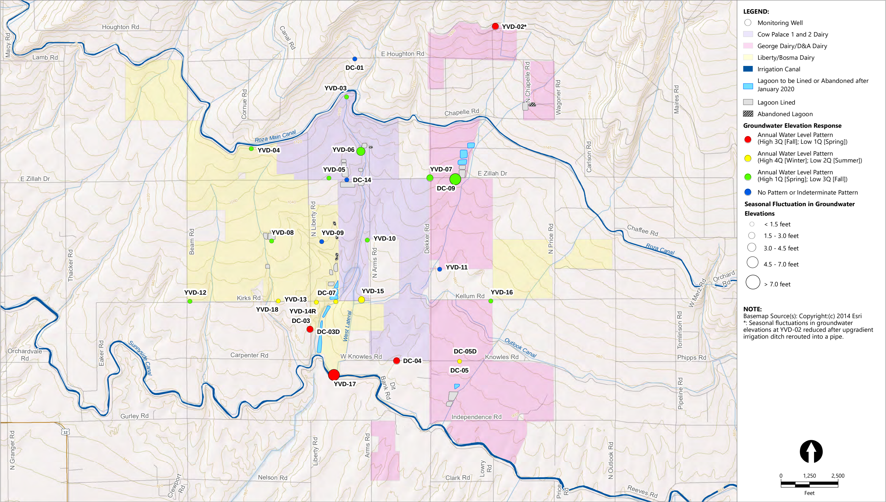
Figure 17 Seasonal Groundwater Elevation Patterns Groundwater Monitoring Data Report – Fourth Quarter 2020 Yakima Valley Dairies
