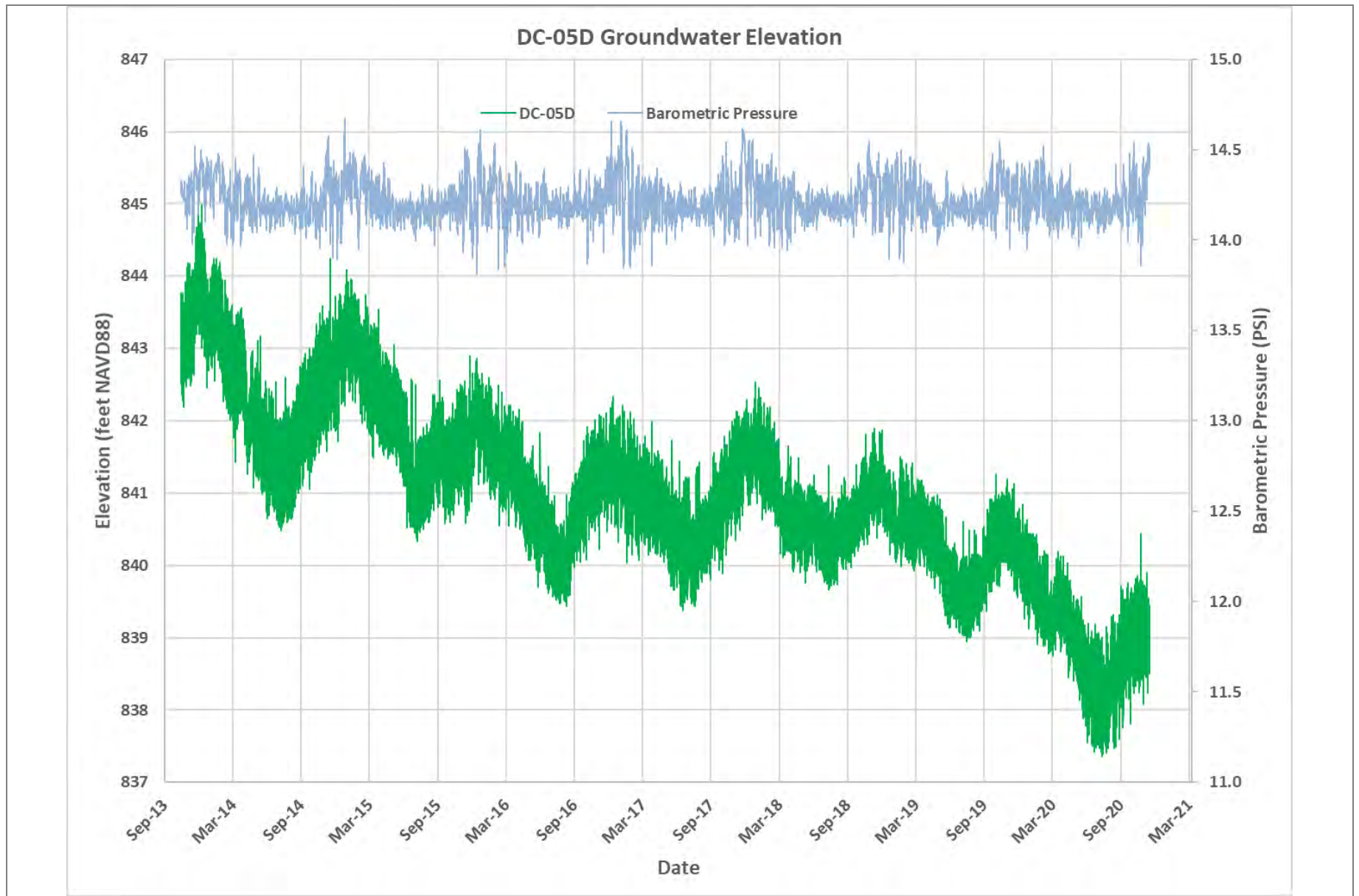
Figure 16D Groundwater Hydrographs – DC-05D Groundwater Monitoring Data Report – Fourth Quarter 2020 Yakima Valley Dairies
