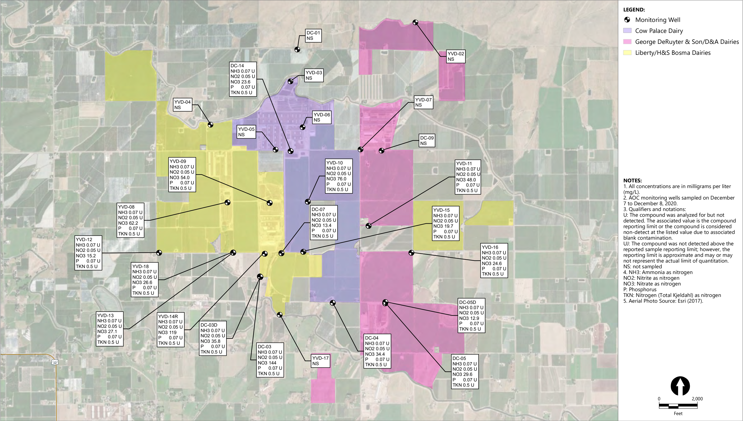
Figure 25 Nutrient Concentrations in Groundwater Fourth Quarter 2020 Groundwater Monitoring Data Report – Fourth Quarter 2020 Yakima Valley Dairies
