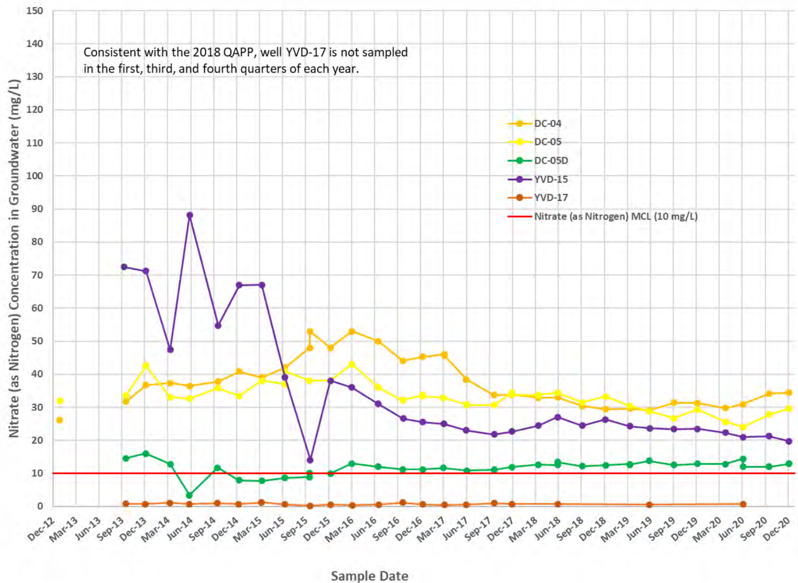
Figure 19 Nitrate Concentrations – East Downgradient Wells Groundwater Monitoring Data Report – Fourth Quarter 2020 Yakima Valley Dairies
