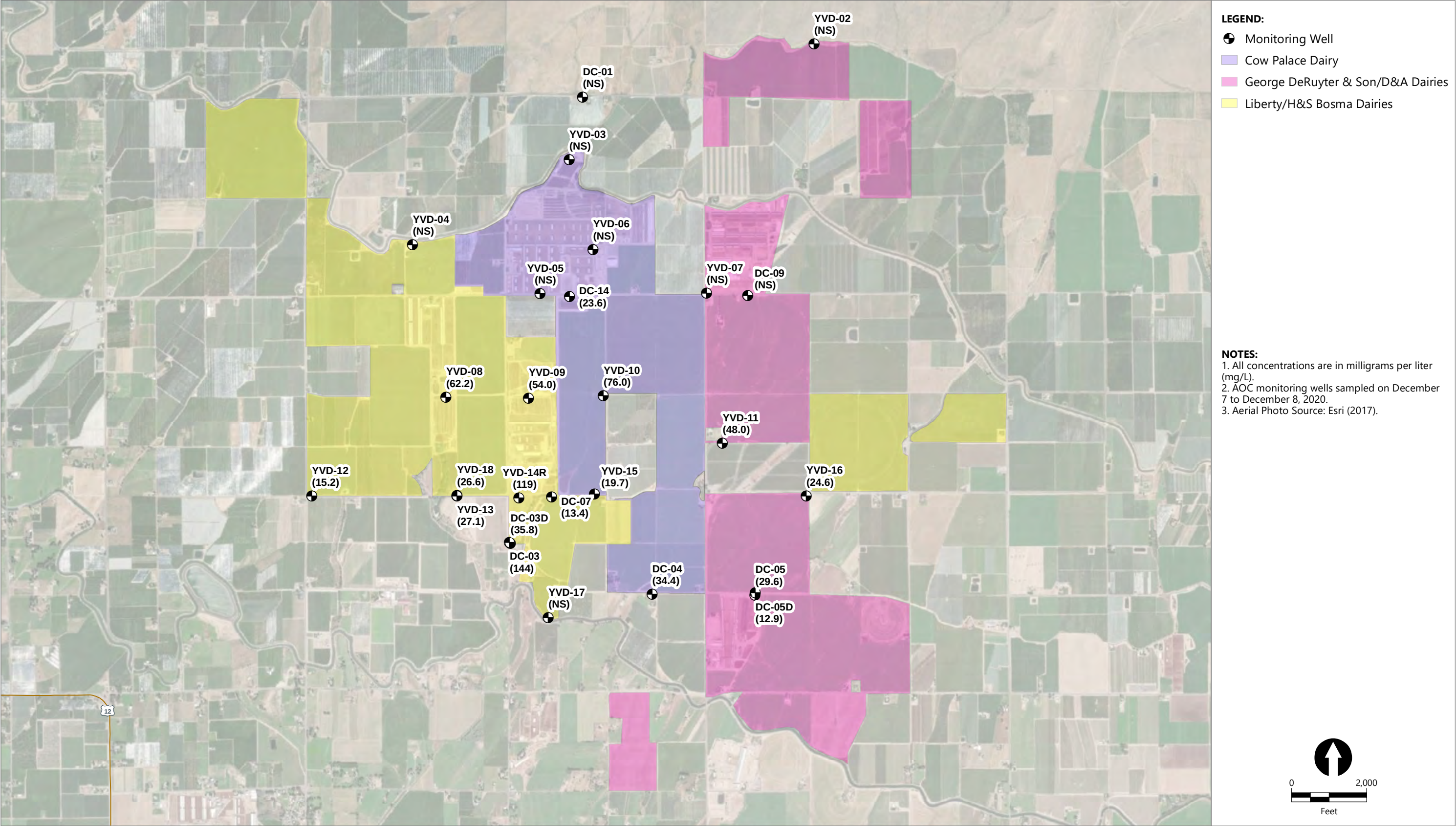
Figure 18A Nitrate Concentrations in Groundwater Fourth Quarter 2020 Groundwater Monitoring Data Report – Fourth Quarter 2020 Yakima Valley Dairies
