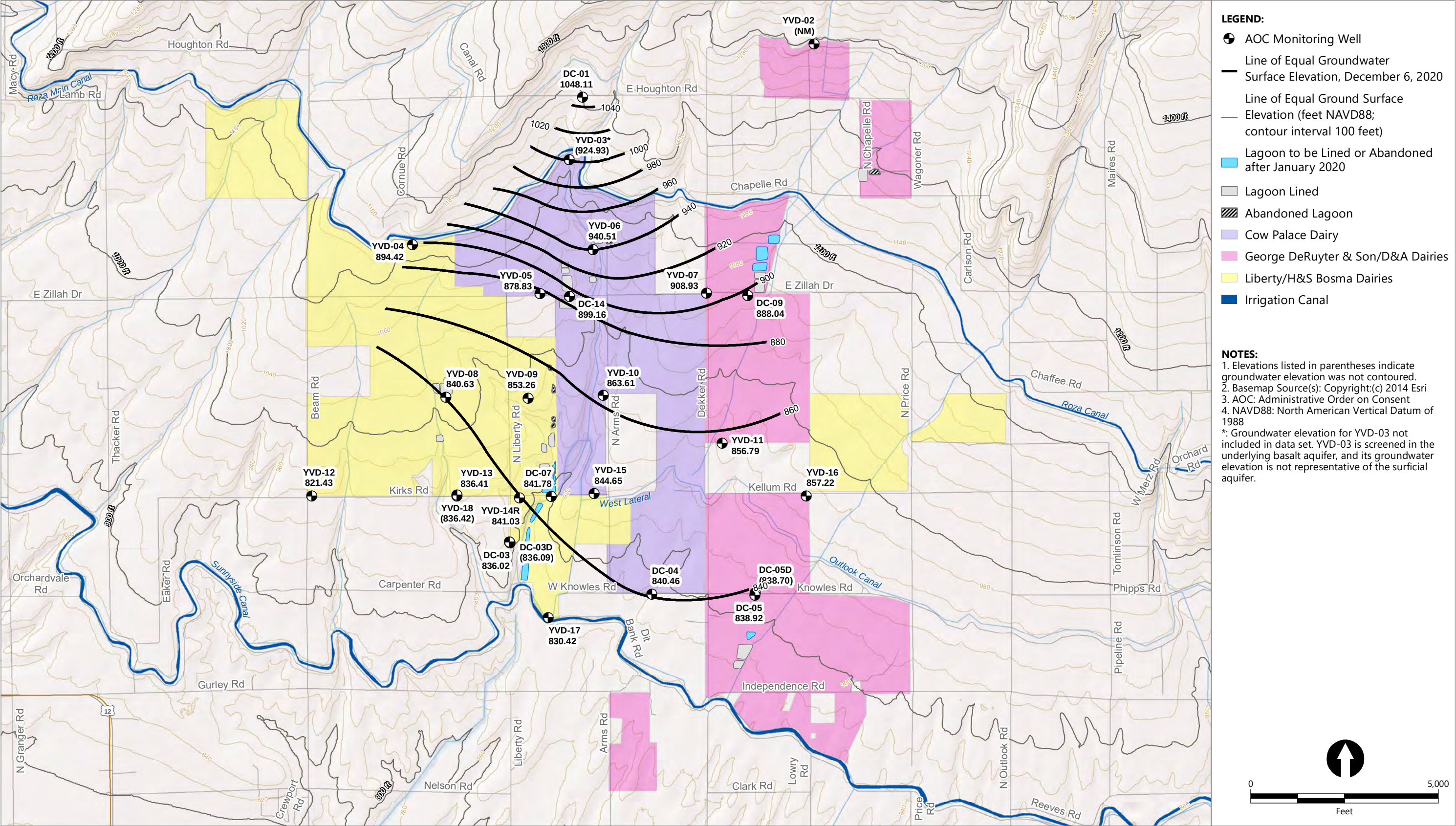
Figure 15 Surficial Aquifer Groundwater Elevation Contour Map Fourth Quarter 2020 Groundwater Monitoring Data Report – Fourth Quarter 2020 Yakima Valley Dairies
