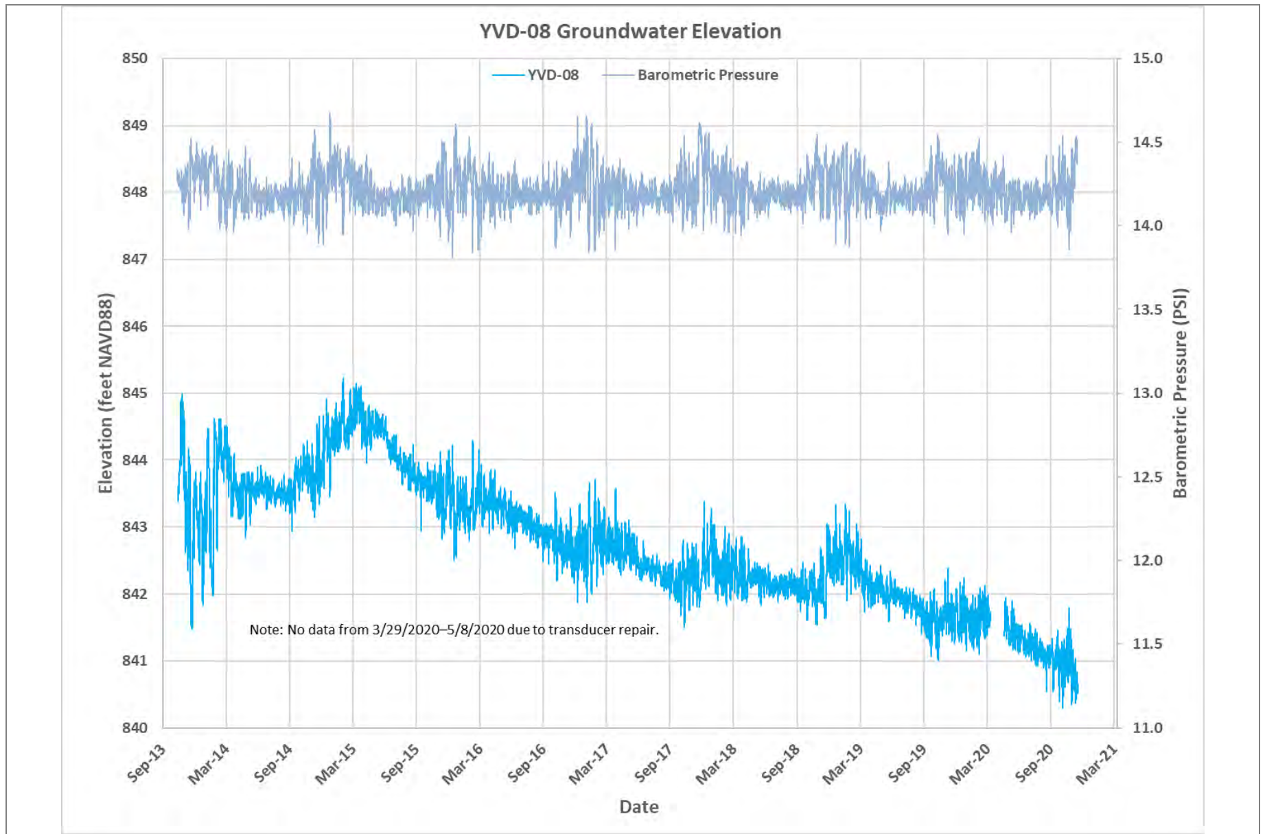
Figure 16F Groundwater Hydrographs – YVD-08 Groundwater Monitoring Data Report – Fourth Quarter 2020 Yakima Valley Dairies
