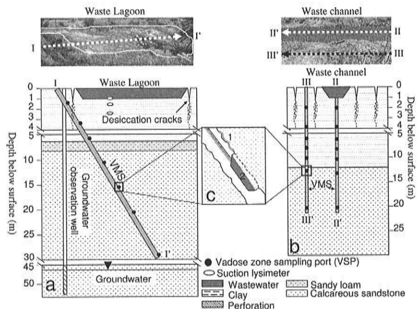
Fig. 1. Schematic illustration of the vadose zone monitoring systems (VMS) and observation well installed in the sediment profile under (a) the waste lagoon and its margins, and (b) the waste channel and its margins. The monitoring units (c) include (1) a flexible time domain reflectometry (FTDR) probe, and (2) a vadose zone porewater sampling port (VSP). (a) shows a side view of the waste lagoon while (b) shows a front view of the waste channel, and thus VMSs II and III appear as vertical lines in (b) although they were installed in slanted boreholes.
