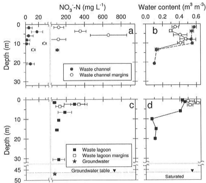
Fig. 5. Vertical distribution of (a) \text{NO}_3^- -N concentrations in porewater from the vadose zone beneath the waste channel and the waste channel margins, and (c) beneath the waste lagoon and the waste lagoon margins. Vertical sediment water content profiles represent the average value measured by the flexible time domain reflectometry probes (b) under the channel and its margins and (d) under the lagoon and its margins. Concentrations in the groundwater presented at 47 m. Results are presented as averages and the horizontal bars are the standard deviation. Transition from clay to sand/loam occurs at 6 m below land surface under the lagoon and at 12 m under the channel (Fig. 1).
