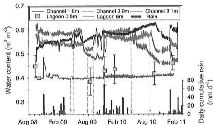
Fig. 3. Temporal changes in sediment water content measured by flexible time domain reflectometry probes under the waste channel and waste lagoon (continuous lines) and by gravimetric methods on sediment cores (squares), along with daily cumulative rain events during 2008–2011 (bars). Dashed arrows indicate events in which sharp increases in sediment water content were not associated with rainstorms.
