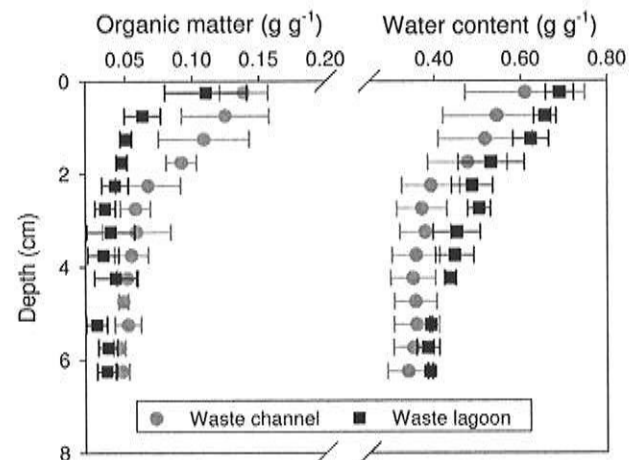
Fig. 2. Organic matter content and water content in the sediments under the waste channel and the waste lagoon. Results are presented as averages, and the horizontal bars are the standard deviation.
