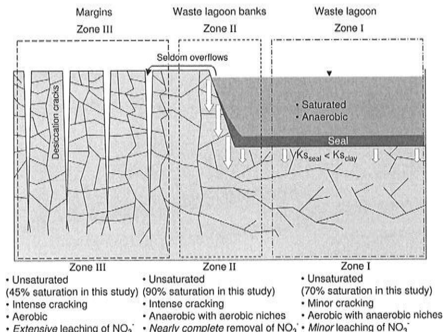
Fig. 7. Conceptual model (not to scale) of the three zones of a waste lagoon constructed in clay sediment, the governing seepage mechanisms, and the resulting fate of the N species in the subsurface. Zone I represents the vadose zone under the center of the waste lagoon (away from the banks); Zone II represents the banks of the waste lagoon; and Zone III represents the lagoon margin area, which is subjected to rare flooding events by wastewater overflow and rain events. Small arrows represent continuous slow ( \text{mm d}^{-1} ) infiltration flux and long arrows represent preferential infiltration via the desiccation-crack network. Relative saturation (%) is the ratio between the measured water content and the water content at saturation.
