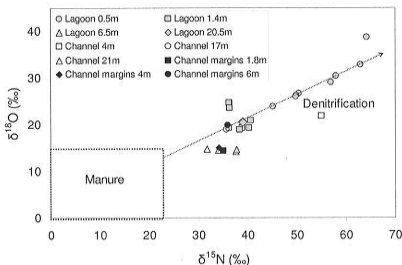
Fig. 6. Isotopic composition of \text{NO}_3^- ( \delta^{15}\text{N} and \delta^{18}\text{O} ) in the propagating porewater from the vadose zone beneath the waste lagoon, waste channel, and their margins. The isotopic composition of dairy manure is based on Kendall (1998).
