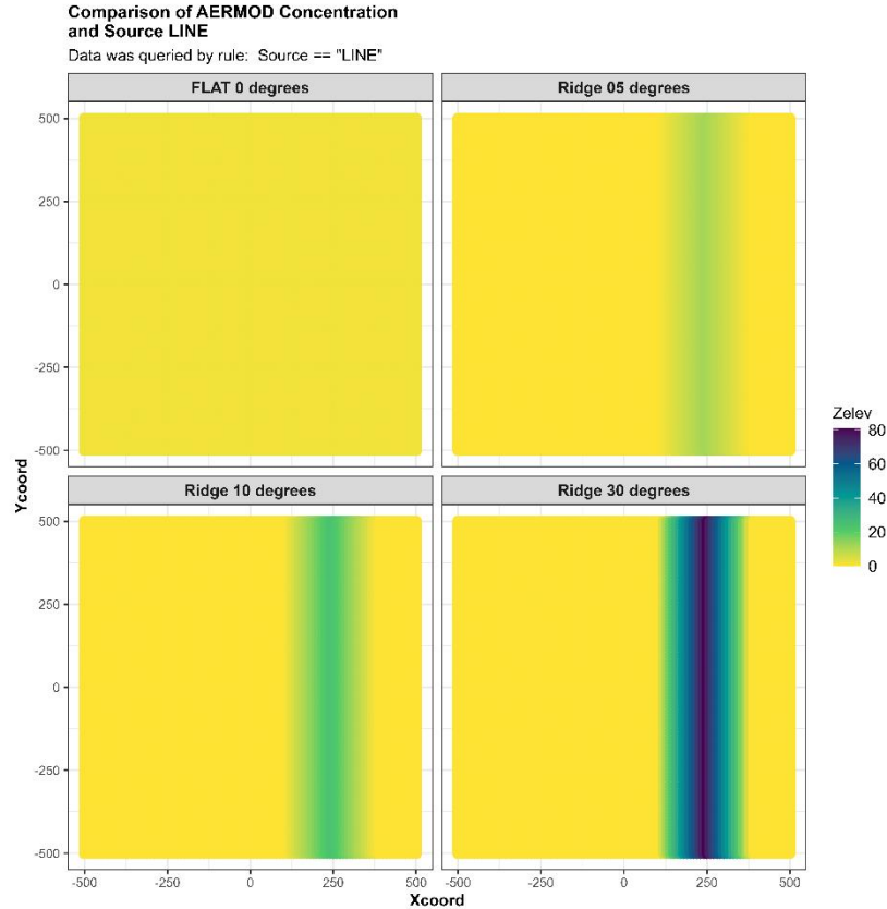
Figure 4: Terrain elevation (Zelev) for all receptor grids and slope angles examined.
