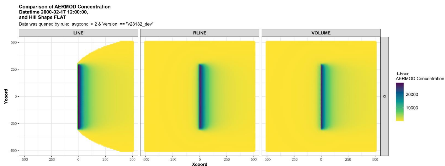
Figure 9: Spatial plot of the LINE, RLINE, and VOLUME source types for flat terrain during a convective hour
