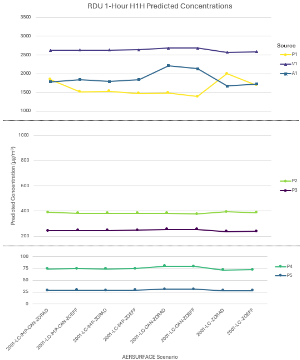
Figure 11-41. RDU H1H Predicted Concentrations by AERSURFACE Scenario and Emission Source
