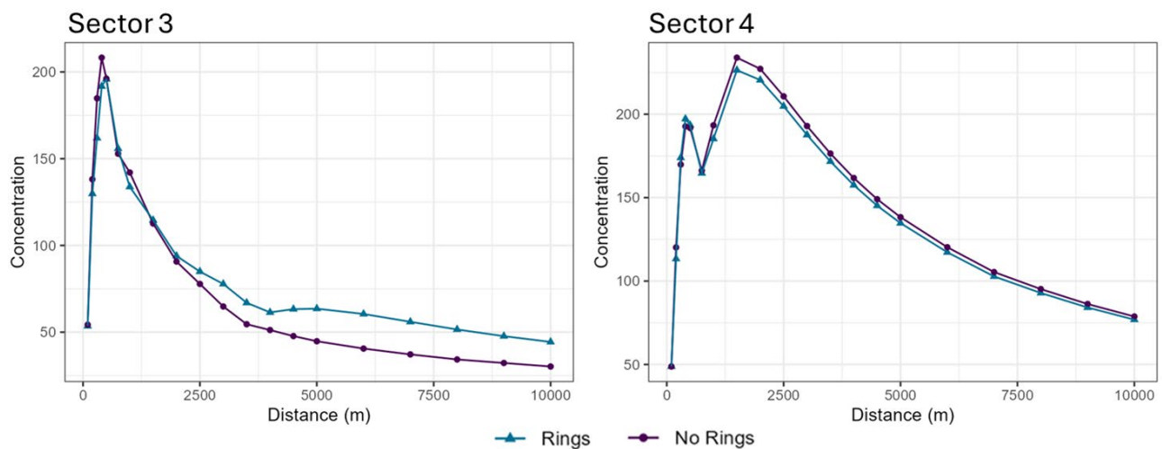
Figure 12-9 H1H for receptors downwind of AERSURFACE sector 3 (left) and sector 4 (right) for point source 3 (P3) for the scenarios with rings (light blue, triangle) and without rings (dark blue, circle).
