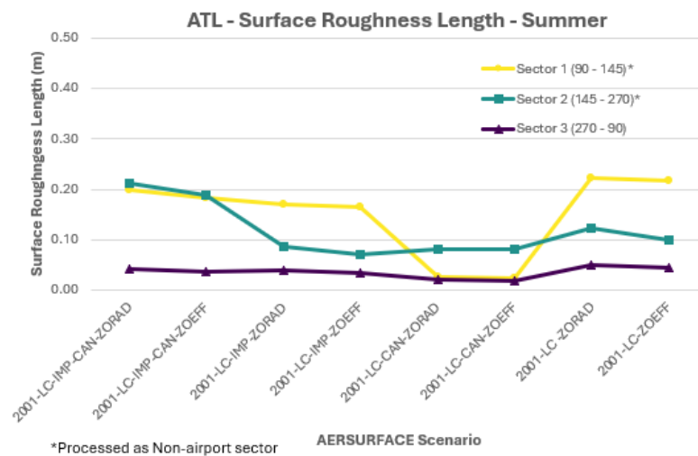
Figure 11-11. ATL Surface Roughness Length by Season, Sector, and AERSURFACE Scenario
