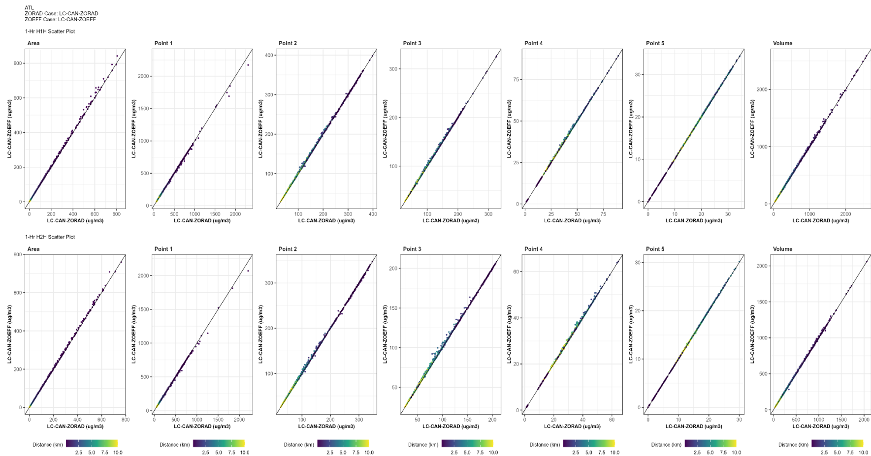
Figure 11-22. ATL, Scatter Plots, H1H and H2H at each Receptor, 2001 LC-CAN-ZORAD Vs. 2001 LC-CAN-ZOEFF
