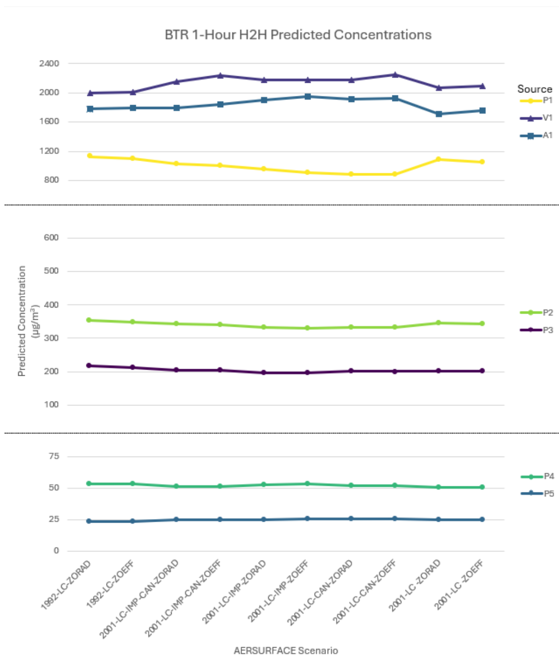
Figure 11-26. BTR H2H Predicted Concentrations by AERSURFACE Scenario and Emission Source
