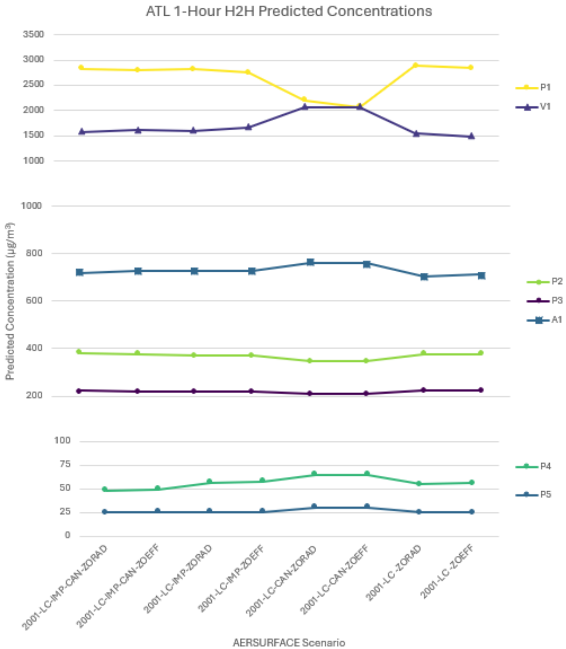
Figure 11-13. ATL H2H Predicted Concentrations by AERSURFACE Scenario and Emission Source
