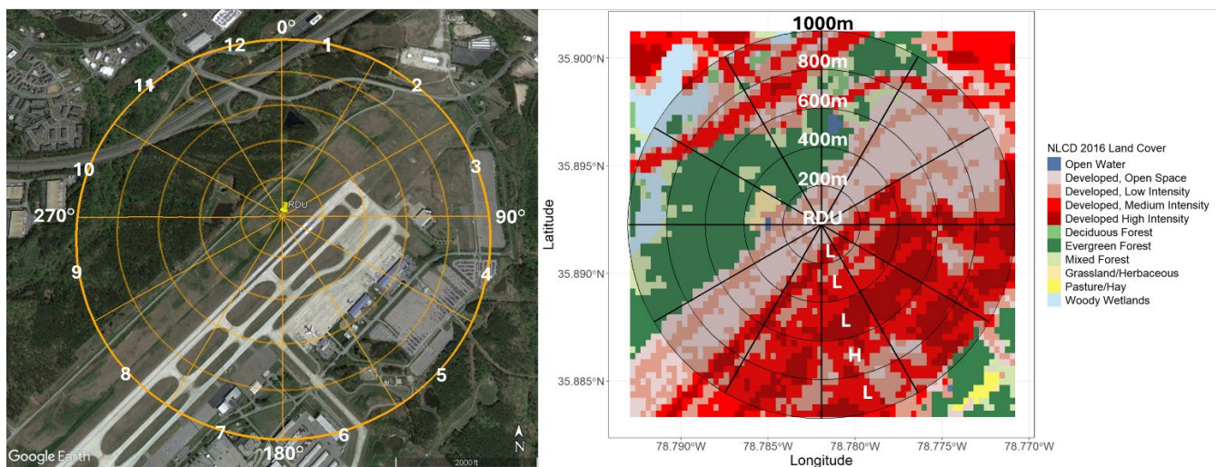
Figure 12-1 RDU (Raleigh, North Carolina) airport satellite view (left) and 2016 NLCD land cover (right). The 1 km circle around the airport meteorological measurement site is divided into 12, 30° sectors with 200 m annular rings.
