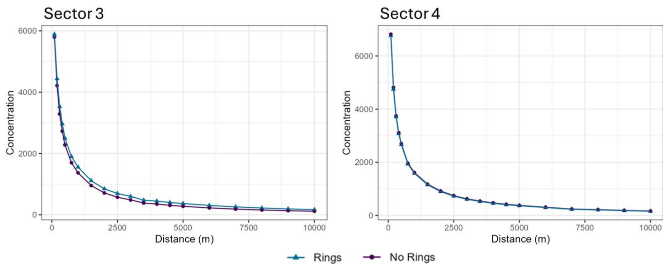
Figure 12-10 H1H for receptors downwind of AERSURFACE sector 3 (left) and sector 4 (right) for volume source (V1) for the scenarios with rings (light blue, triangle) and without rings (dark blue, circle).
