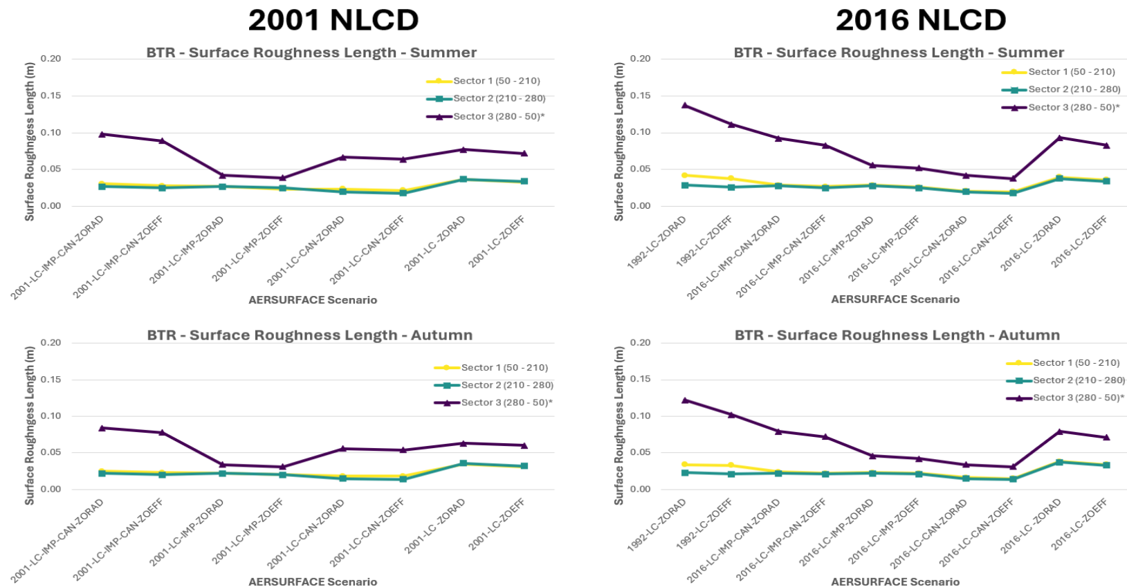
Figure 11-58. Surface Roughness Length Estimated for BTR using 2001 NLCD (2011 Edition) and 2016 NLCD Summer Months (top), Autumn Months (bottom)
