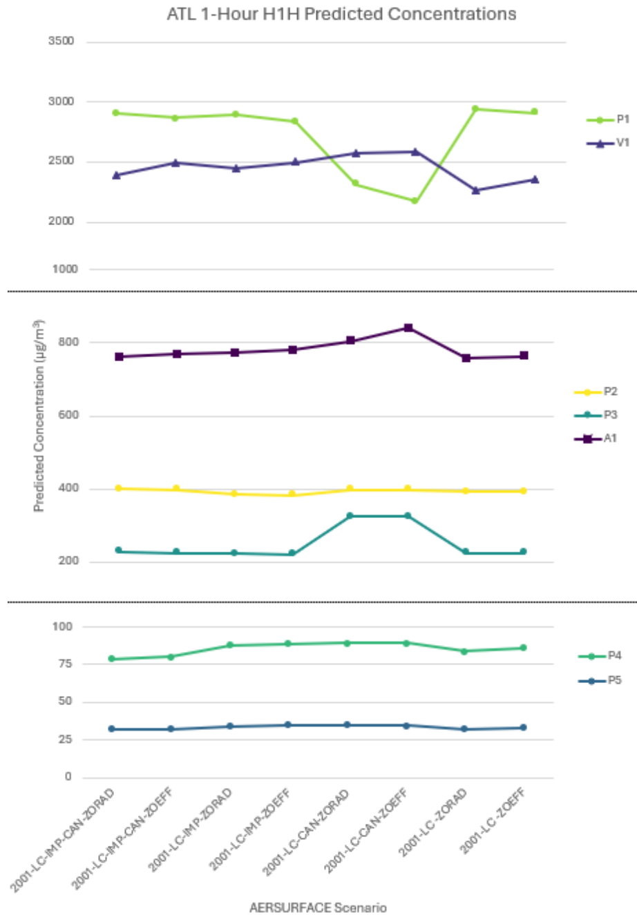
Figure 11-12. ATL H1H Predicted Concentrations by AERSURFACE Scenario and Emission Source
