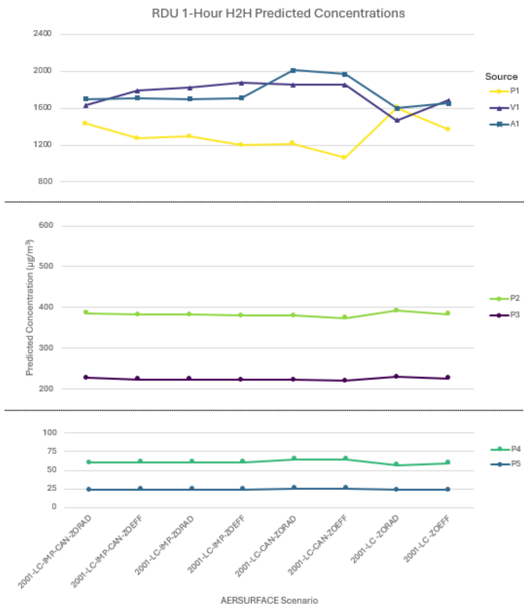
Figure 11-42. RDU H2H Predicted Concentrations by AERSURFACE Scenario and Emission Source
