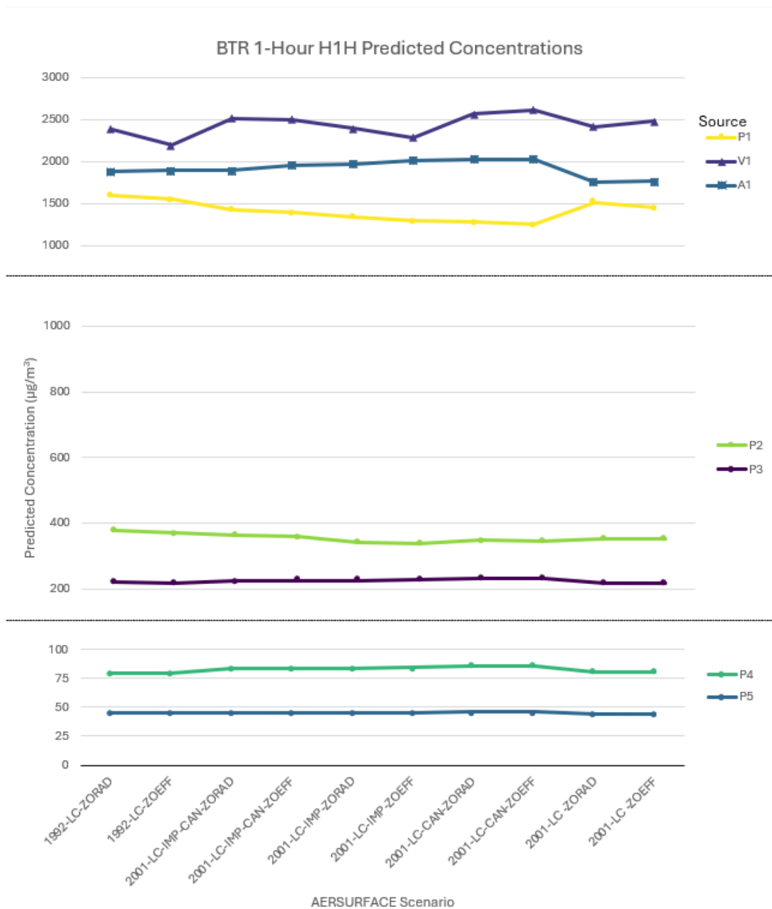
Figure 11-25. BTR H1H Predicted Concentrations by AERSURFACE Scenario and Emission Source
