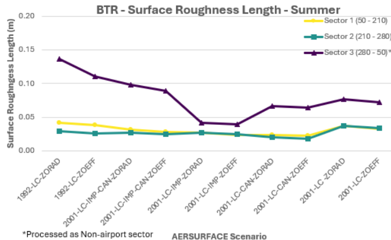
Figure 11-24. BTR Surface Roughness Length by Season, Sector, and AERSURFACE Scenario
