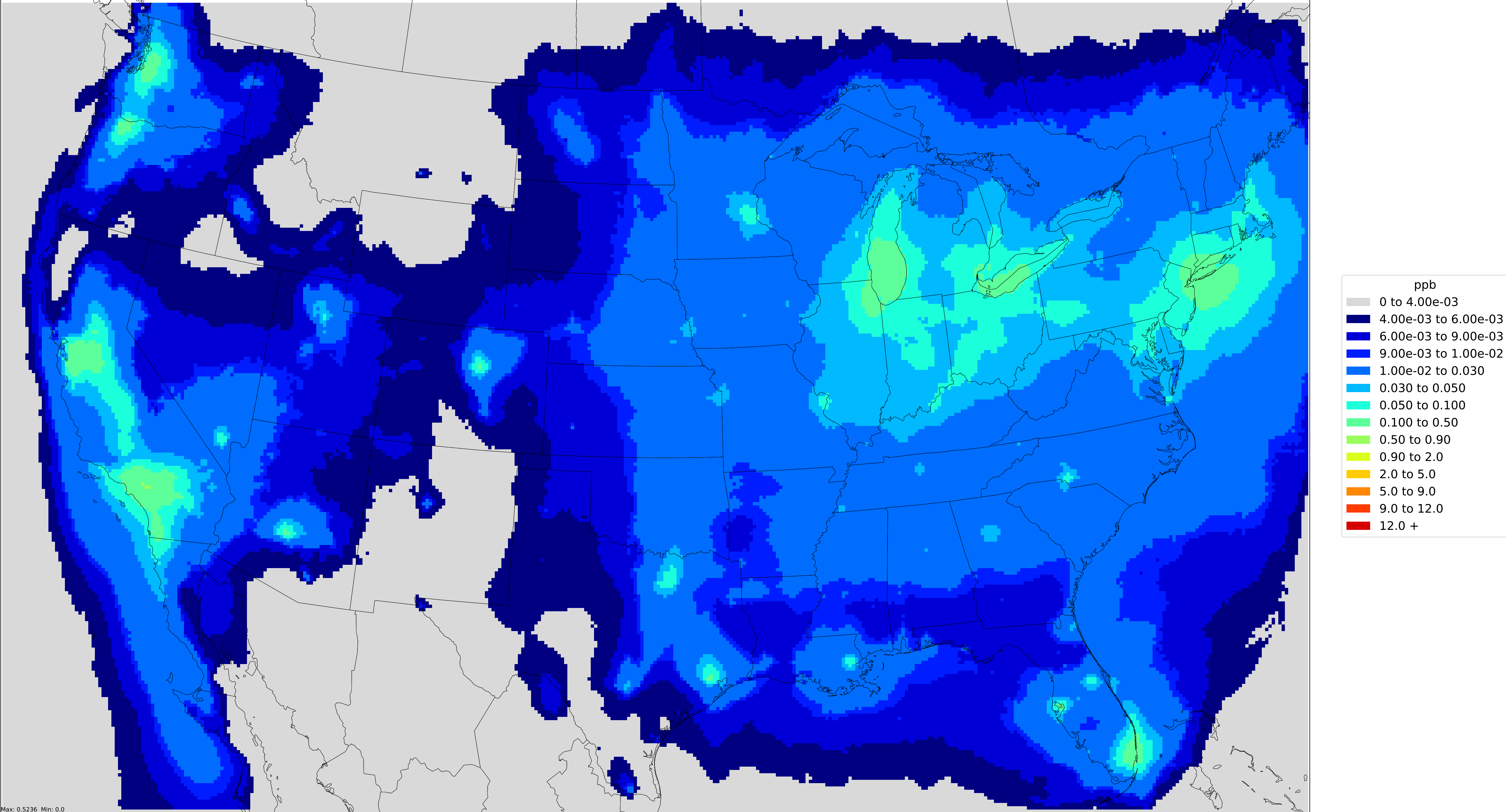
Projected 8-h max Average Seasonal Ozone concentration(ppb) from VOC in 2025 Nonroad Diesel
