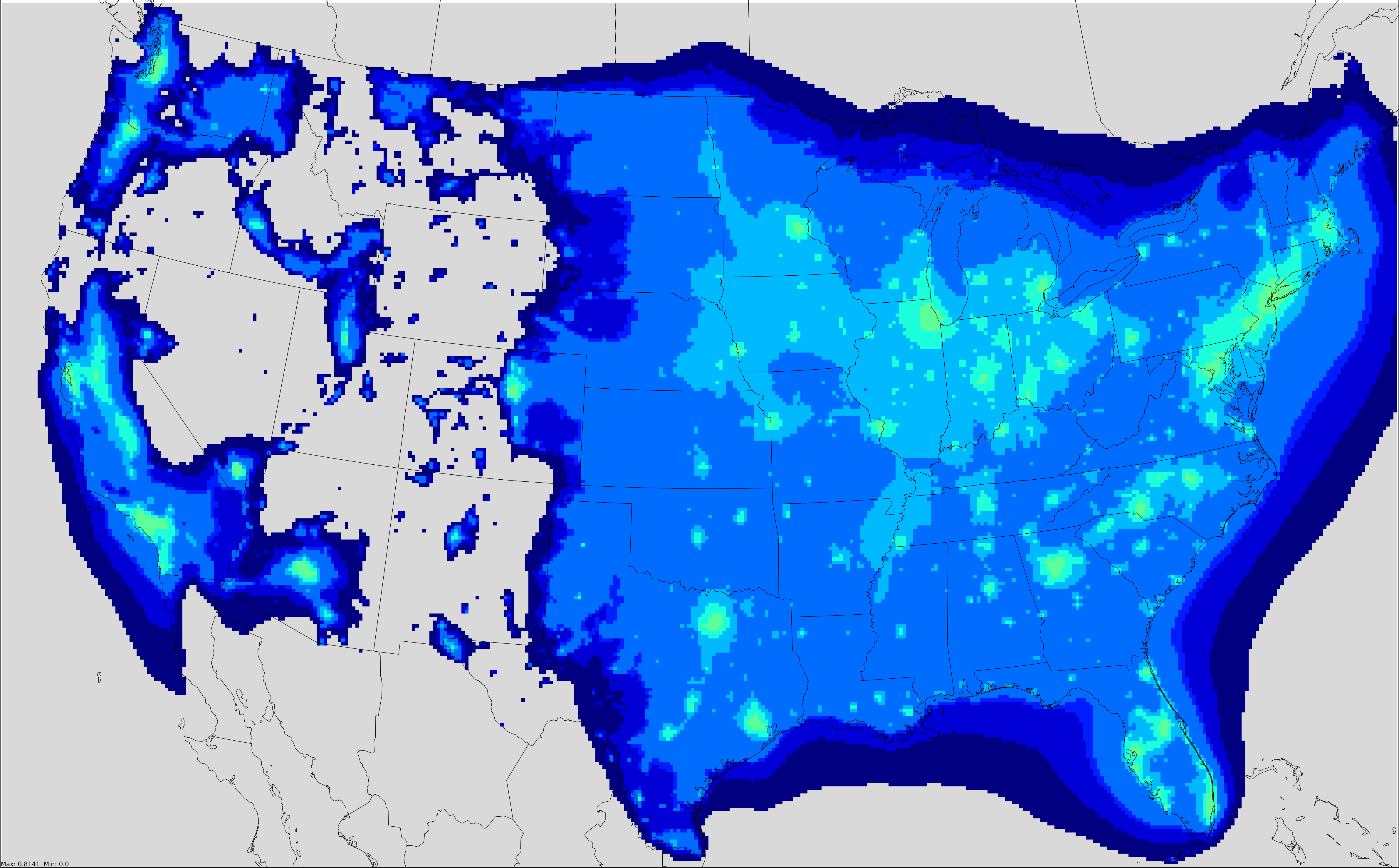
Projected Annual Average Primary PM2.5 concentration(ug/m3) in 2025 Nonroad Diesel
