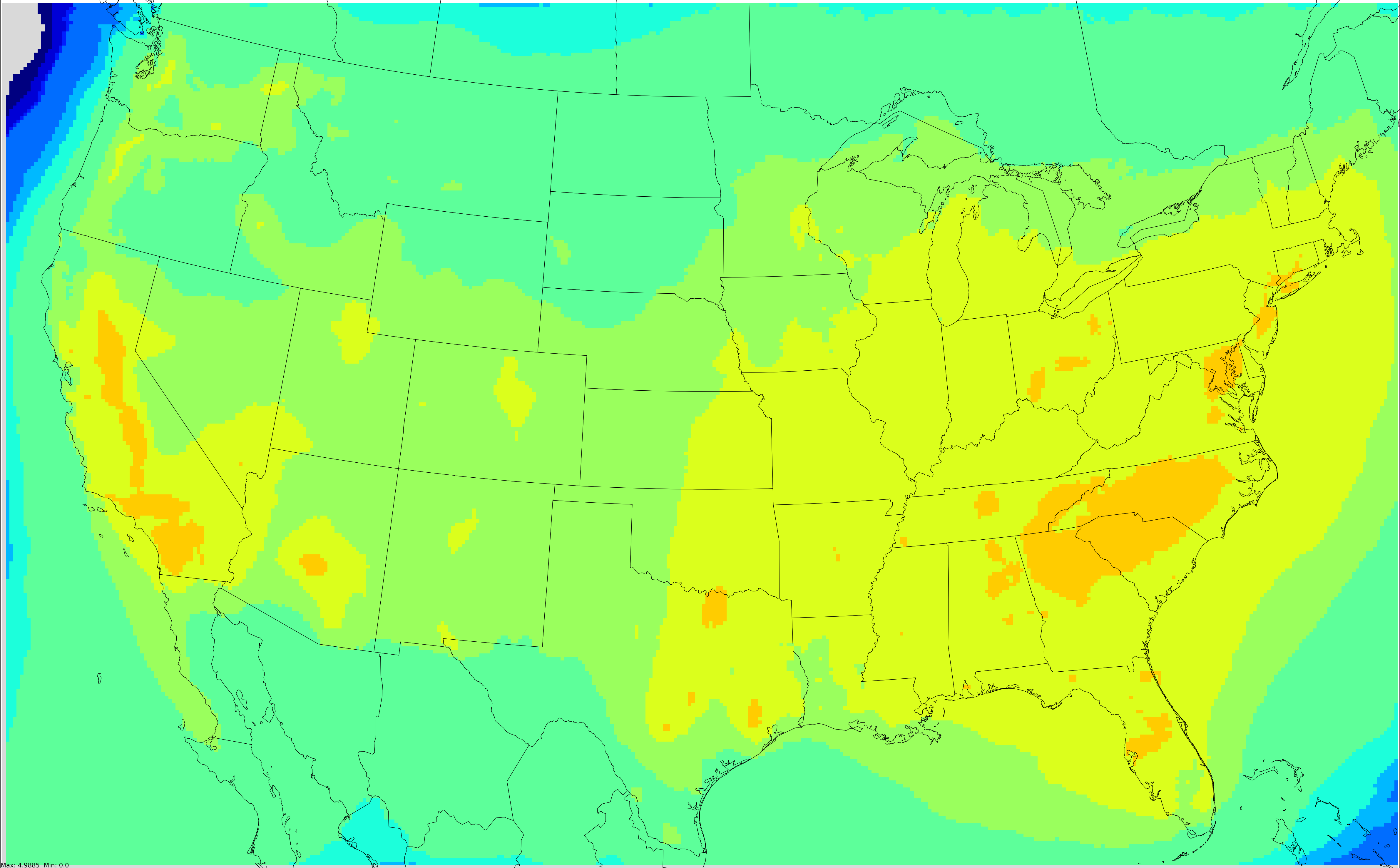
Projected 8-h max Average Seasonal Ozone concentration(ppb) from NOx in 2025 Onroad Light Duty
