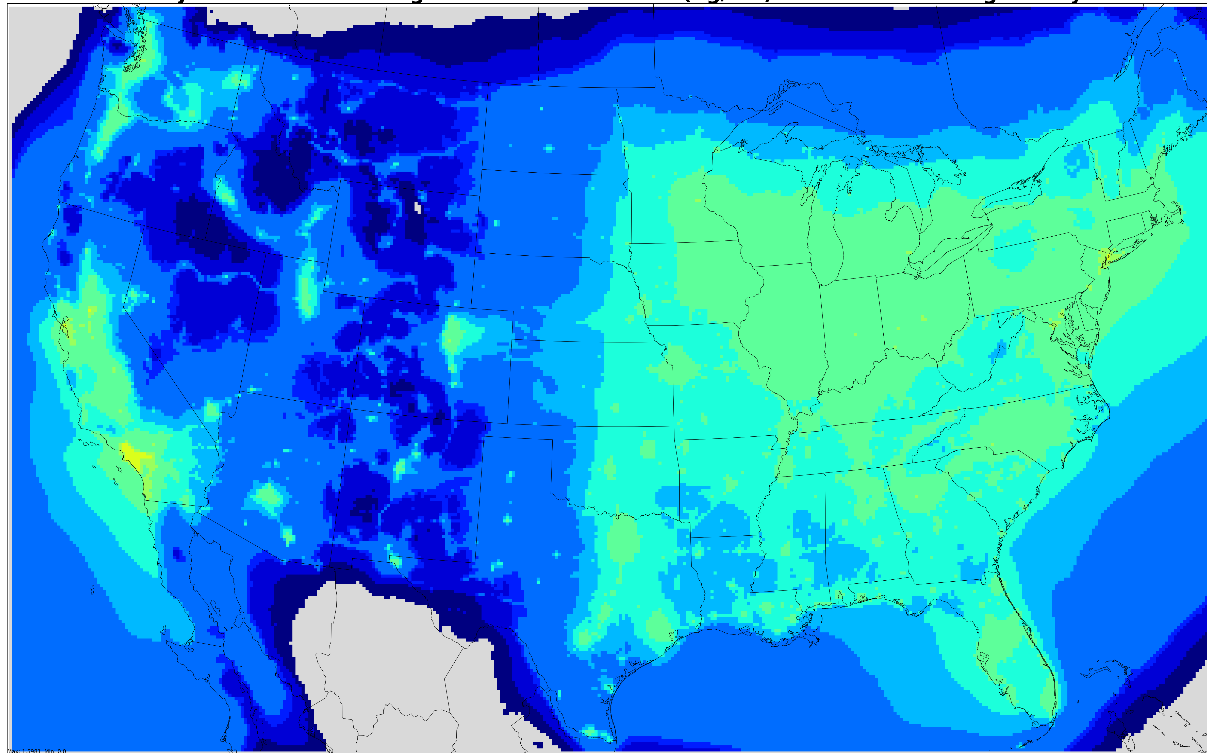
Projected Annual Average PM2.5 concentration(ug/m3) in 2025 Onroad Light Duty
