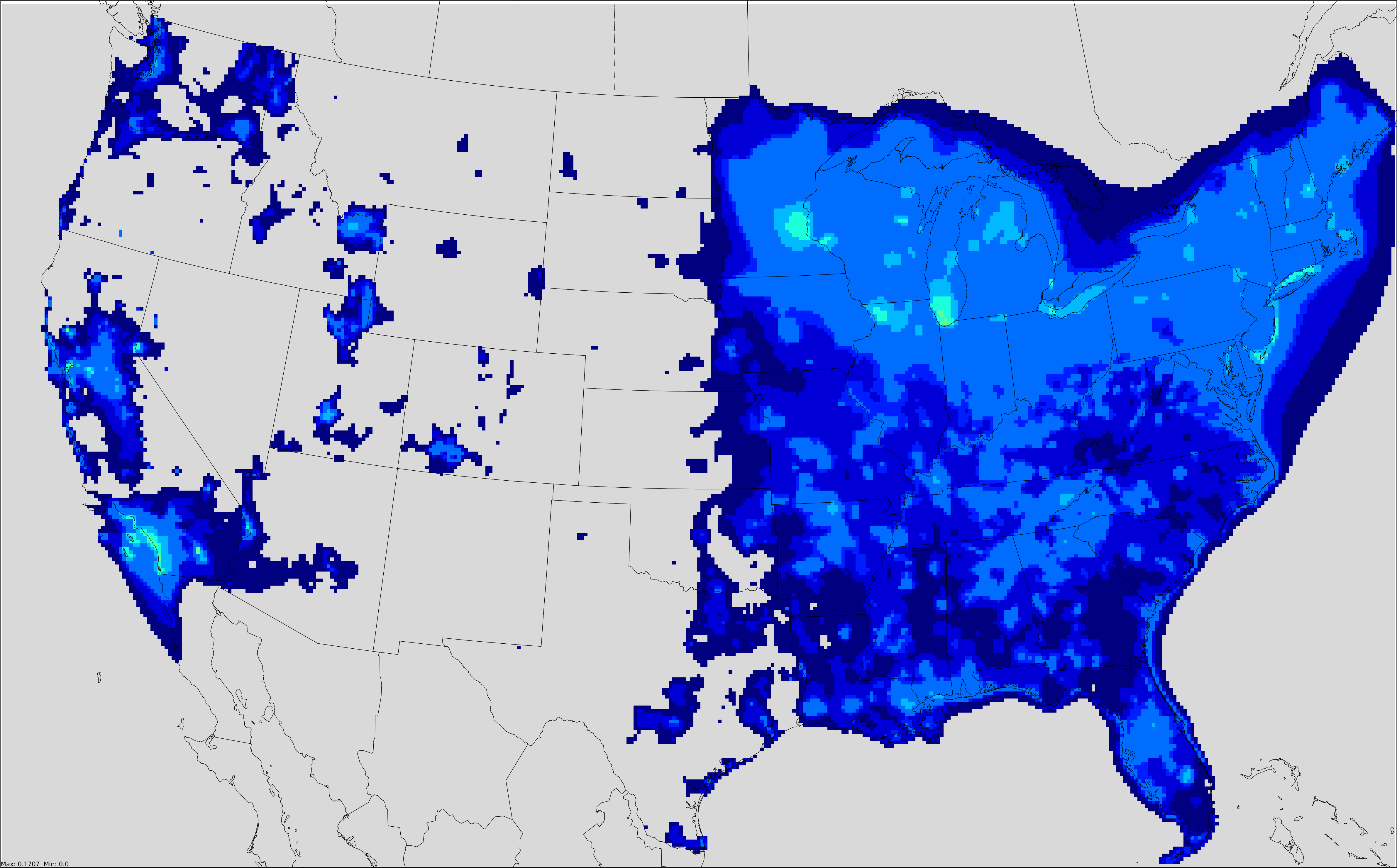
Projected annual average Primary PM2.5 concentration(ug/m3) in 2025 Nonroad recreational
