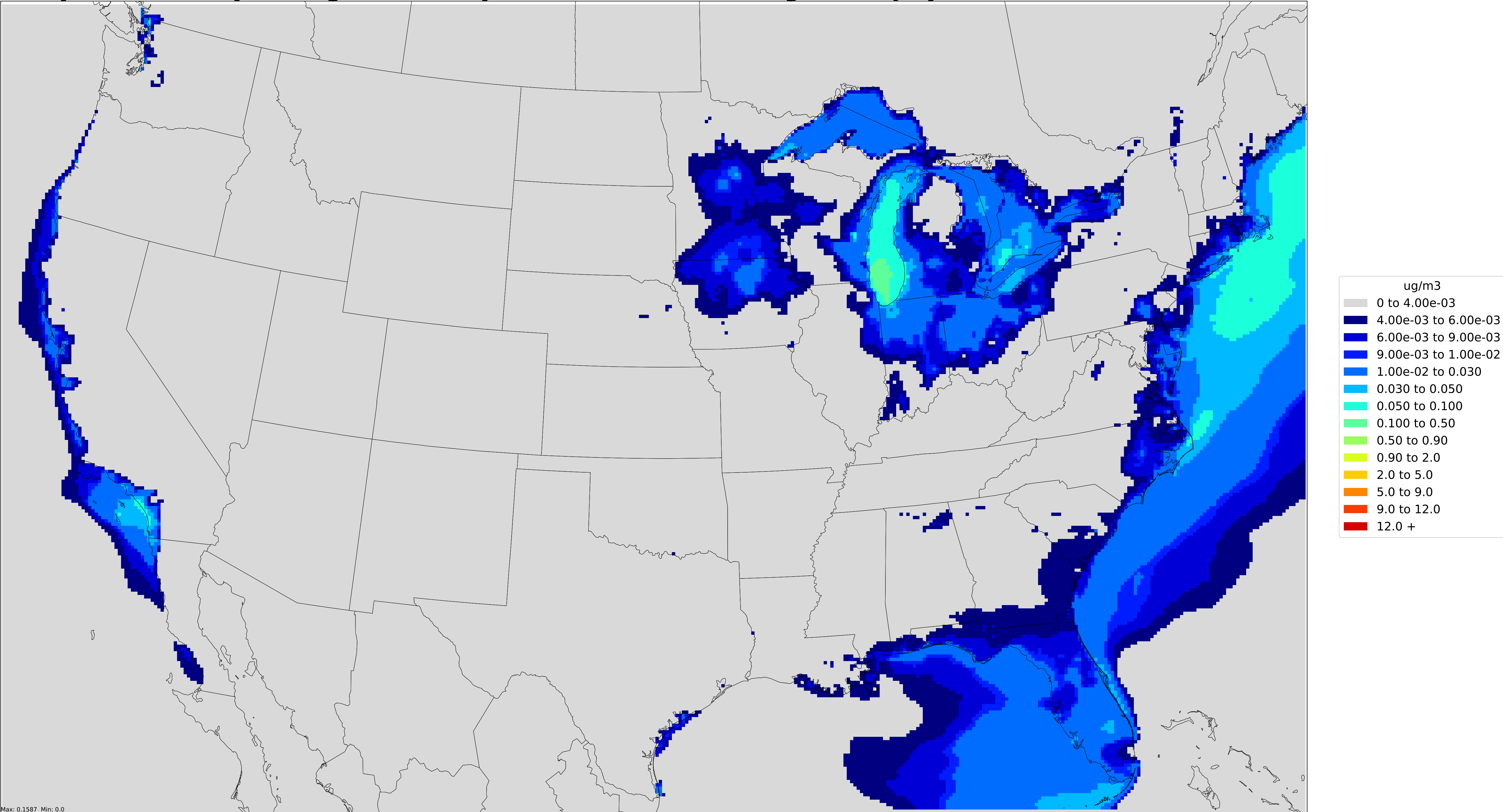
Projected Monthly Average Secondary PM2.5 concentration(ug/m3) in July 2025 Nonroad recreational
