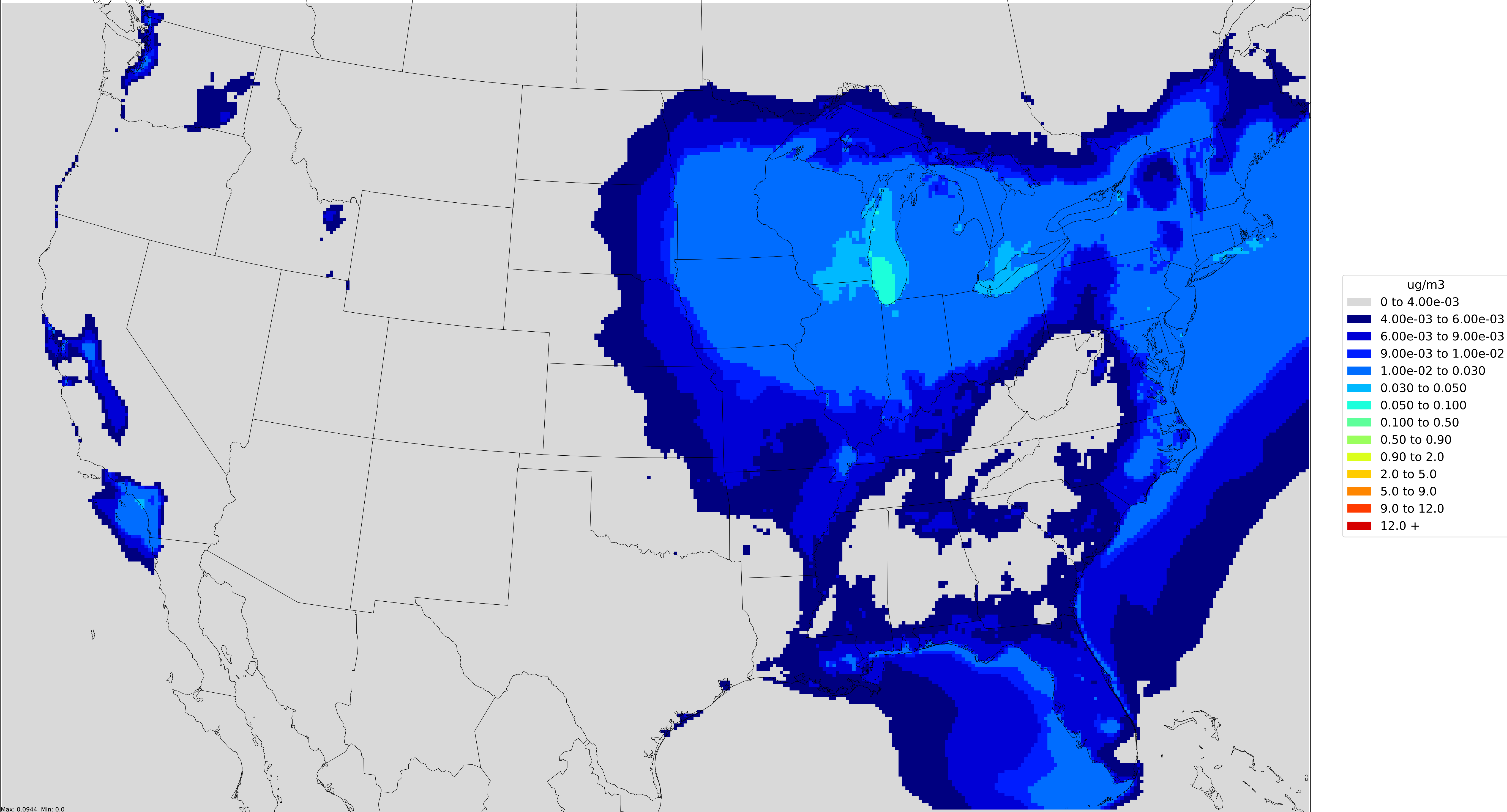
Projected annual average Secondary PM2.5 concentration(ug/m3) in 2025 Nonroad recreational
