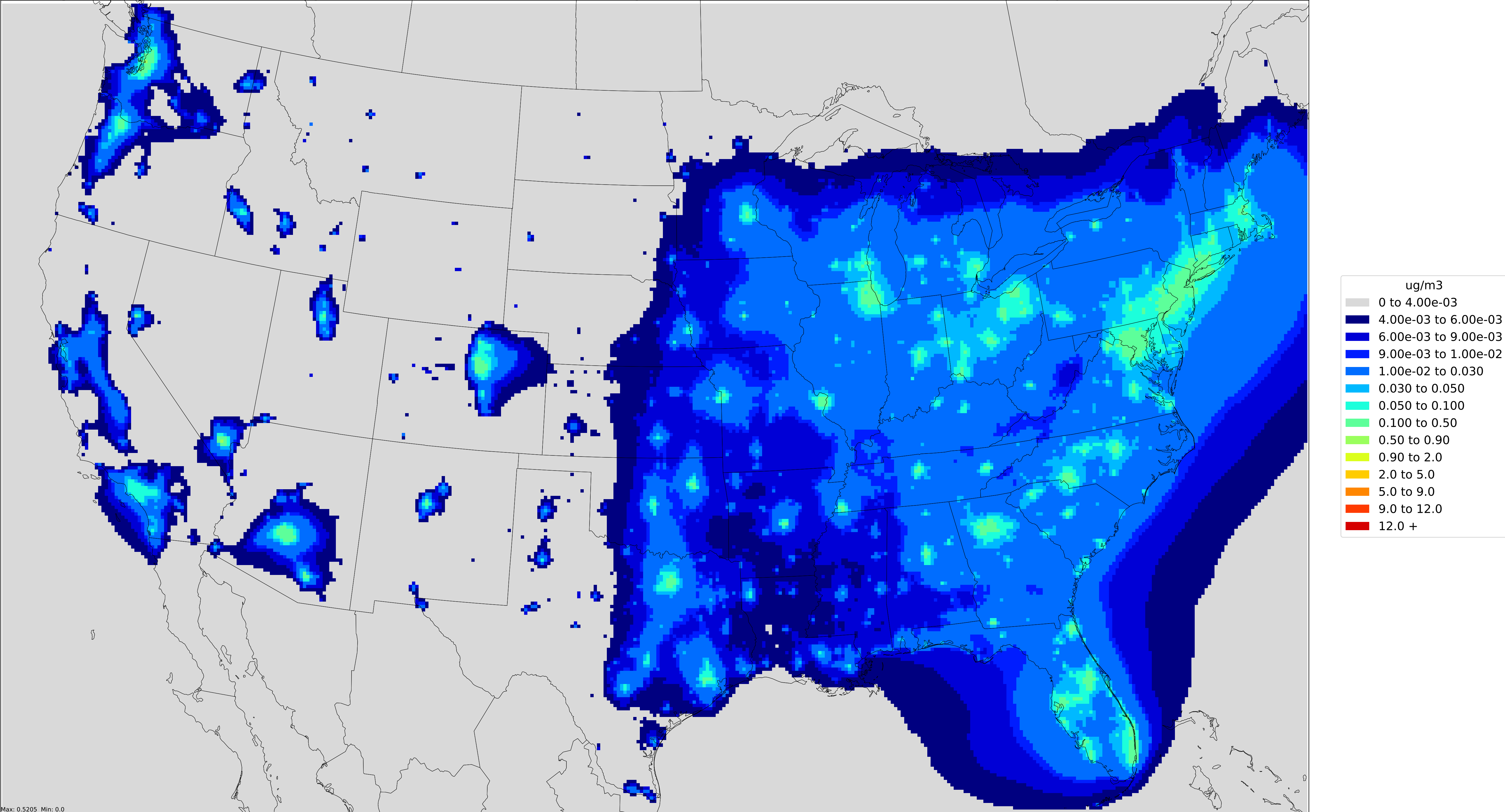
Projected annual average PM2.5 concentration(ug/m3) in 2025 Nonroad lawn and garden commercial
