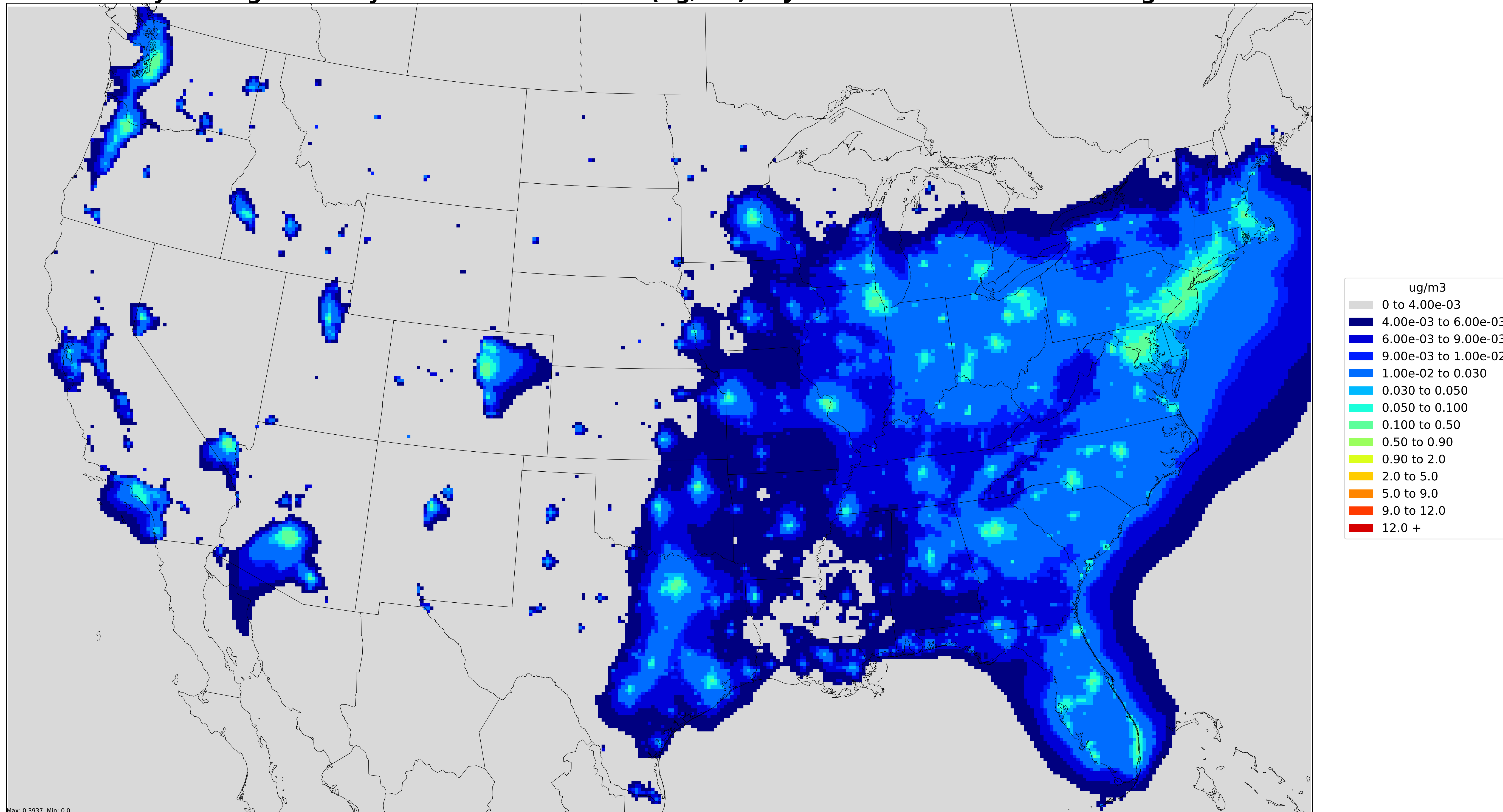
Projected Monthly Average Primary PM2.5 Concentration(ug/m3)in Jan 2025 Nonroad lawn and garden commercial
