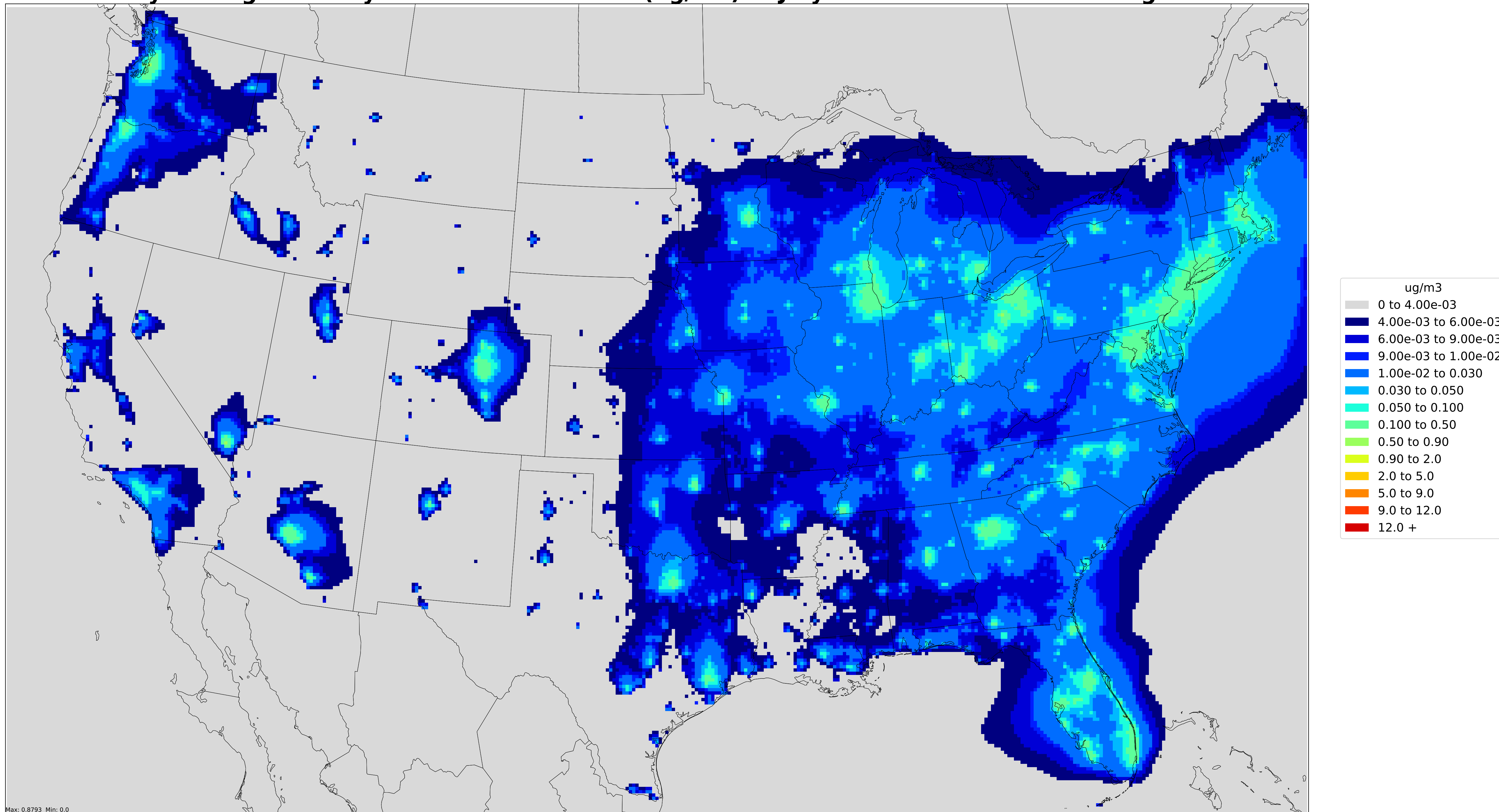
Projected Monthly Average Primary PM2.5 Concentration(ug/m3) in July 2025 Nonroad lawn and garden commercial
