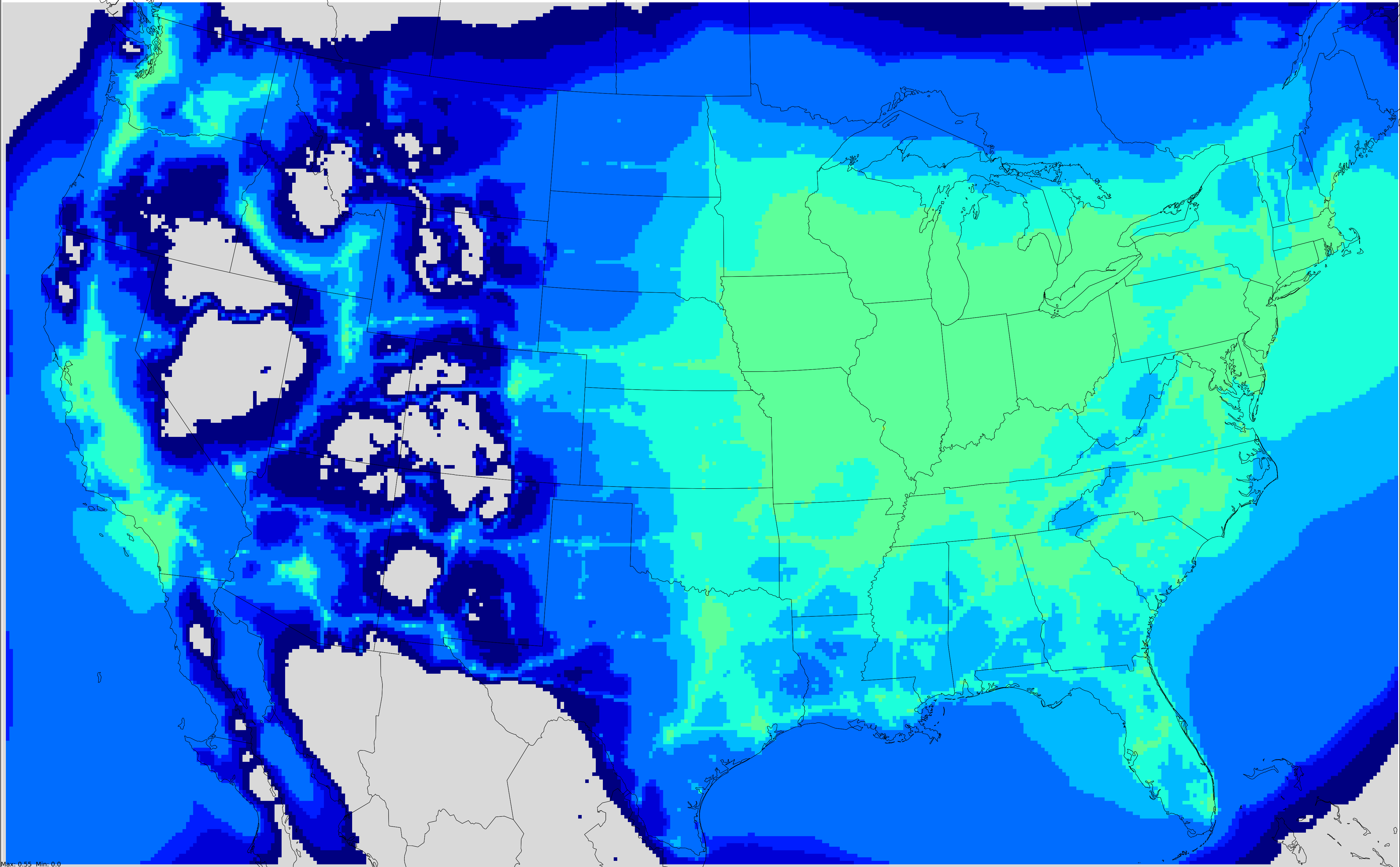
Projected annual average PM2.5 concentration(ug/m3) in 2025 Onroad heavy duty diesel
