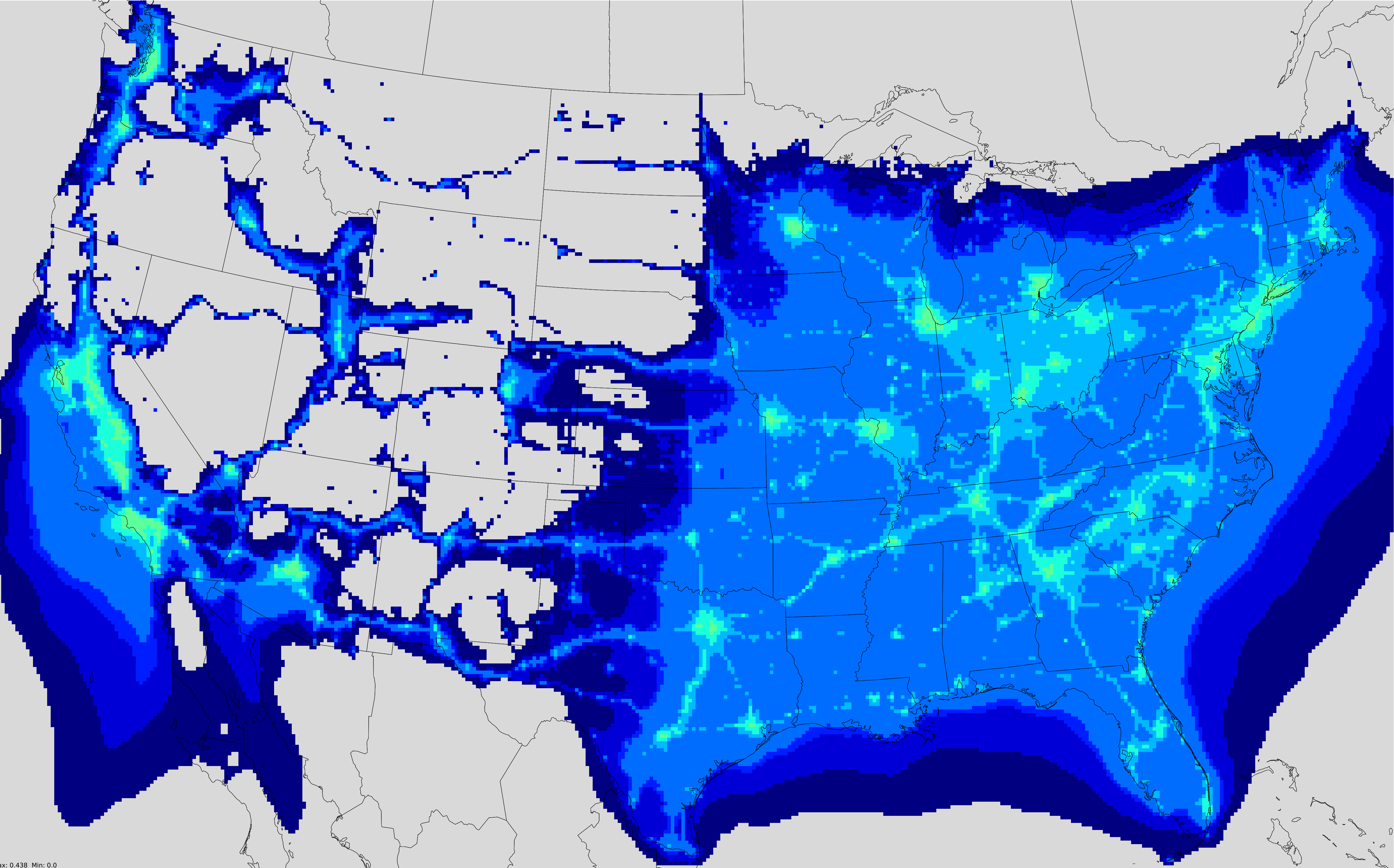
Projected Monthly Average Primary PM2.5 Concentration(ug/m3) in Jan 2025 Onroad heavy duty diesel
