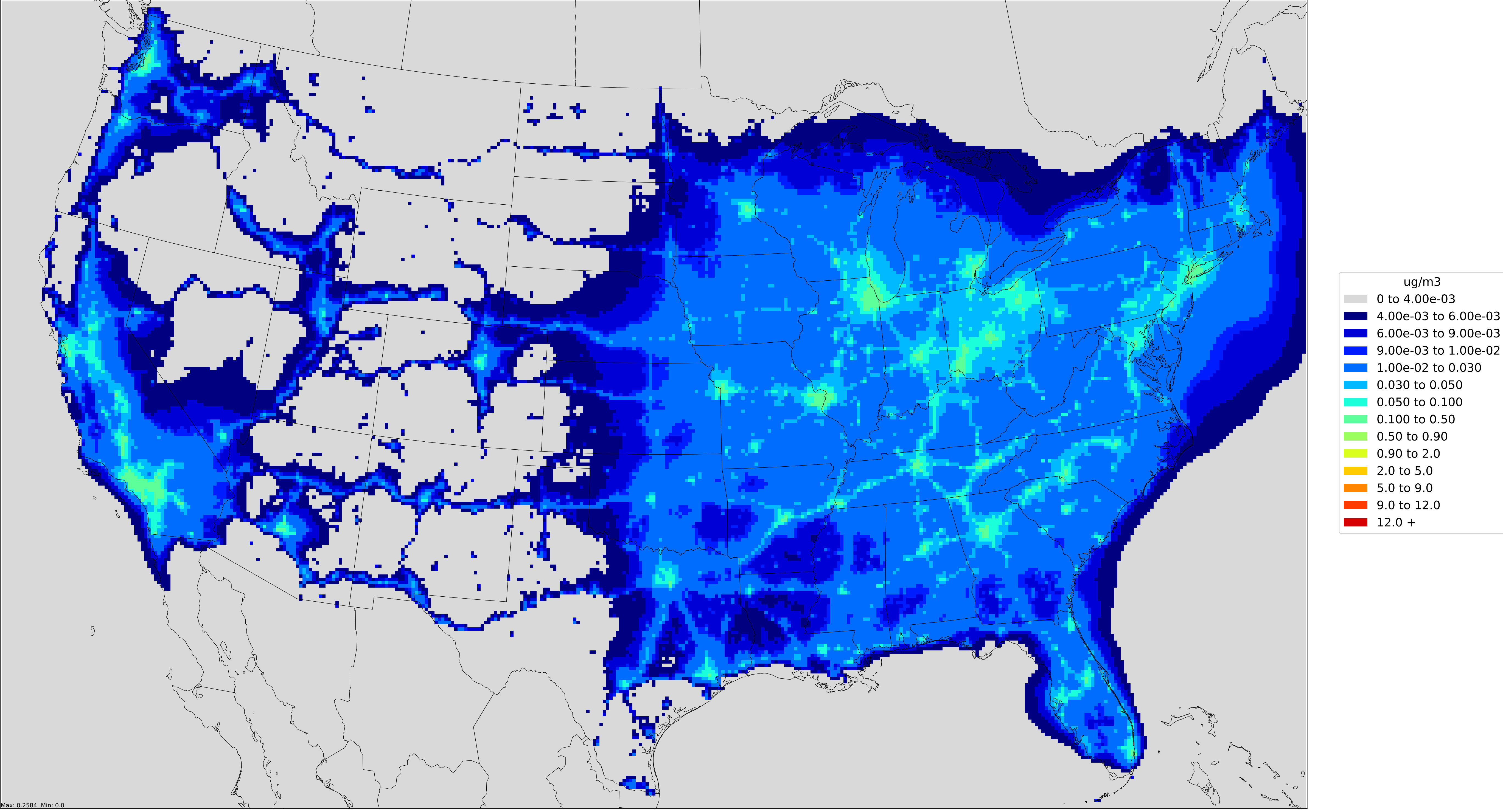
Projected Monthly Average Primary PM2.5 Concentration(ug/m3) in July 2025 Onroad heavy duty diesel
