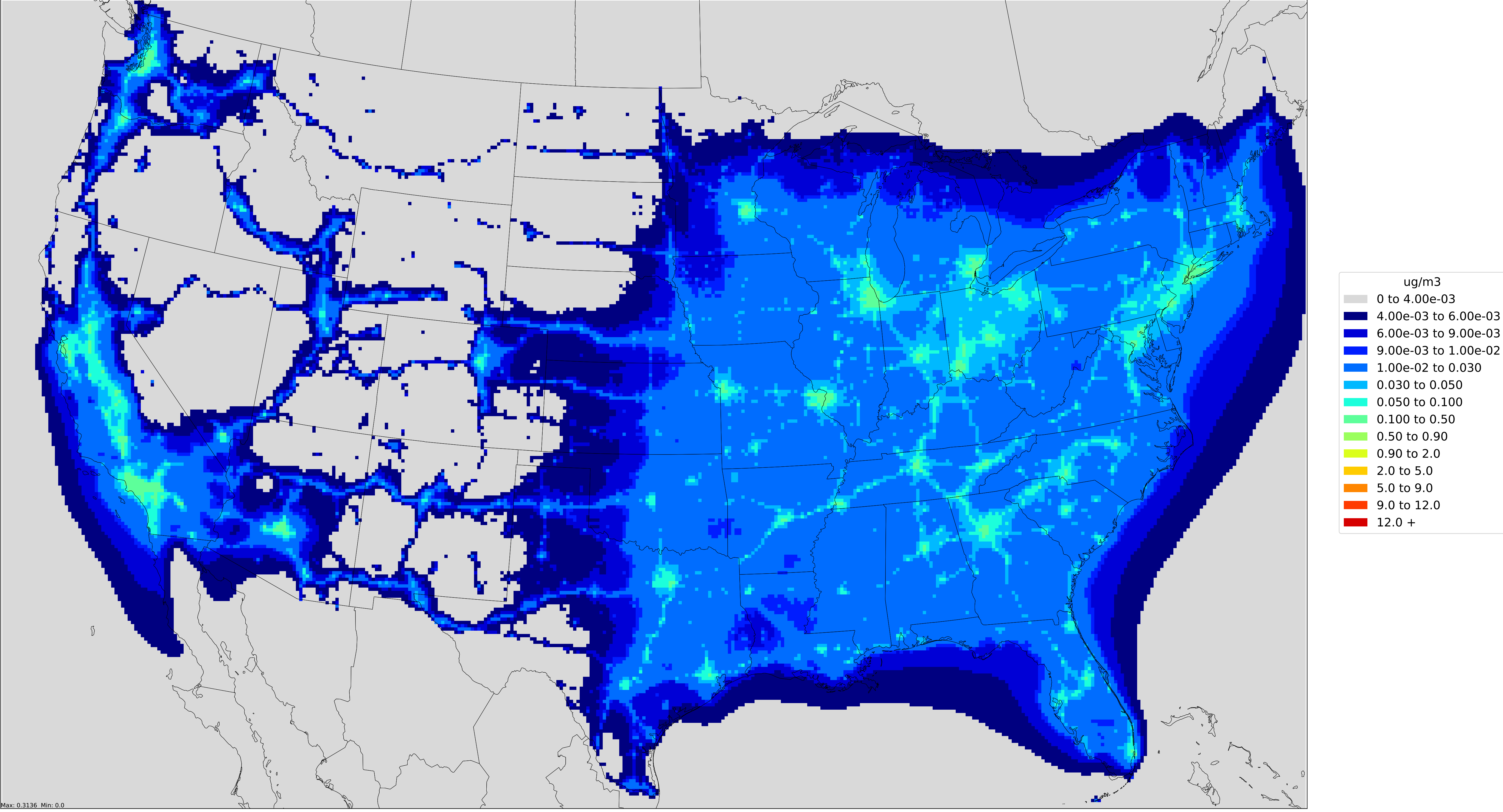
Projected annual average Primary PM2.5 concentration(ug/m3) in 2025 Onroad heavy duty diesel
