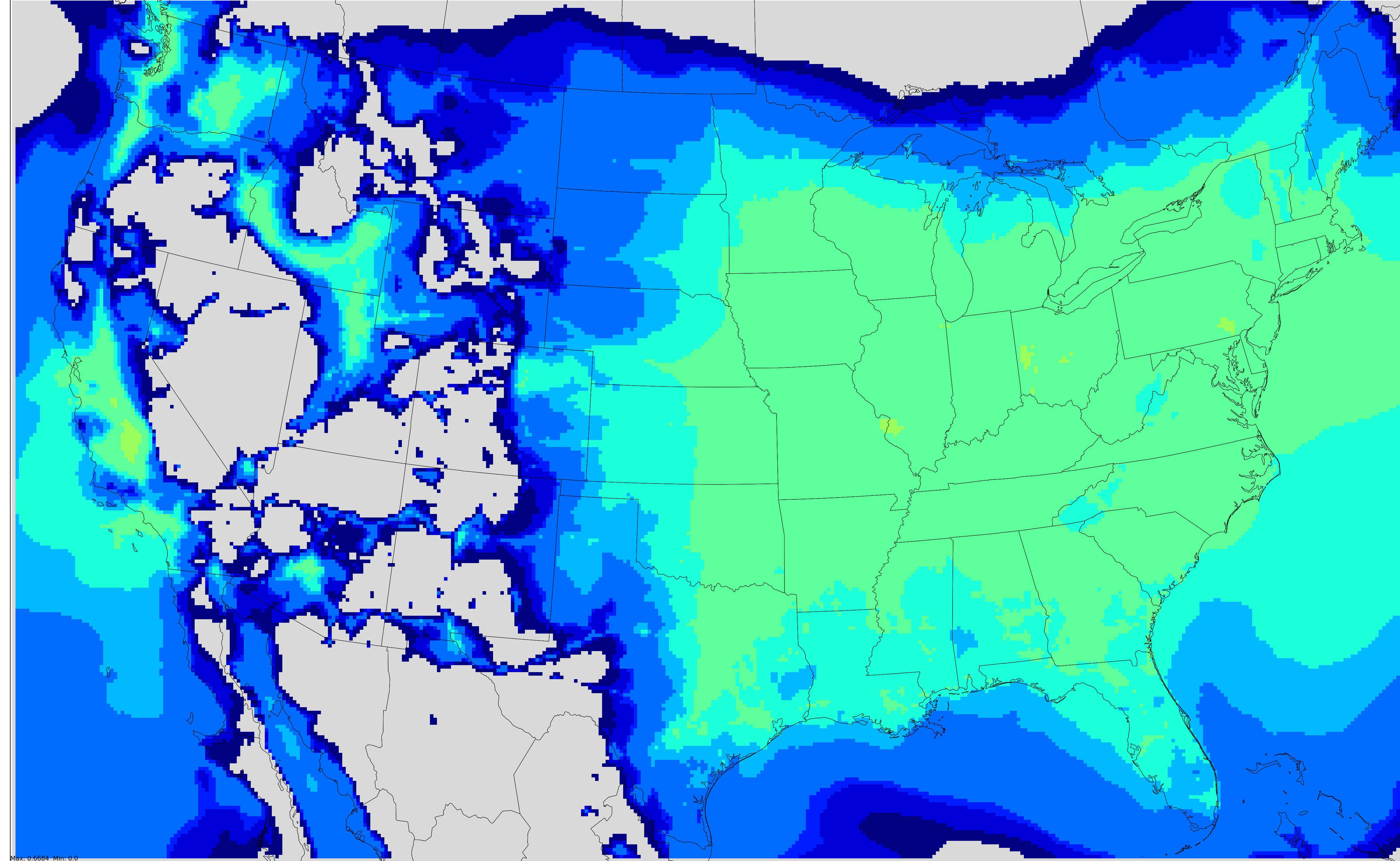
Projected Monthly Average Secondary PM2.5 concentration(ug/m3) in Jan 2025 Onroad heavy duty diesel
