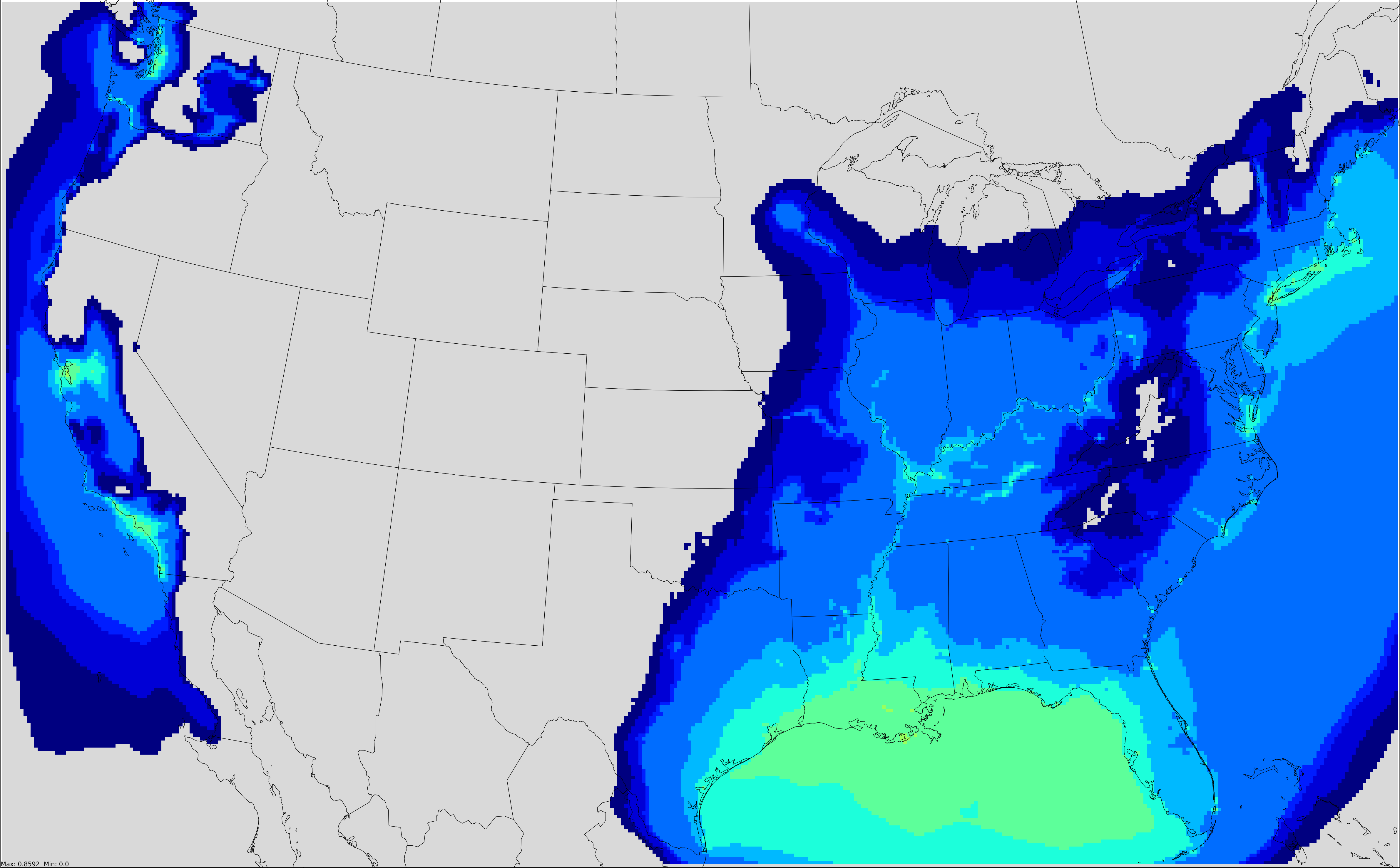
Projected annual average PM2.5 concentration(ug/m3) in 2025 C1C2 marine
