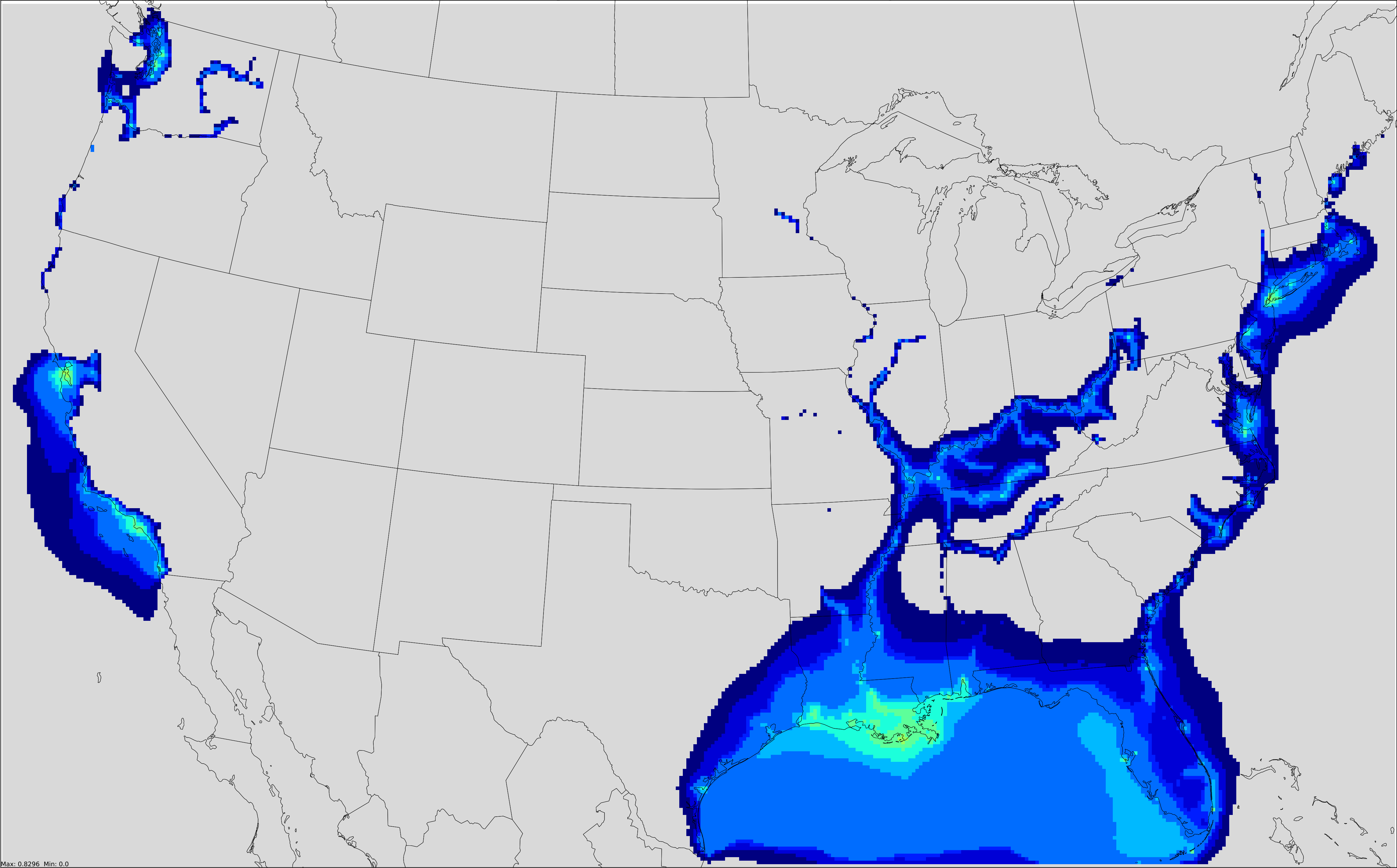
Projected Monthly Average Primary PM2.5 Concentration(ug/m3) in Jan 2025 C1C2 marine
