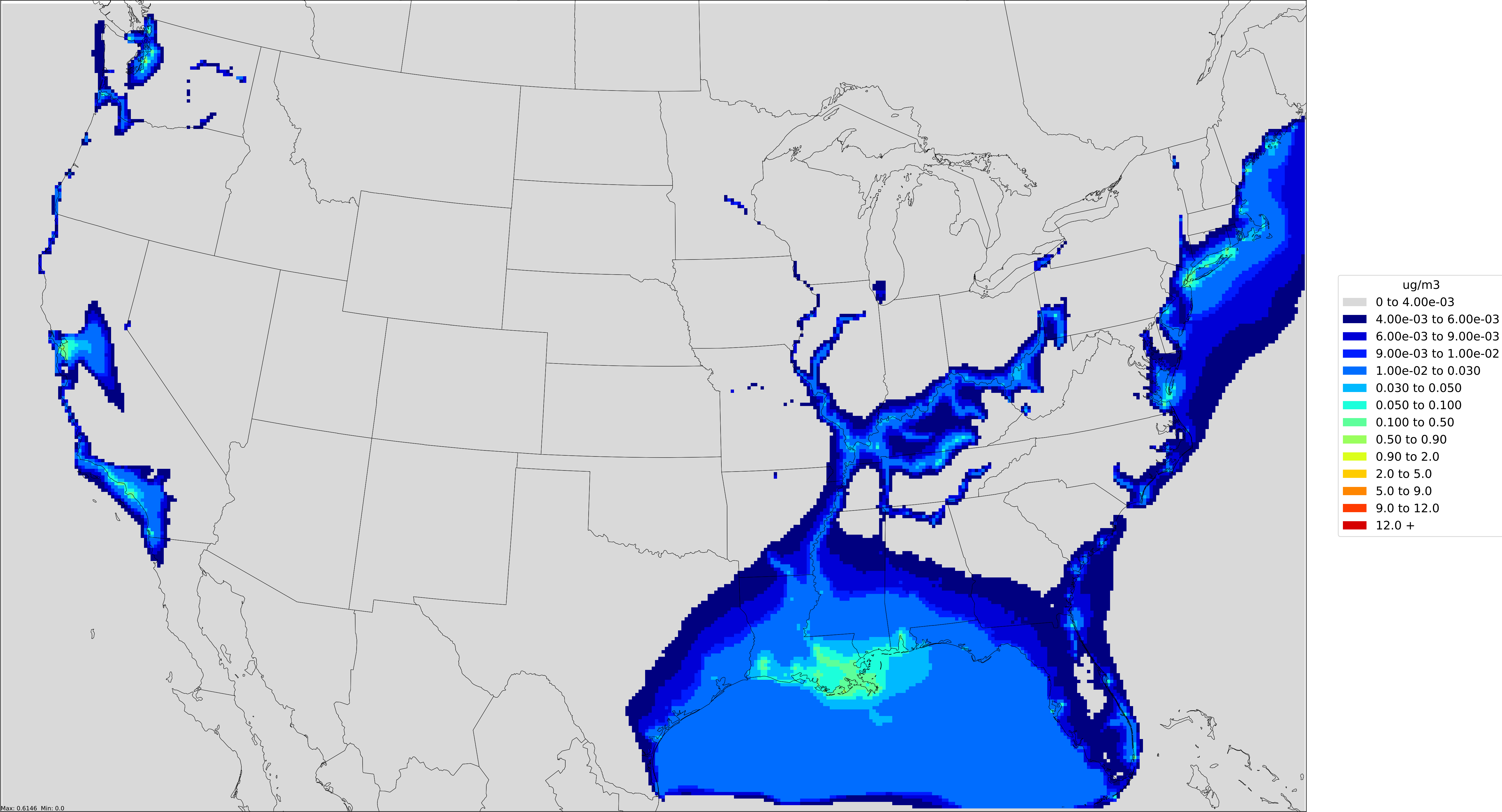
Projected Monthly Average Primary PM2.5 Concentration(ug/m3) in July 2025 C1C2 marine
