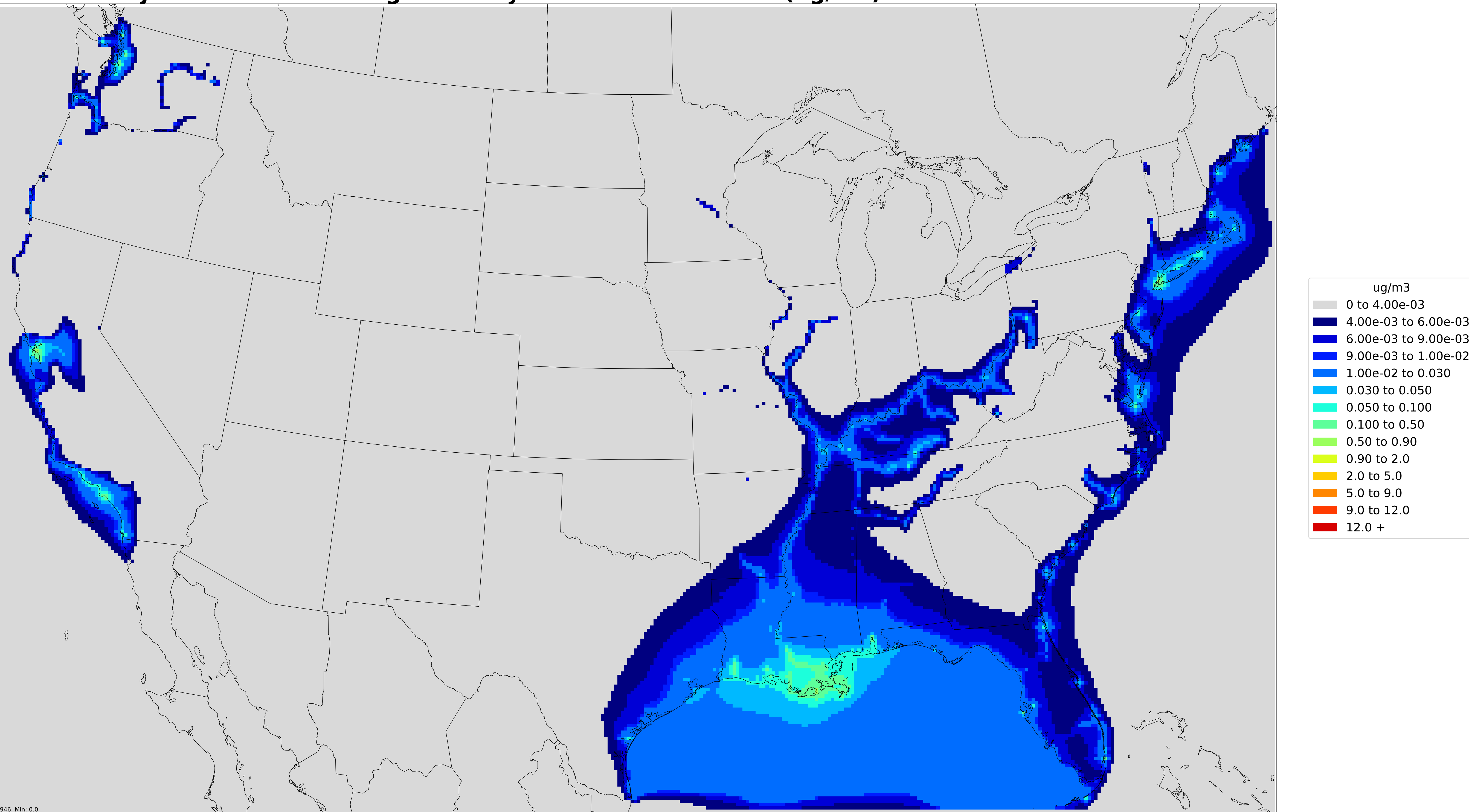
Projected annual average Primary PM2.5 concentration(ug/m3) in 2025 C1C2 marine
