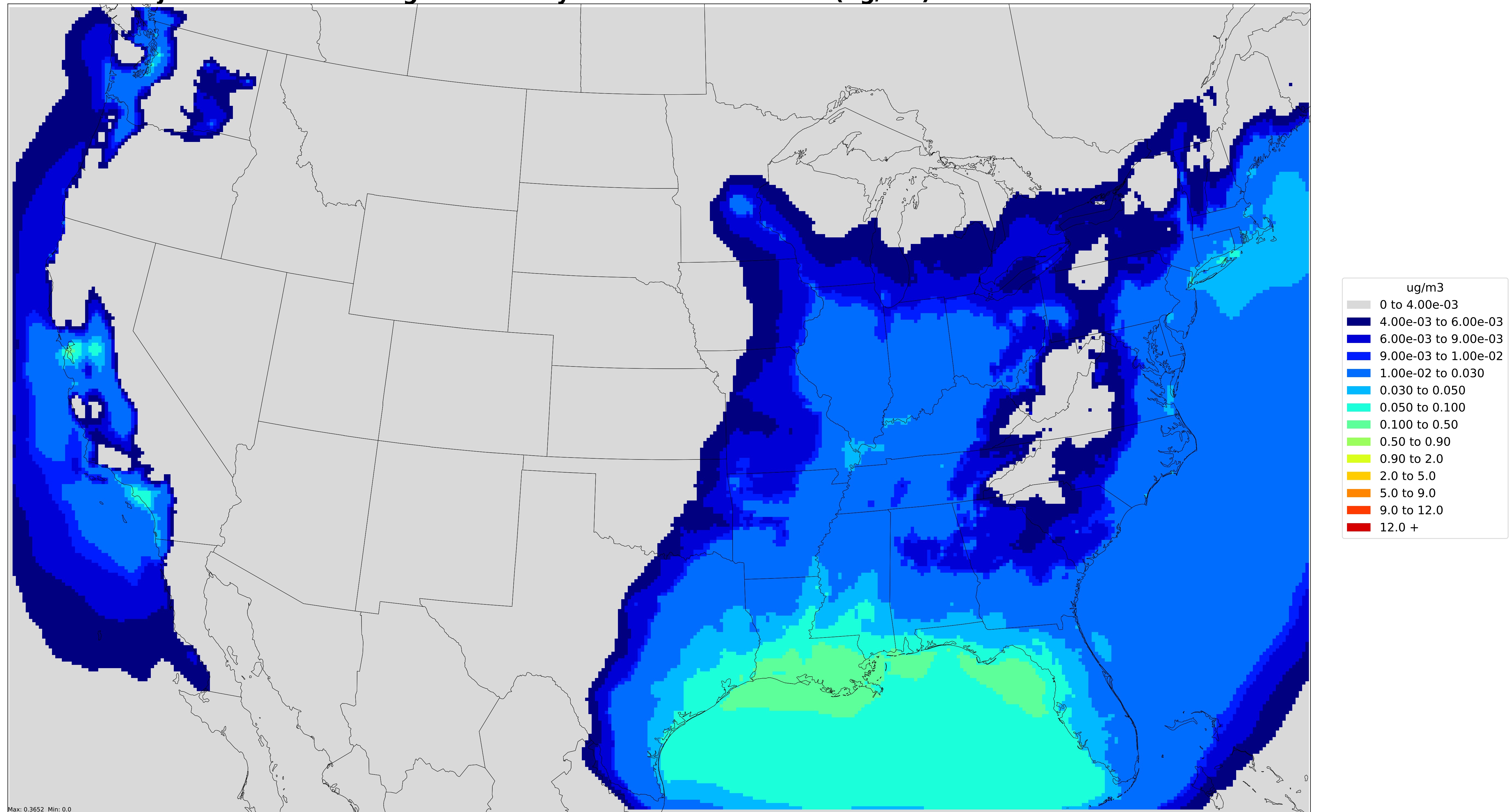
Projected annual average Secondary PM2.5 concentration(ug/m3) in 2025 C1C2 marine
