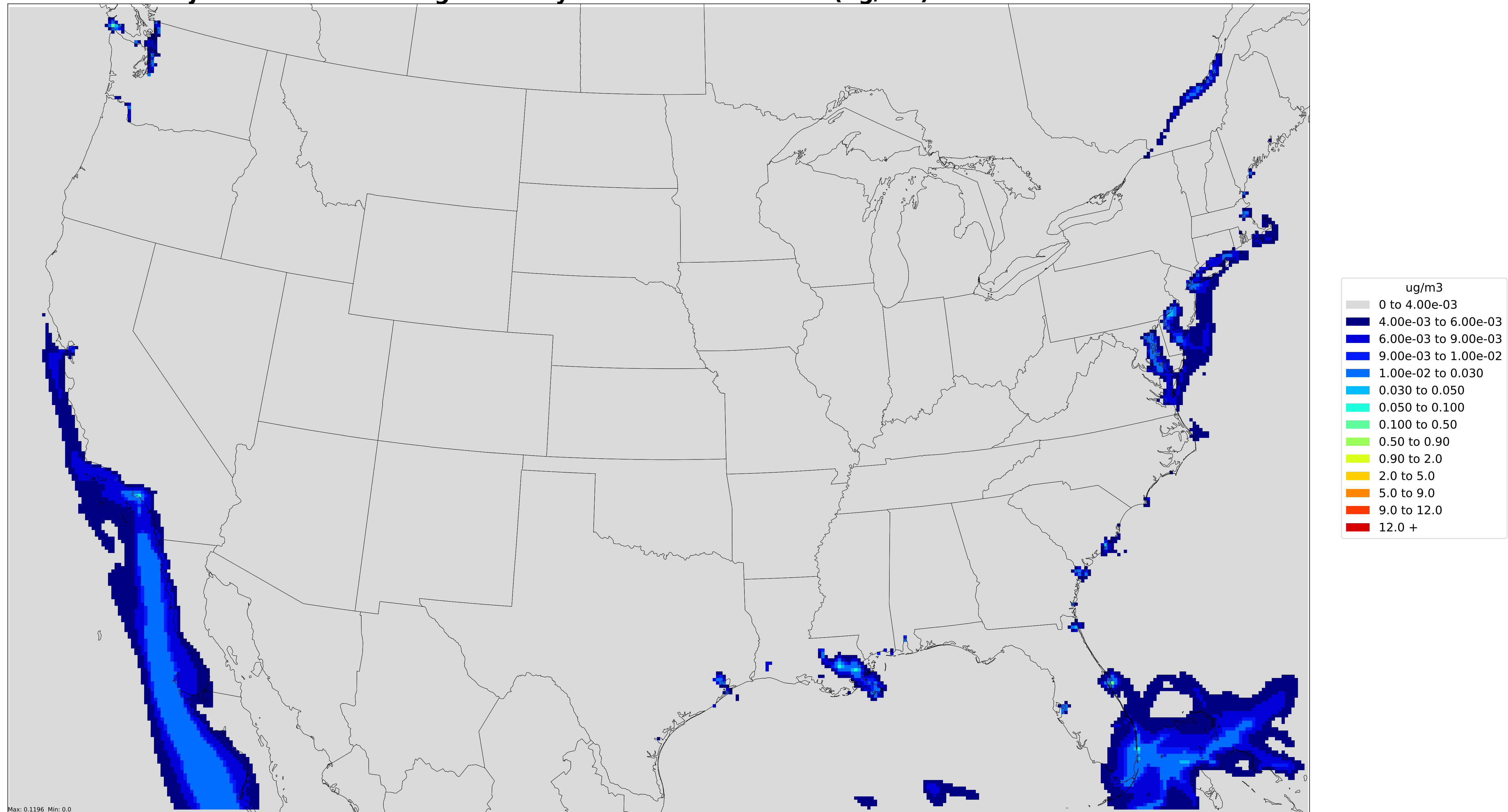
Projected annual average Primary PM2.5 concentration(ug/m3) in 2025 C3 marine
