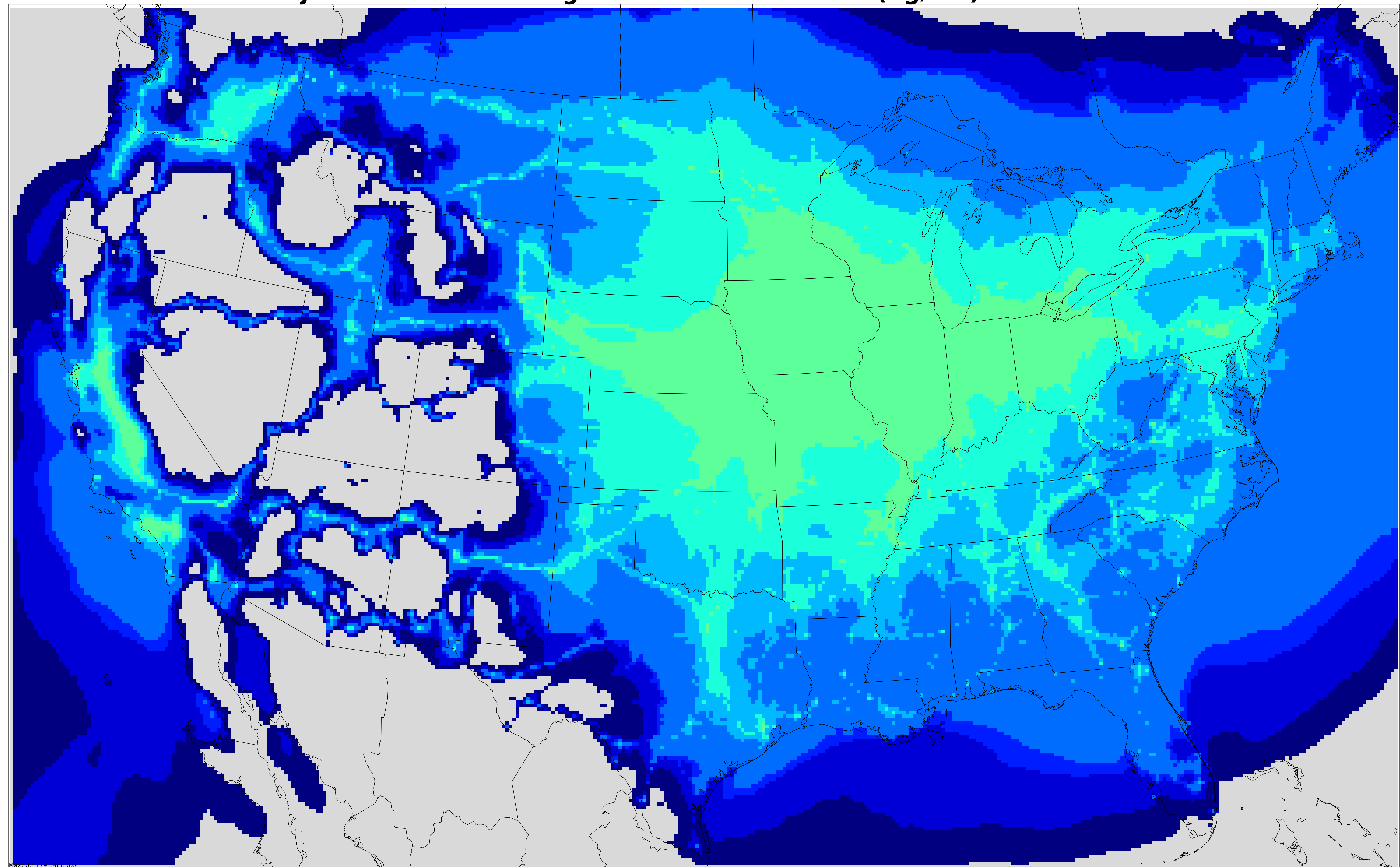
Projected annual average PM2.5 concentration(ug/m3) in 2025 Rail
