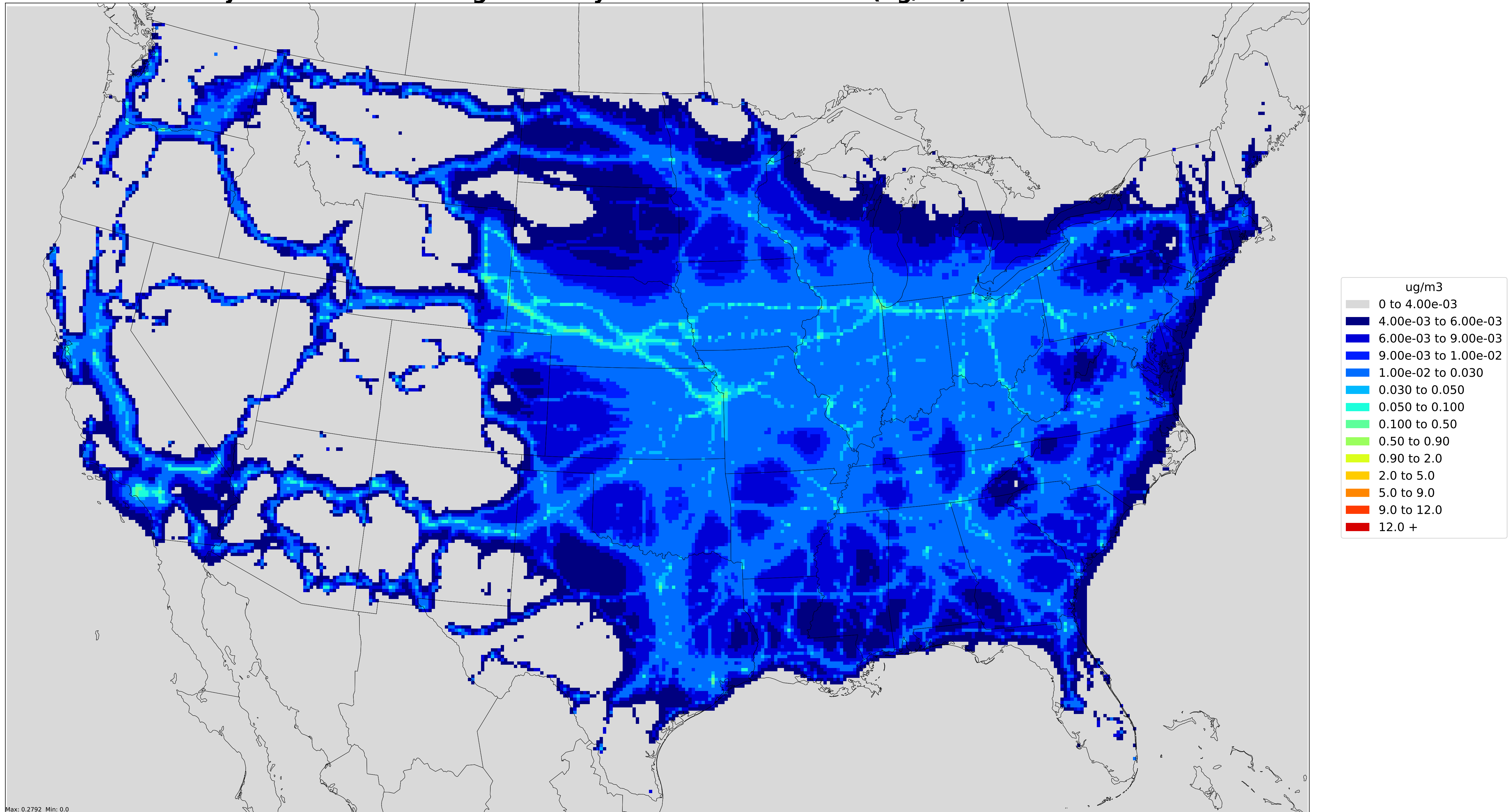
Projected annual average Primary PM2.5 concentration(ug/m3) in 2025 Rail
