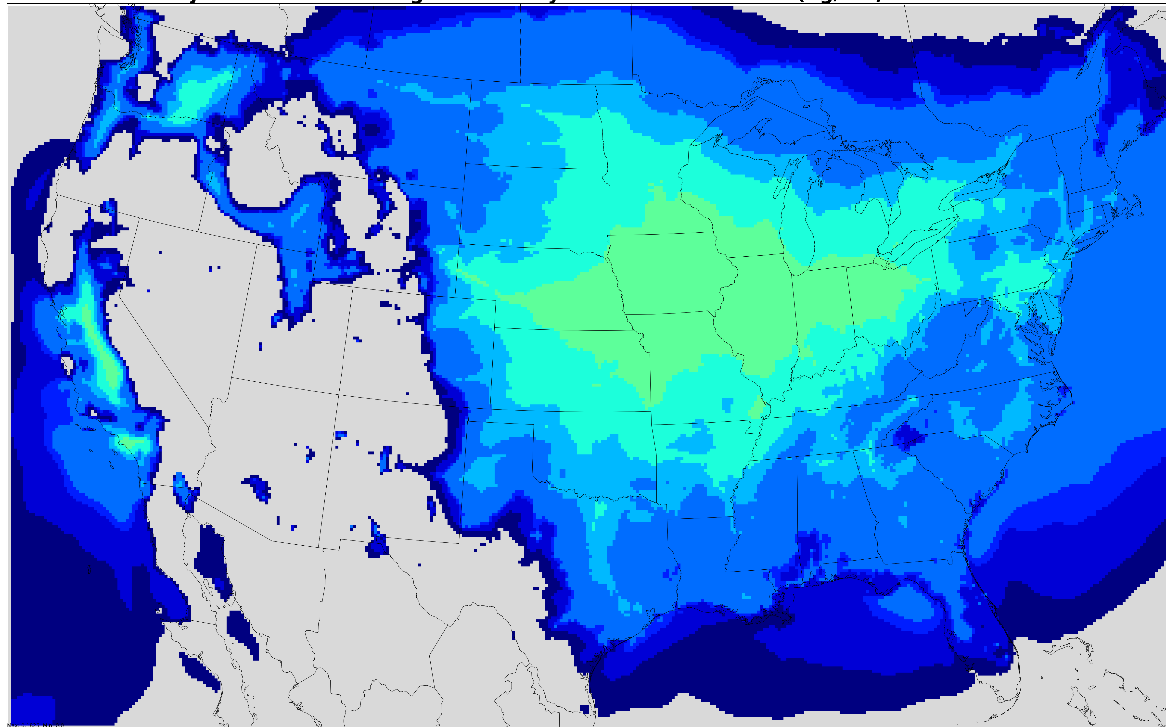
Projected annual average Secondary PM2.5 concentration(ug/m3) in 2025 Rail
