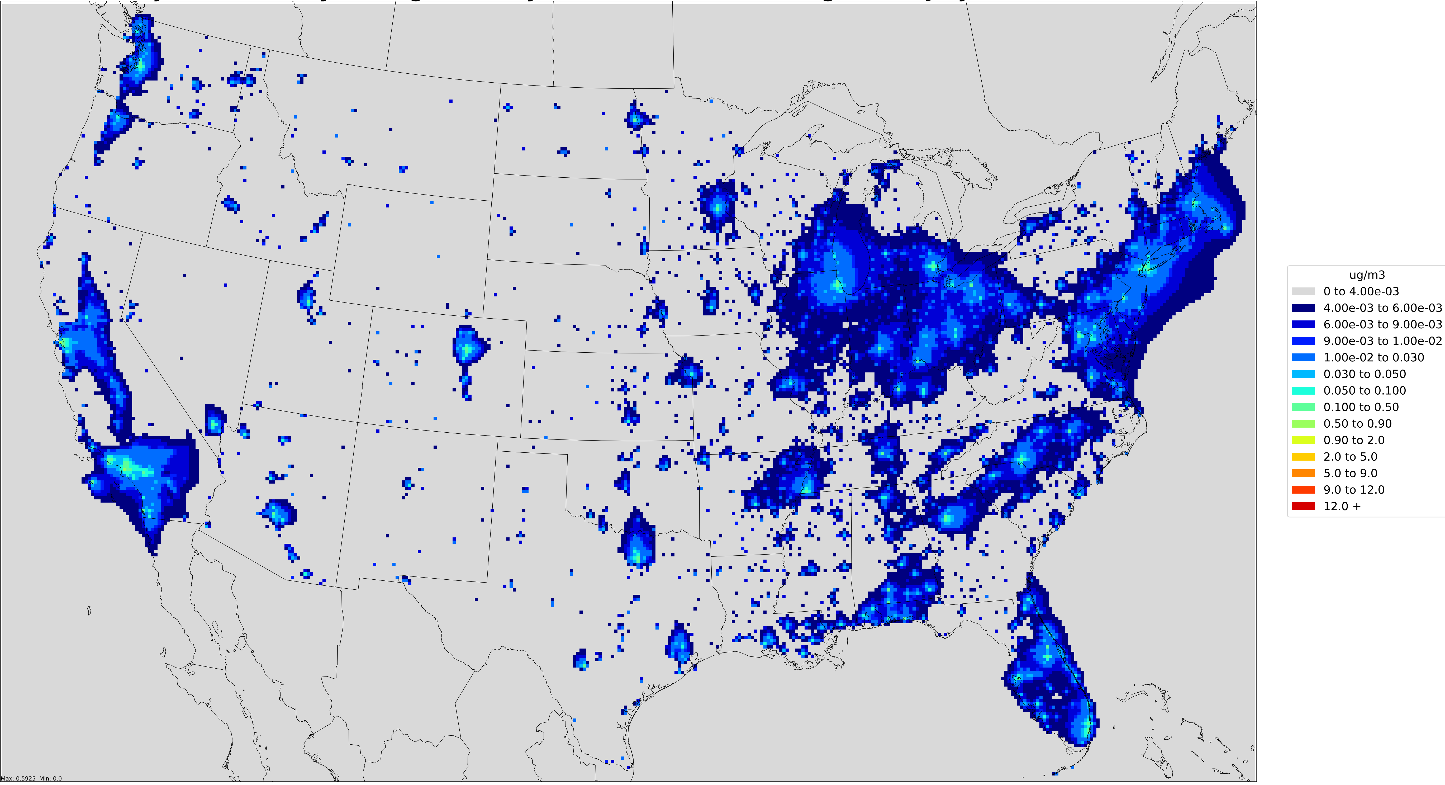
Projected Monthly Average Primary PM2.5 Concentration(ug/m3) in July 2025 Aircraft
