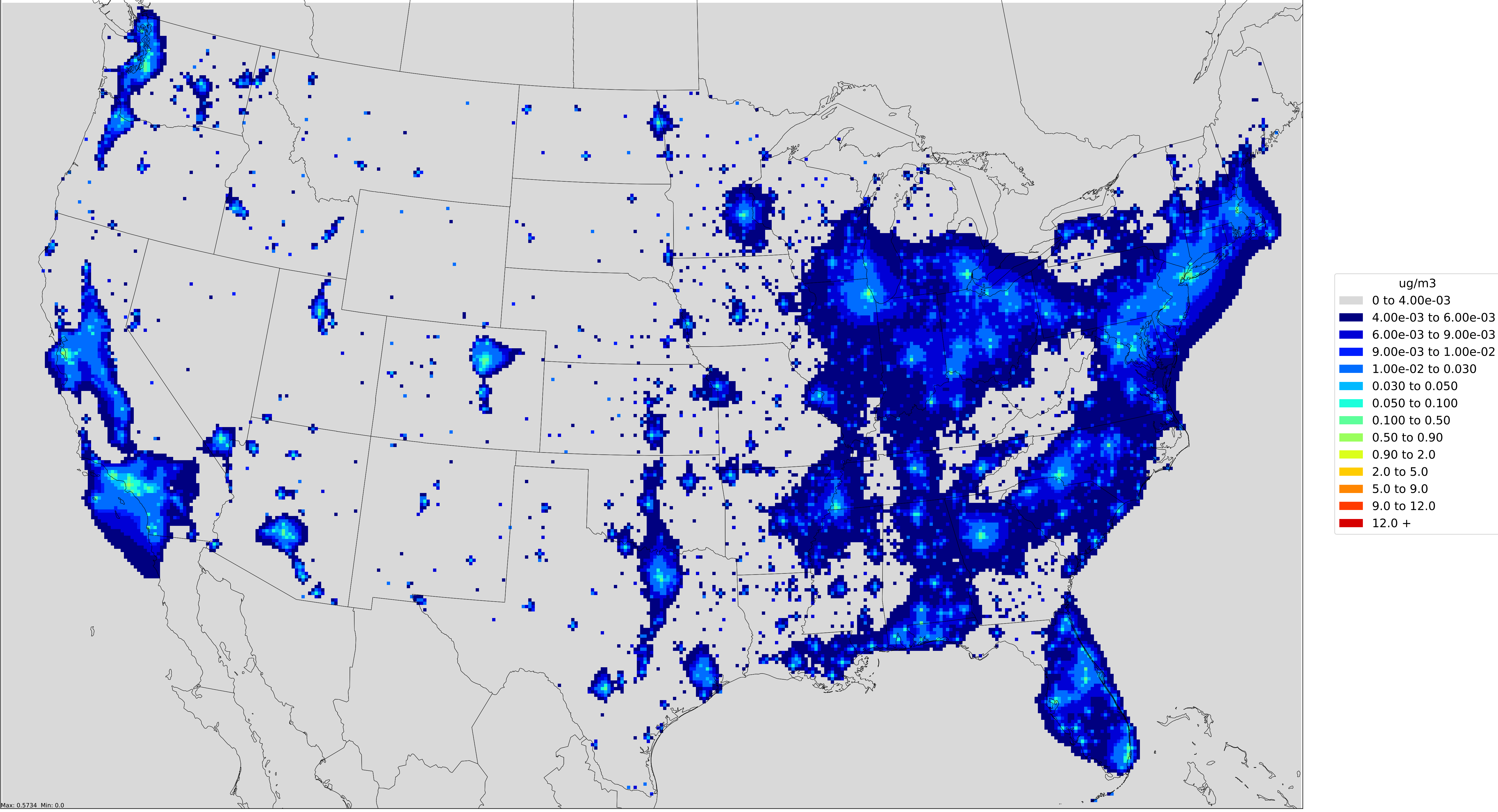
Projected annual average Primary PM2.5 concentration(ug/m3) in 2025 Aircraft
