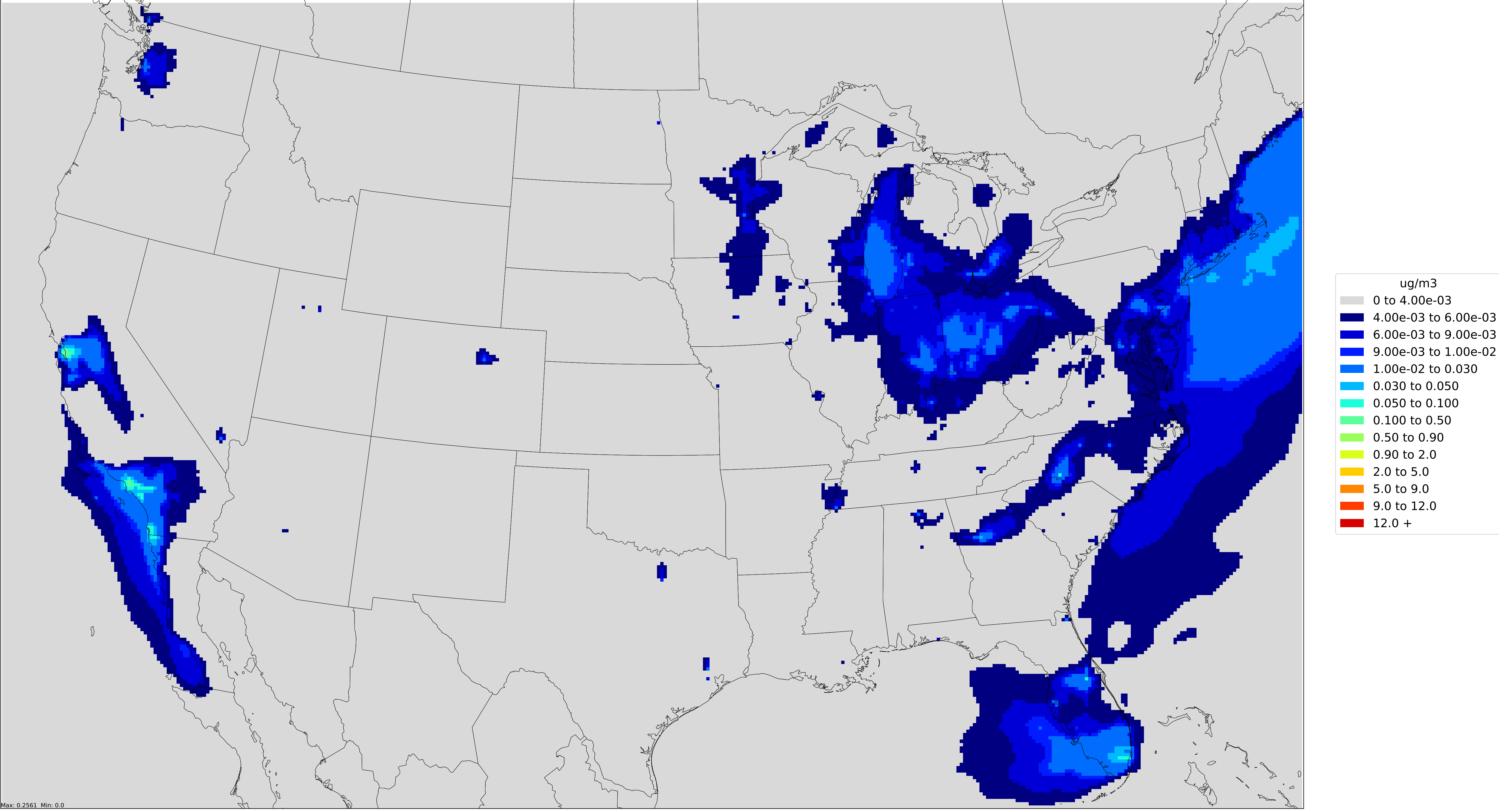
Projected Monthly Average Secondary PM2.5 concentration(ug/m3) in July 2025 Aircraft
